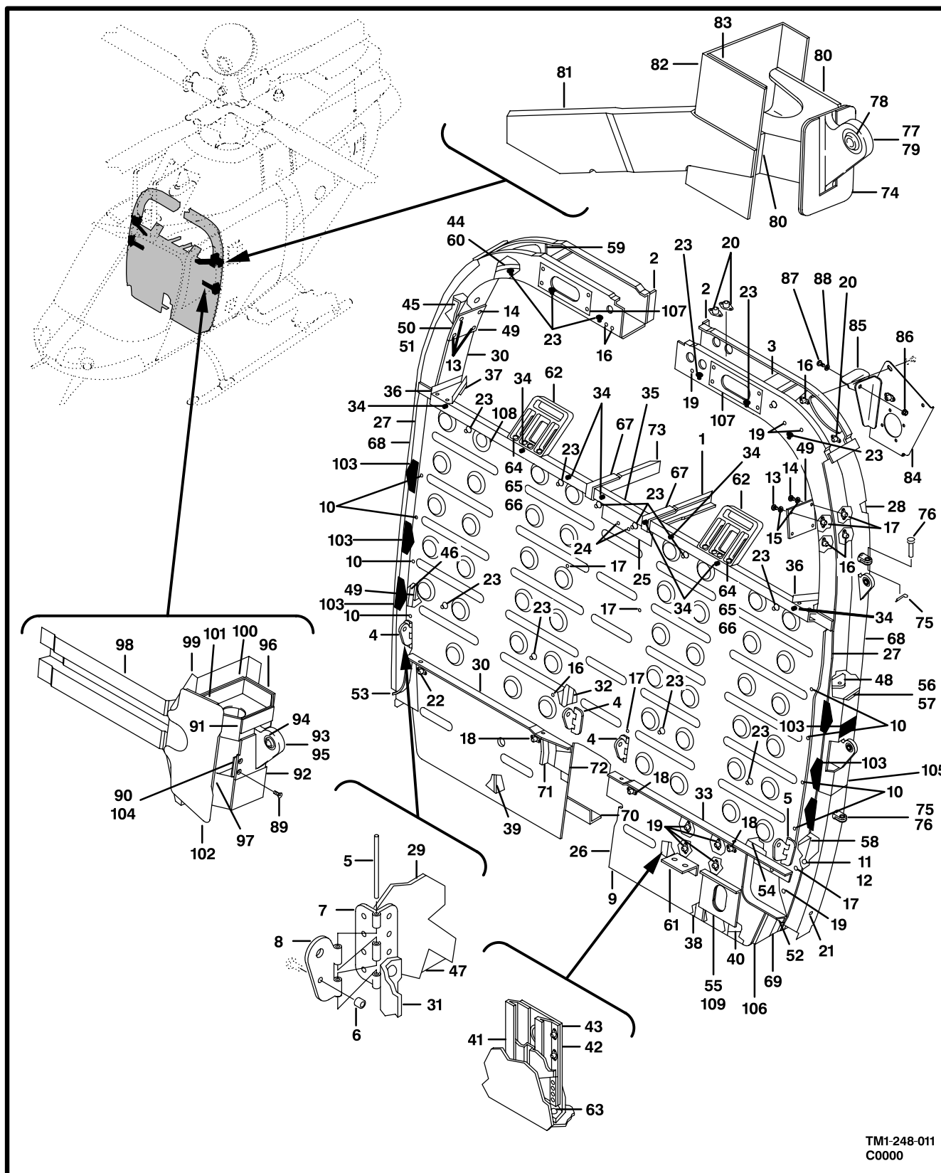
Figure 11. Bulkhead Installation
