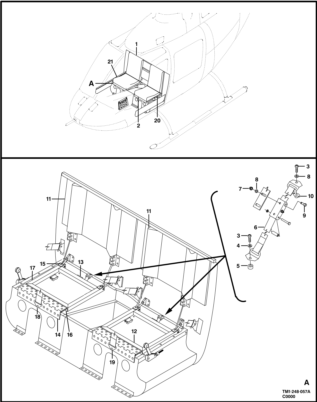
Figure 57A. CrewSeat MOD, Energy Attenuating
