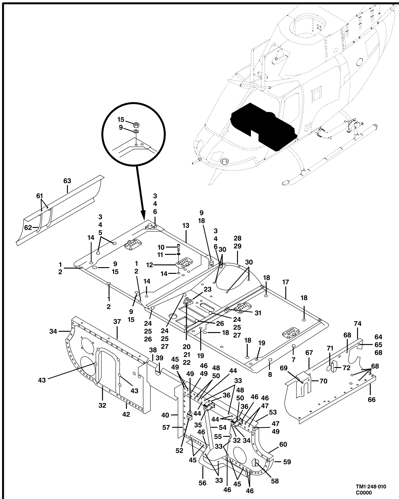
Figure 10. Seat Installation, Pilot and Copilot
