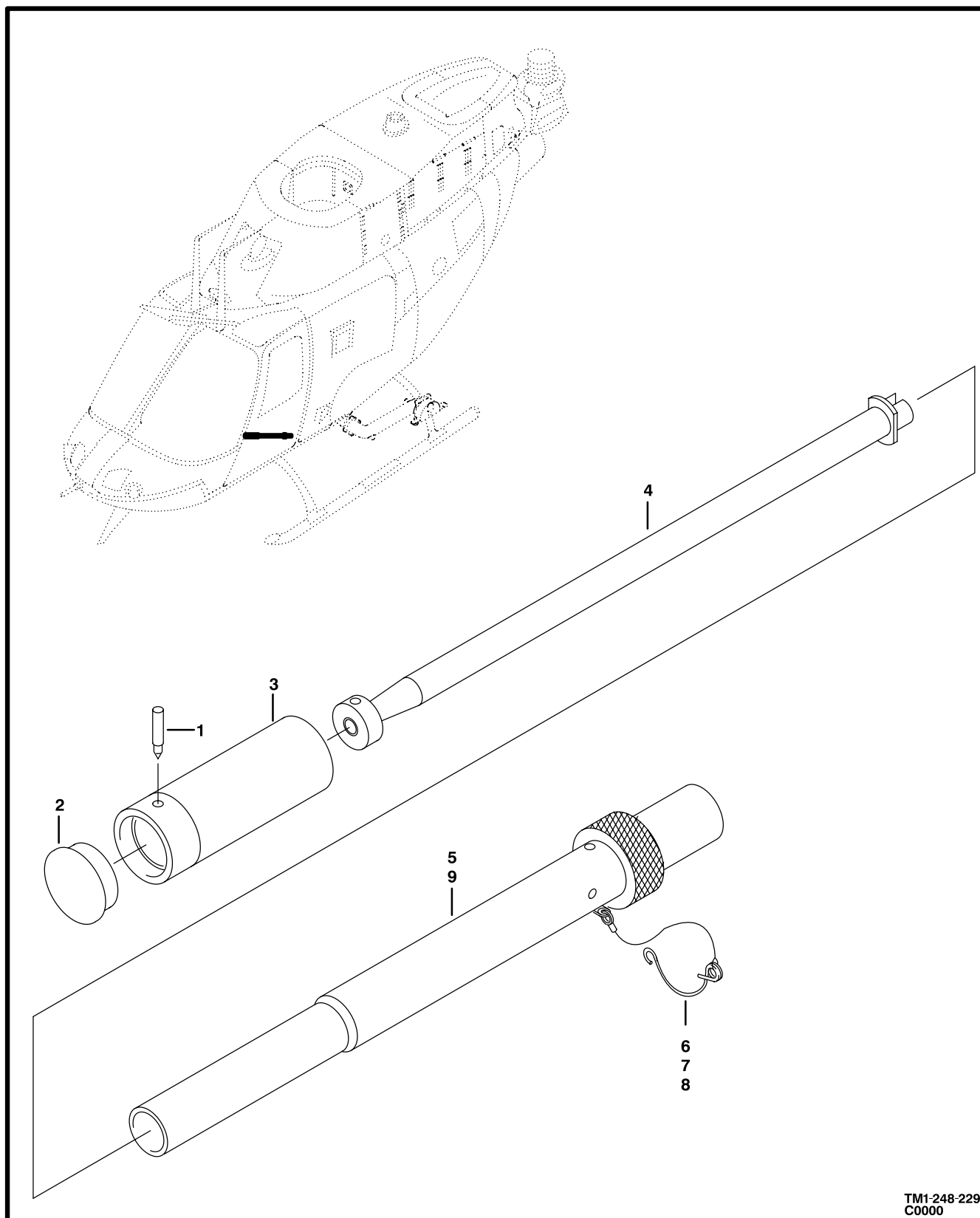
Figure 247. Stick Assembly, Copilot
