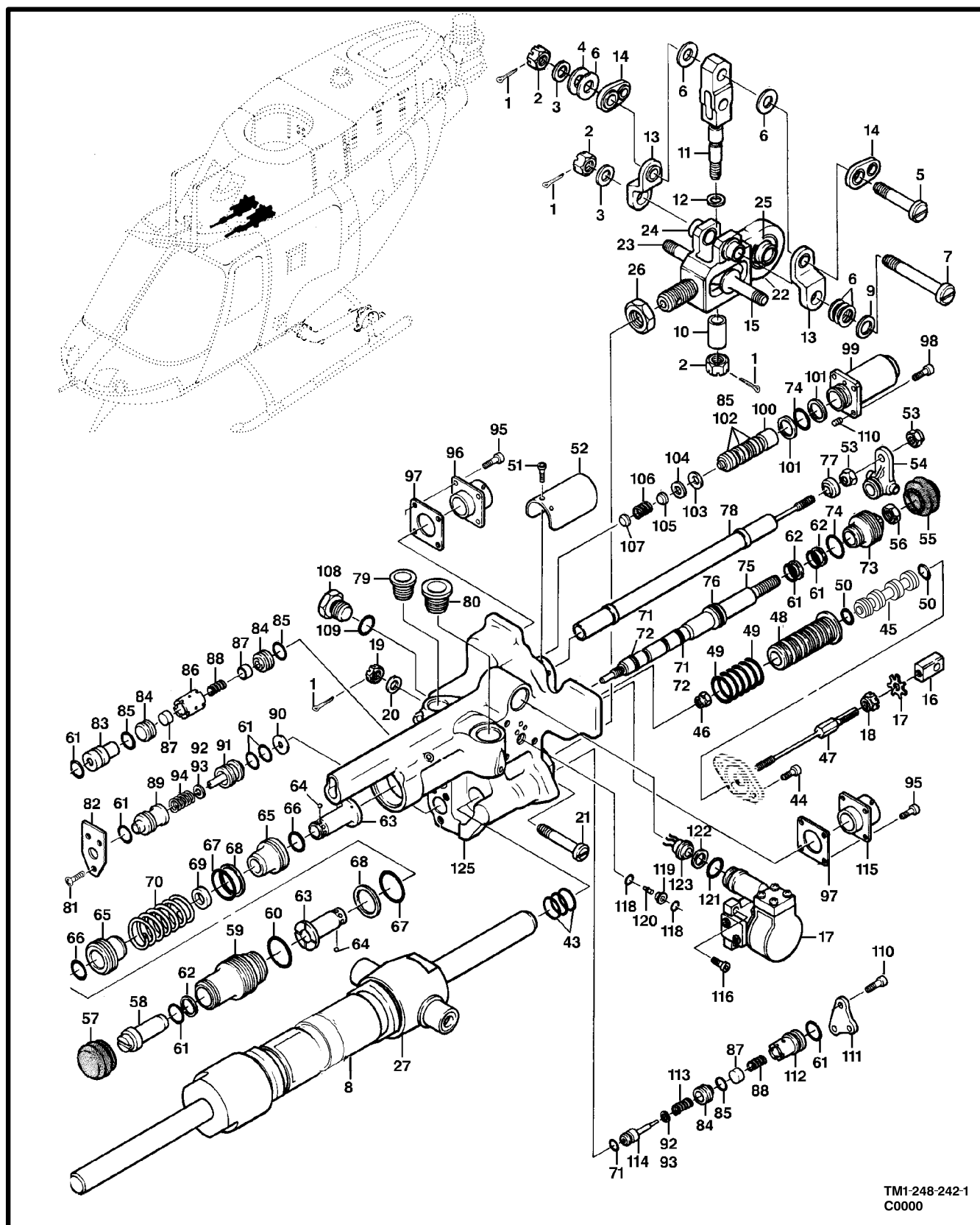
Figure 259. Actuator Assembly
