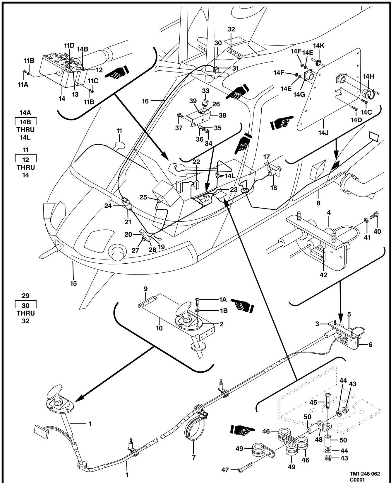
Figure 61. MOD-Cargo Hook Provisions
