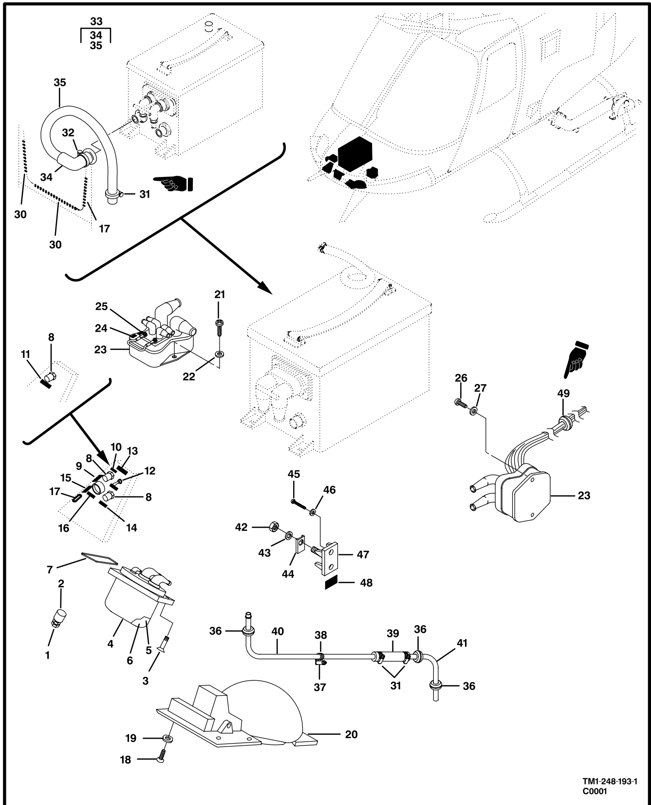
Figure 188. Electrical and Avionics Installation, Nose Compartment and Pedestal (Sheet 1 of 2)
