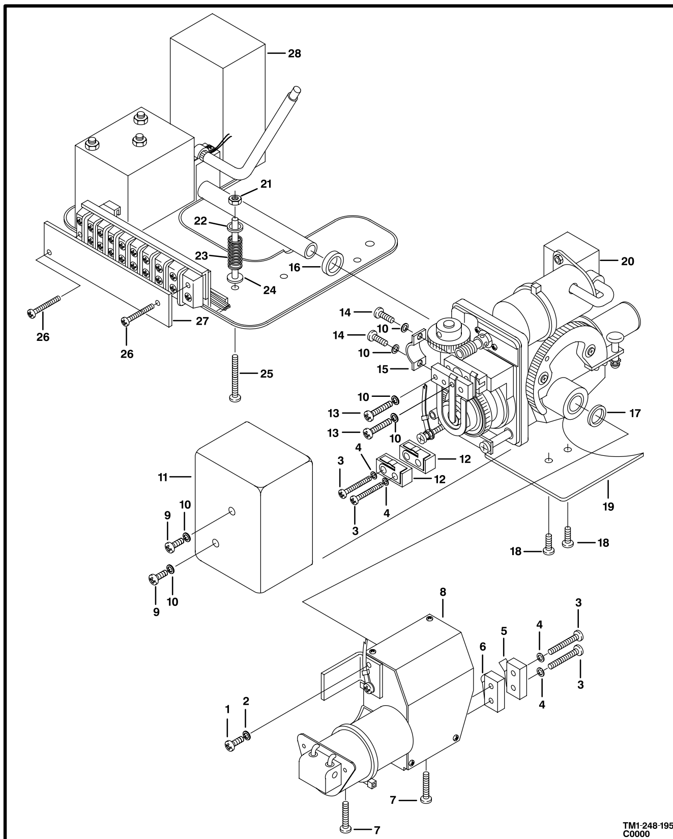
Figure 190. Motor Assembly, Dual
