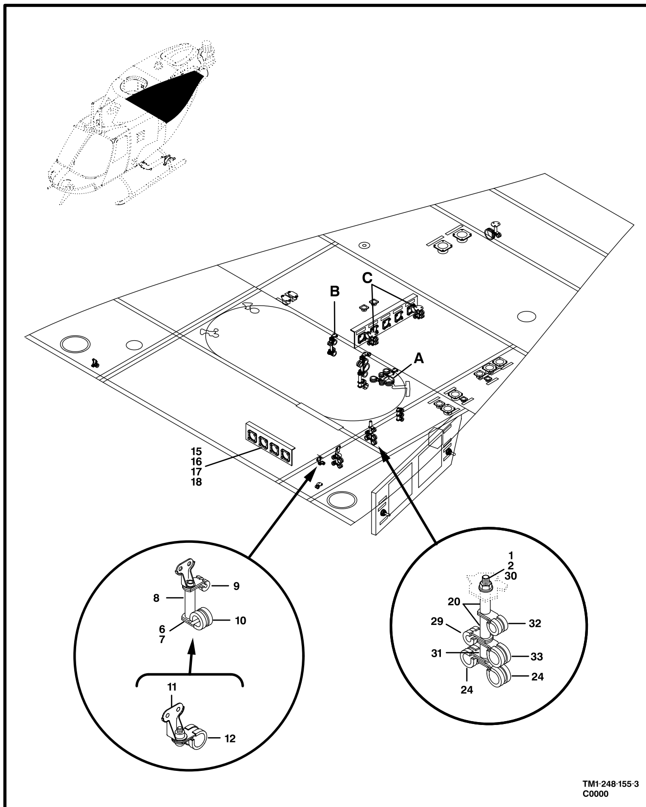
Figure 150. Electrical Installation,Canted Web (Sheet 3 of 5)
