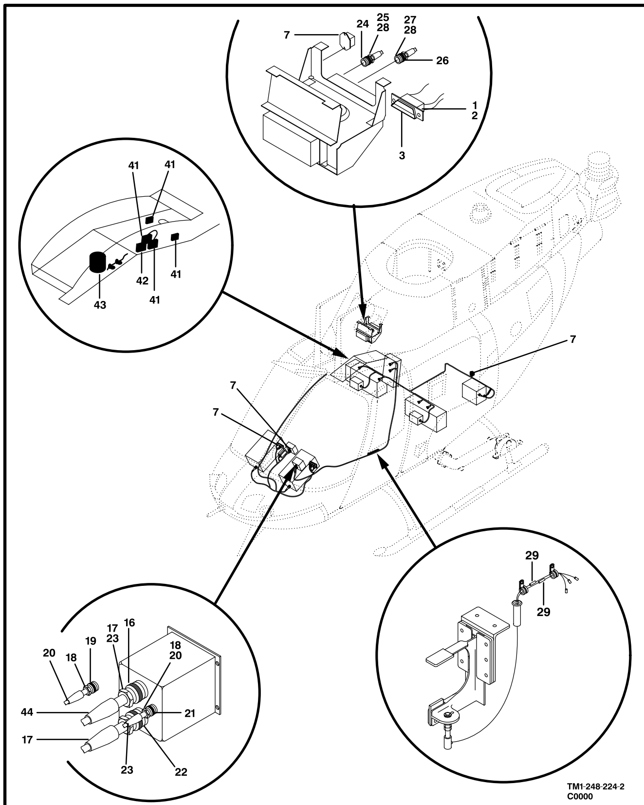
Figure 218. Cable Assembly,Control Display System (Sheet 2 of 2)
