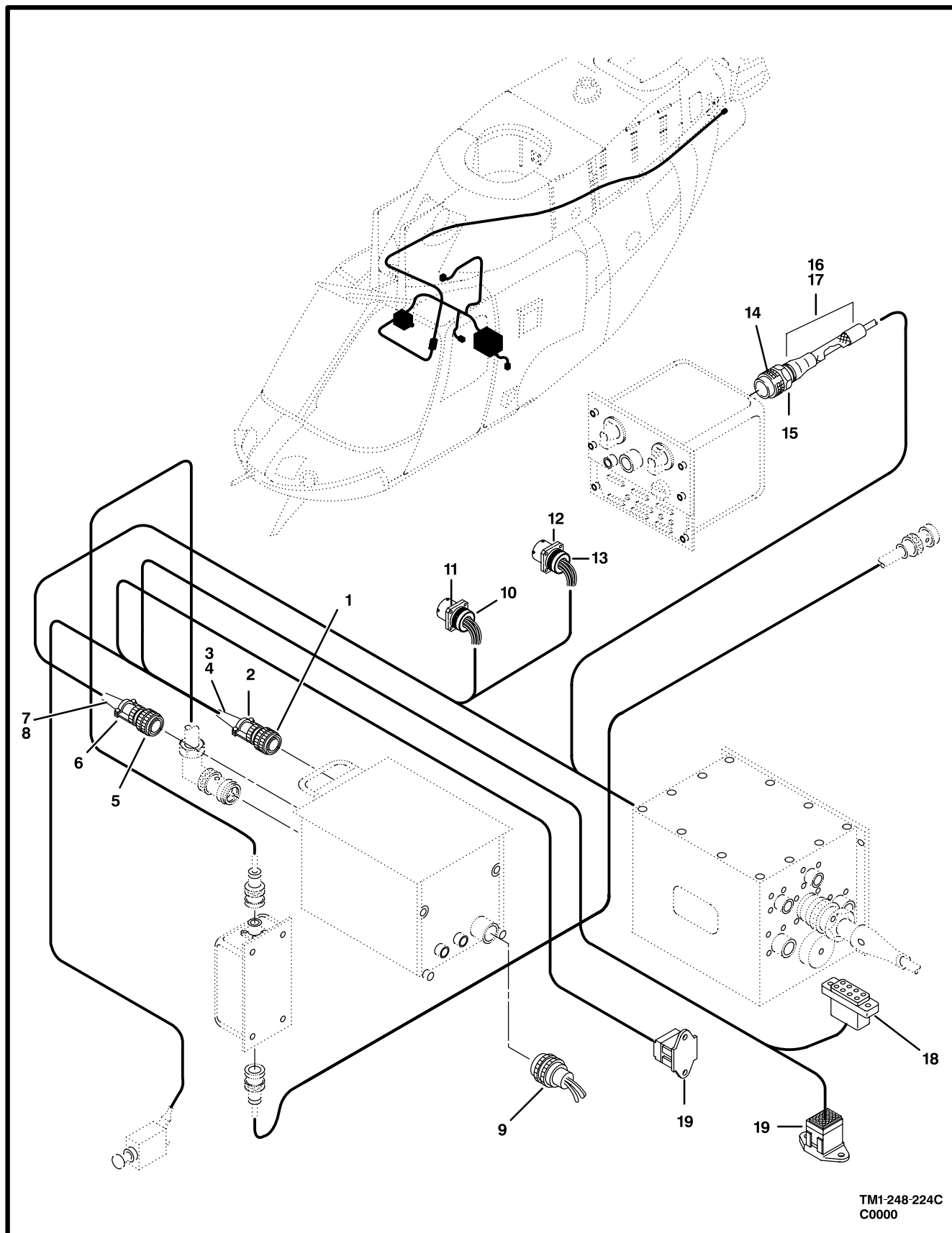
Figure 221. Cable Assembly,VHF-FM Communication System
