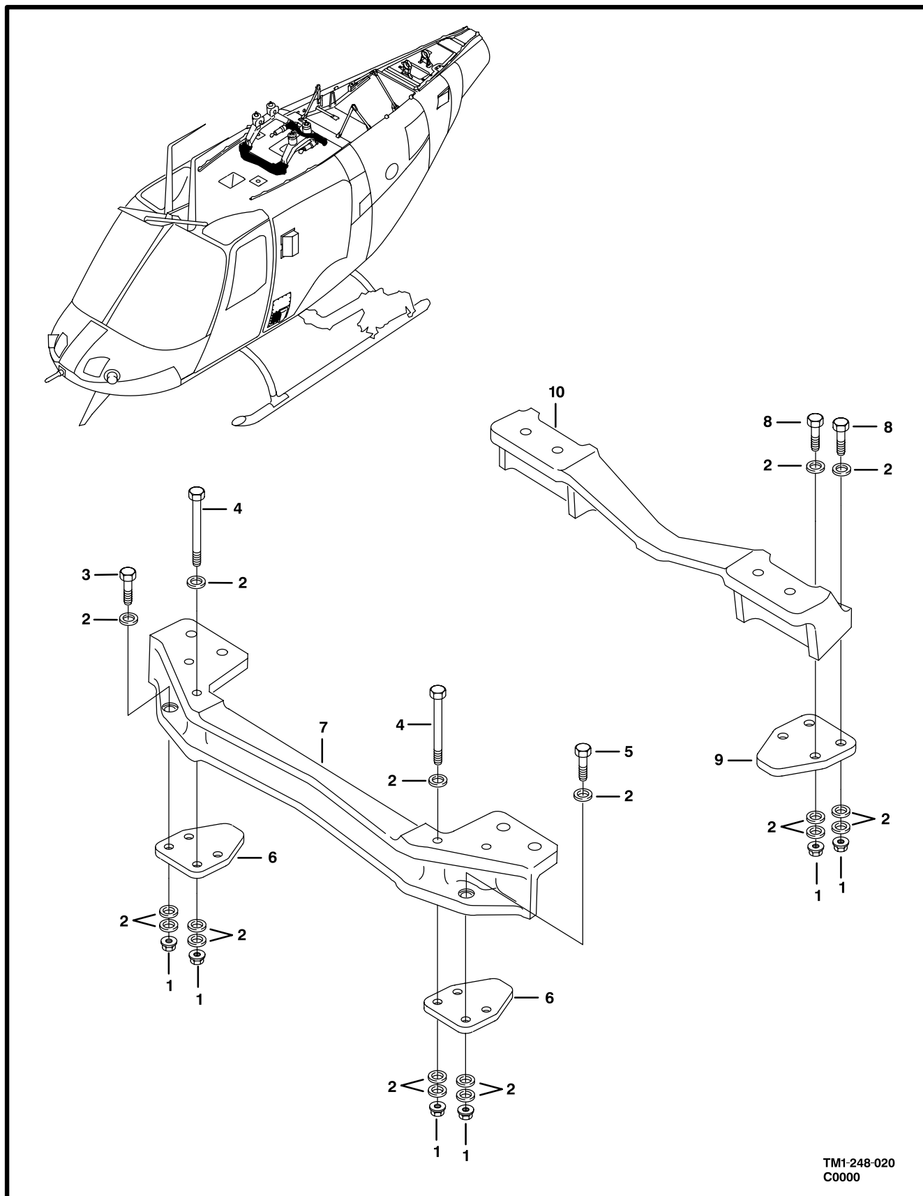
Figure 20. Beam Installation, Transverse
