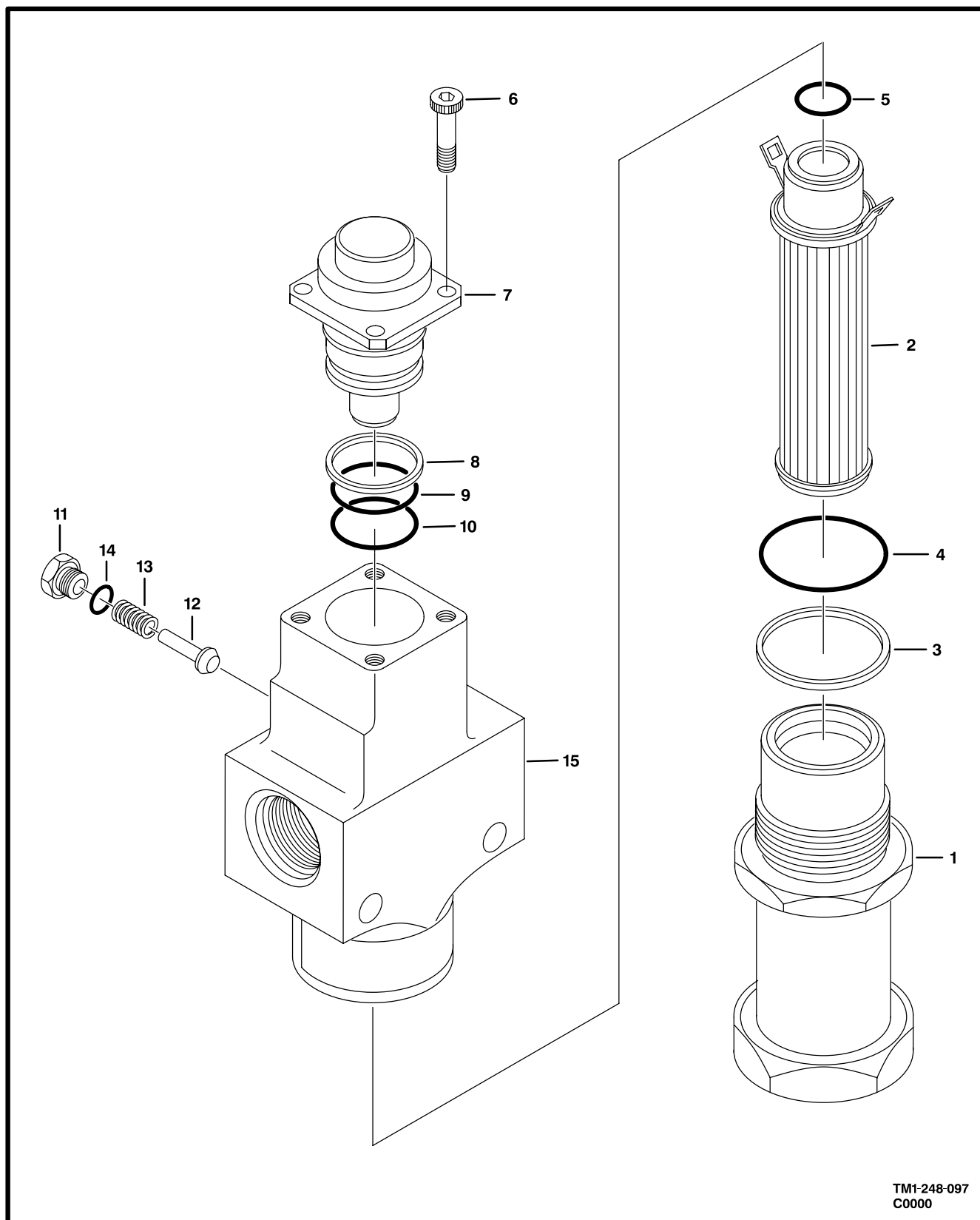
Figure 94. Fluid Filter Assembly
