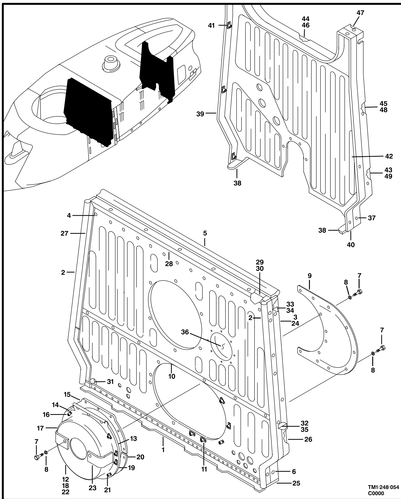
Figure 53. Firewall Installation, FWD
