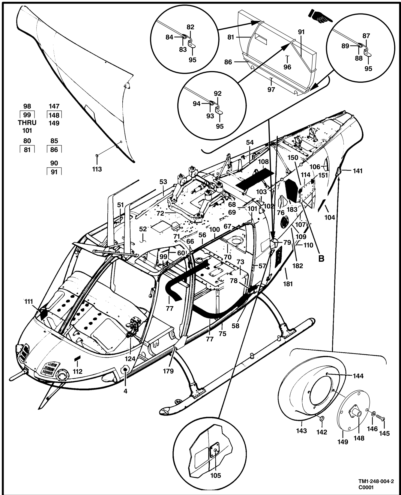
Figure 4. Structure Assembly, Fuselage (Sheet 2 of 4)
