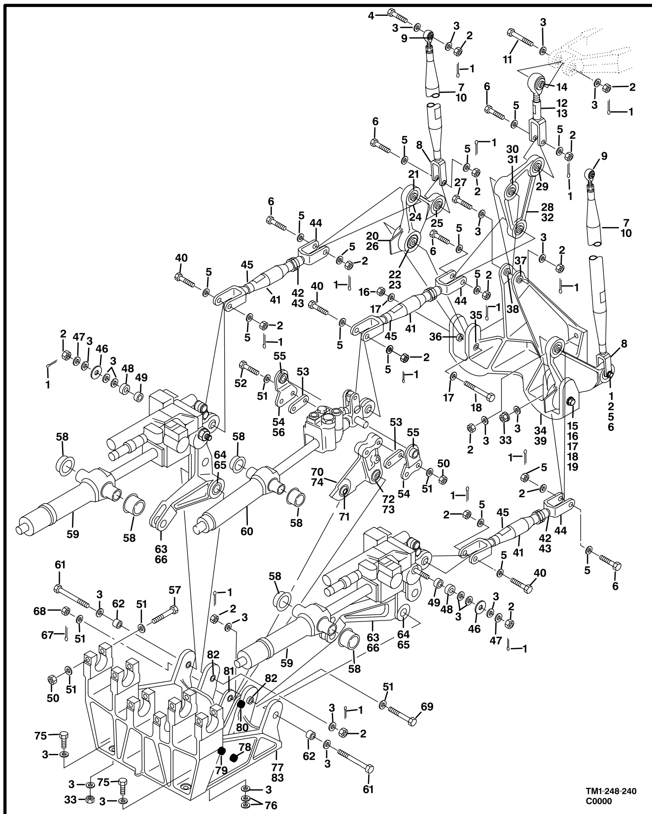
Figure 257. Controls Installation, Collective And Cyclic
