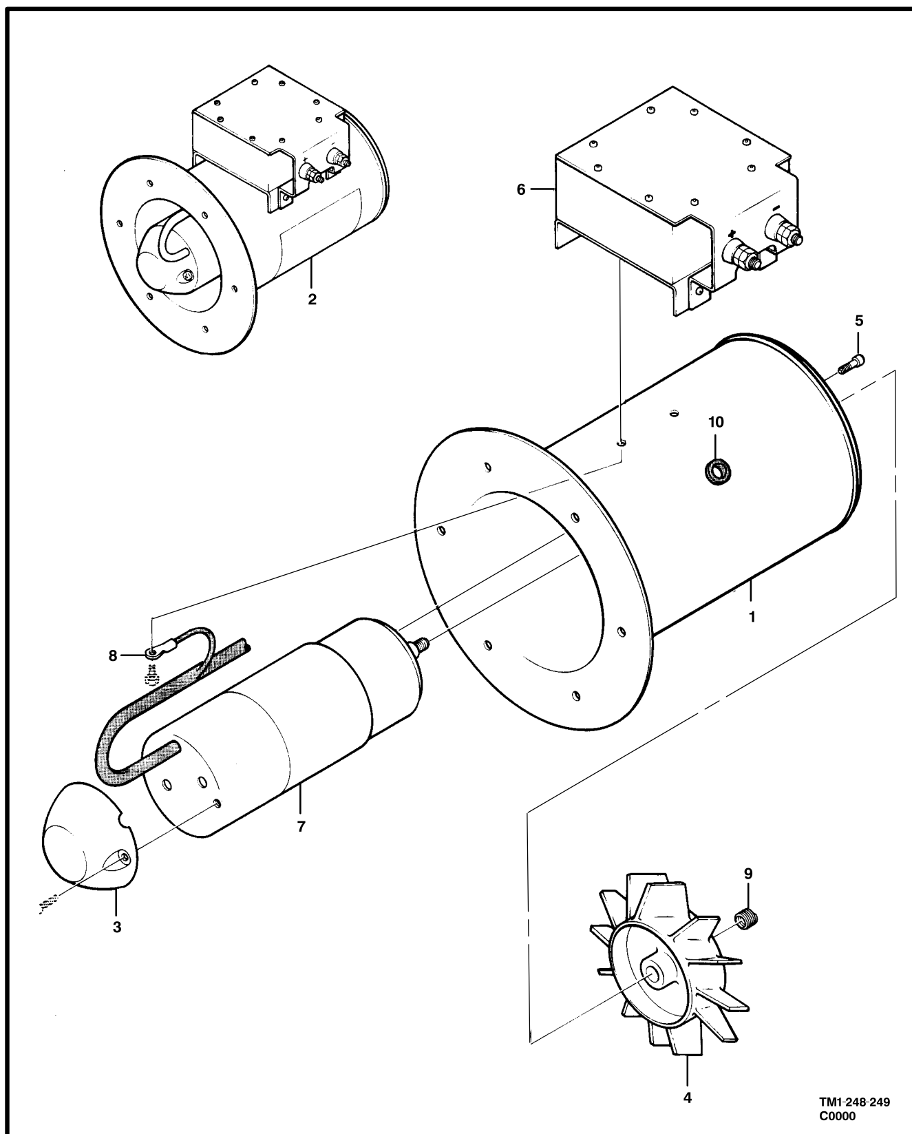
Figure 265. Blower Assembly,Avionics Cooling
