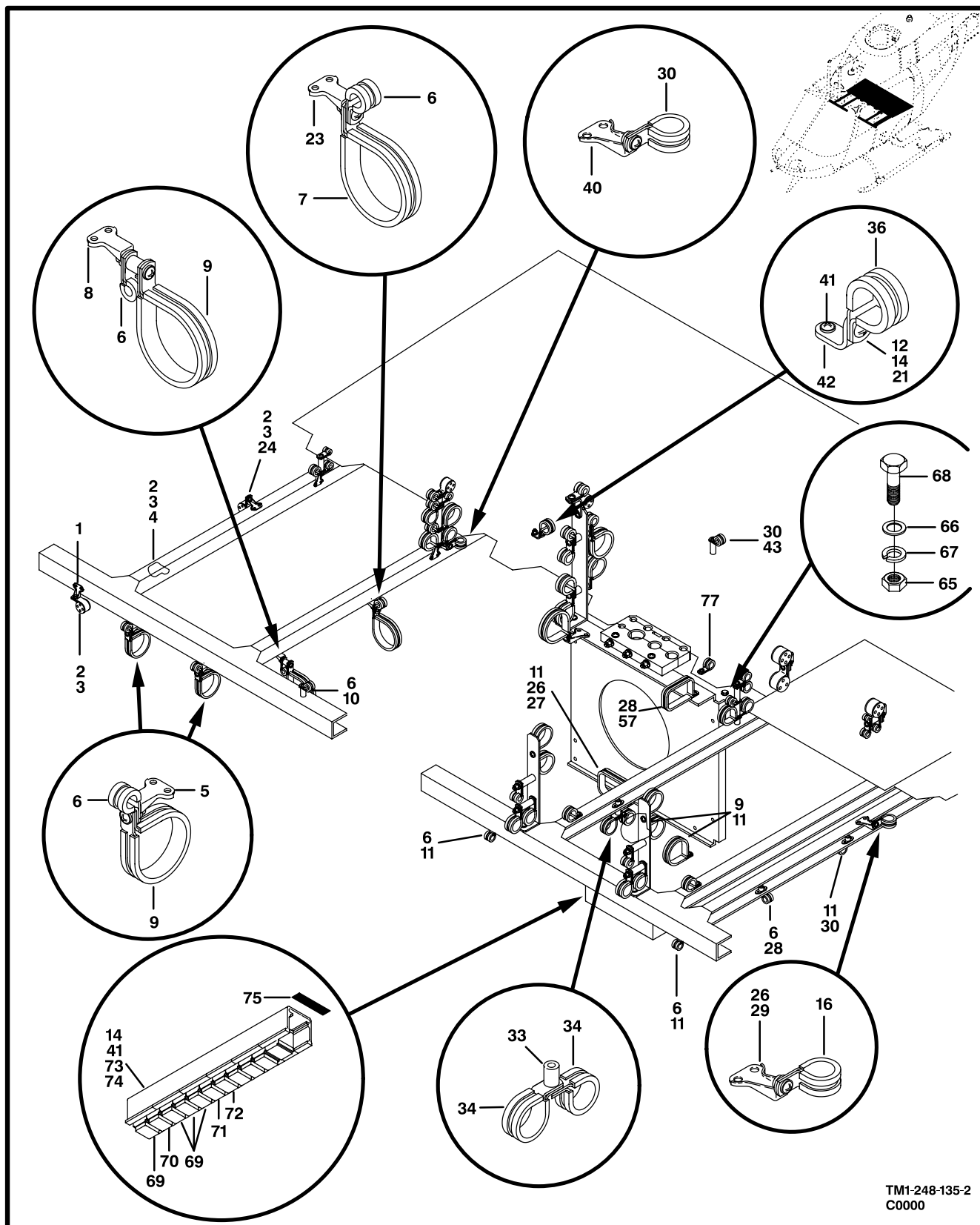
Figure 130. Electrical Installation, Shelf (Sheet 2 of 2)
