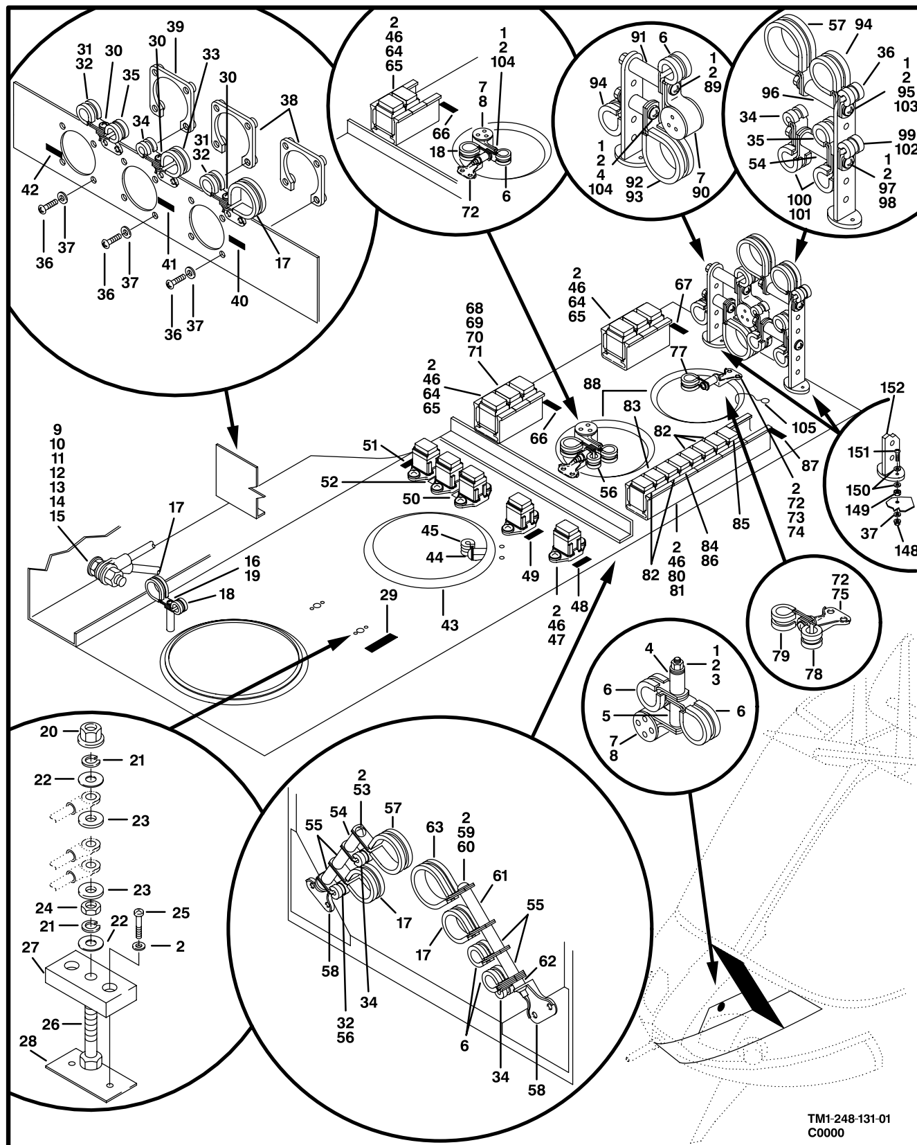
Figure 126. Electrical Installation, Nose (Sheet 1 of 2)
