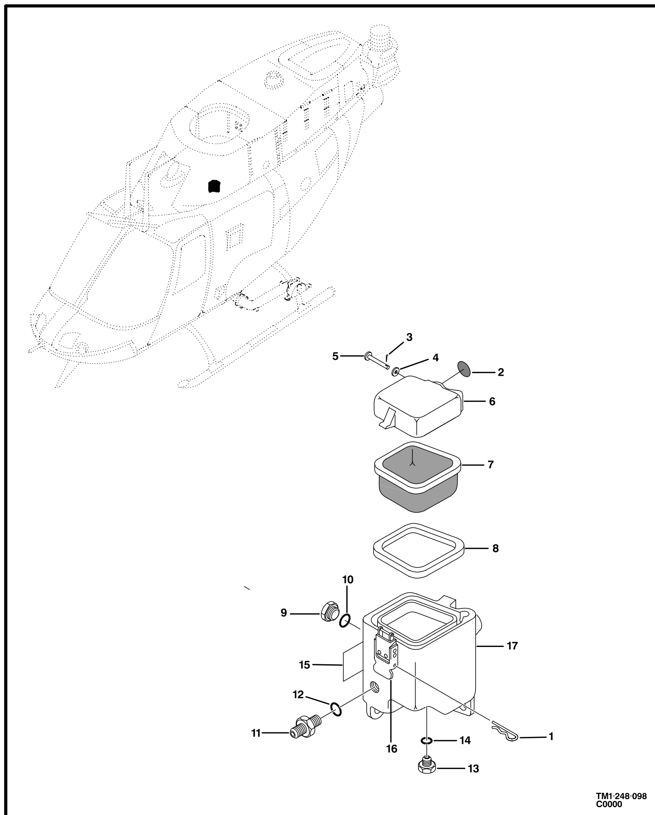
Figure 95. Reservoir Assembly
