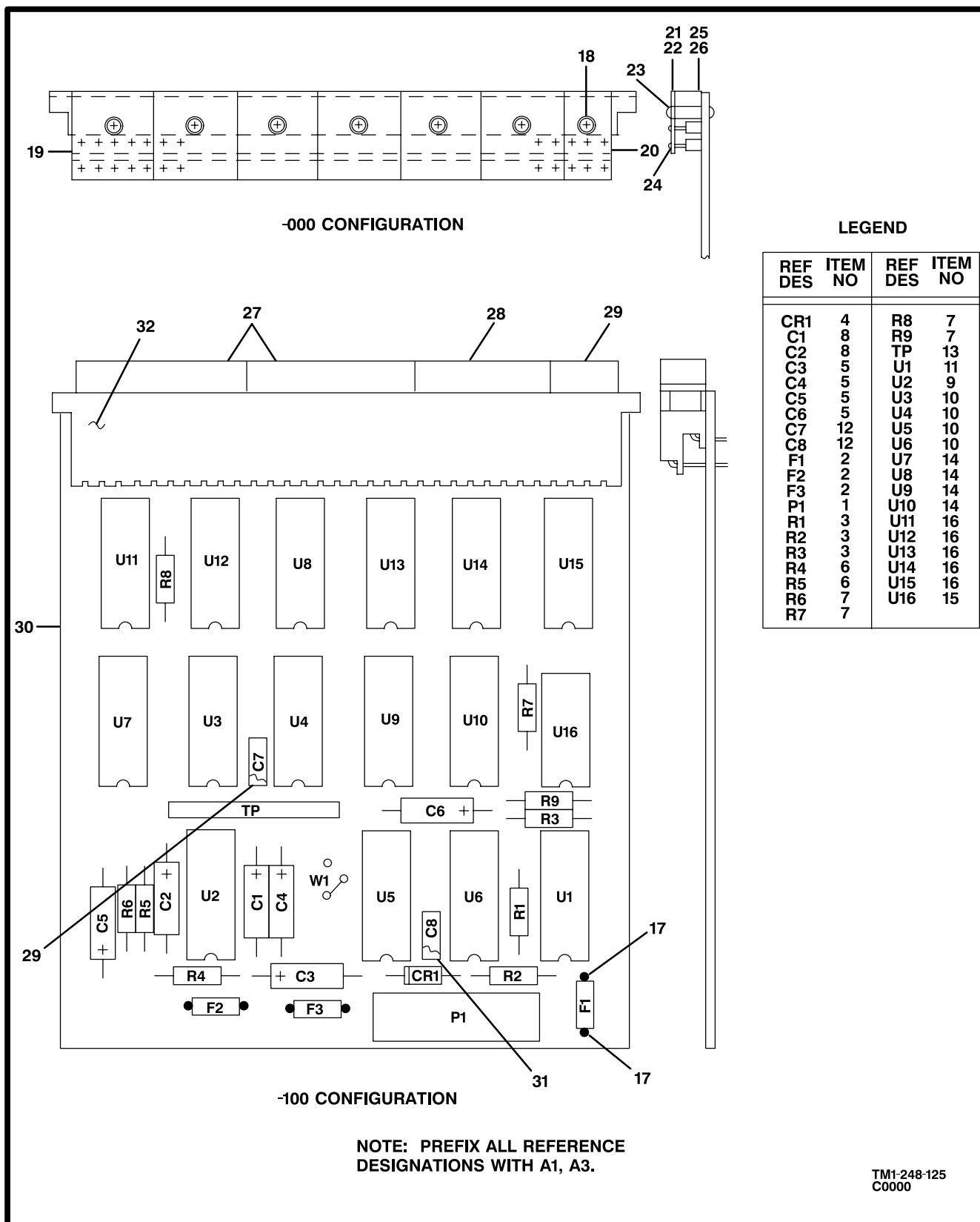
Figure 120. Driver, 33 Lamp
