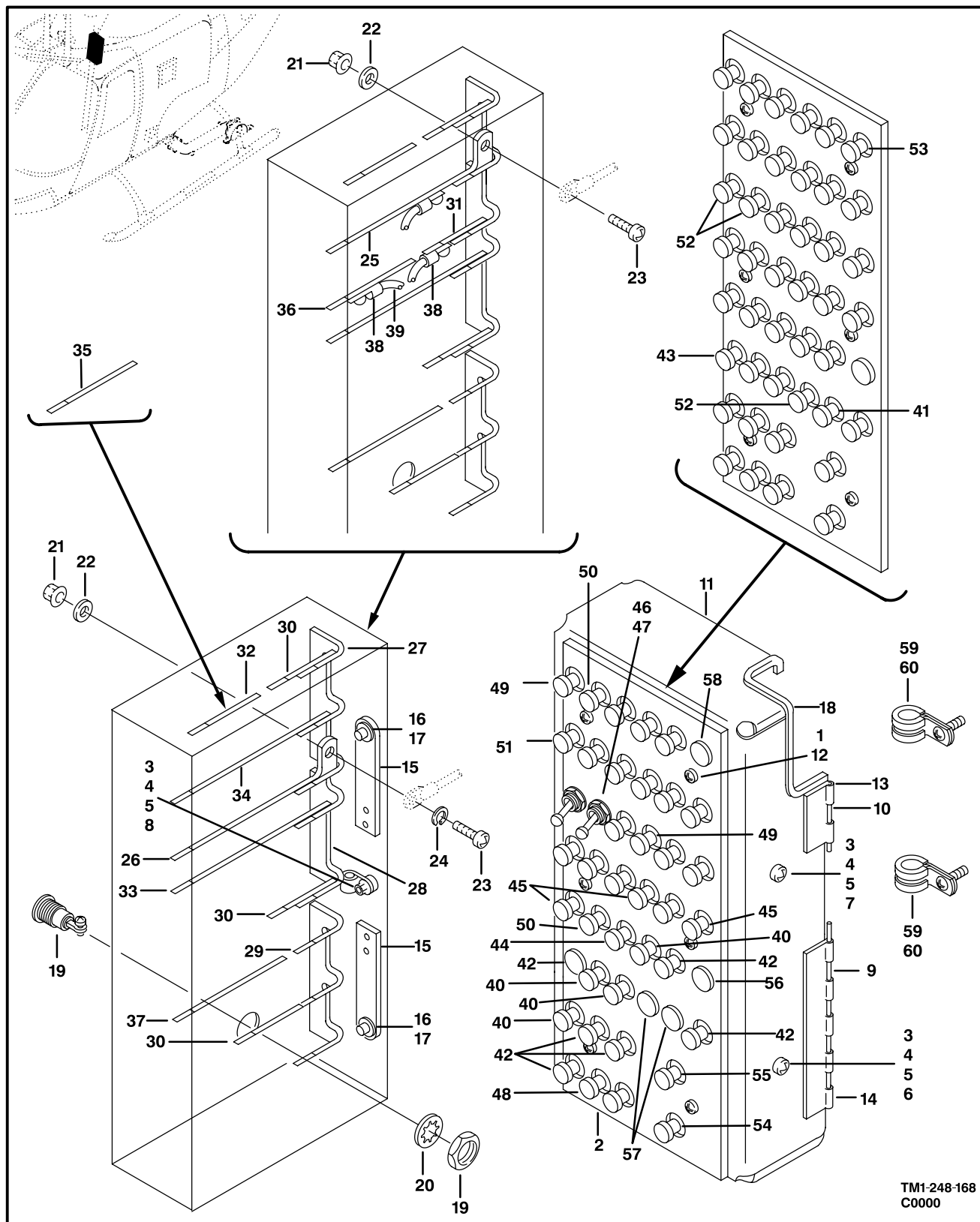
Figure 163. Circuit Breaker Installation
