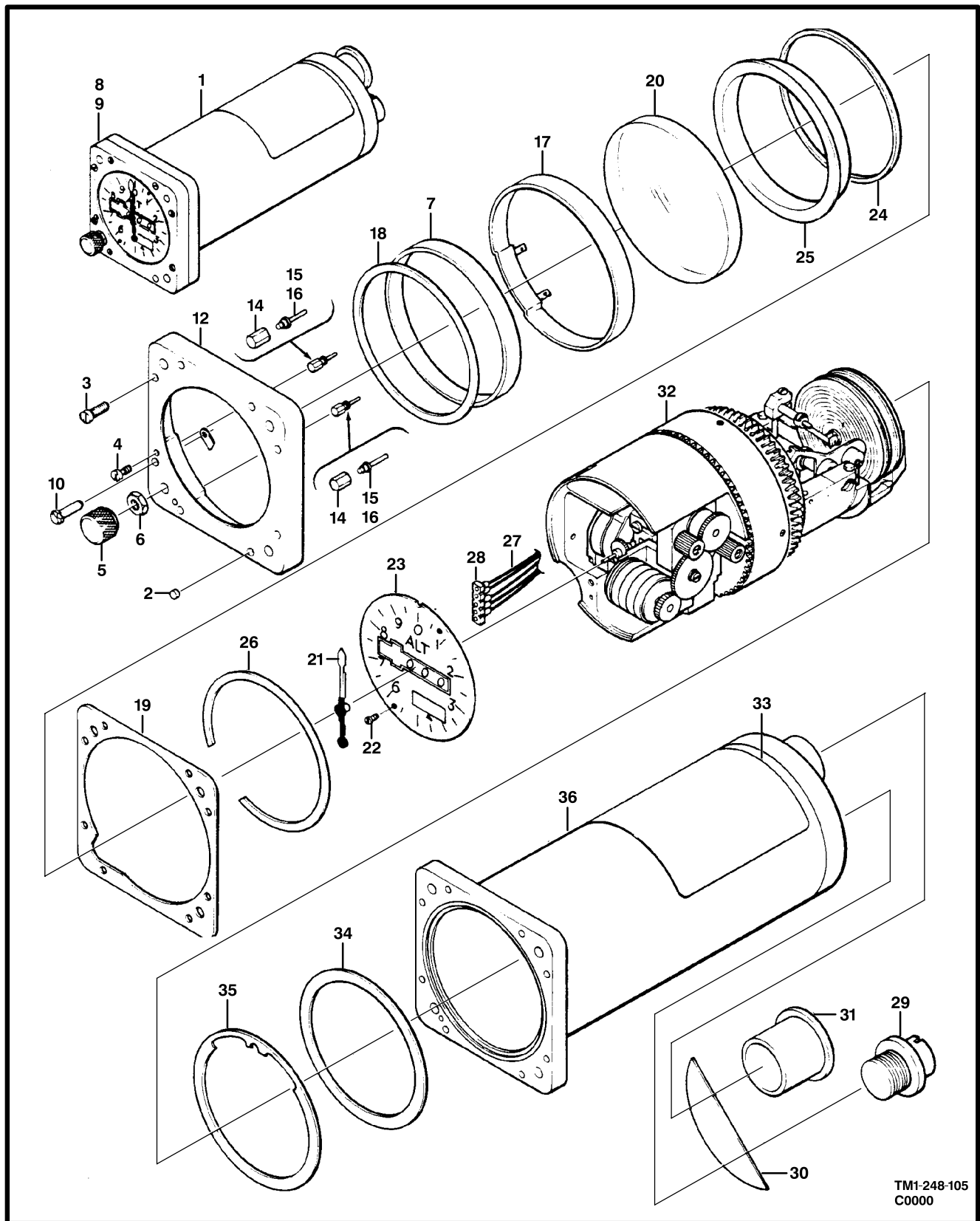
Figure 100. Indicator, Altimeter
