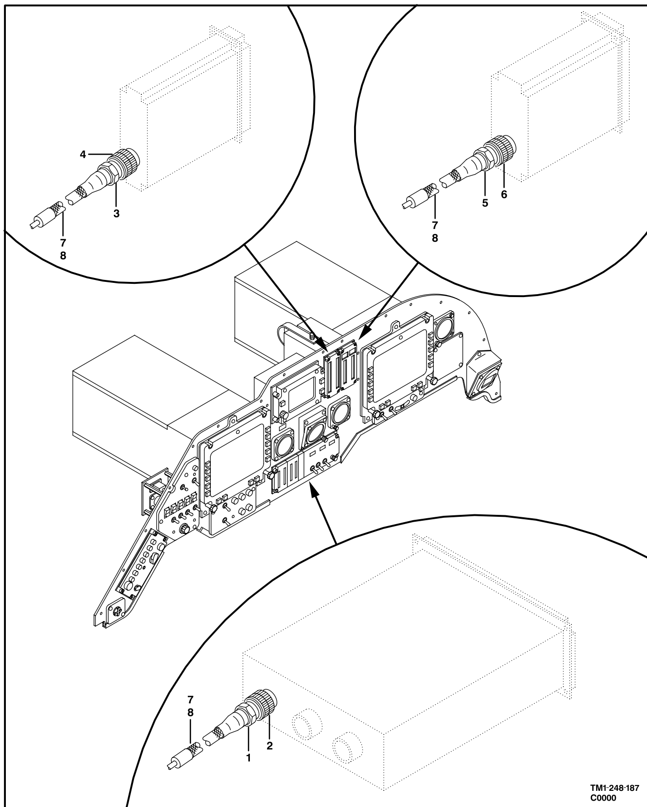
Figure 182. Cable Assembly,Power Plant and Transmission
