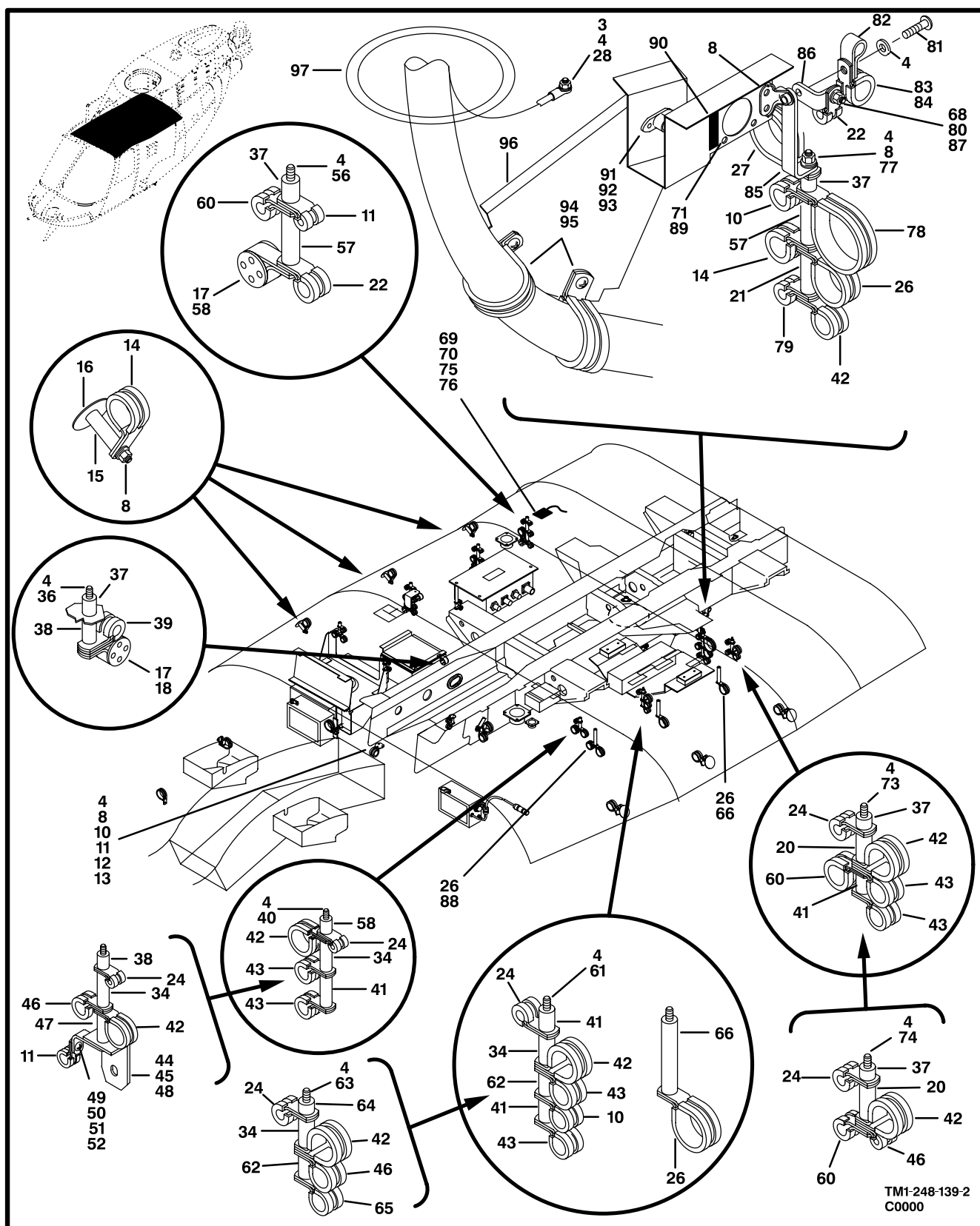
Figure 134. Electrical Installation,Bulkhead (Sheet 2 of 2)
