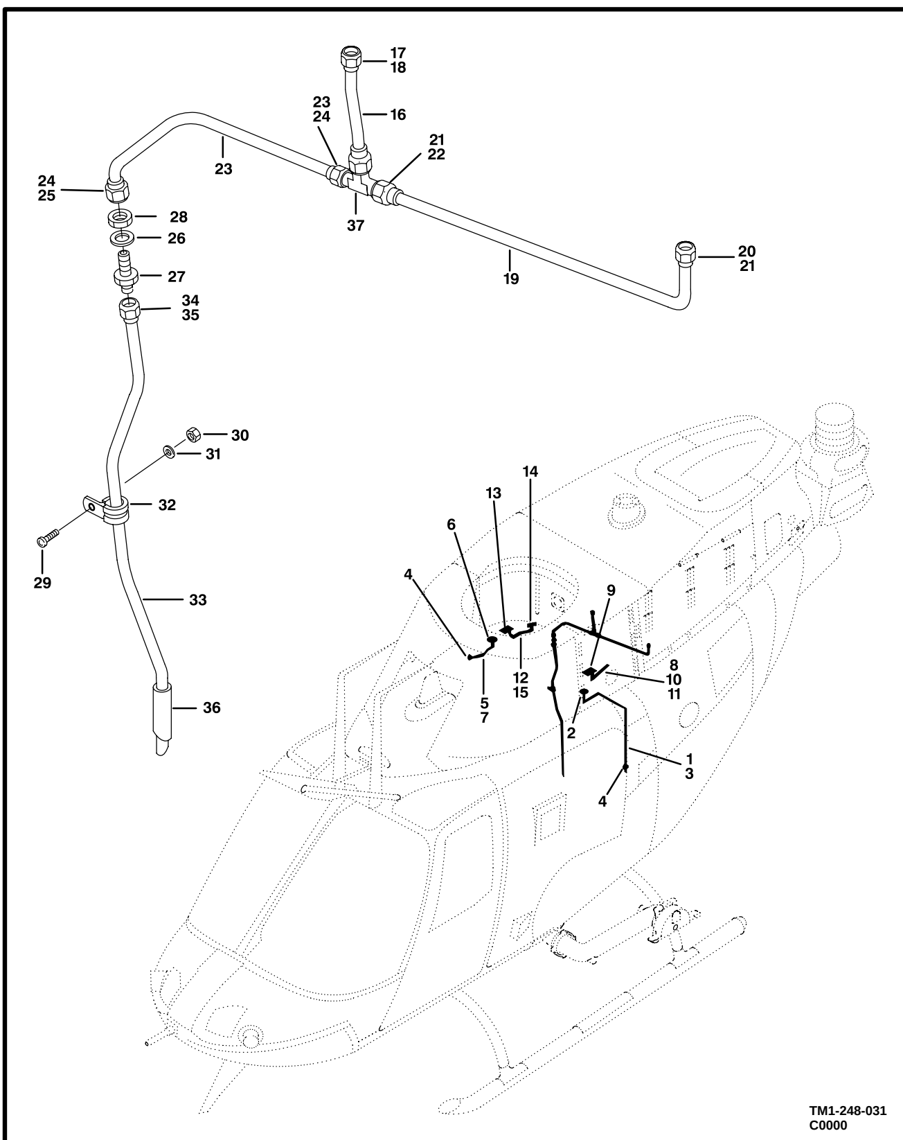
Figure 30. Drain Installation
