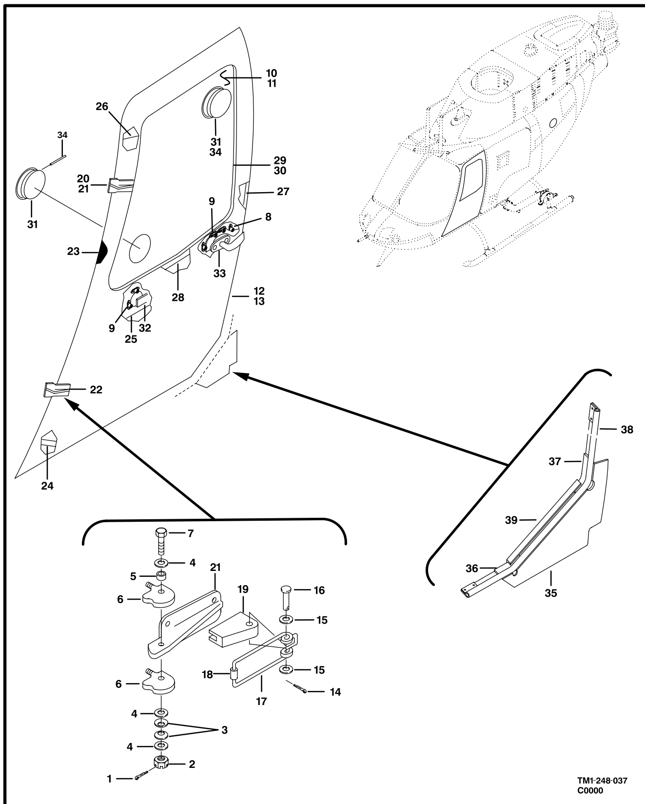
Figure 36. Door Installation,Crew
