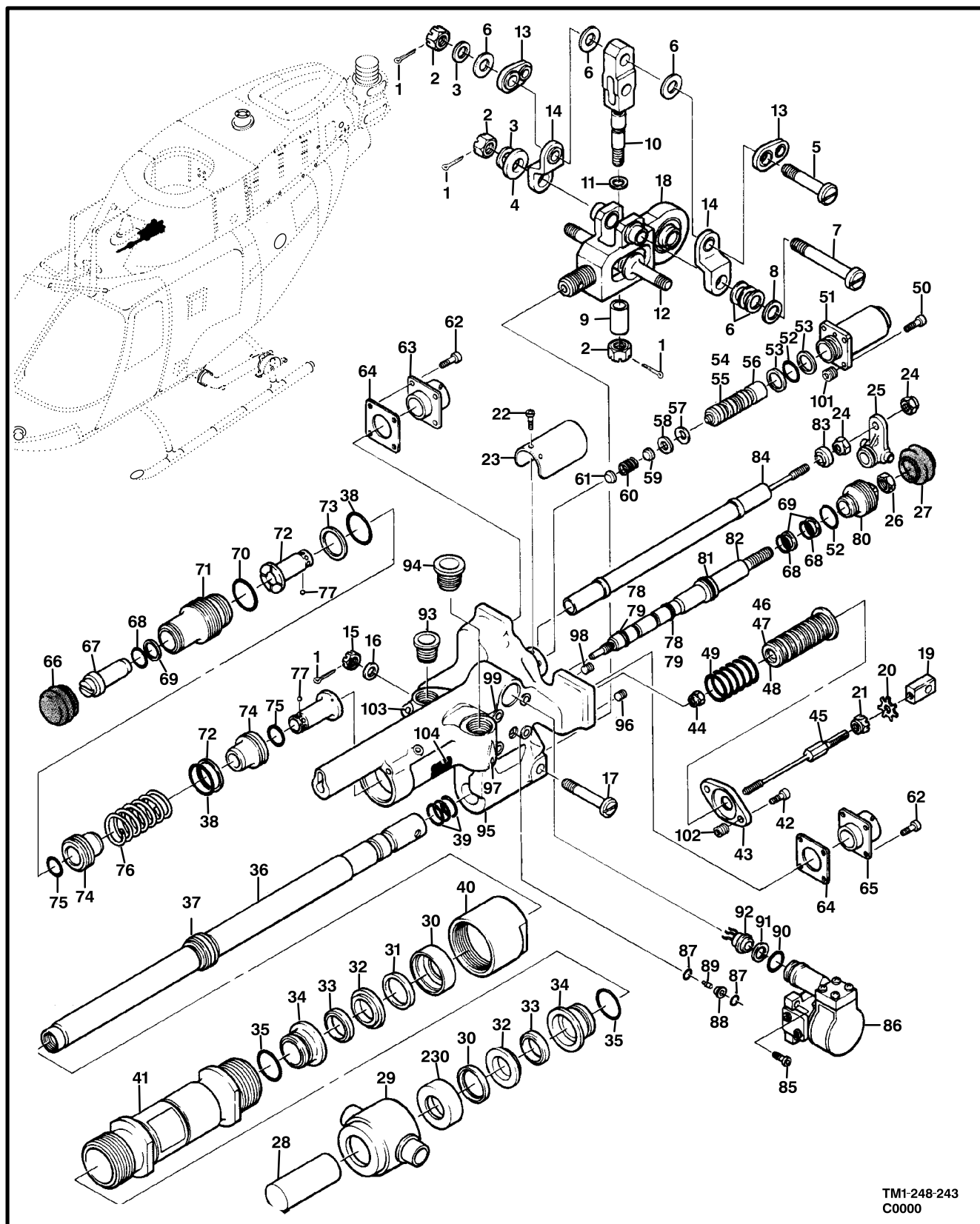
Figure 260. Actuator Assembly
