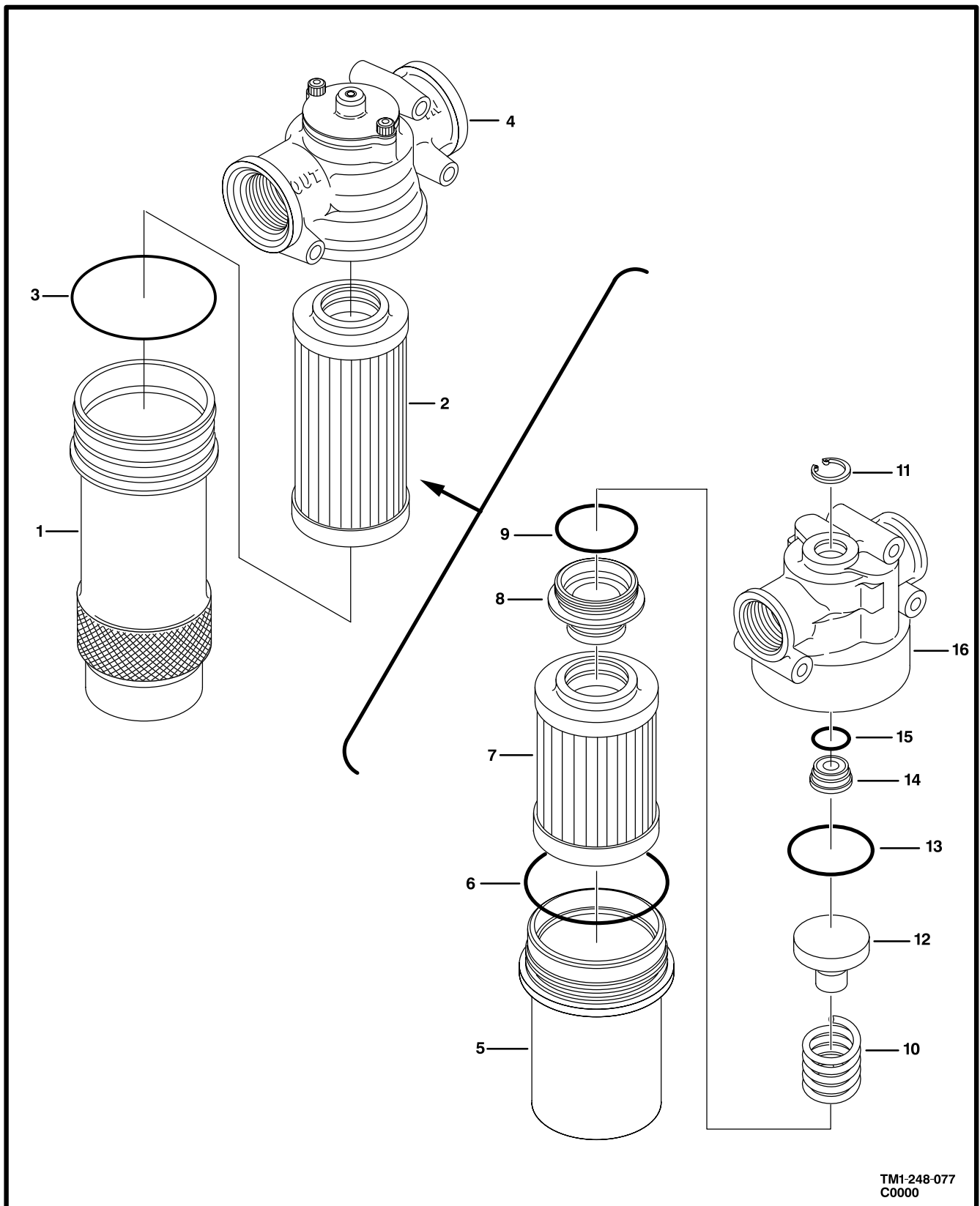
Figure 76. Filter Assembly
