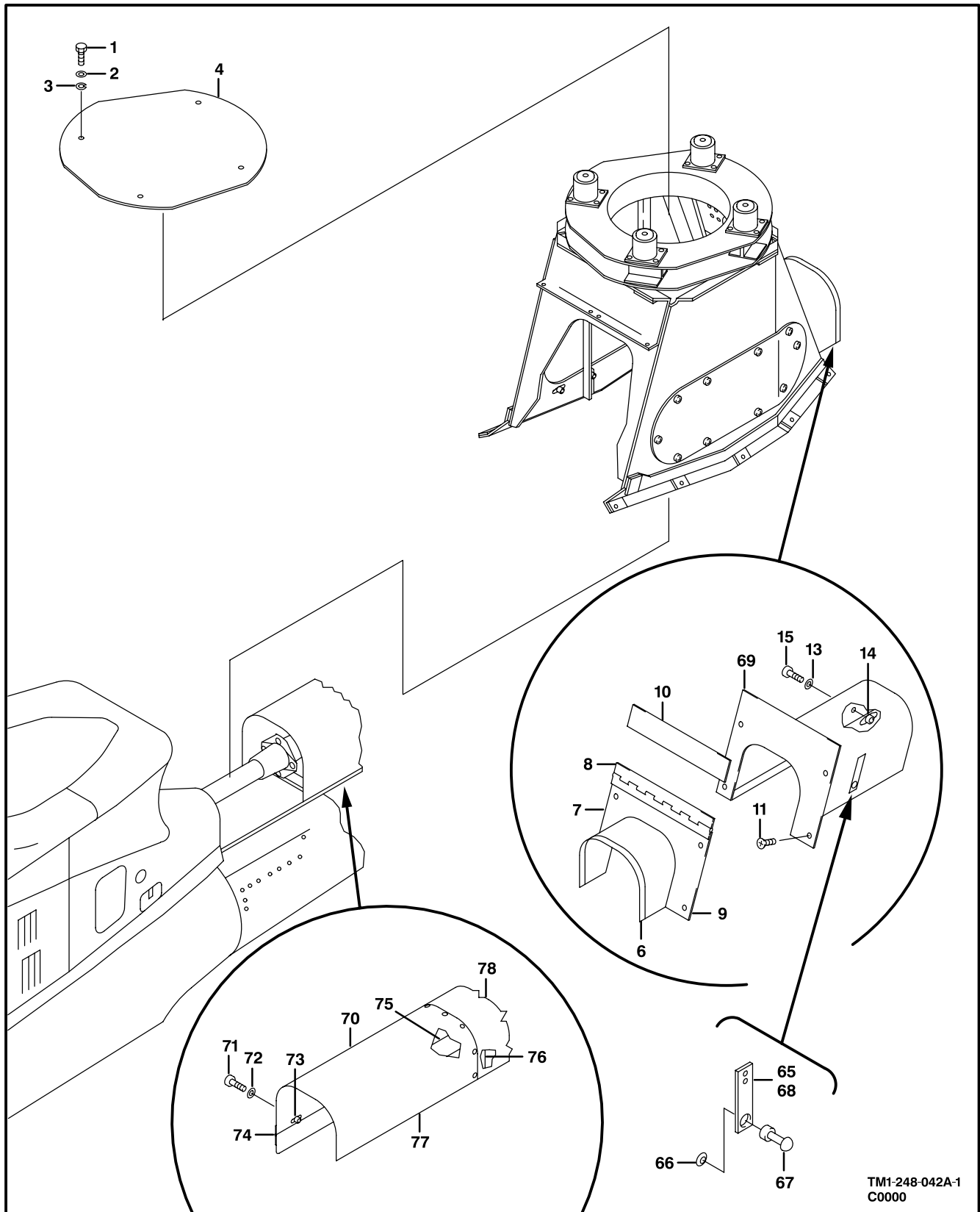
Figure 42. Countermeasures Set AN/ALQ-144 IR Jammer Mount Installation (Sheet 1 of 2)
