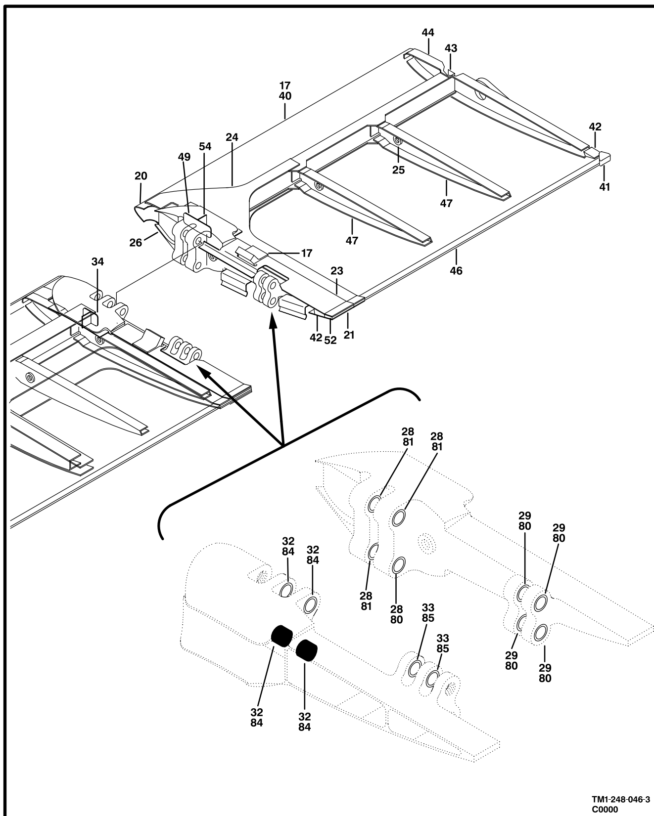
Figure 46. Stabilizer Installation, Horizontal (Sheet 3 of 3)
