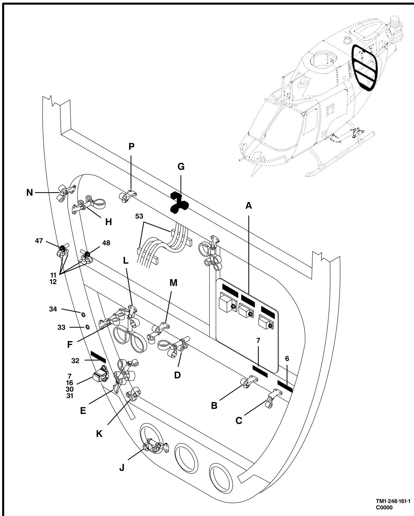
Figure 156. Electrical Installation (USBL EFF 95-0080 AND SUB) (Sheet 1 of 2)
