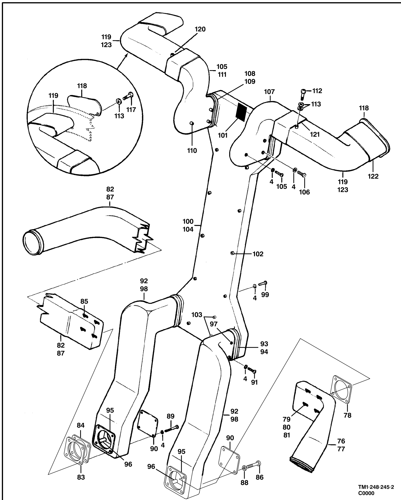
Figure 261. Environmental Control System (Sheet 2 of 3)
