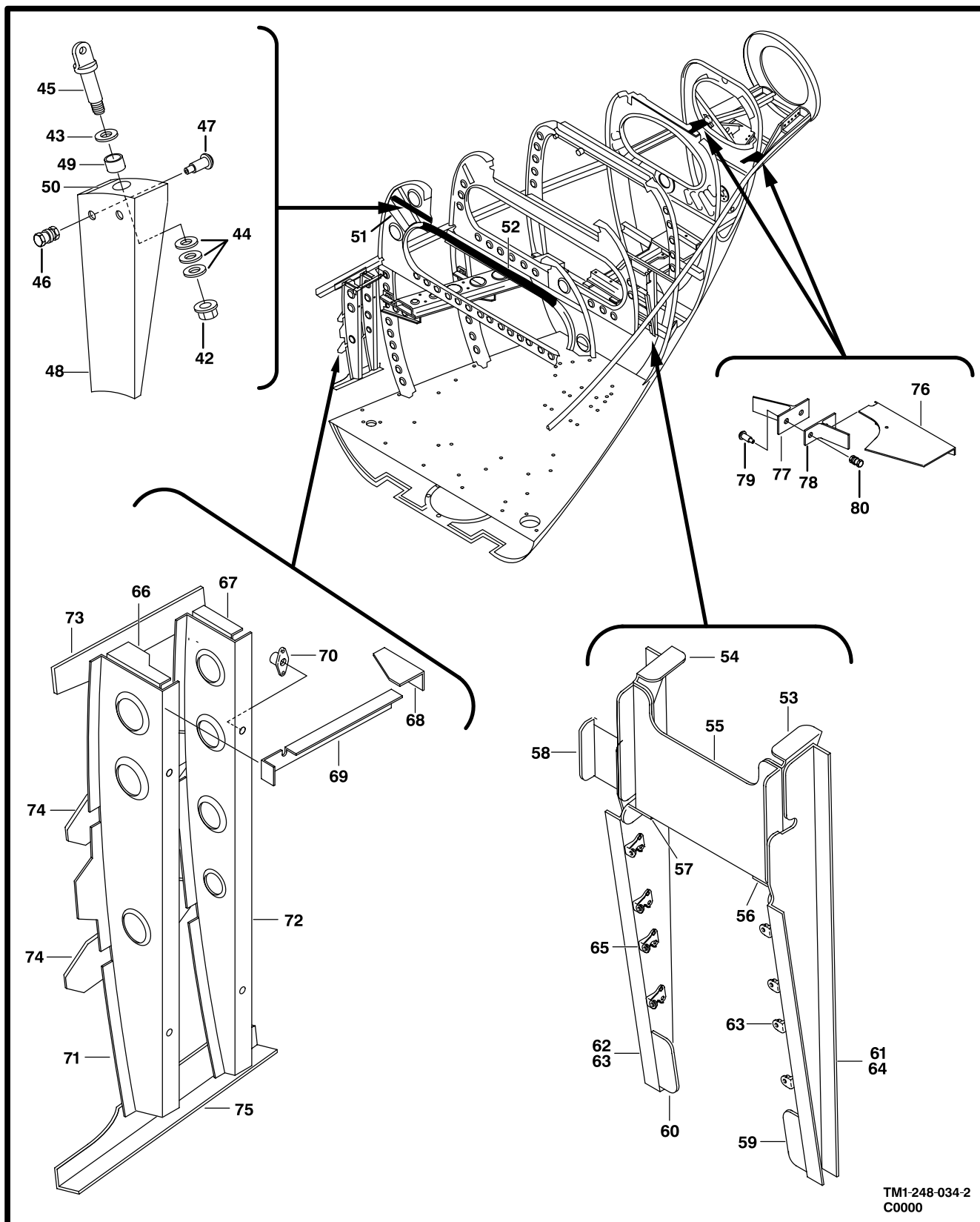
Figure 33. MOD-Support Installation (Sheet 2 of 2)
