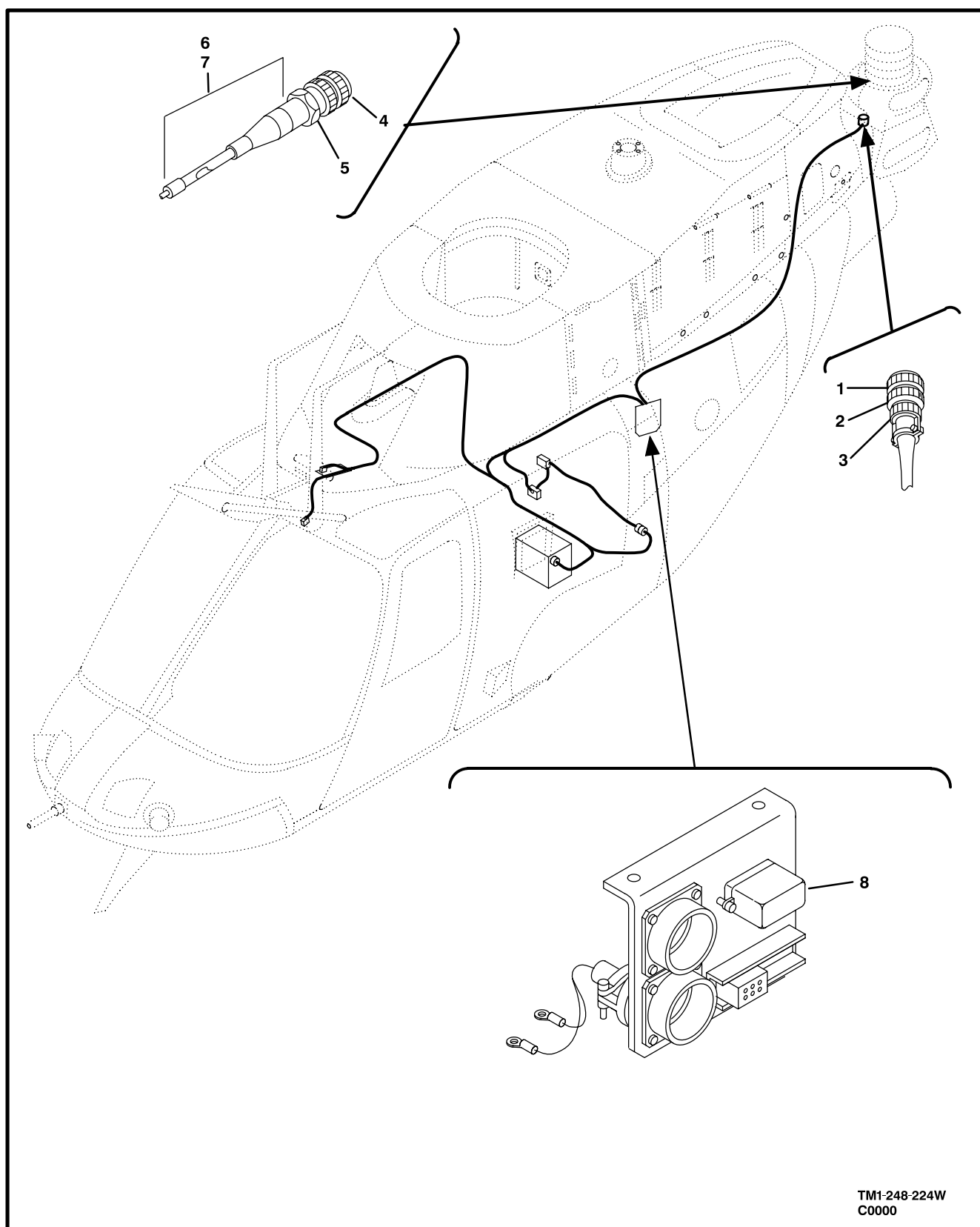
Figure 240. Cable Assembly,IR Jammer
