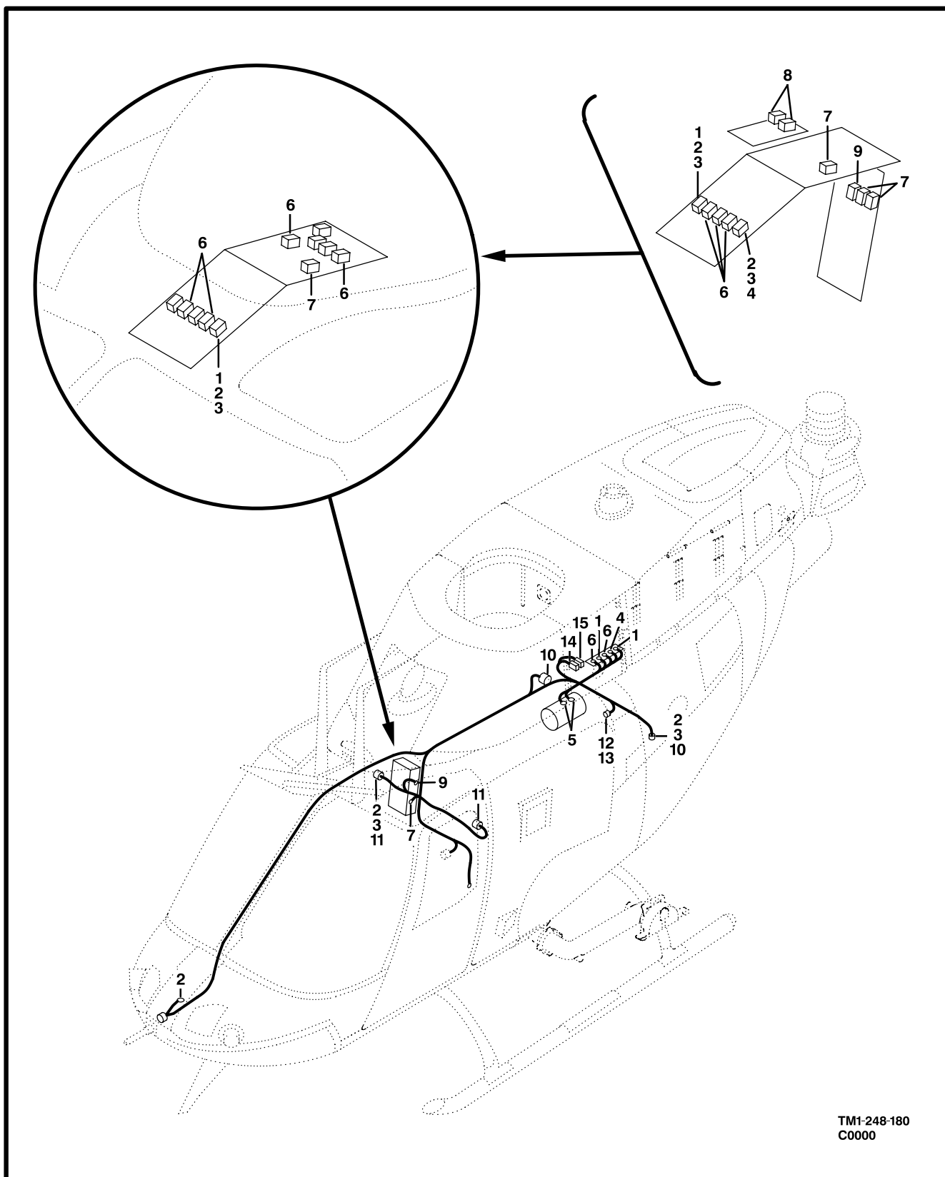
Figure 175. Cable Assembly,Environmental
