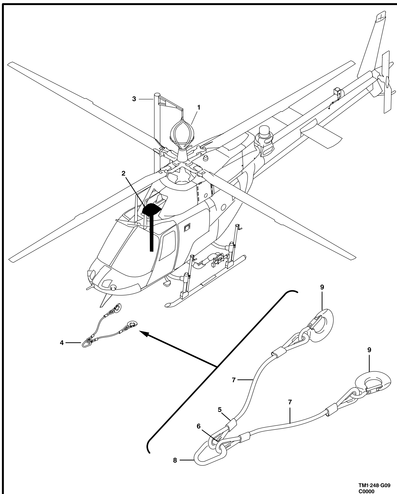
Figure G4. Kit,Rapid Deployment
