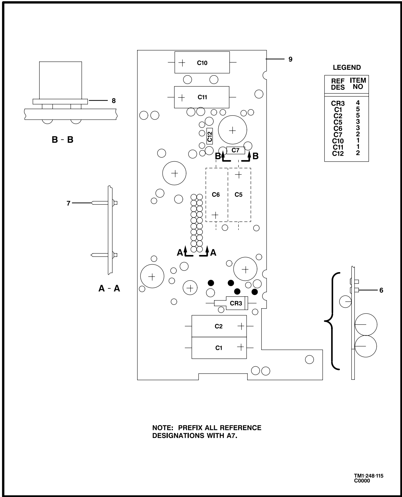
Figure 110. Interconnecting Board
