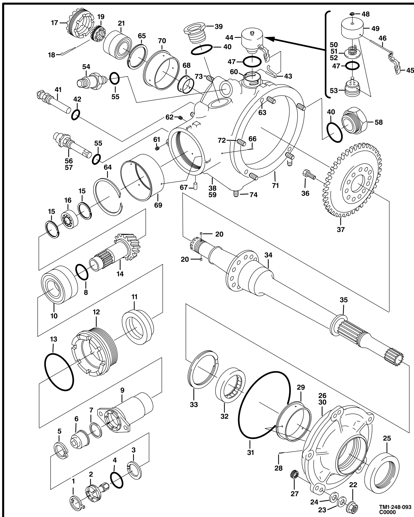
Figure 90. Gearbox Assembly, Tail Rotor
