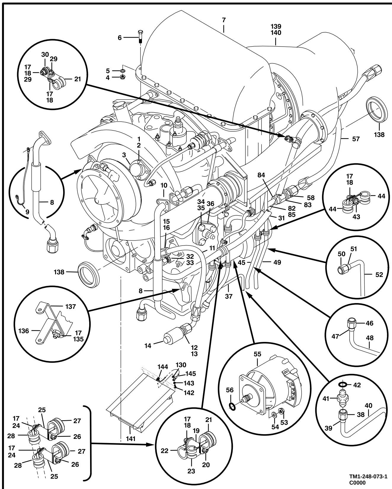
Figure 71. Engine Assembly (Sheet 1 of 2)
