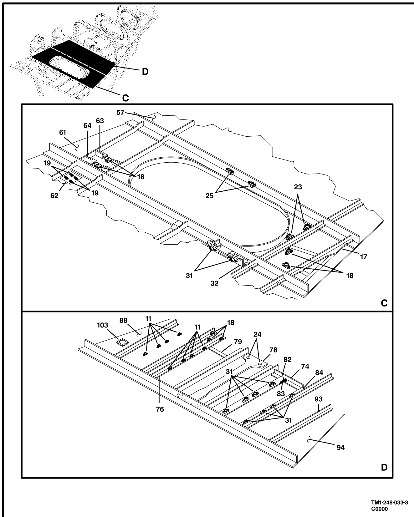
Figure 32. Web Installation (Sheet 3 of 3)
