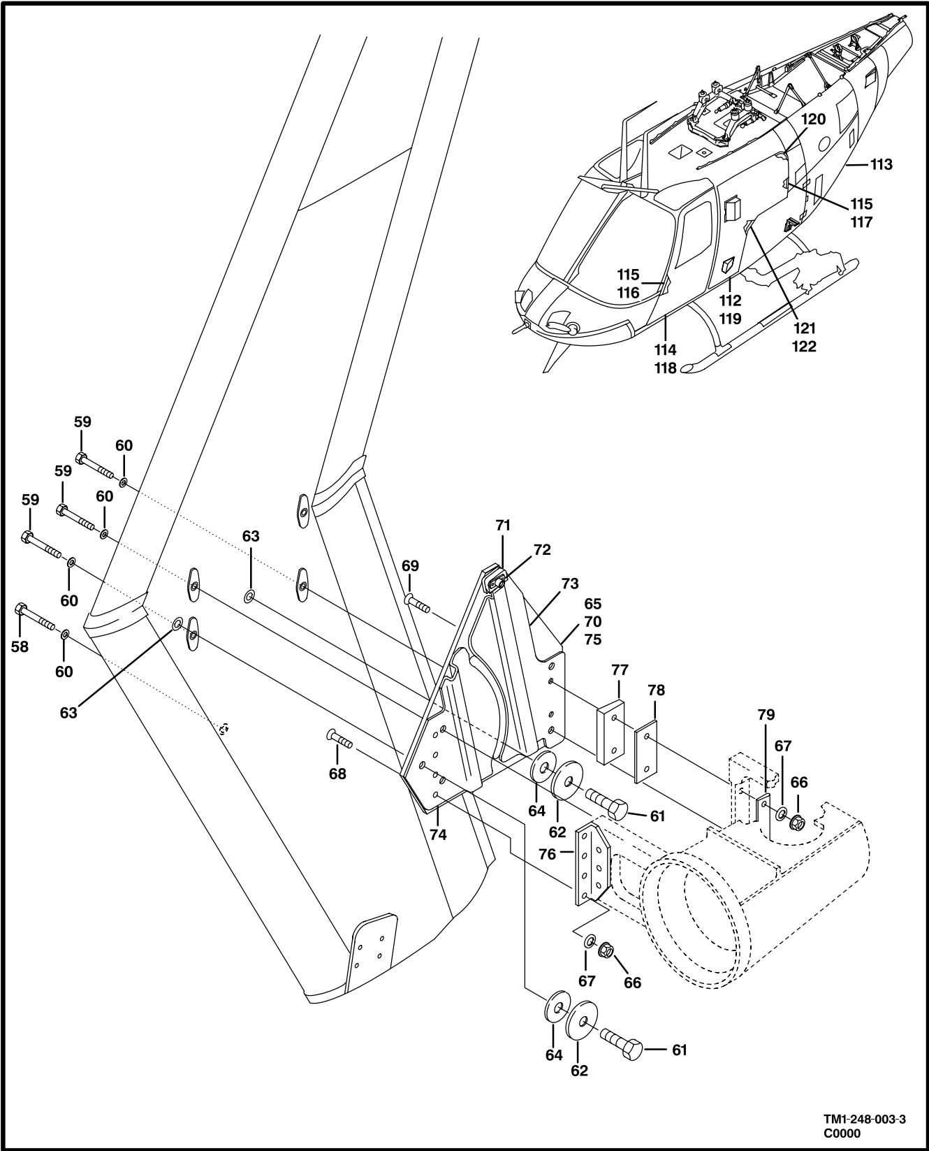
Figure 3. Fuselage Assembly (Sheet 3 of 4)
