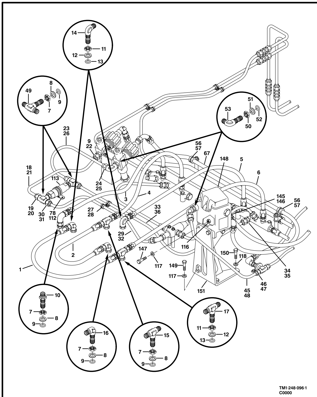
Figure 93. Hydraulic System Installation, Flight Controls (Sheet 1 of 3)
