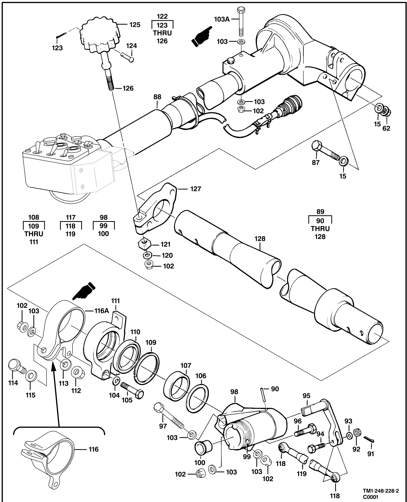
Figure 246. Controls Installation, Collective Pitch (Sheet 2 of 2)
