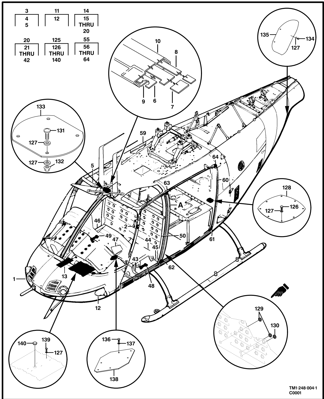
Figure 4. Structure Assembly, Fuselage (Sheet 1 of 4)
