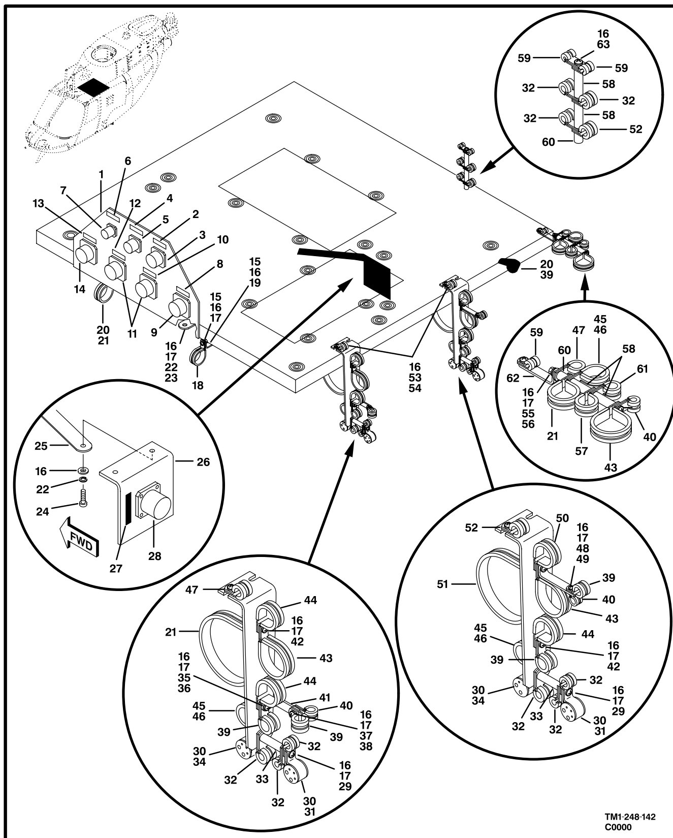
Figure 137. Electrical Installation, Shelf
