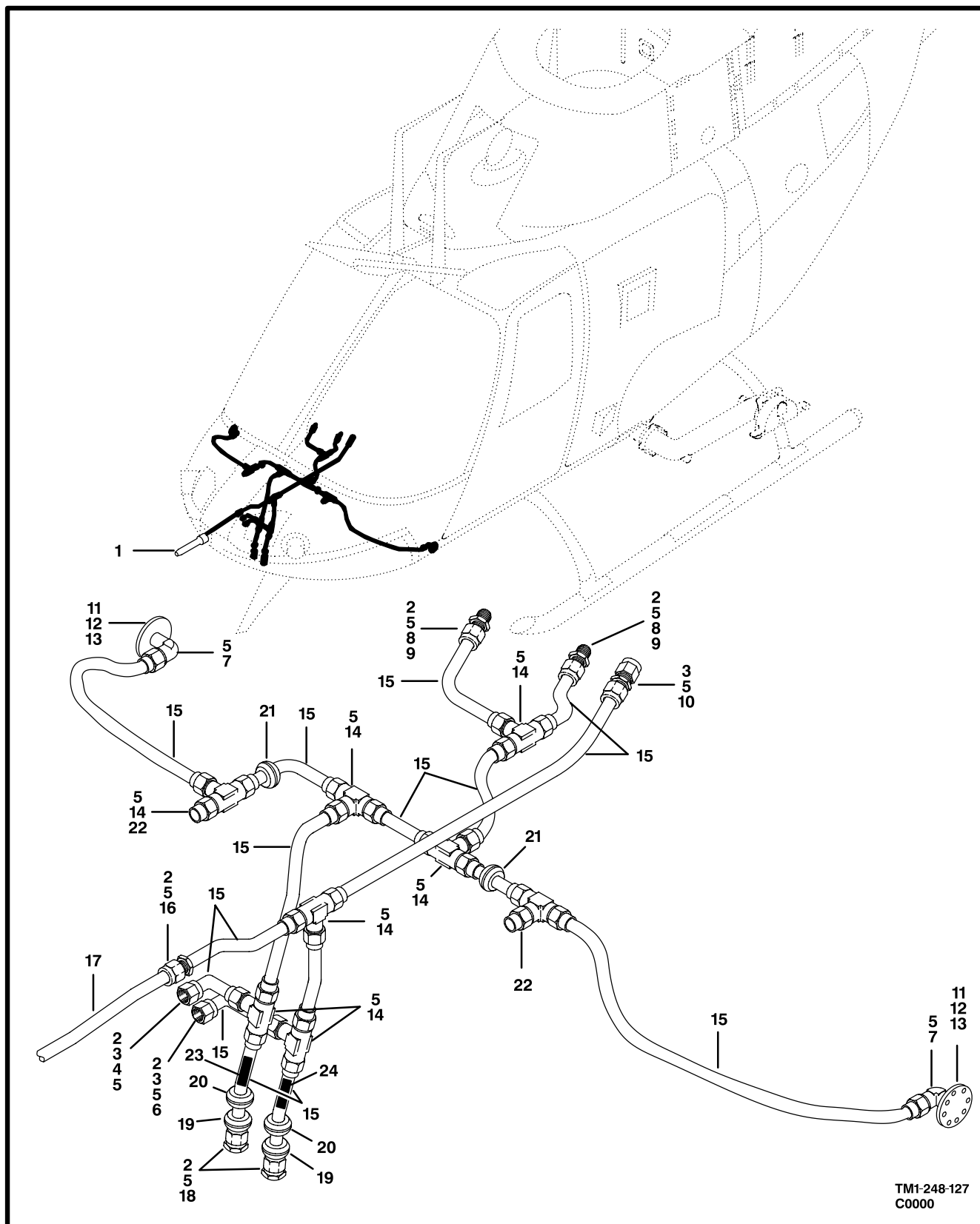
Figure 122. Pitot Static System
