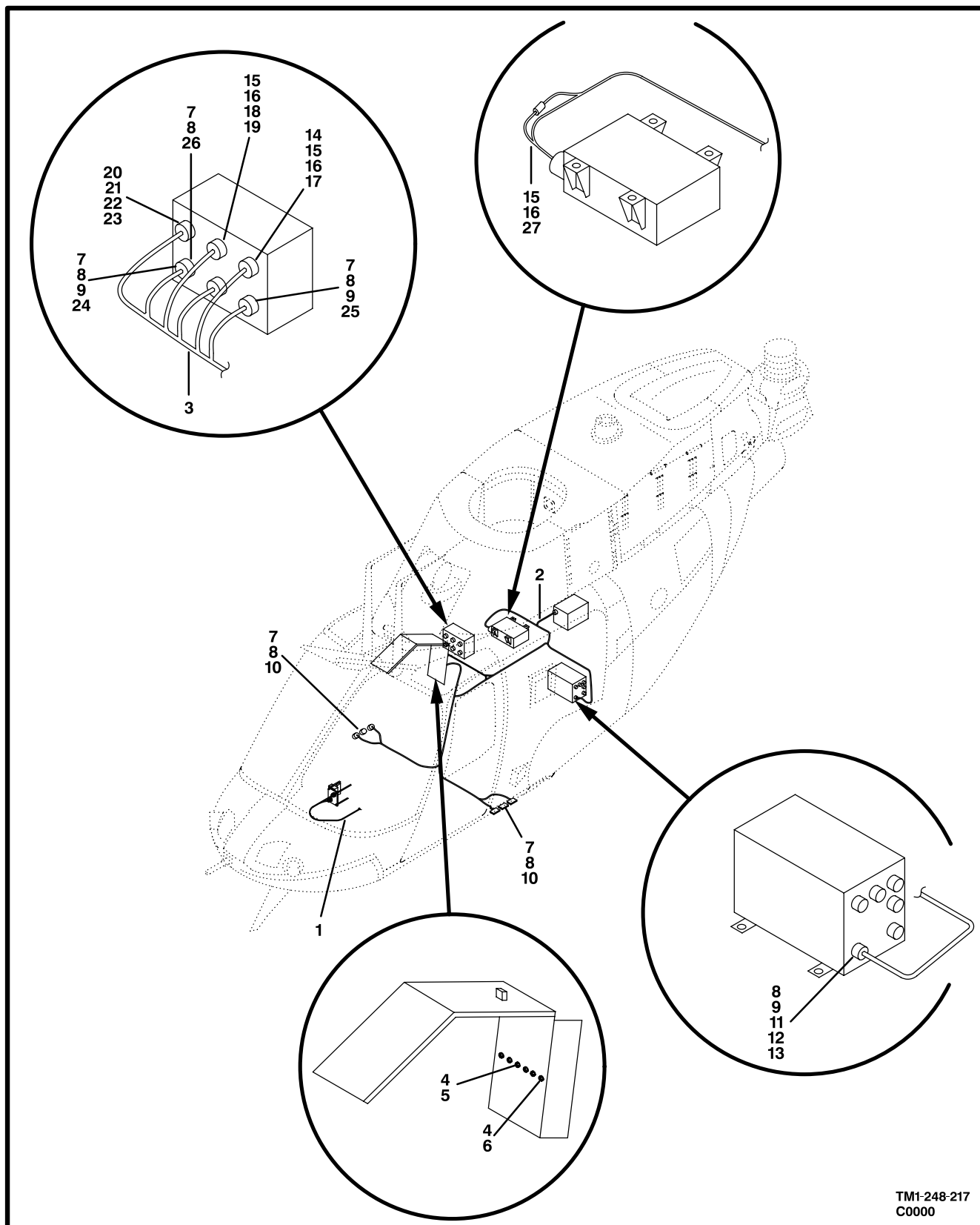
Figure 212. Harness Assembly, Armament
