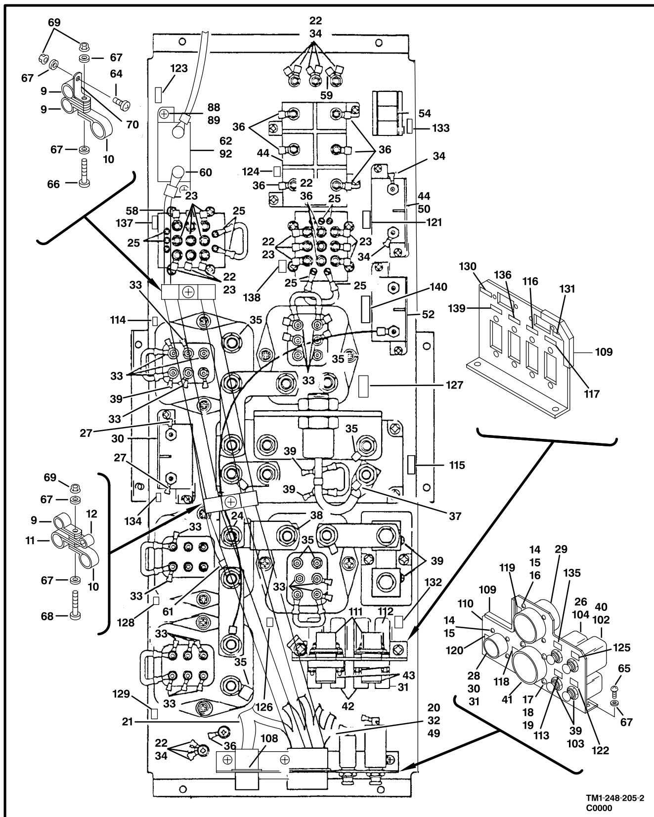
Figure 200. Electrical Assembly, DC Equipment (Sheet 2 of 2)
