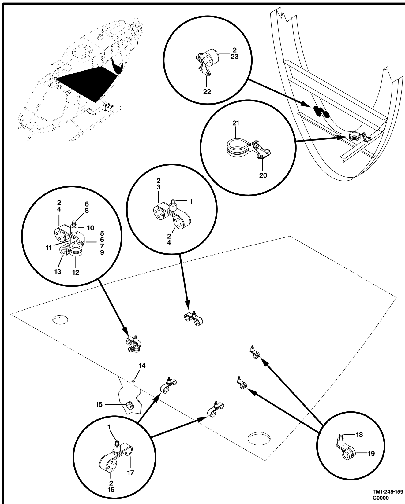
Figure 154. Electrical Installation, Canted Web
