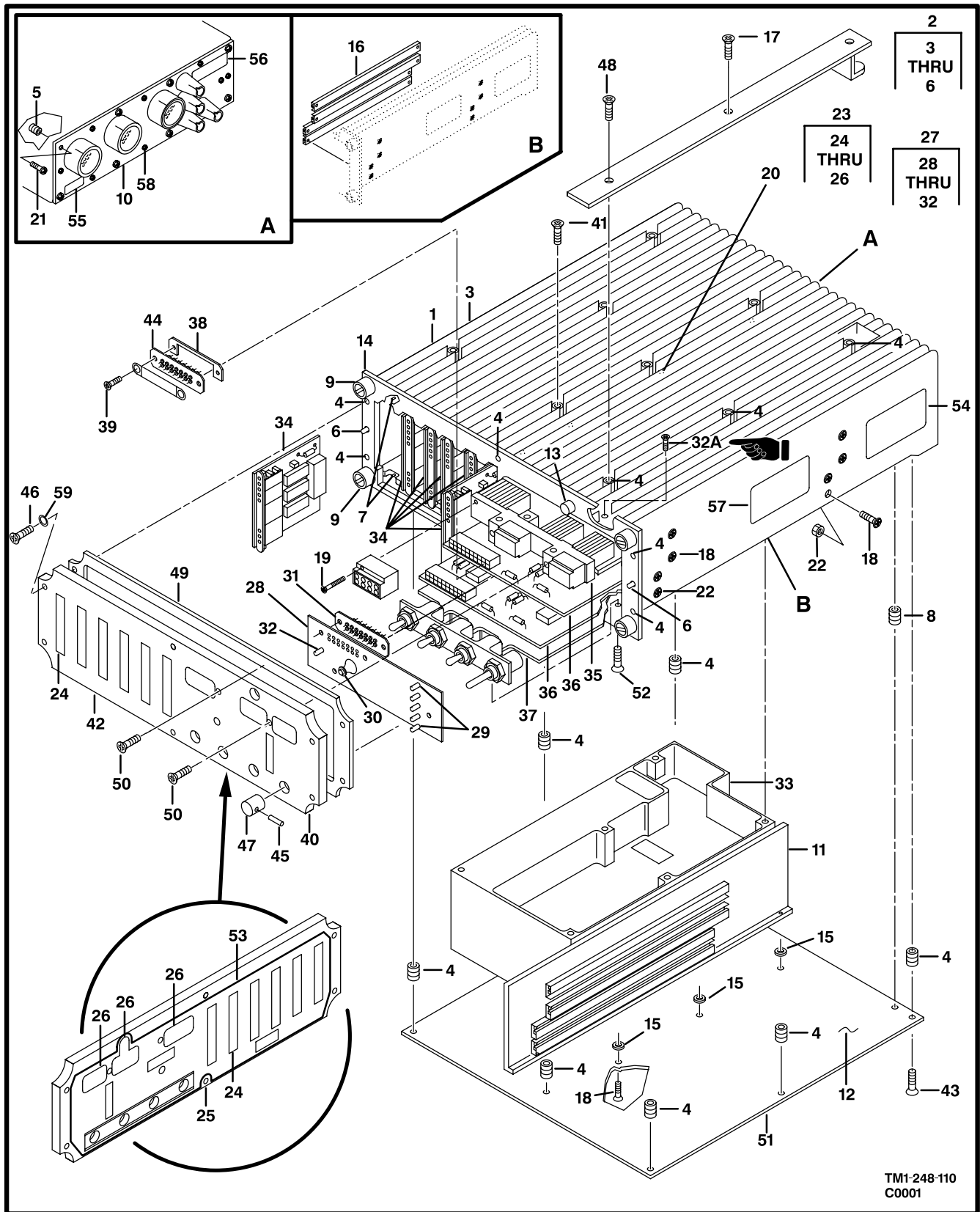
Figure 105. Indicator, Multi-Parameter
