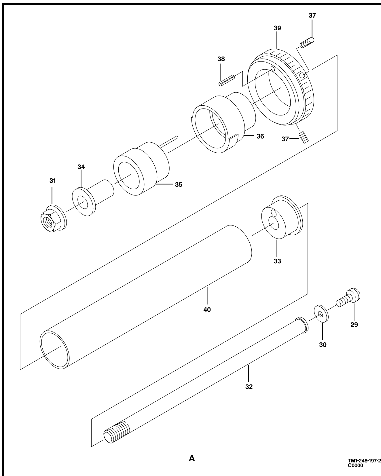
Figure 192. Rotation Assembly (Sheet 2 of 2)
