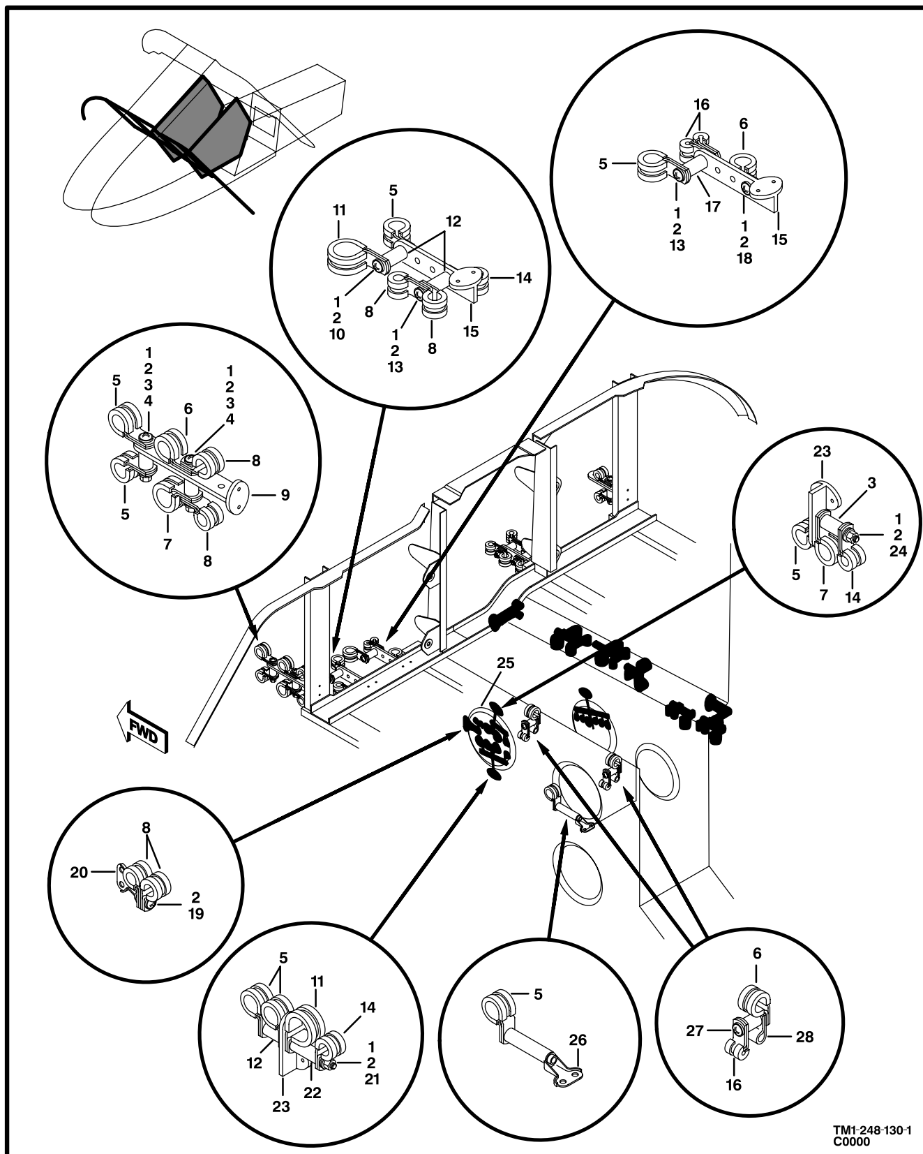
Figure 125. Electrical Installation,Nose (Sheet 1 of 2)
