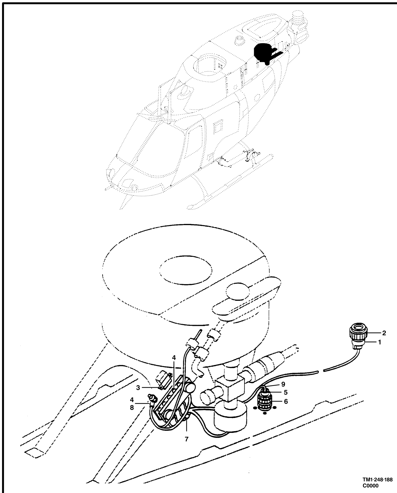
Figure 183. Cable Assembly,Power Plant and Transmission
