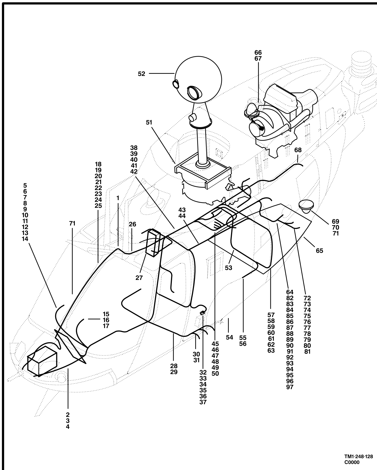
Figure 123. Electrical Installation,Cable Assembly
