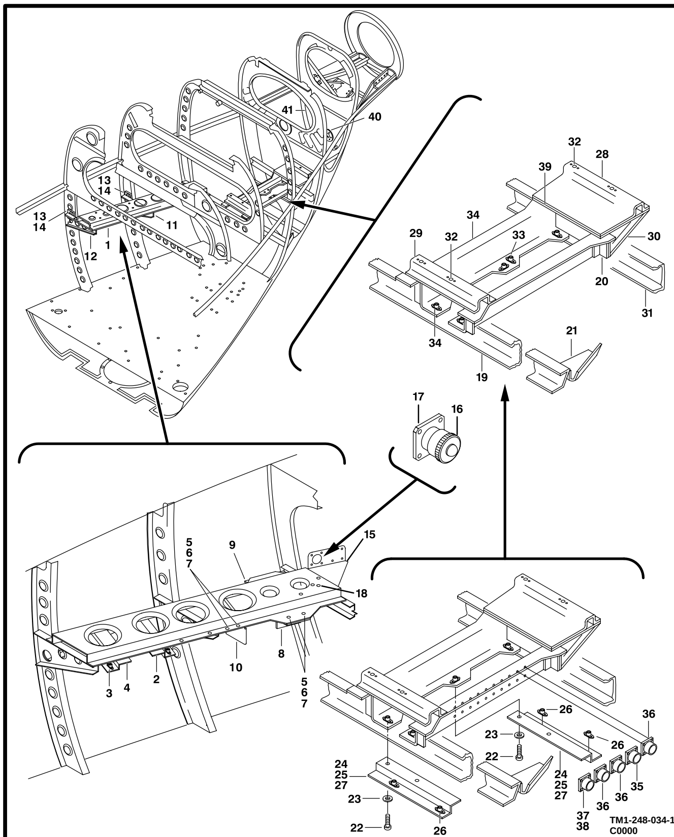
Figure 33. MOD-Support Installation (Sheet 1 of 2)
