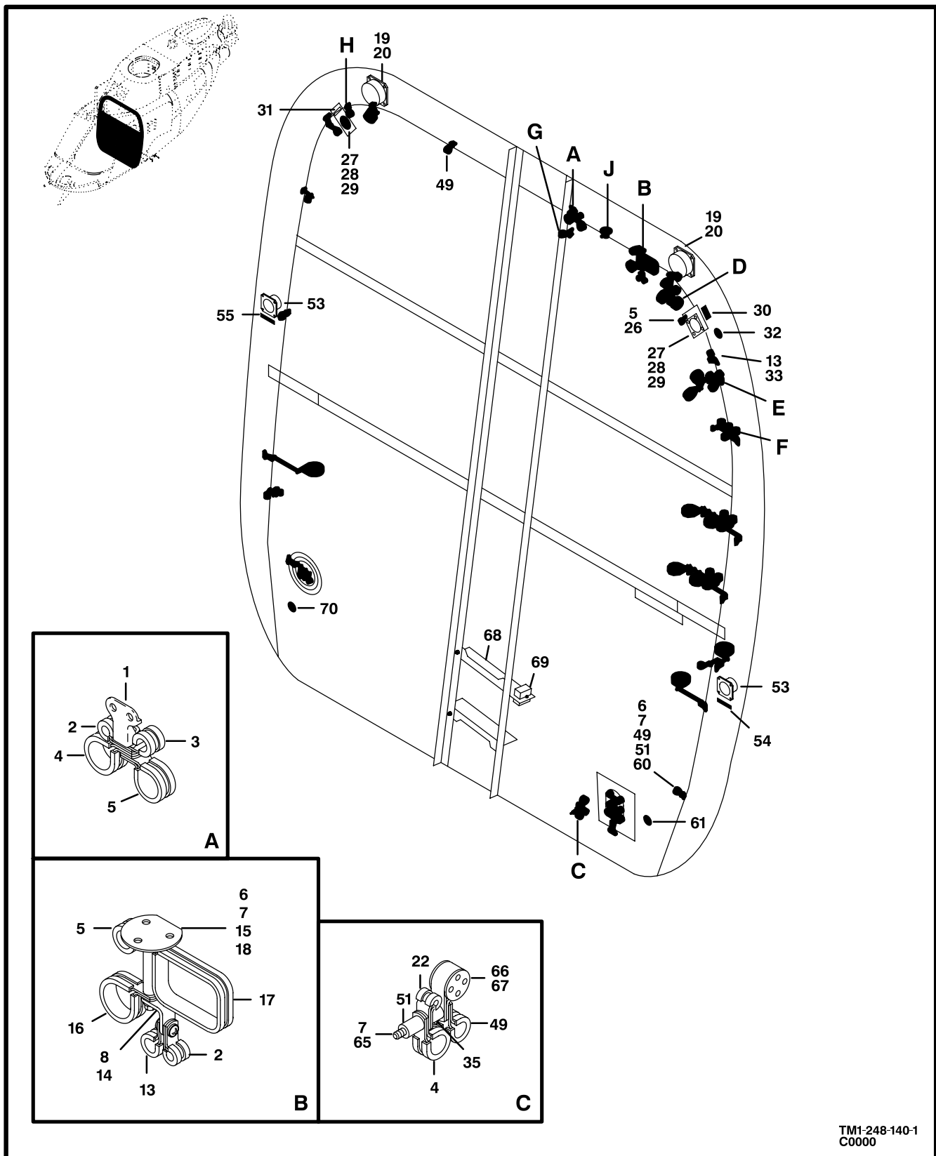
Figure 135. Electrical Installation, Bulkhead (Sheet 1 of 4)
