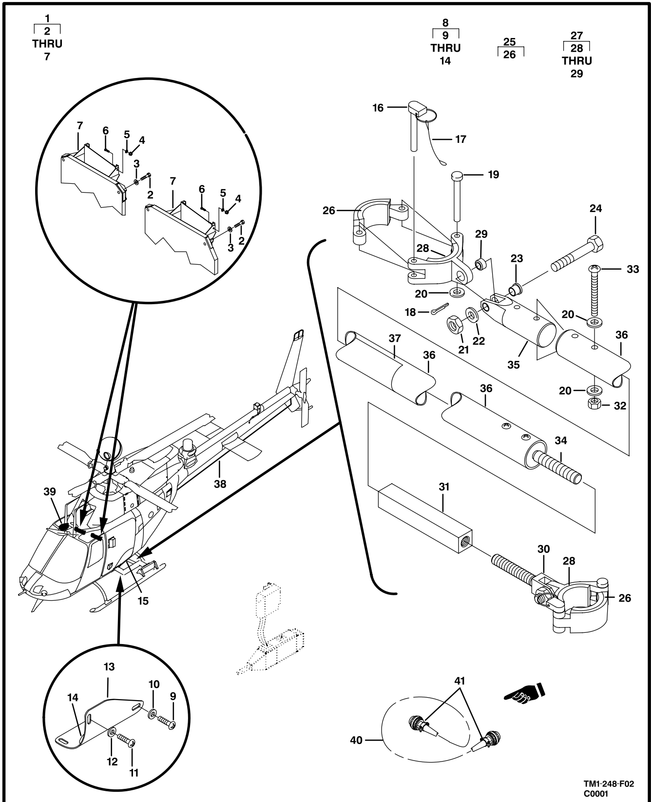
Figure F2. MOD-Loose Equipment
