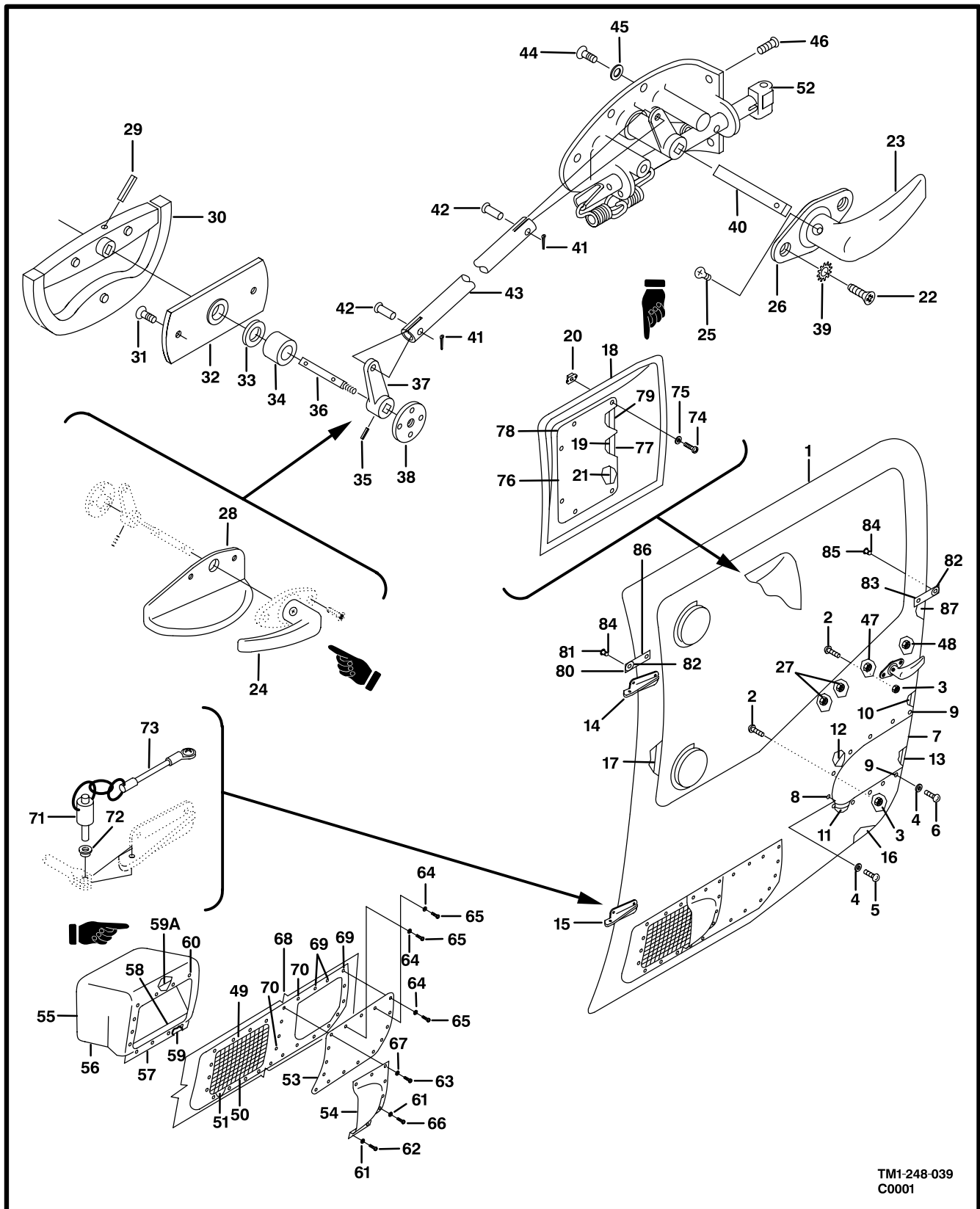
Figure 38. Door Installation, Passenger
