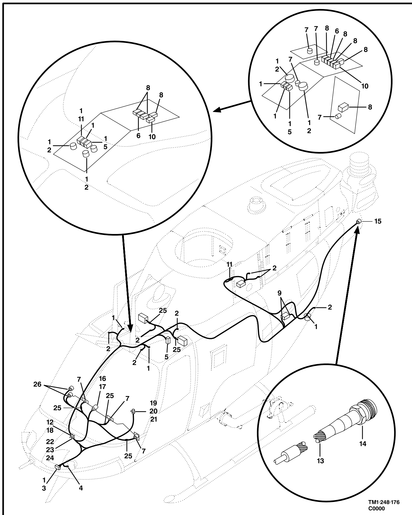
Figure 171. Cable Assembly, Lighting System
