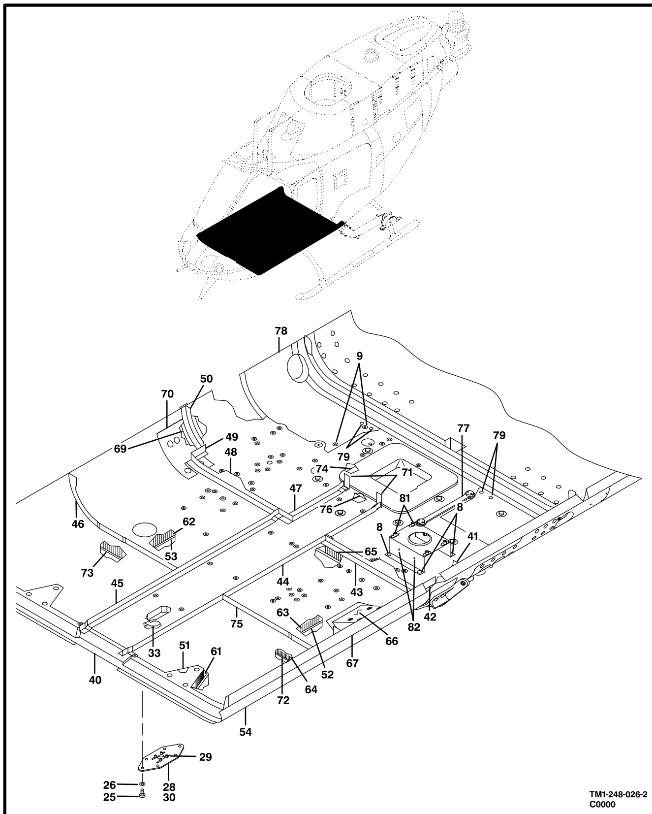
Figure 25. Shell Assembly, FWD (Sheet 2 of 2)
