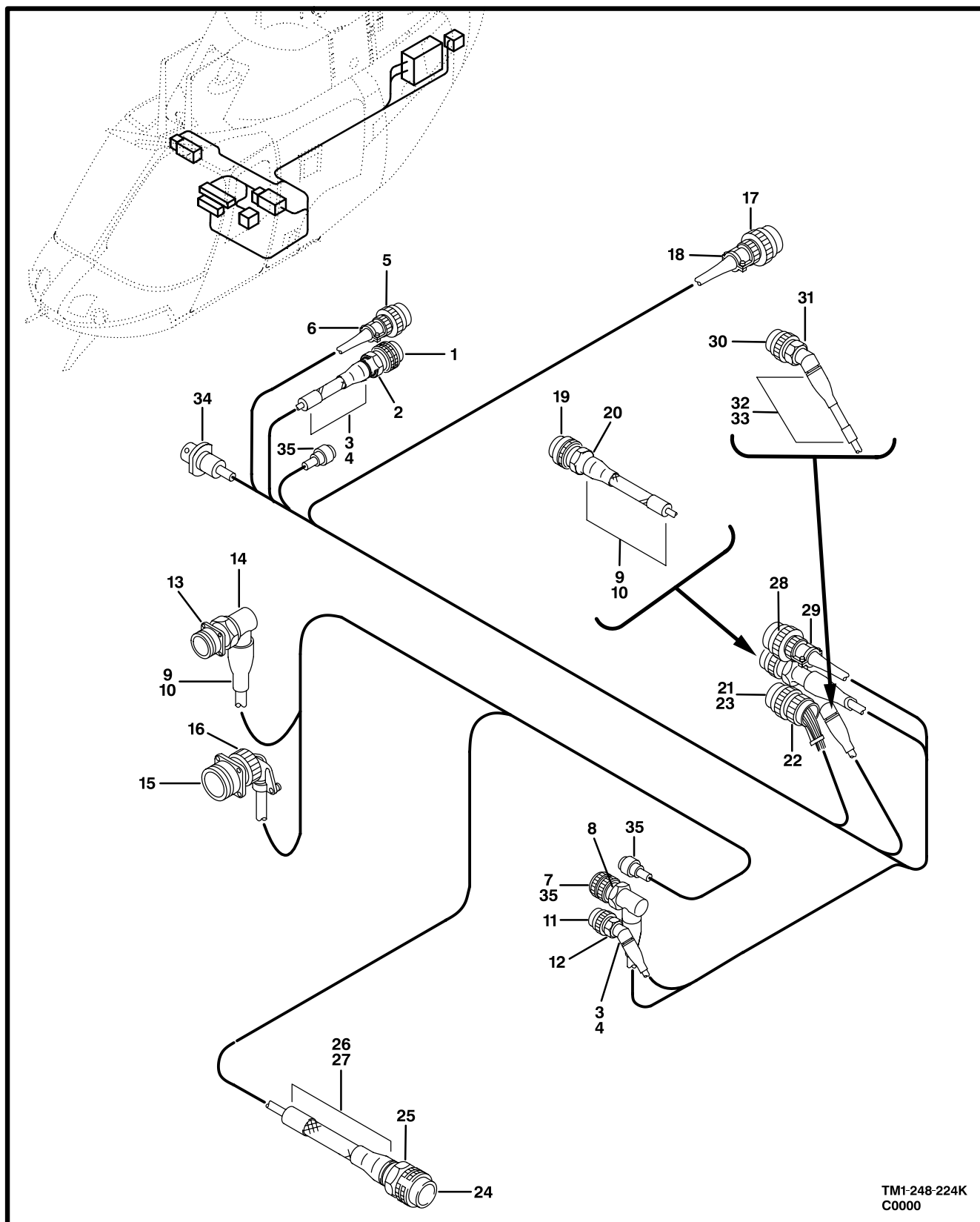
Figure 229. Cable Assembly, HF-Amplifier
