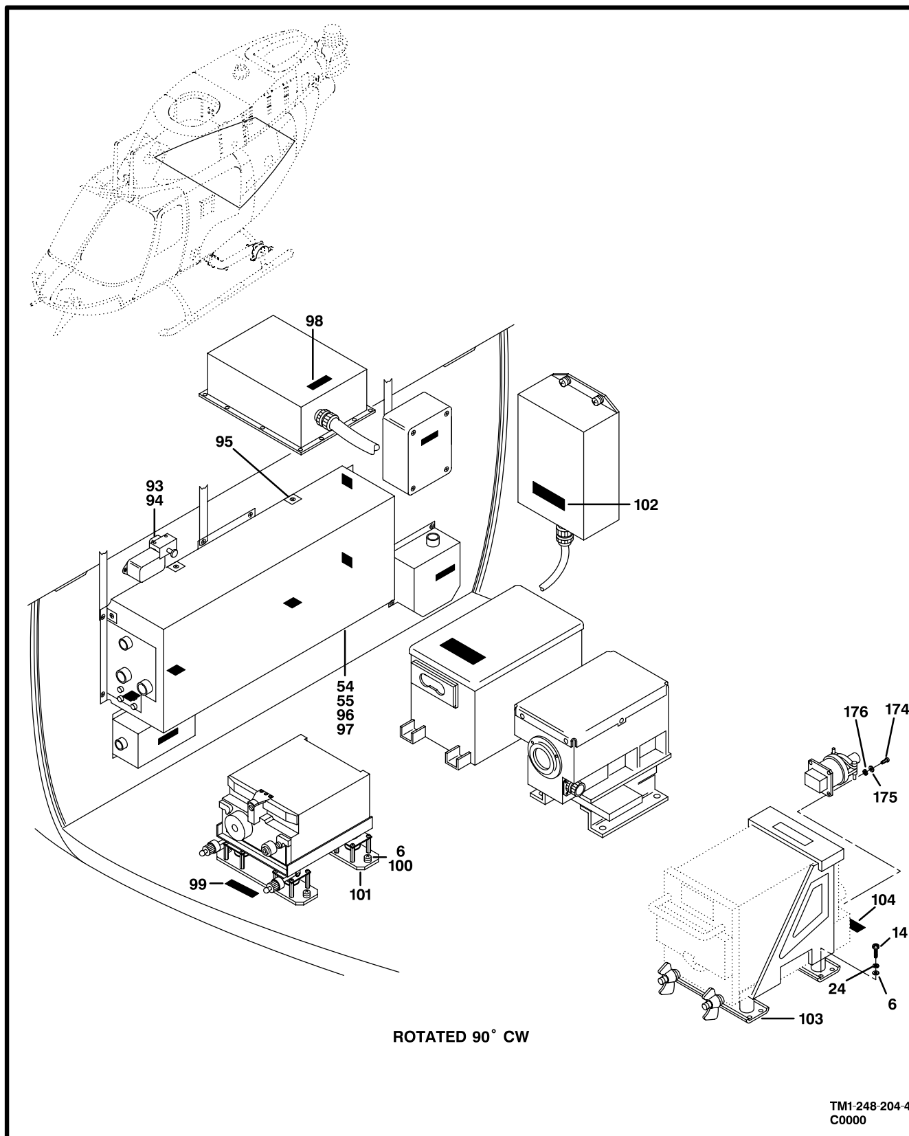
Figure 199. Electrical Assembly, Avionics Installation, AFT Cabin (Sheet 4 of 5)
