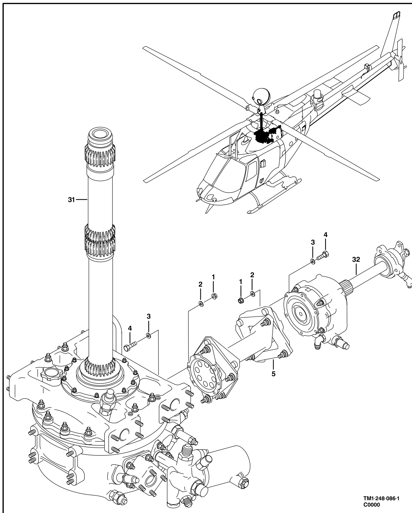
Figure 84. Drive System Installation (Sheet 1 of 2)
