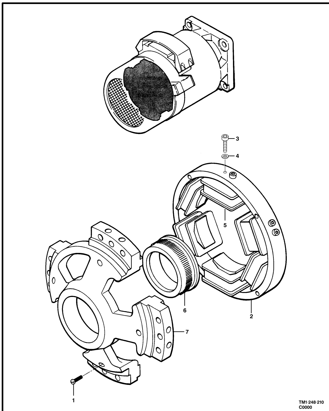
Figure 205. Bearing Support Assembly
