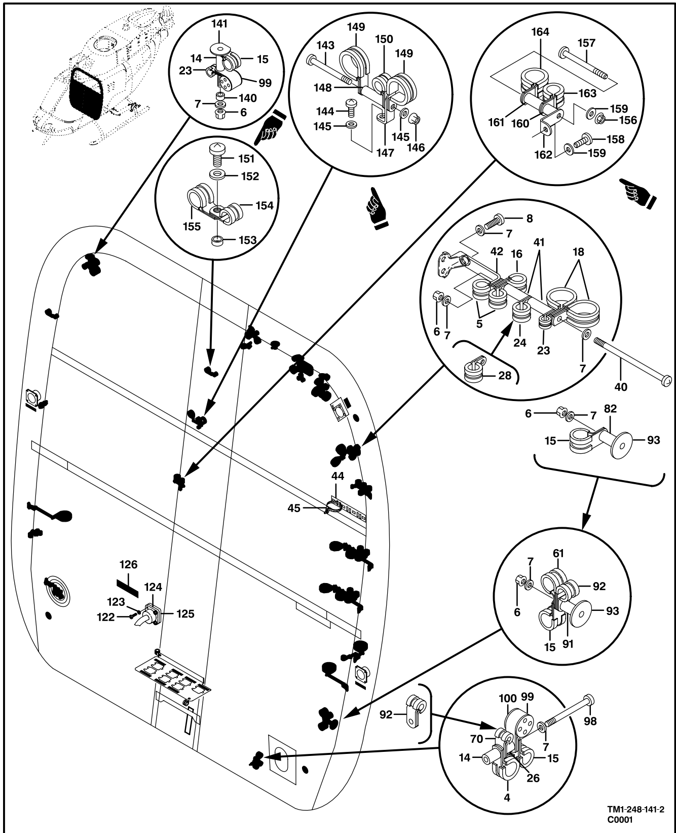
Figure 136. Electrical Installation, Bulkhead (Sheet 2 of 4)
