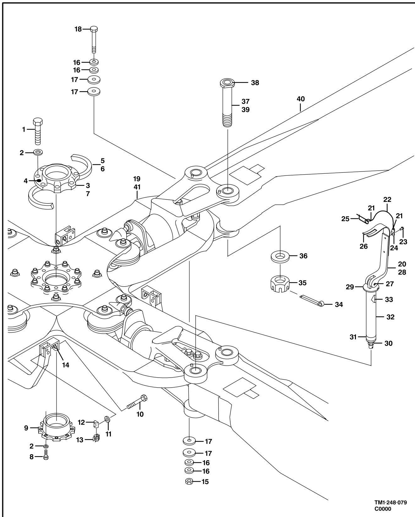
Figure 78. Hub and Blade Installation
