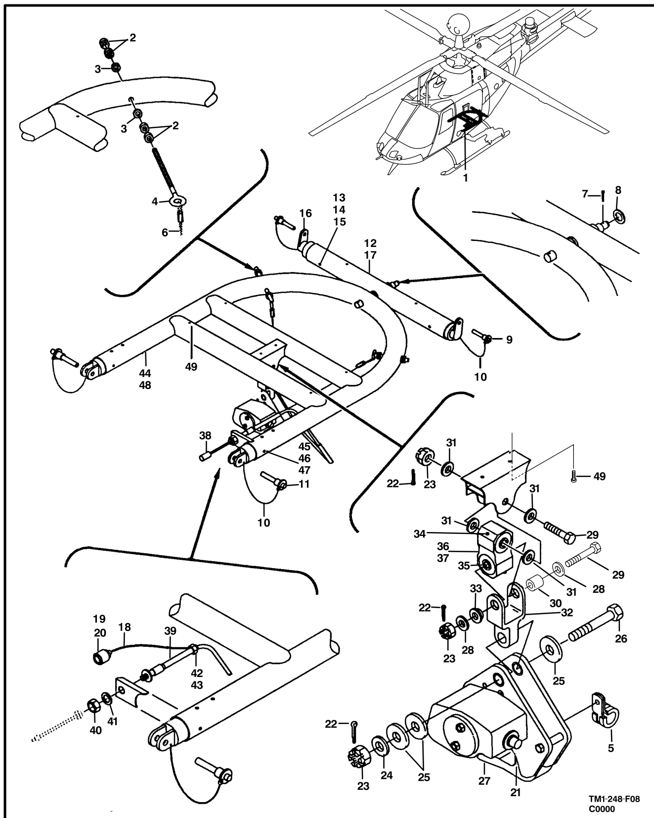
Figure F7. Kit,Cargo Hook
