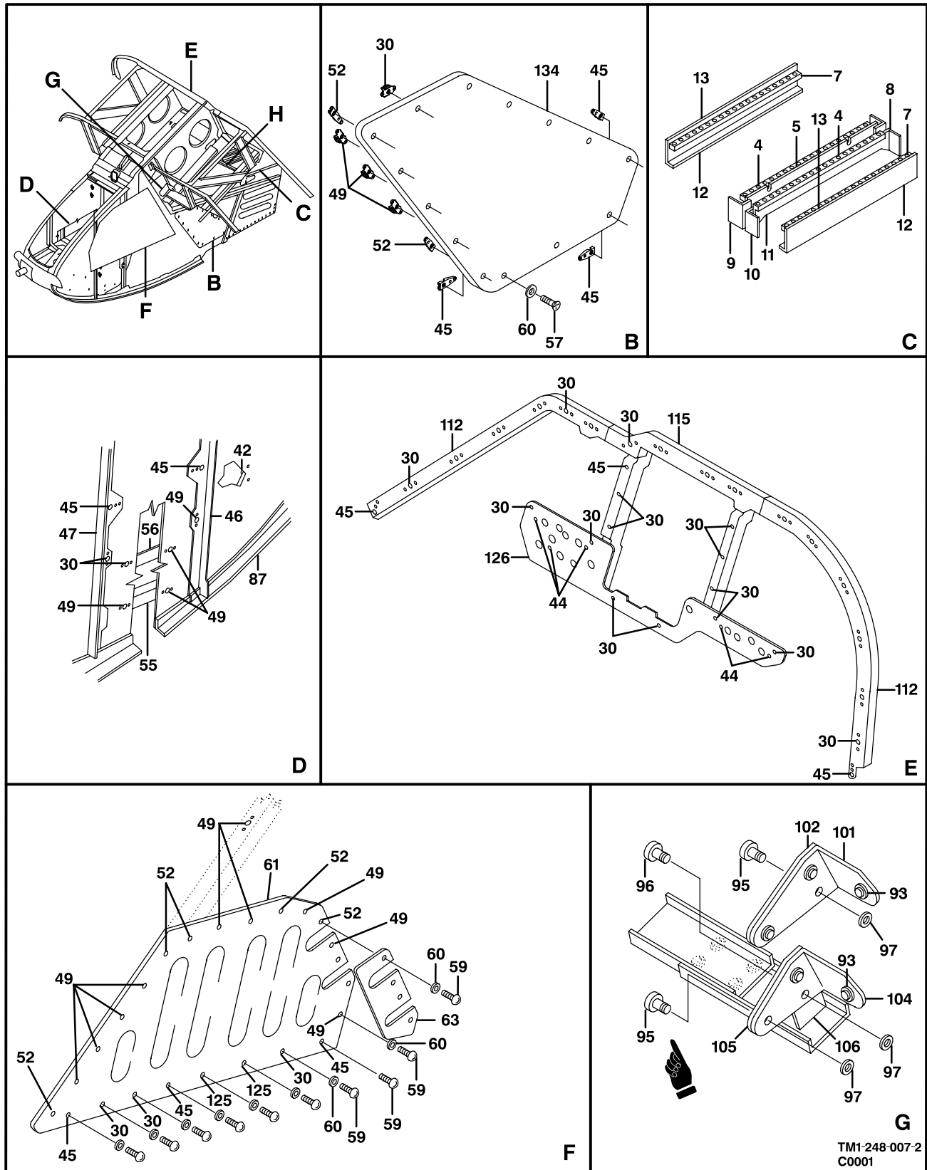
Figure 7. Console Installation (Sheet 2 of 3)
