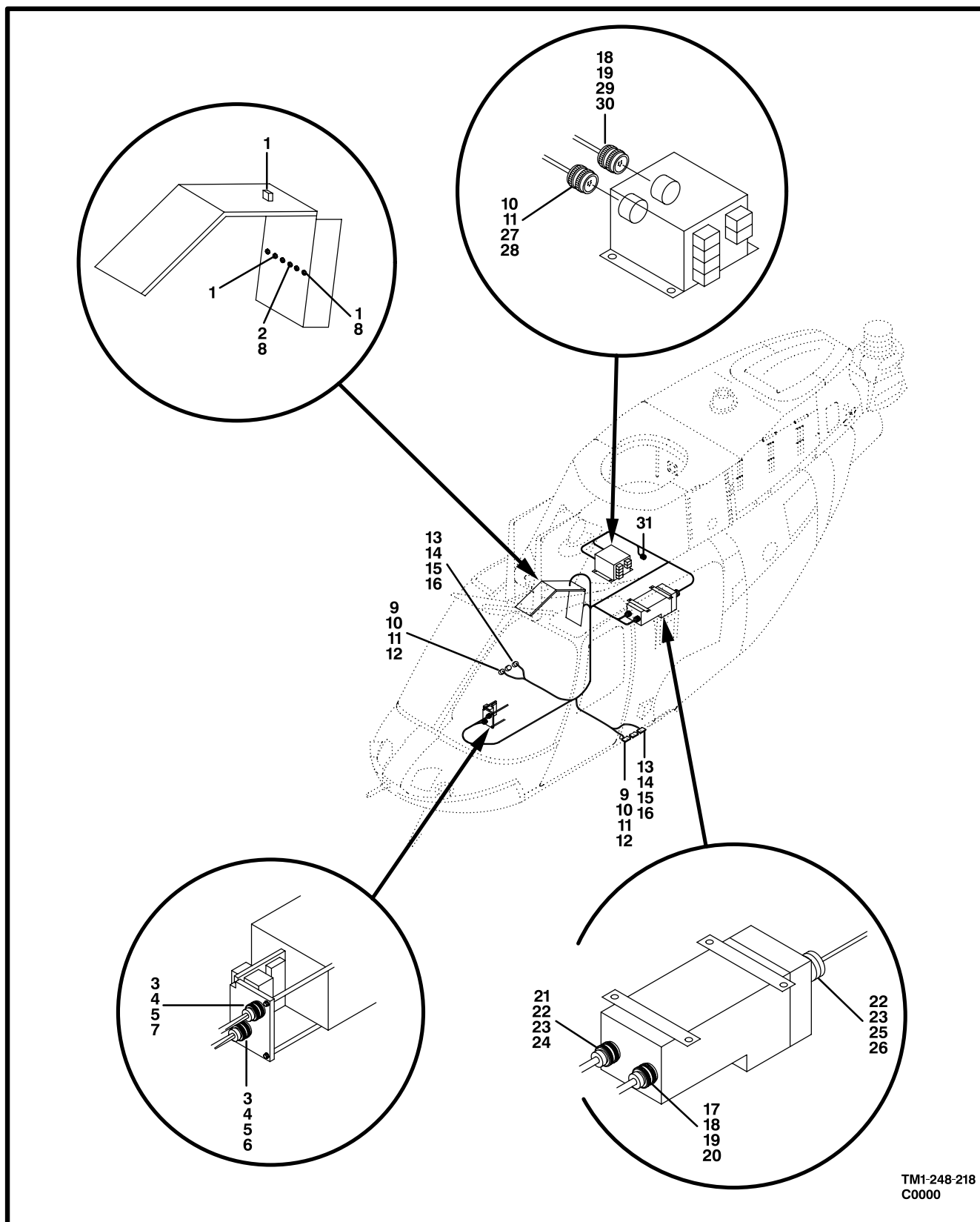
Figure 213. Cable Assembly, Guns and Rockets
