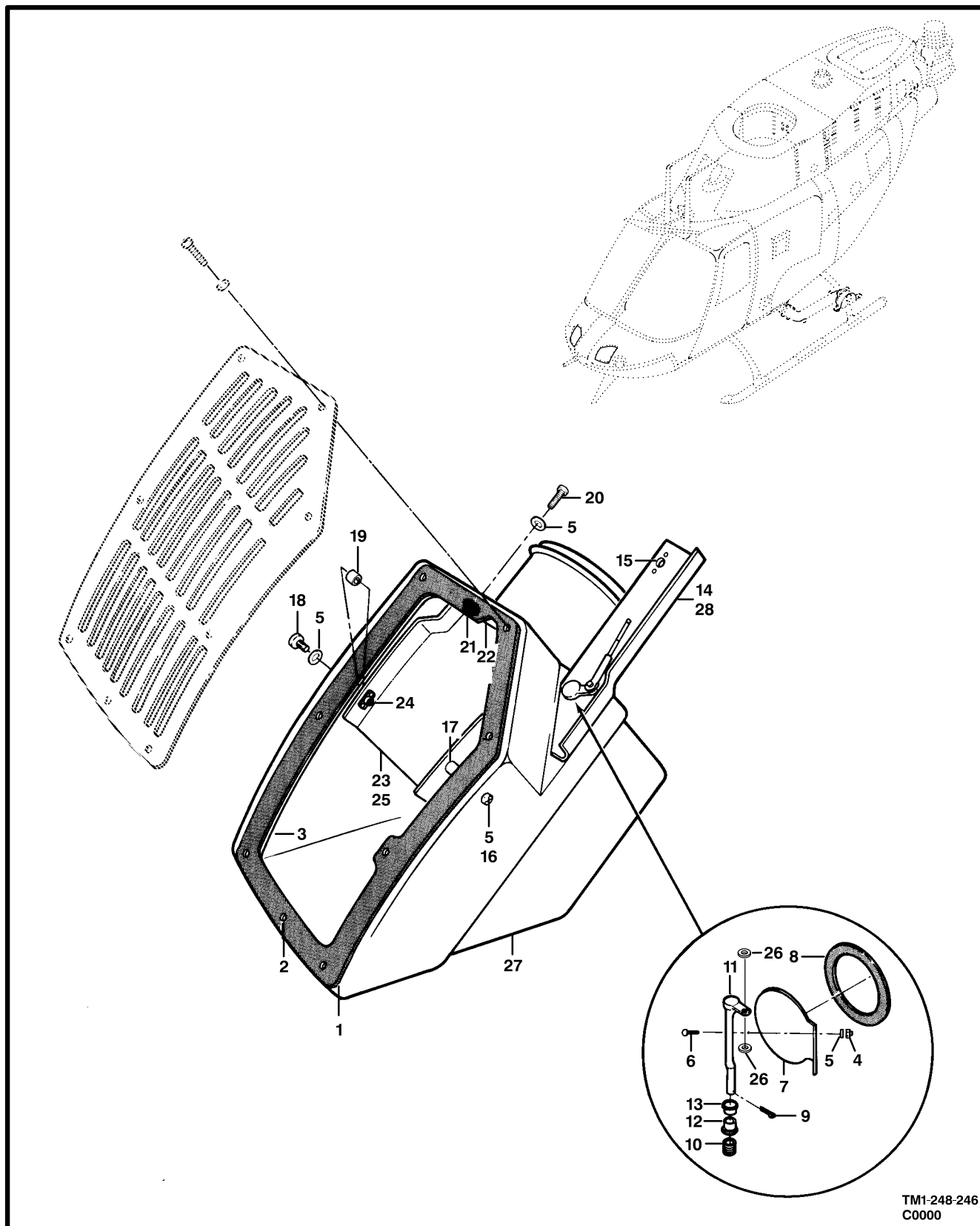
Figure 262. Plenum Assembly
