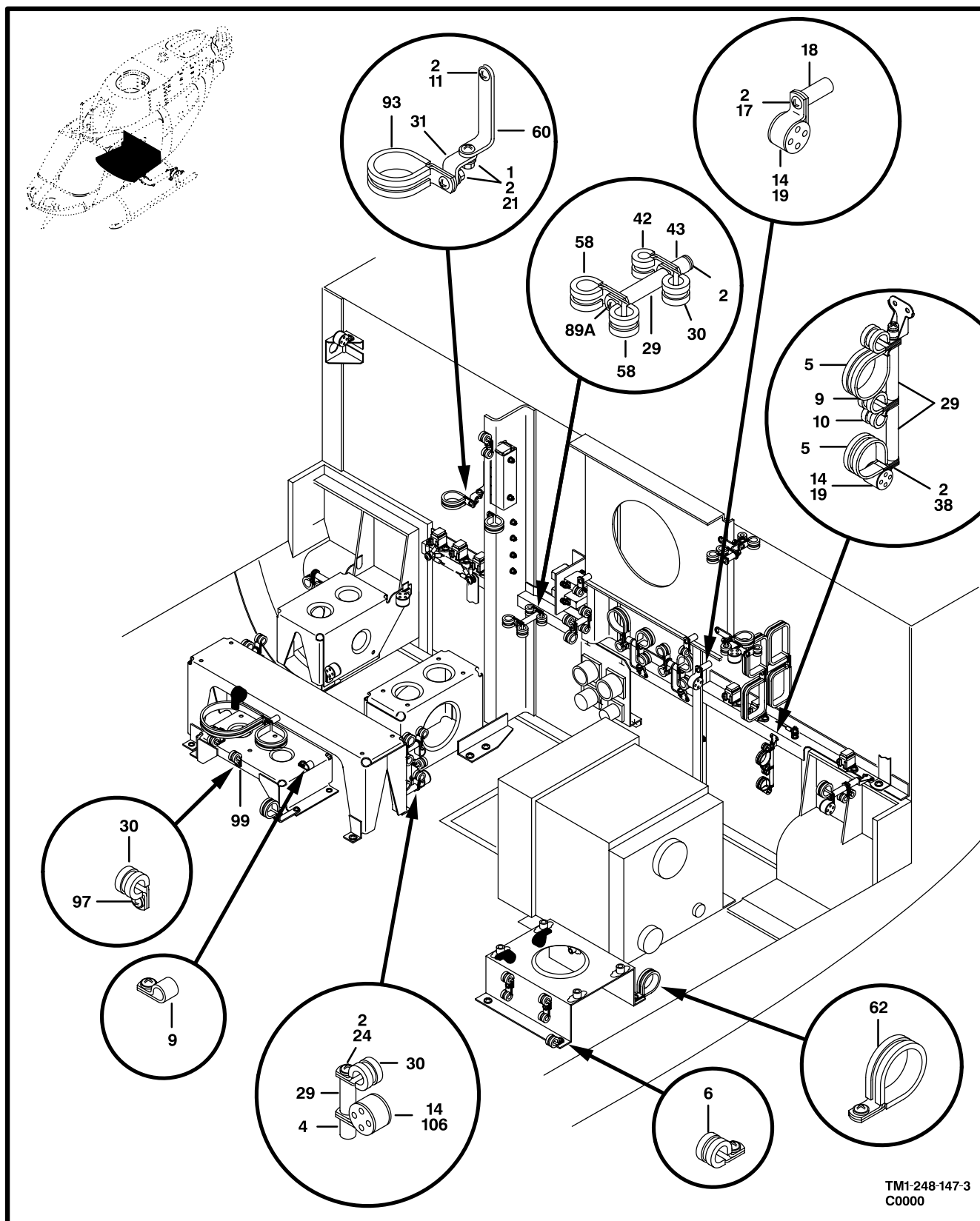
Figure 142. Electrical Installation,Bulkhead (Sheet 3 of 5)
