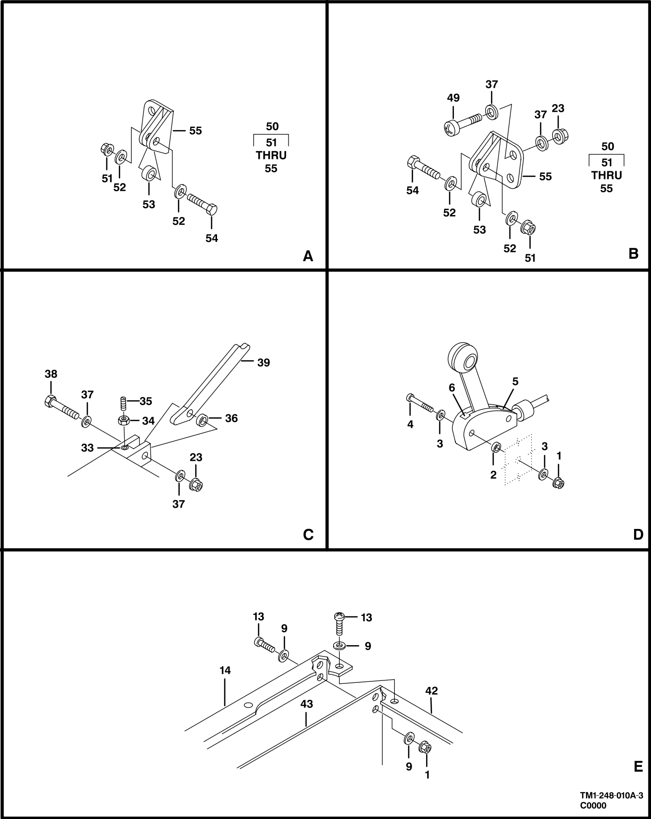
Figure 10A. Crewseat Installation, Energy Attenuating (Sheet 3 of 3)
