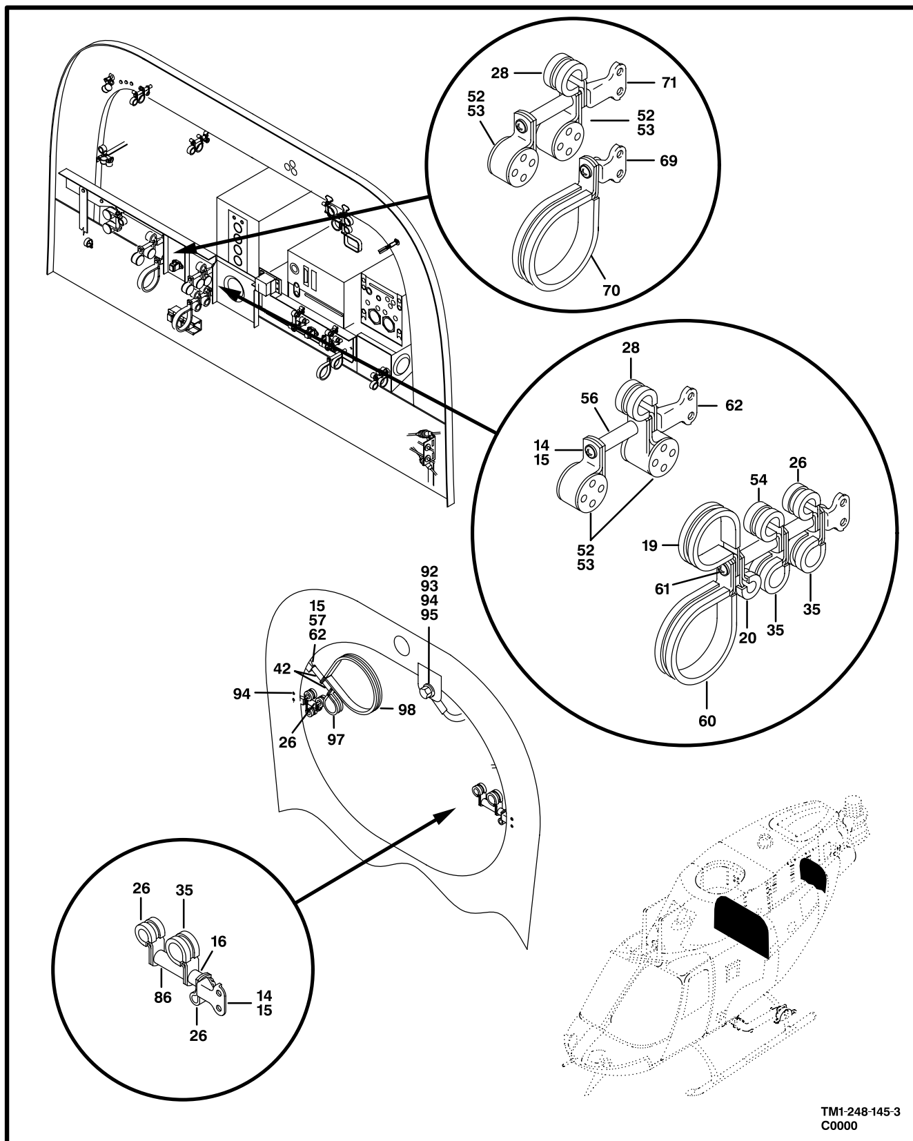
Figure 140. Electrical Installation,Bulkhead (Sheet 3 of 3)
