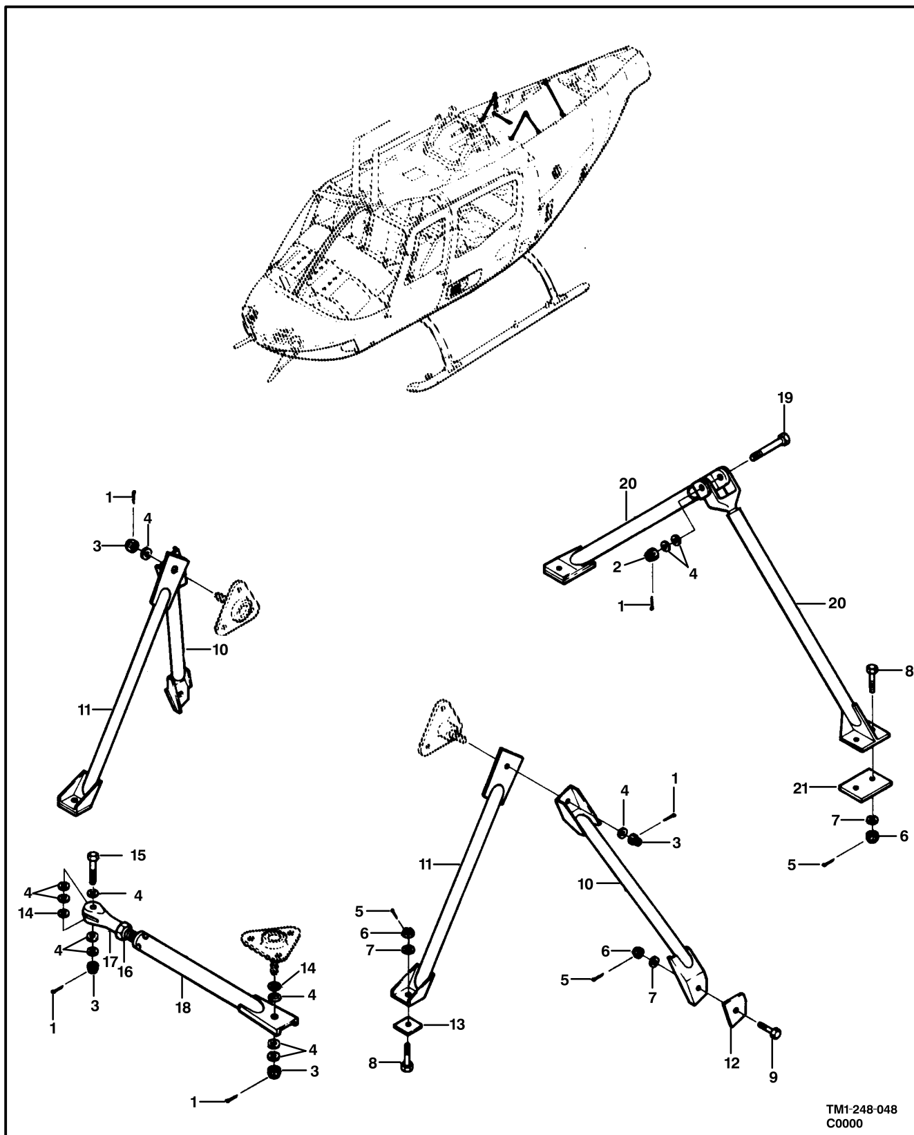
Figure 48. Engine Mount Installation
