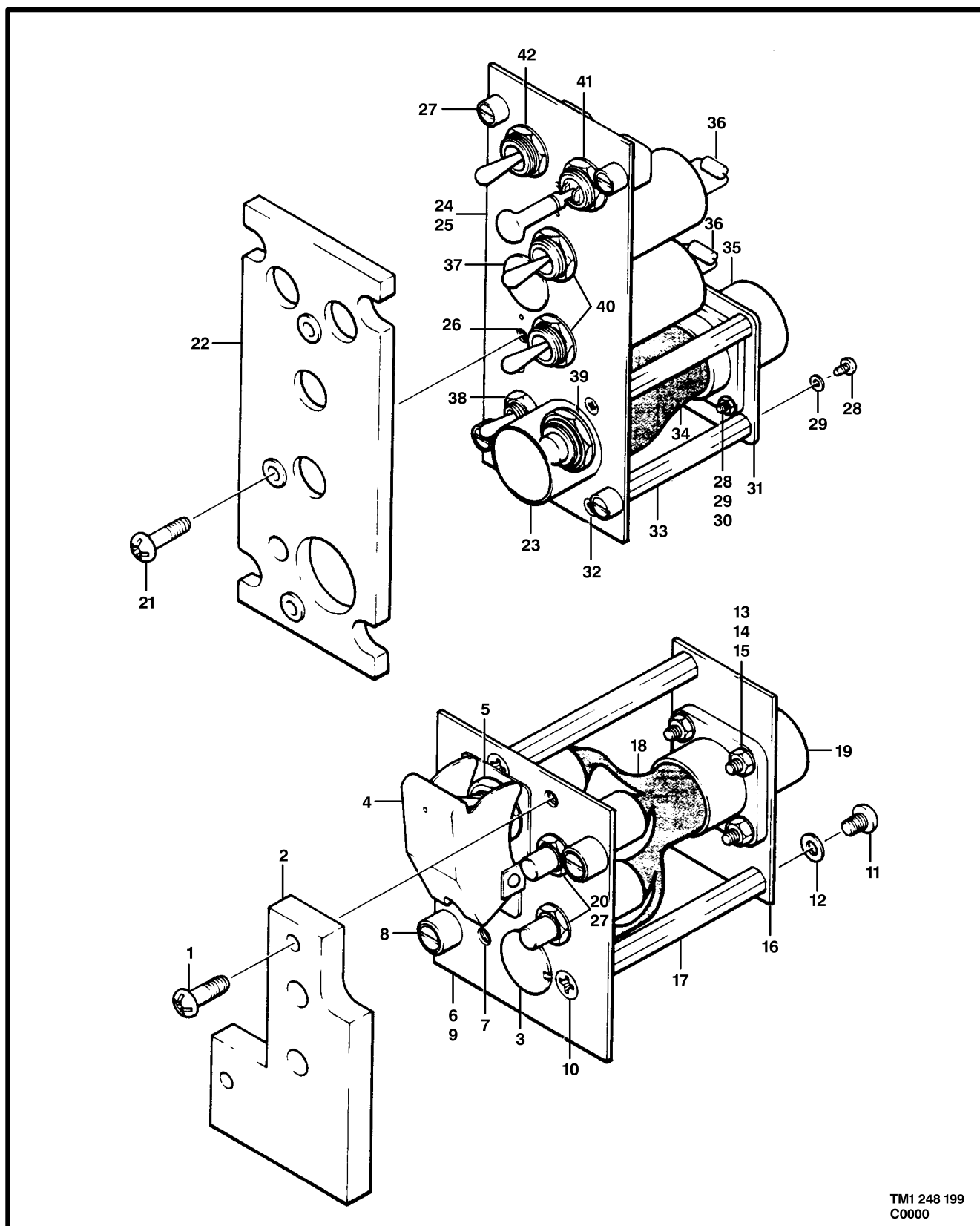
Figure 194. Panel Assembly
