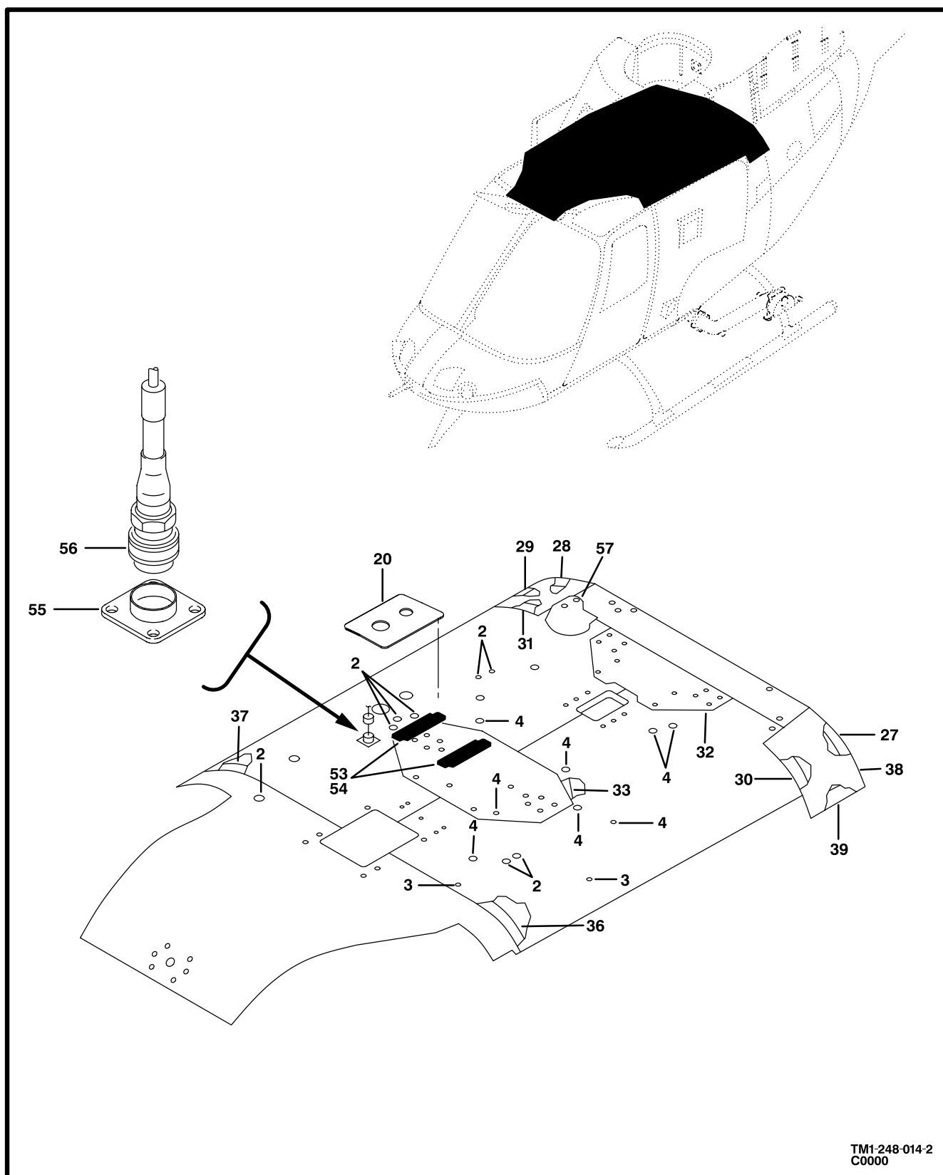
Figure 14. Shell Assembly (Sheet 2 of 2)
