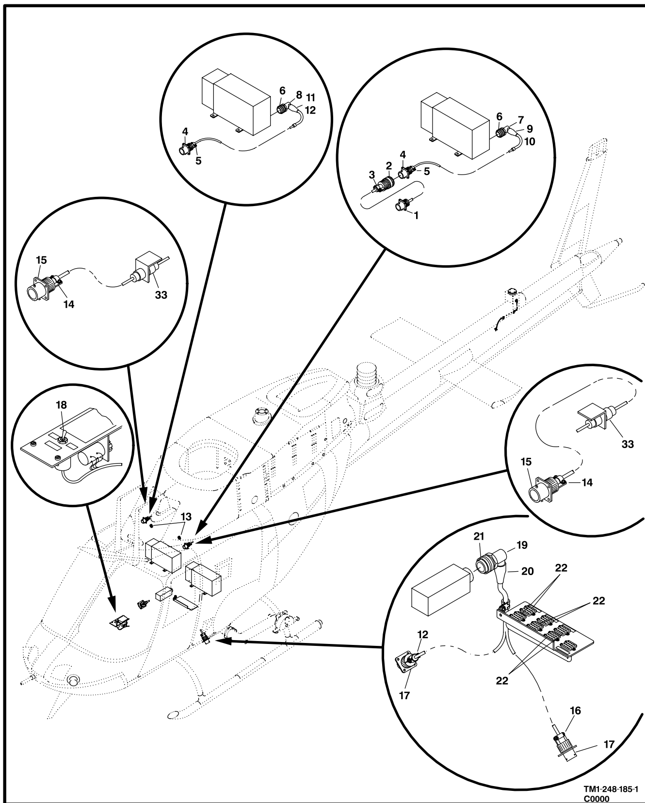
Figure 180. Cable Assembly, Lighting System (Sheet 1 of 2)
