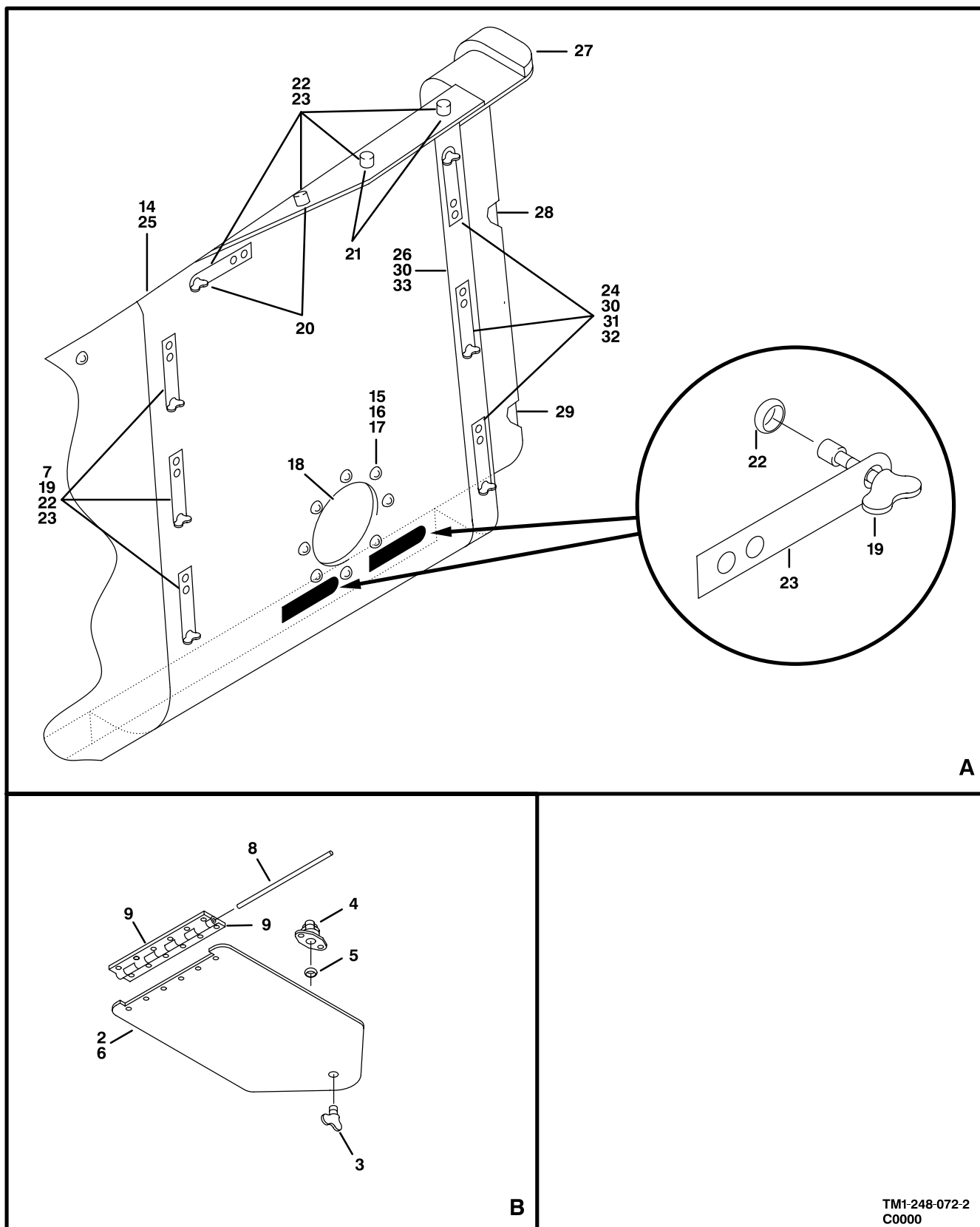
Figure 70. Shield Assembly (Sheet 2 of 2)
