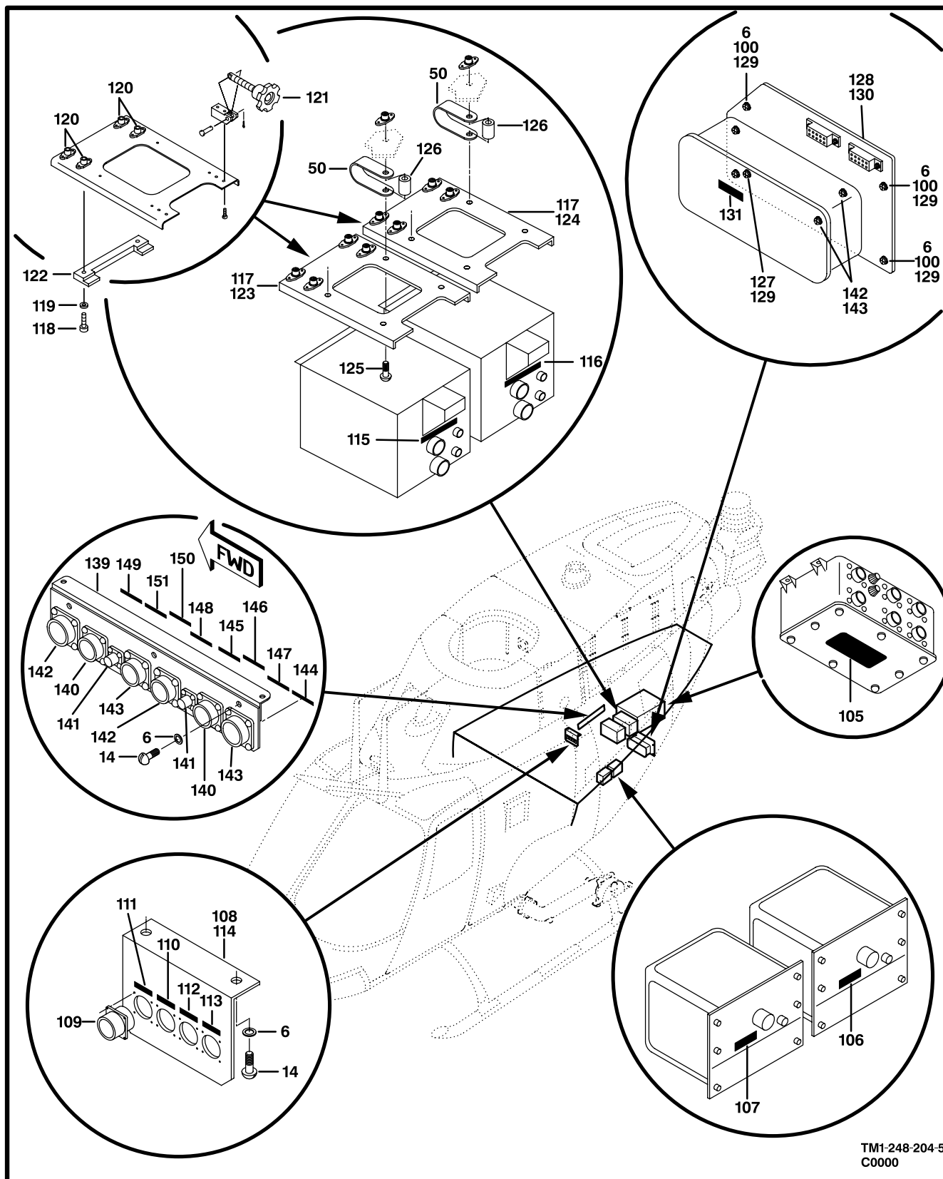
Figure 199. Electrical Assembly, Avionics Installation, AFT Cabin (Sheet 5 of 5)
