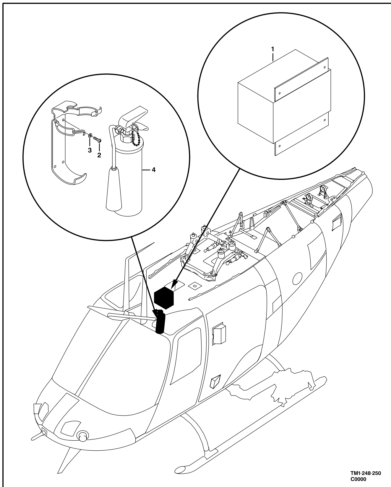
Figure 266. First Aid Kit and Fire Extinguisher Installation
