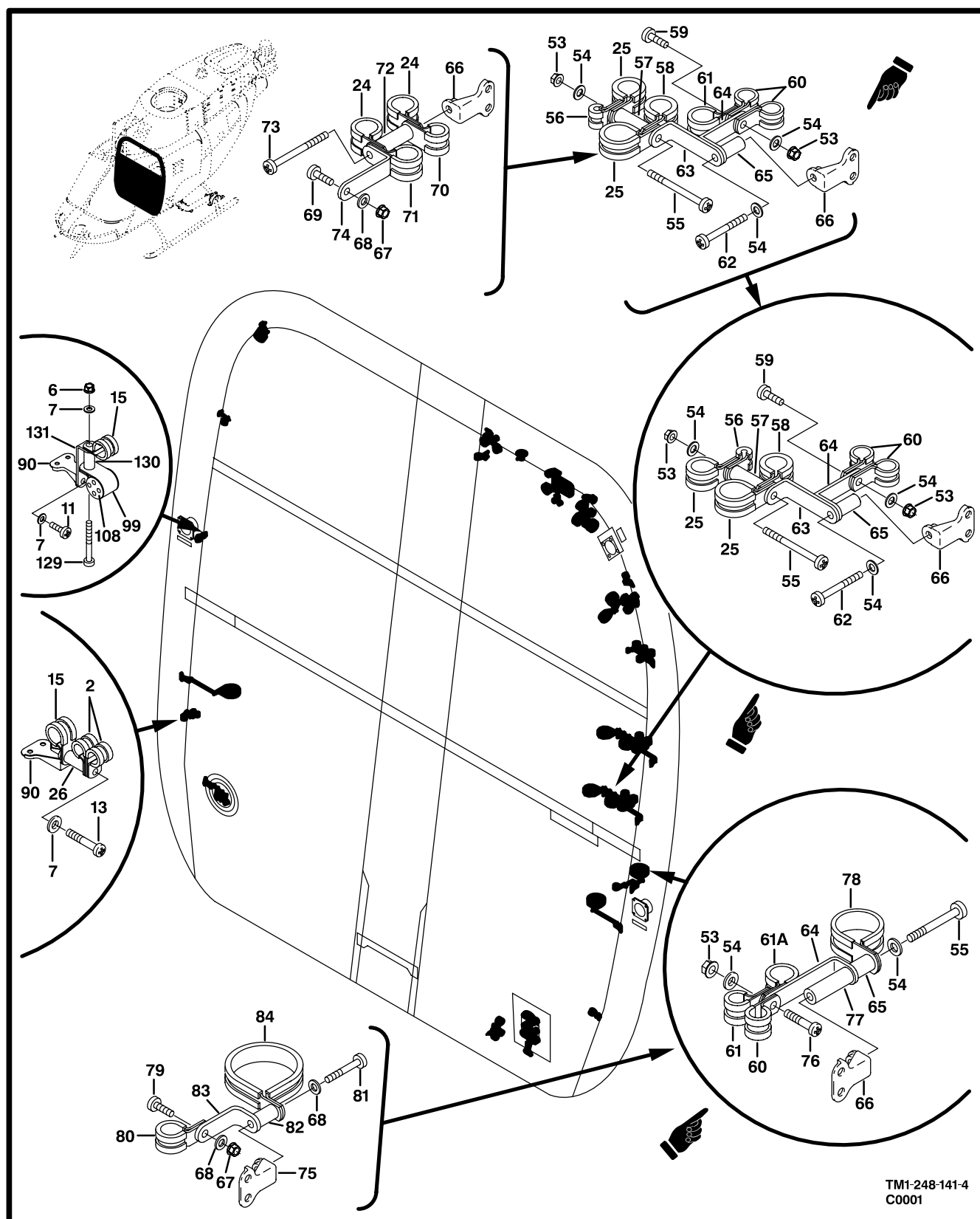
Figure 136. Electrical Installation, Bulkhead (Sheet 4 of 4)
