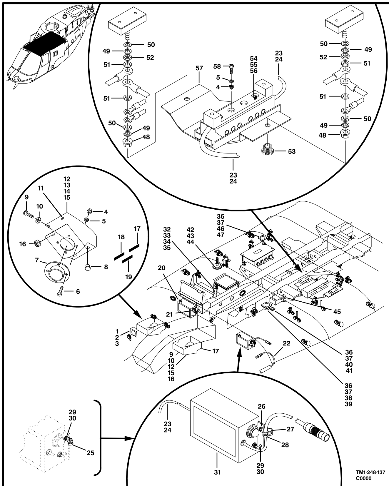
Figure 132. Electrical Installation, Roof
