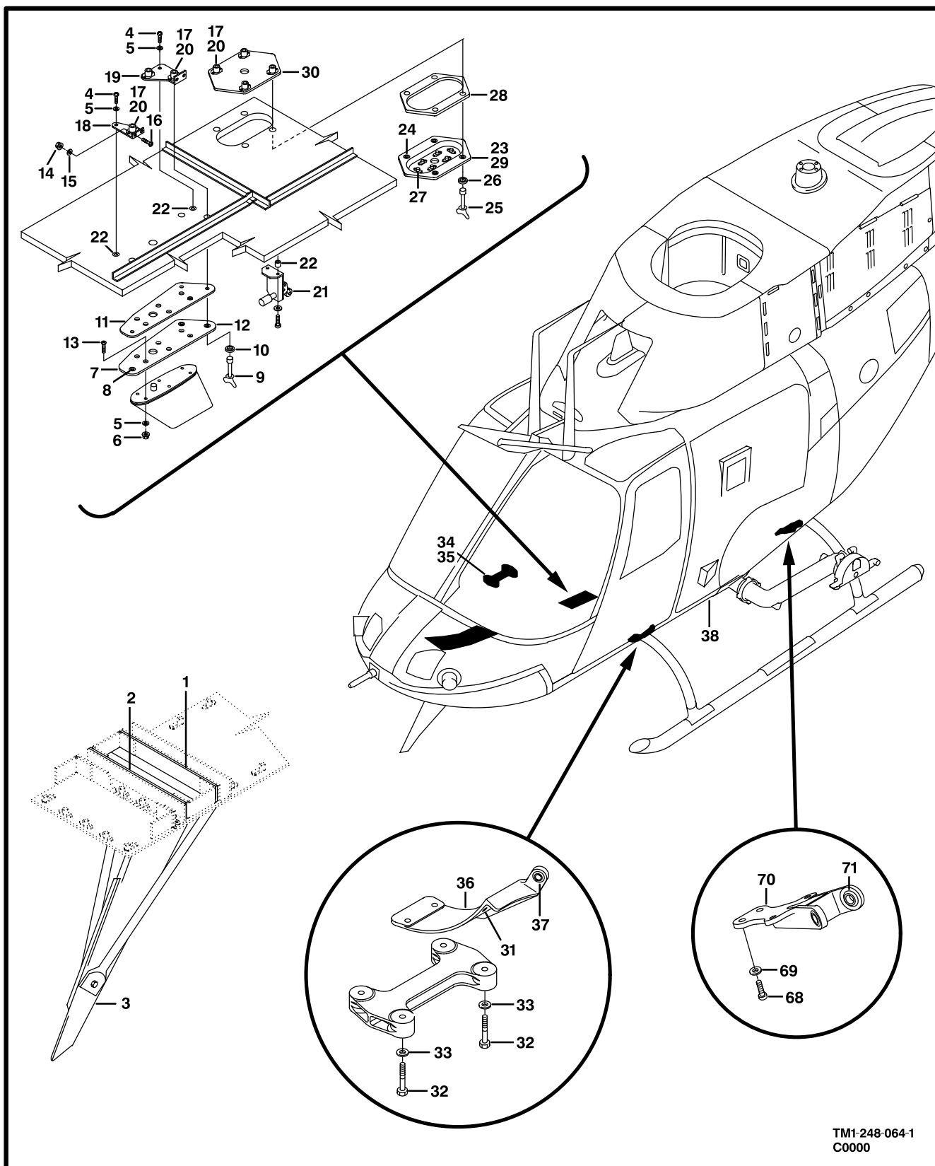
Figure 63. MOD-Fuselage Structure (Sheet 1 of 2)
