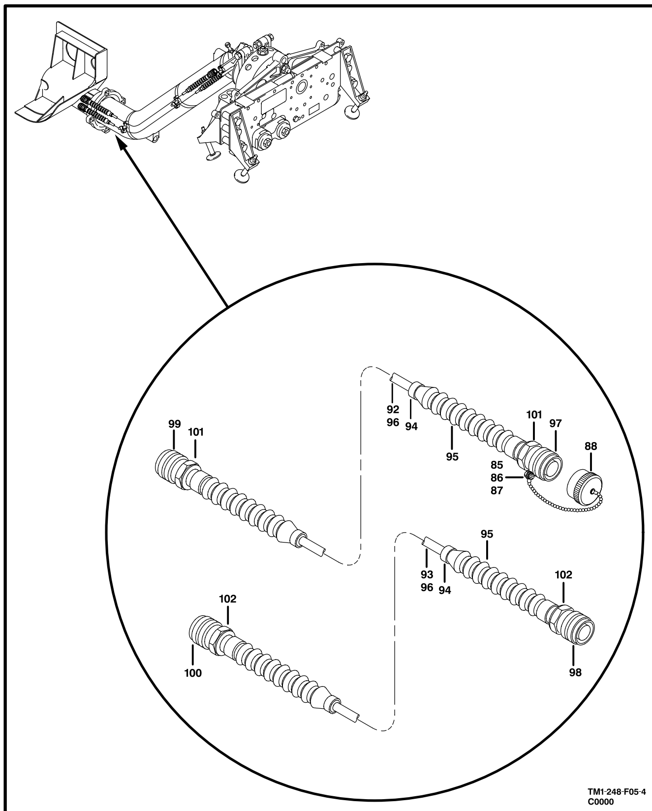
Figure F5. Universal Pylon Installation (Sheet 4 of 4)
