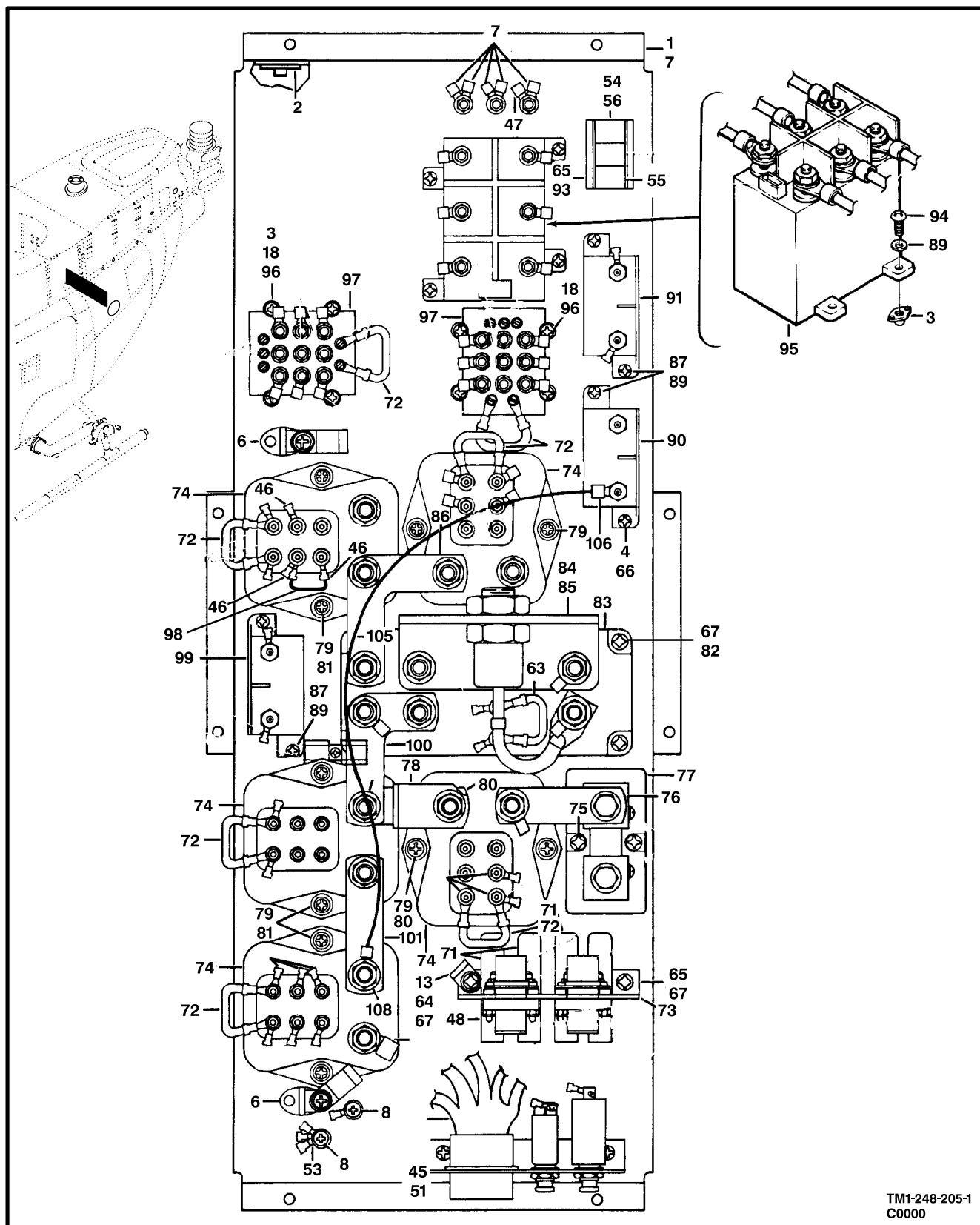
Figure 200. Electrical Assembly, DC Equipment (Sheet 1 of 2)
