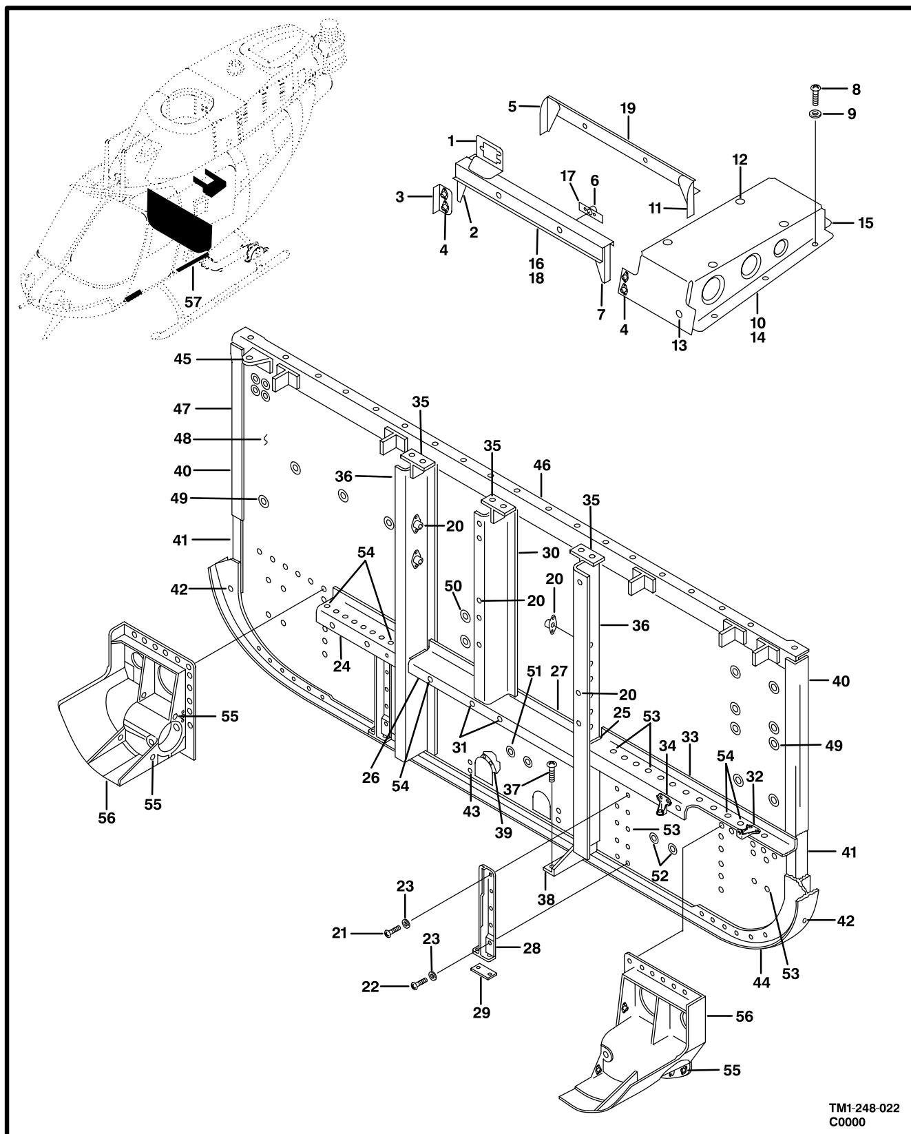
Figure 22. Support Installation, Electrical
