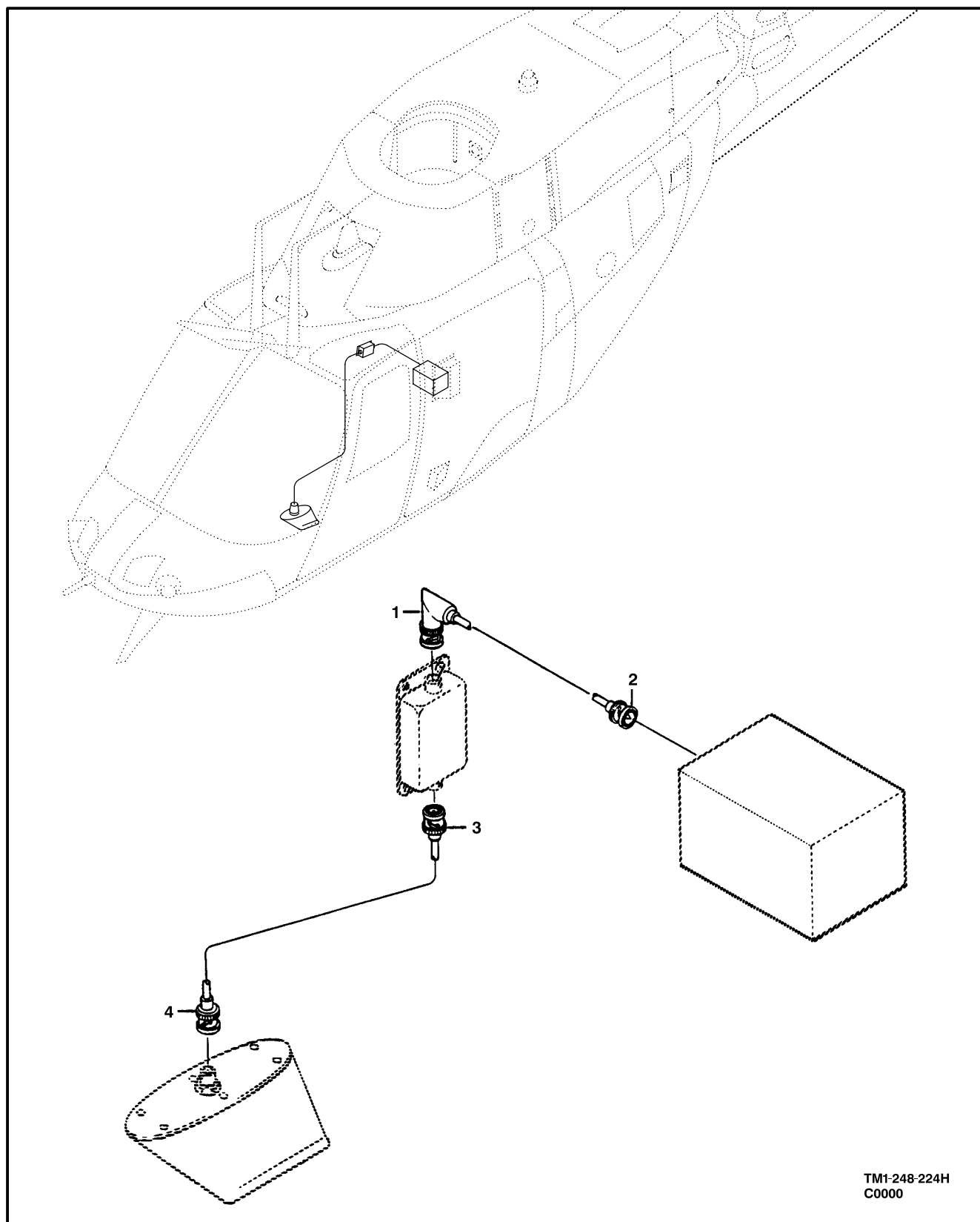
Figure 226. Cable Assembly,UHF-AM Communication System
