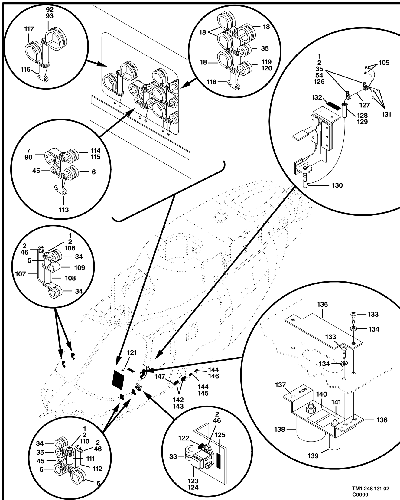
Figure 126. Electrical Installation, Nose (Sheet 2 of 2)
