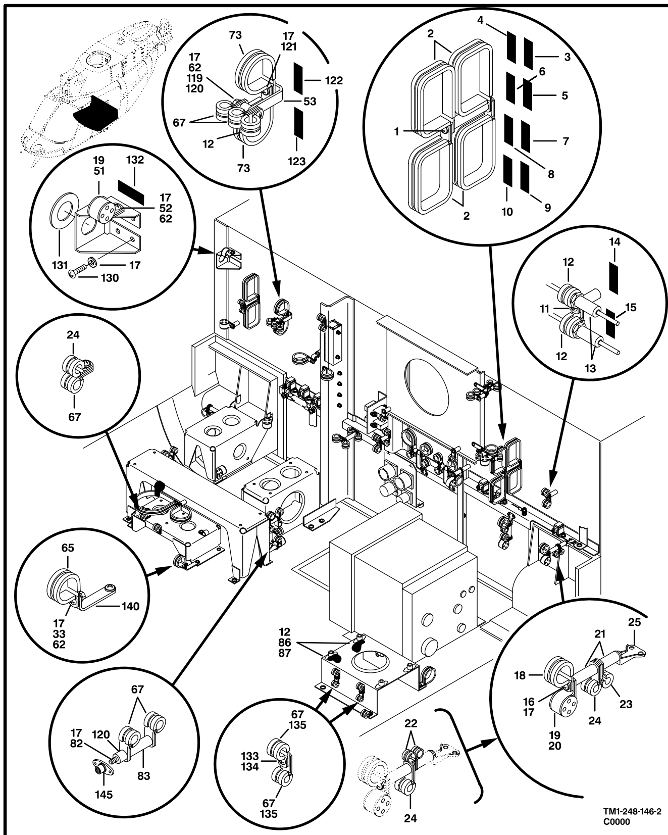
Figure 141. Electrical Installation,Bulkhead (Sheet 2 of 4)
