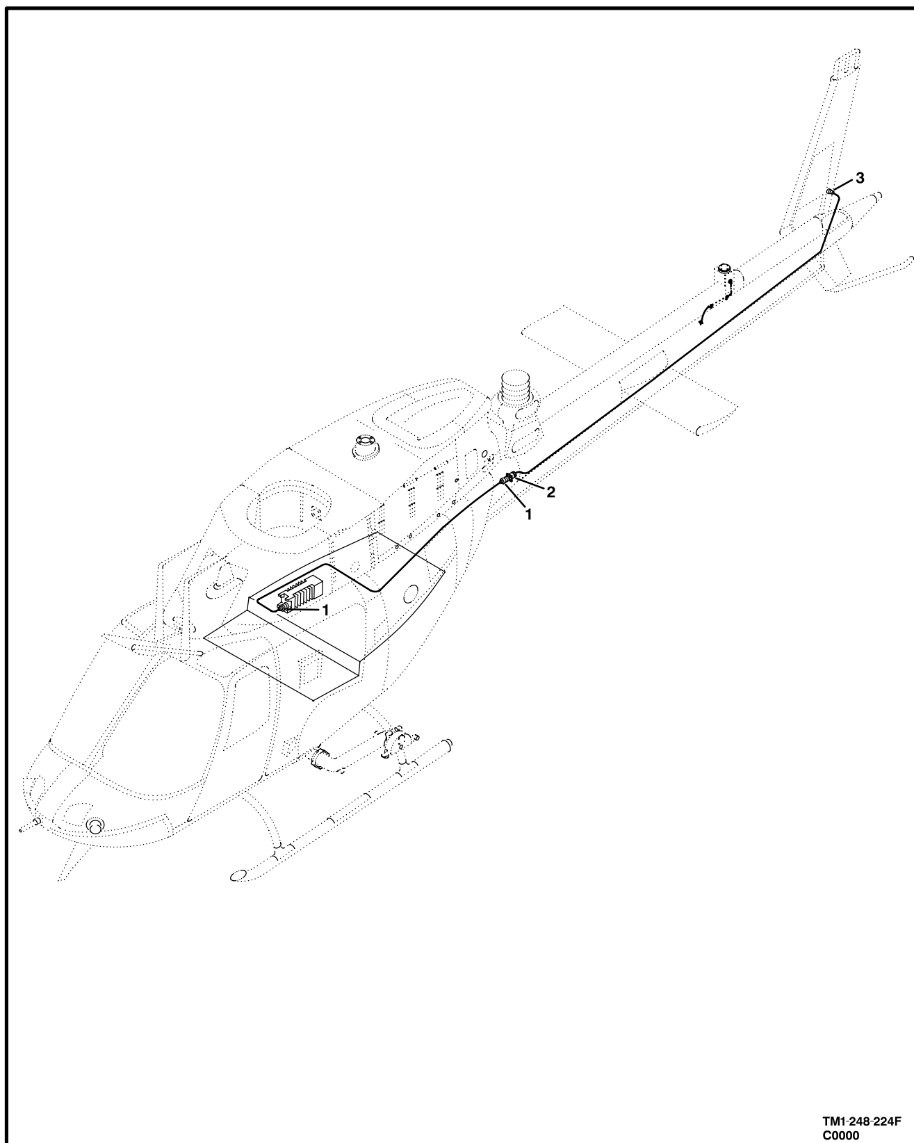
Figure 224. Cable Assembly,VHF-FM Communication System
