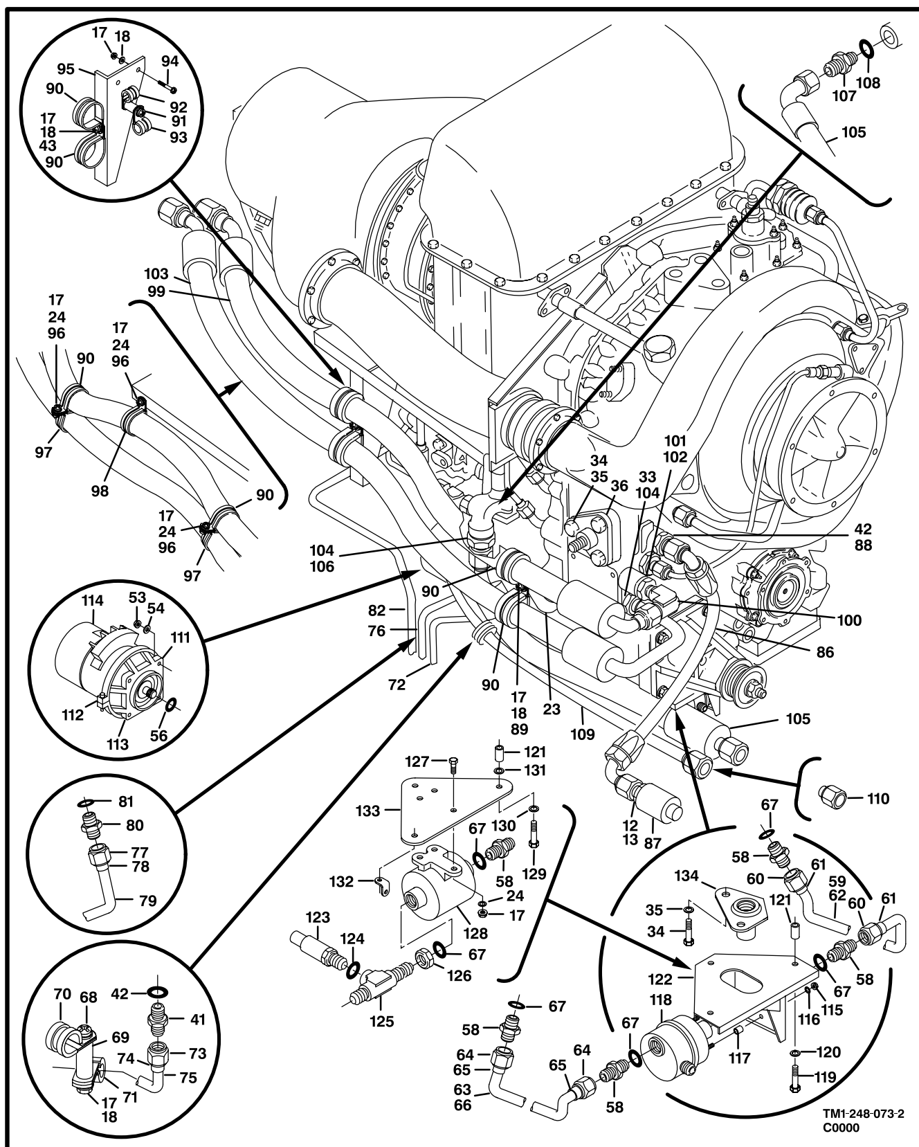
Figure 71. Engine Assembly (Sheet 2 of 2)
