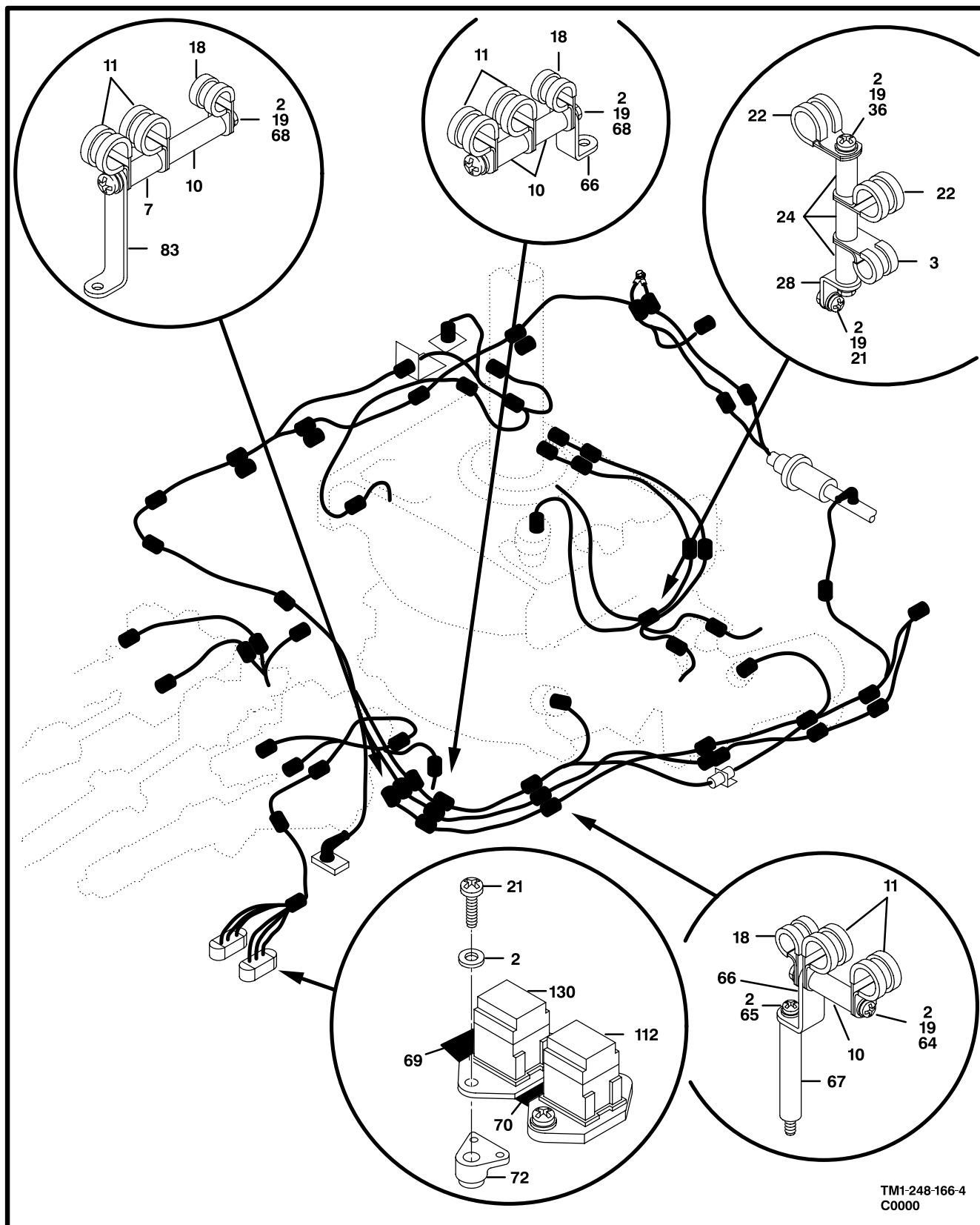
Figure 161. Electrical Installation, Mast Mounted Sight (Sheet 4 of 6)
