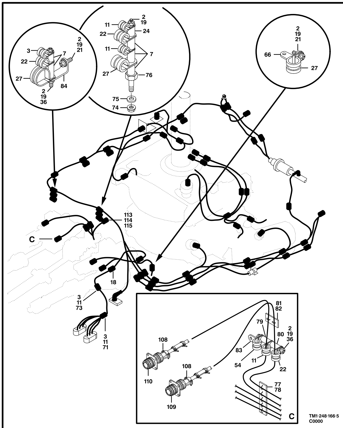
Figure 161. Electrical Installation, Mast Mounted Sight (Sheet 5 of 6)
