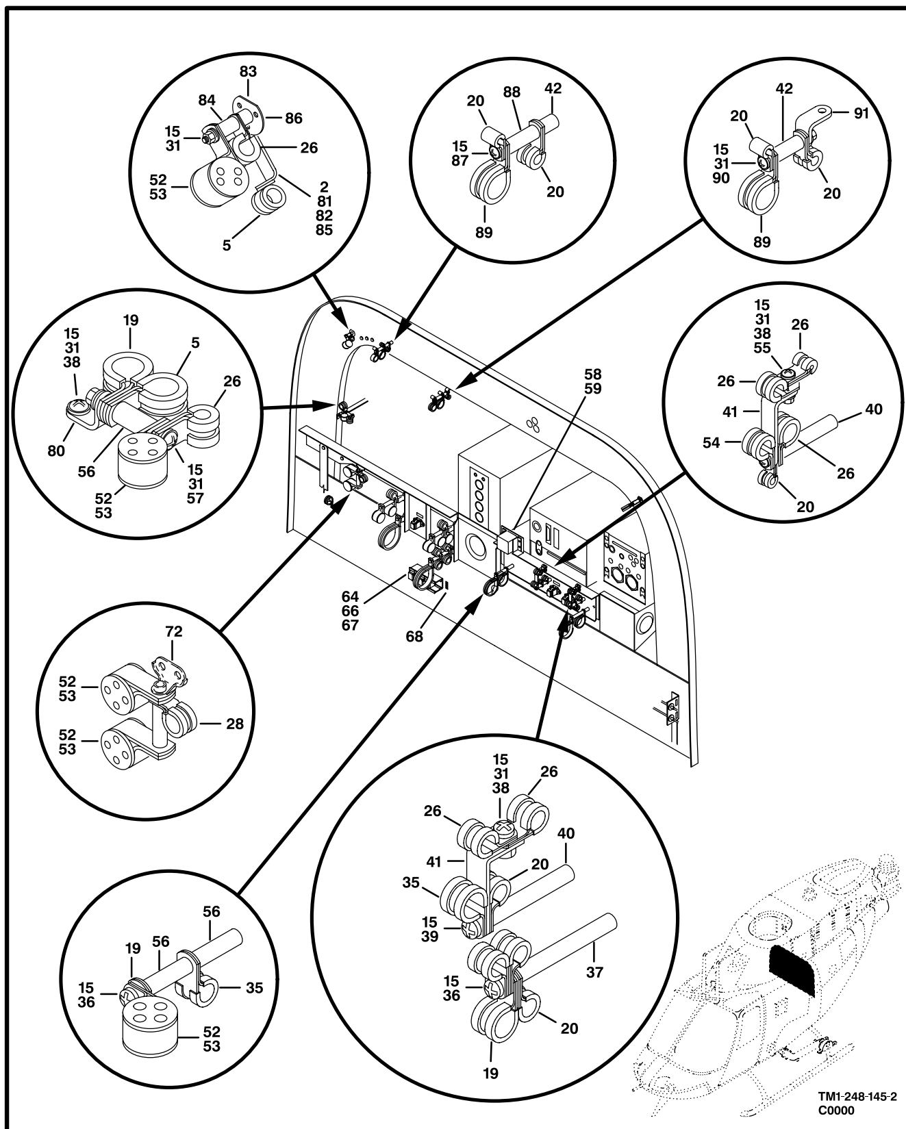
Figure 140. Electrical Installation, Bulkhead (Sheet 2 of 3)
