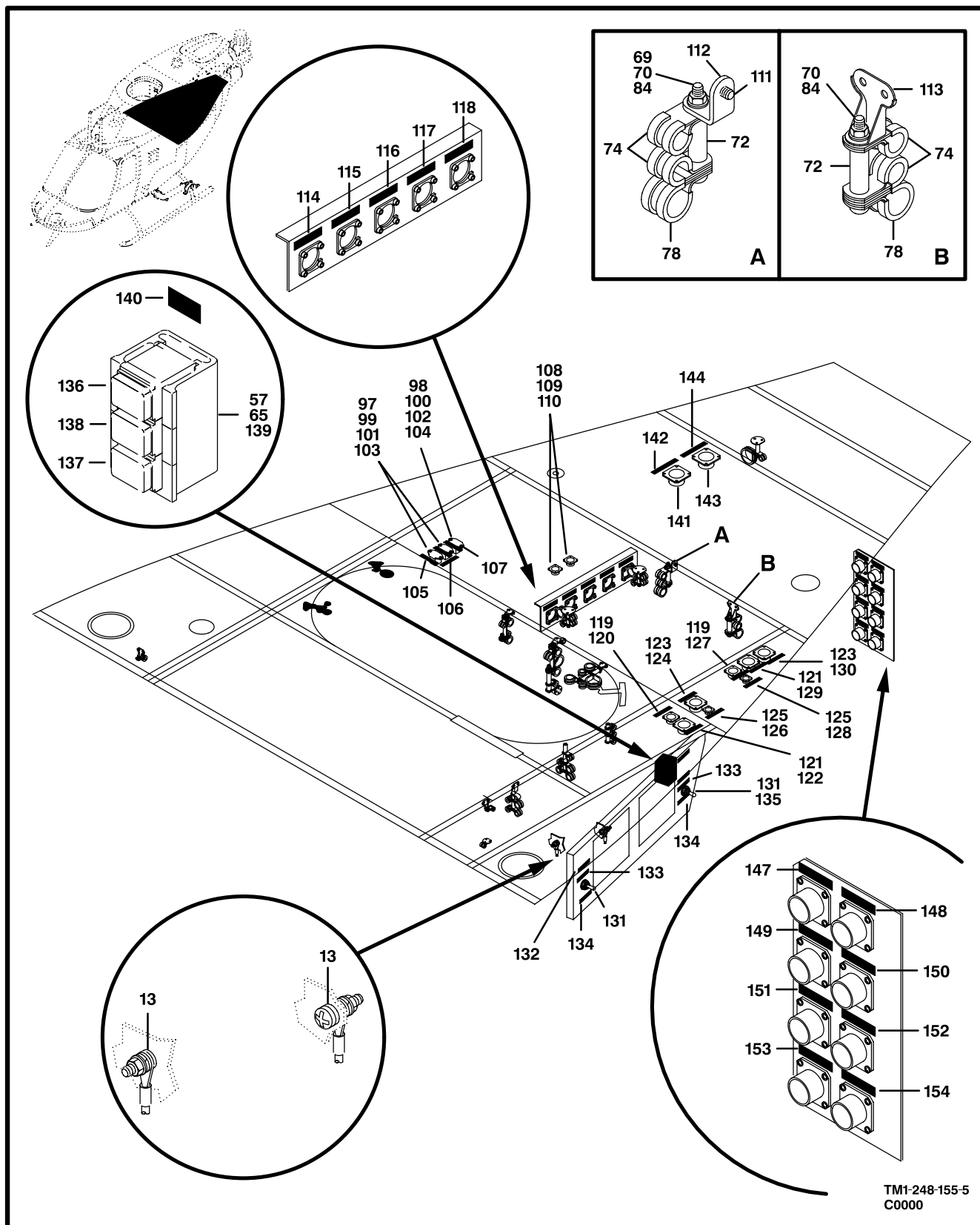
Figure 150. Electrical Installation, Canted Web (Sheet 5 of 5)
