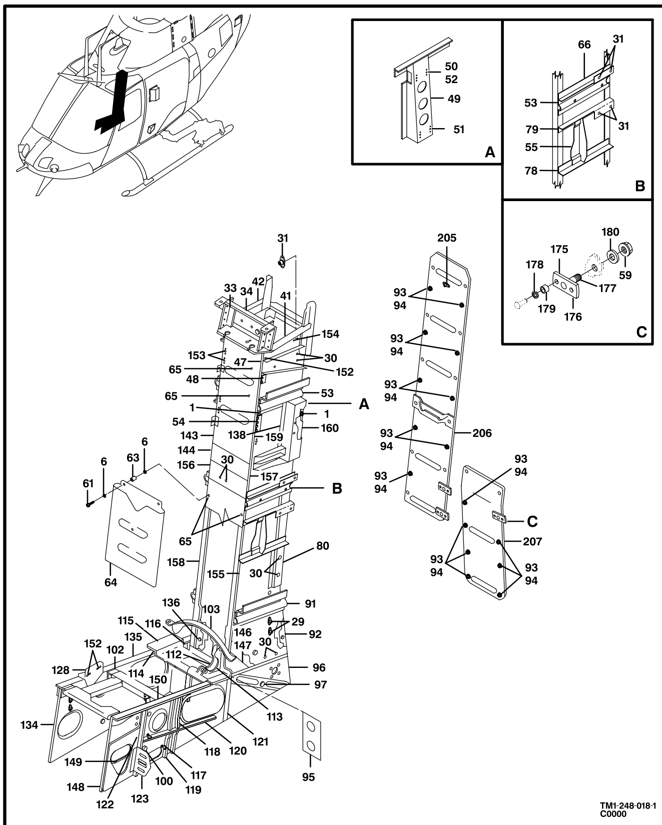
Figure 18. MOD-Support, Post/Door Assy, Center Post, AFT Access (Sheet 1 of 4)
