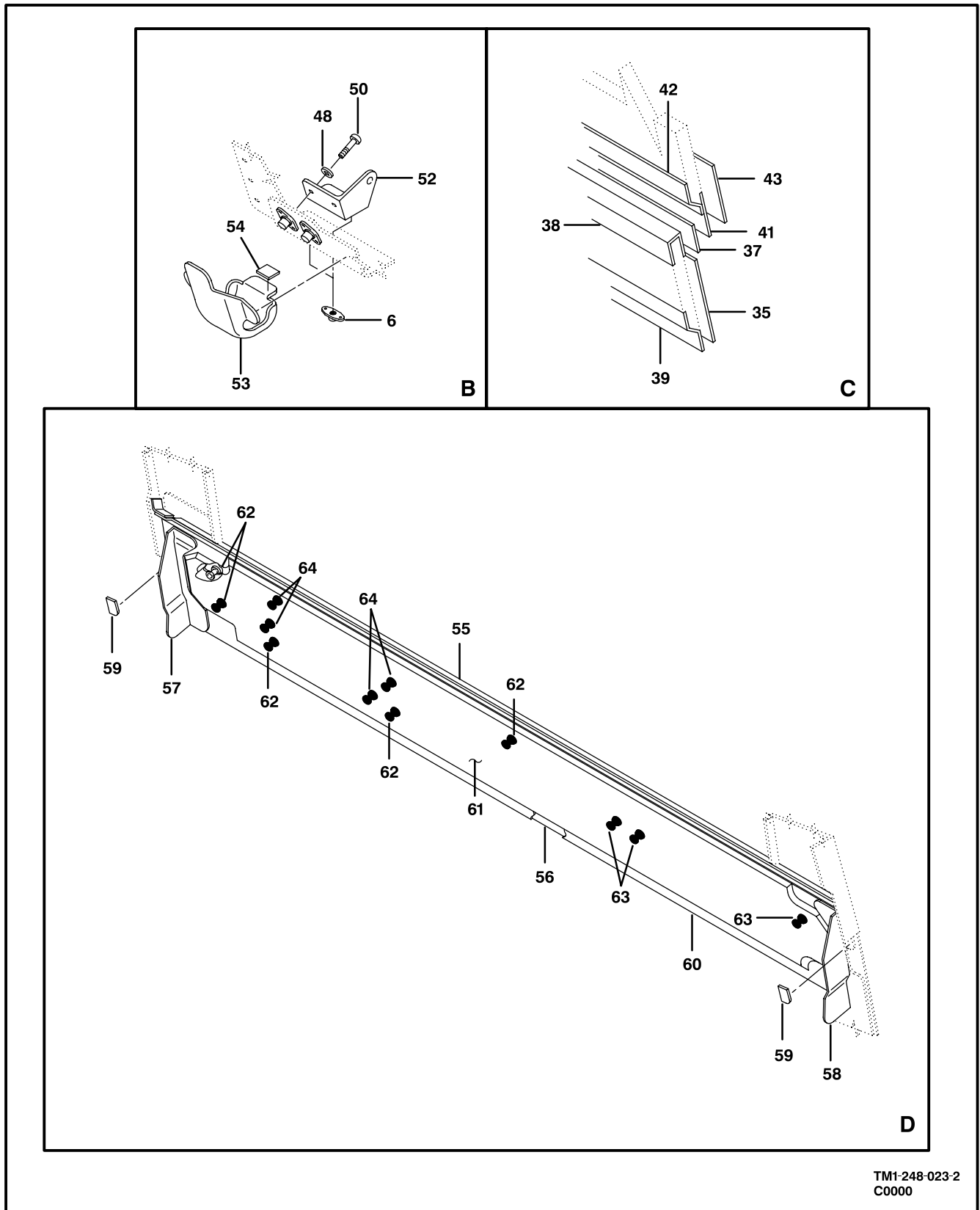
Figure 23. Bulkhead Installation (Sheet 2 of 2)
