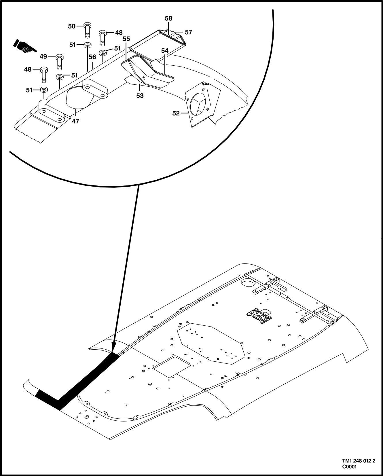
Figure 12. MOD-Roof,FWD (Sheet 2 of 2)
