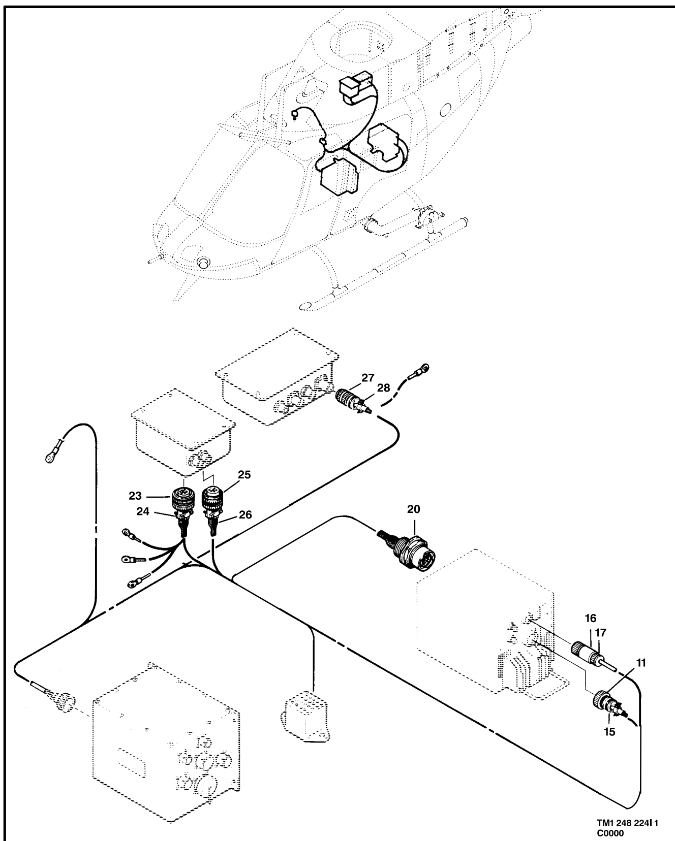
Figure 227. Cable Assembly, NO. 2 VHF-FM Communication System (Sheet 1 of 3)
