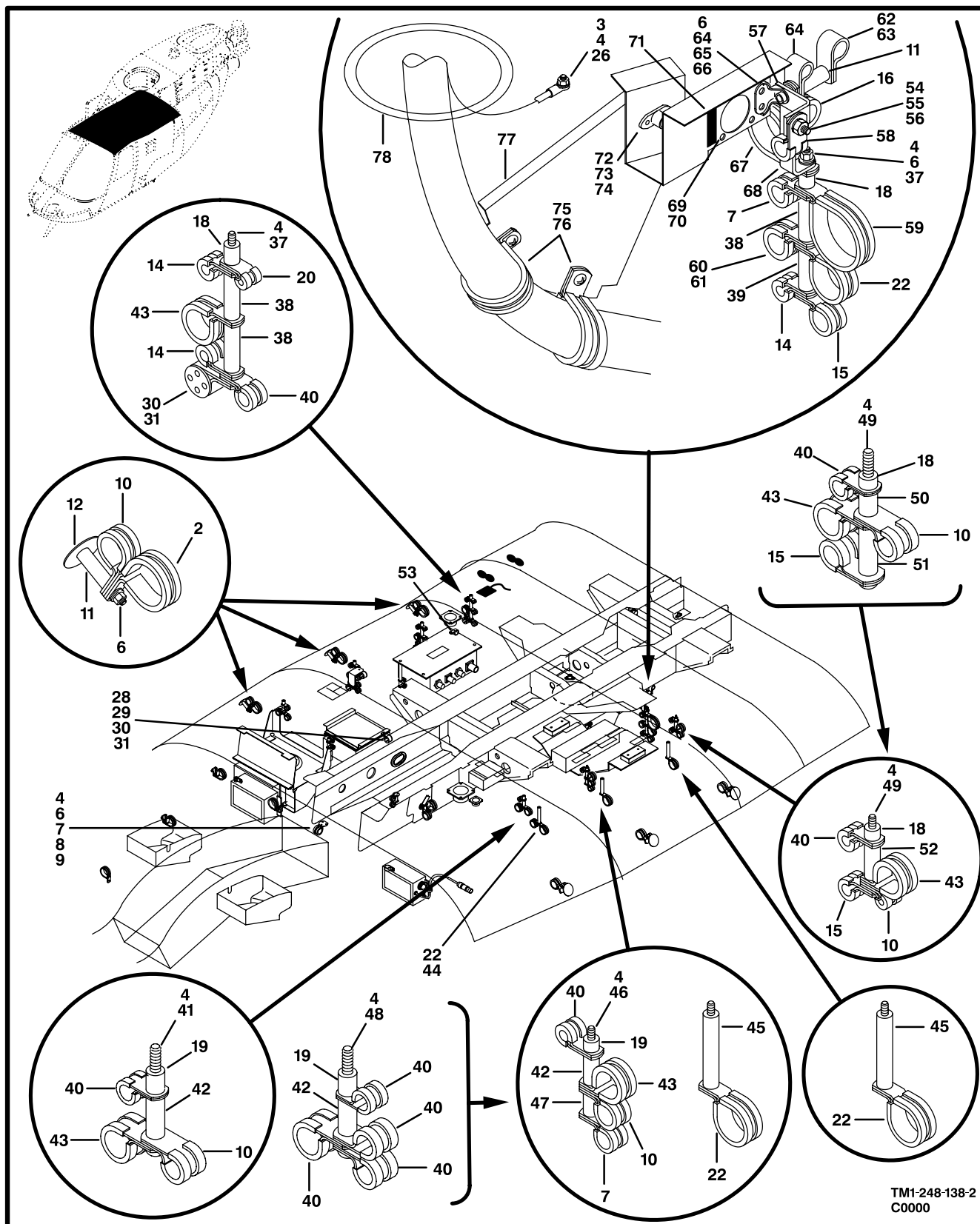
Figure 133. Electrical Installation,Bulkhead (Sheet 2 of 2)
