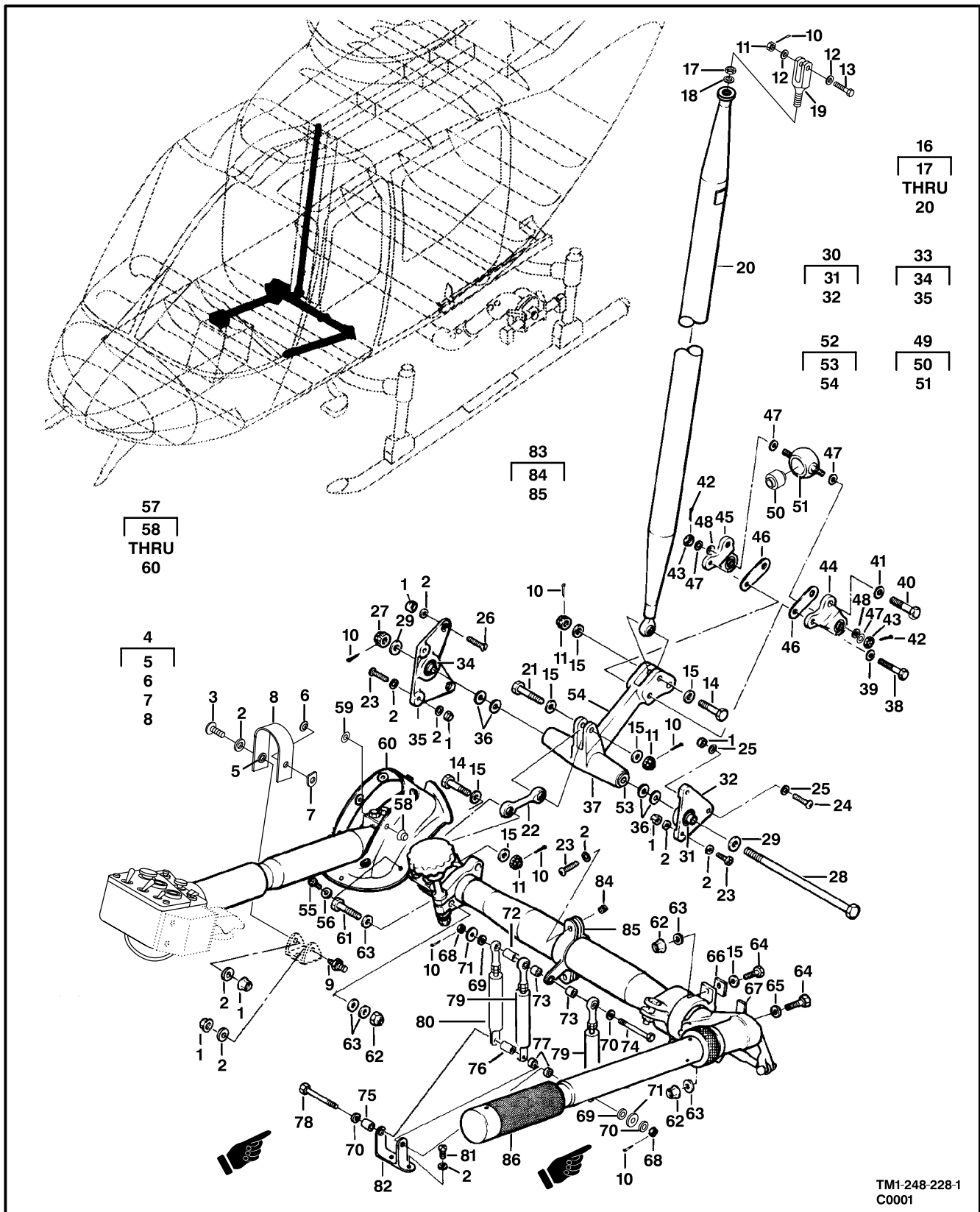
Figure 246. Controls Installation, Collective Pitch (Sheet 1 of 2)
