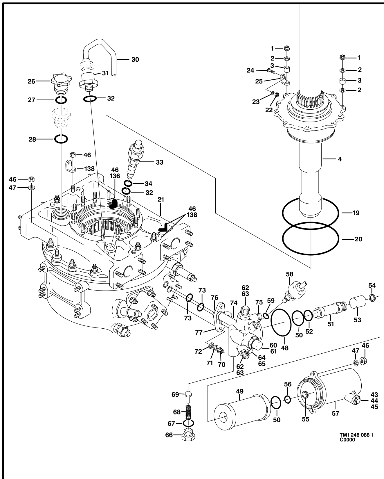
Figure 86. Transmission and Mast Assembly (Sheet 1 of 4)
