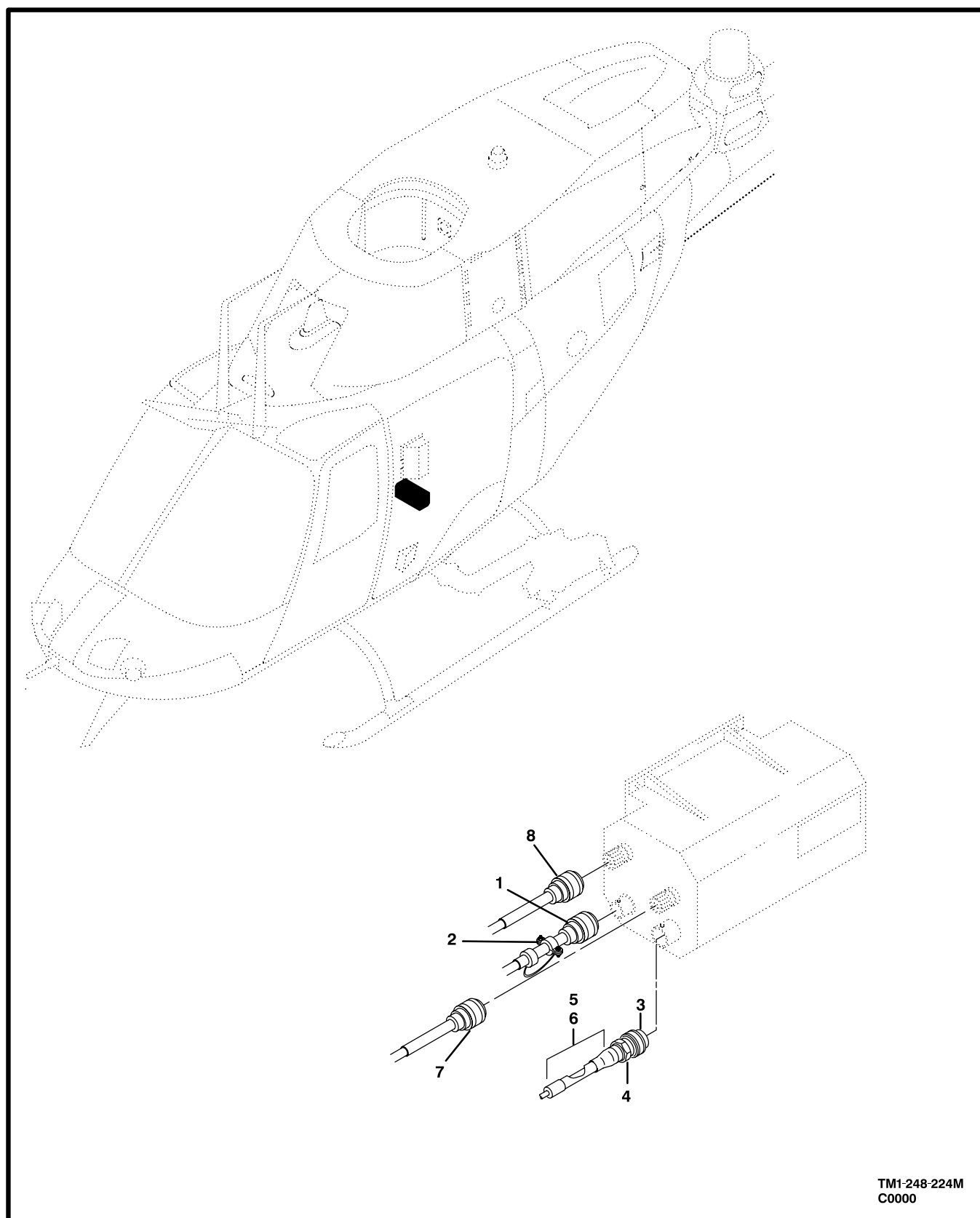
Figure 231. Cable Assembly,Radar Altimeter
