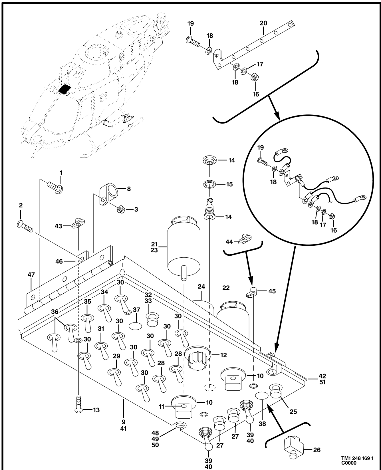
Figure 164. Console Installation, Overhead Electrical (Sheet 1 of 4)
