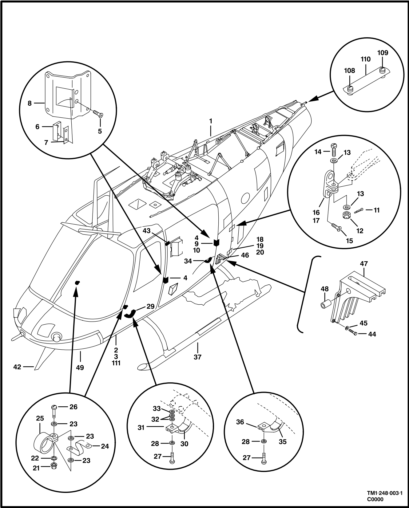
Figure 3. Fuselage Assembly (Sheet 1 of 4)
