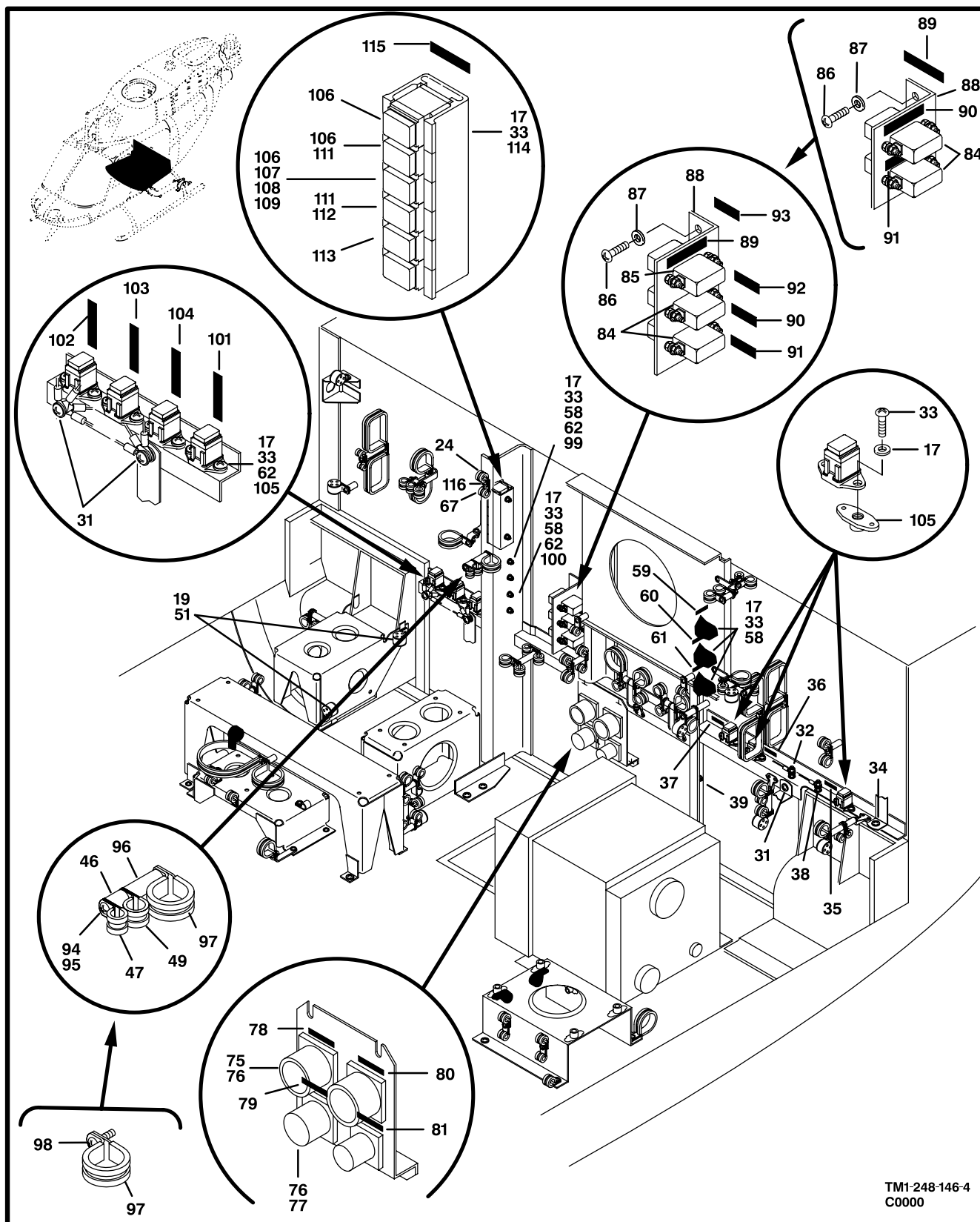
Figure 141. Electrical Installation,Bulkhead (Sheet 4 of 4)
