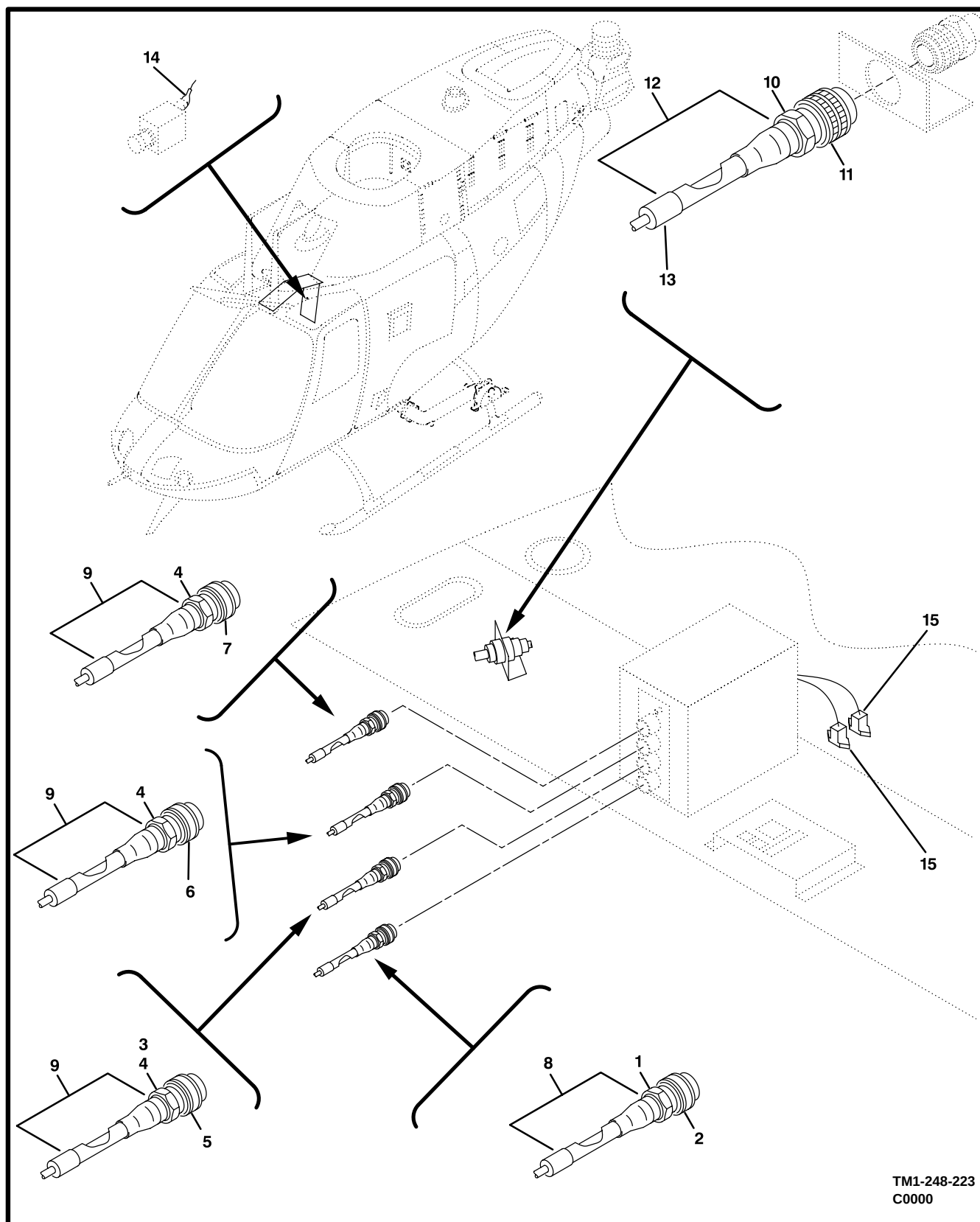
Figure 217. Improved Data Modem Cable Assembly
