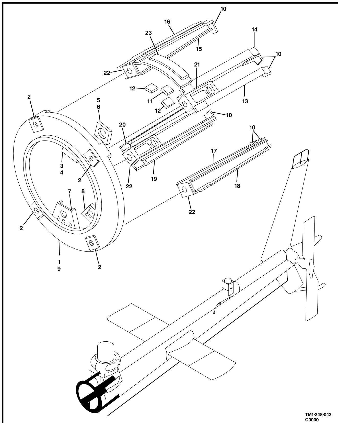
Figure 43. Bulkhead Installation
