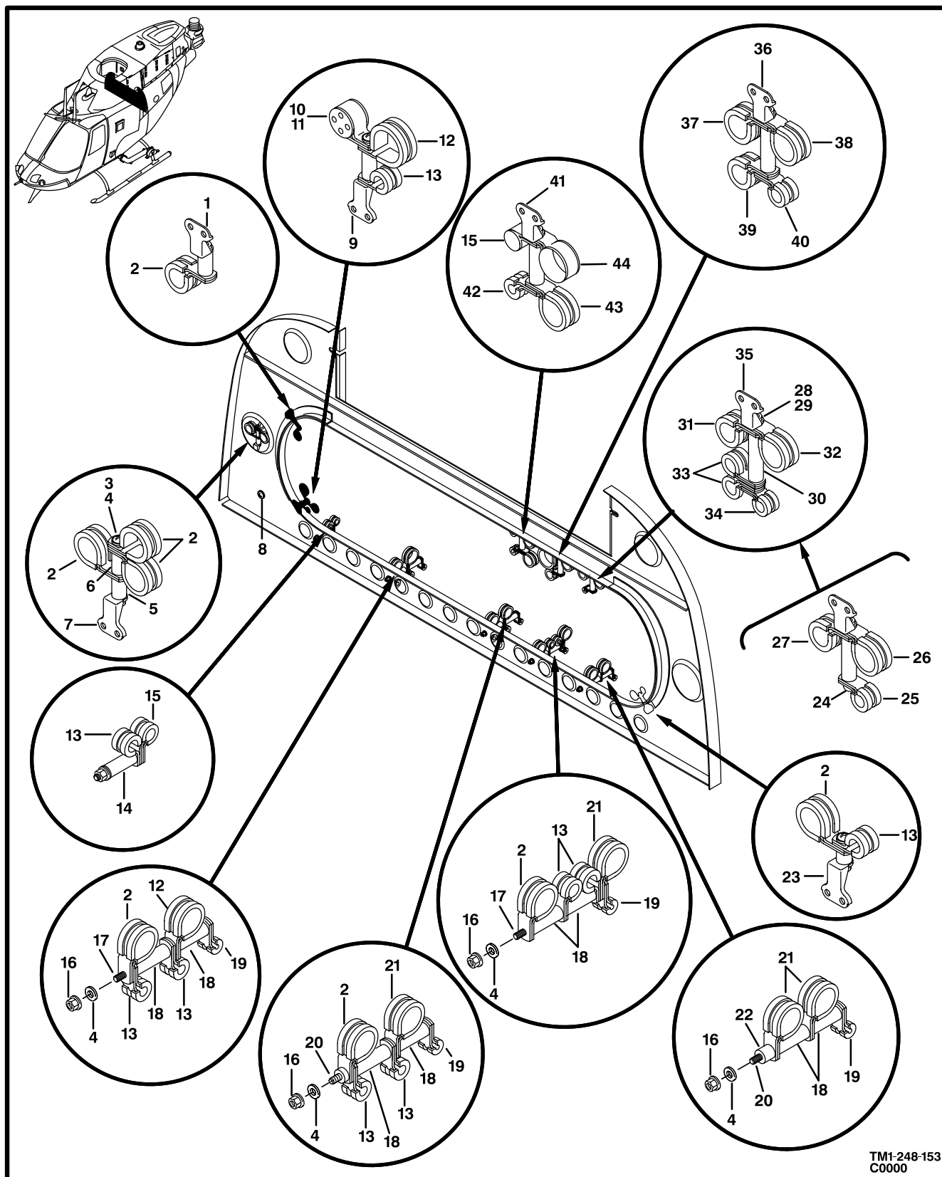
Figure 148. Electrical Installation,Bulkhead
