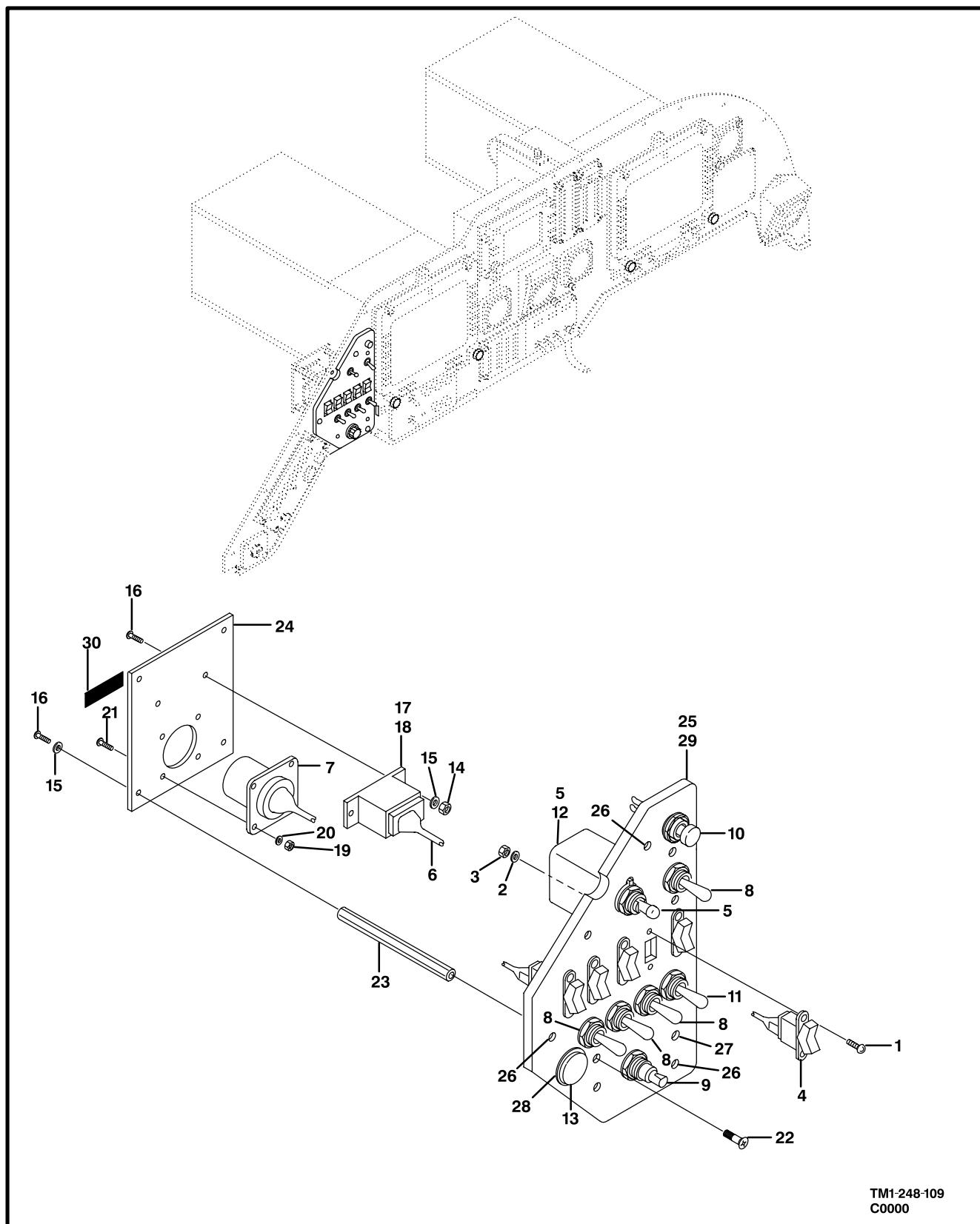
Figure 104. Panel Assembly
