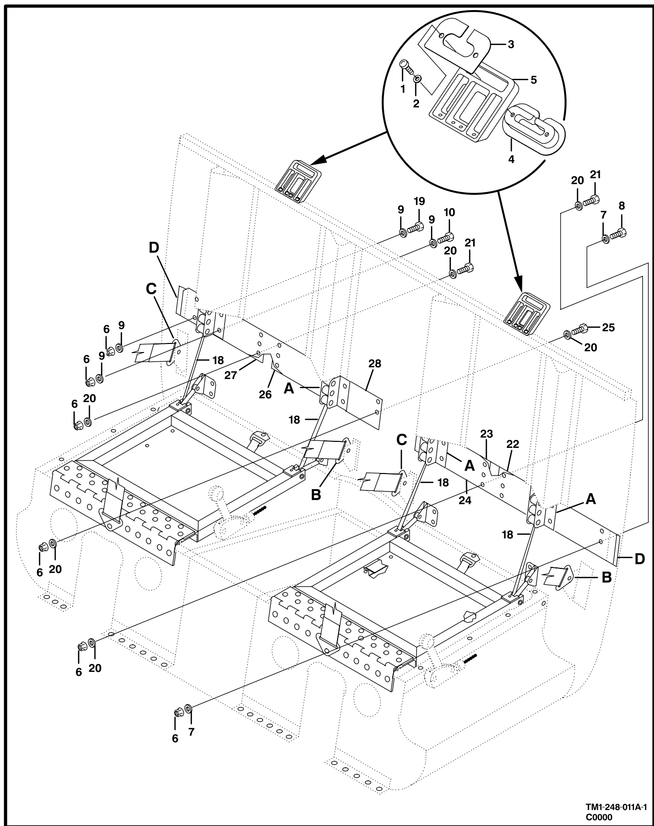
Figure 11A. CrewSeat Installation, Energy Attenuating (Sheet 1 of 2)
