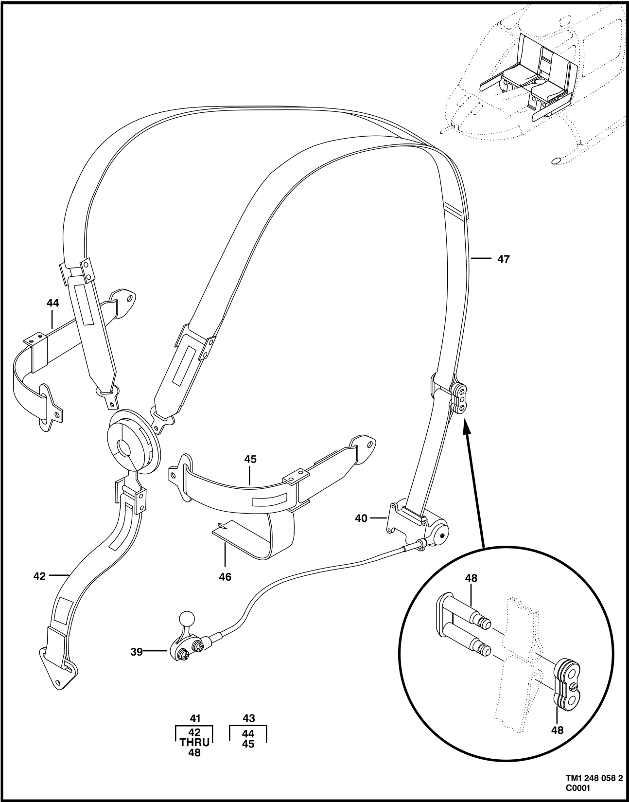
Figure 57. Seat and Restraint Assembly (Sheet 2 of 2)
