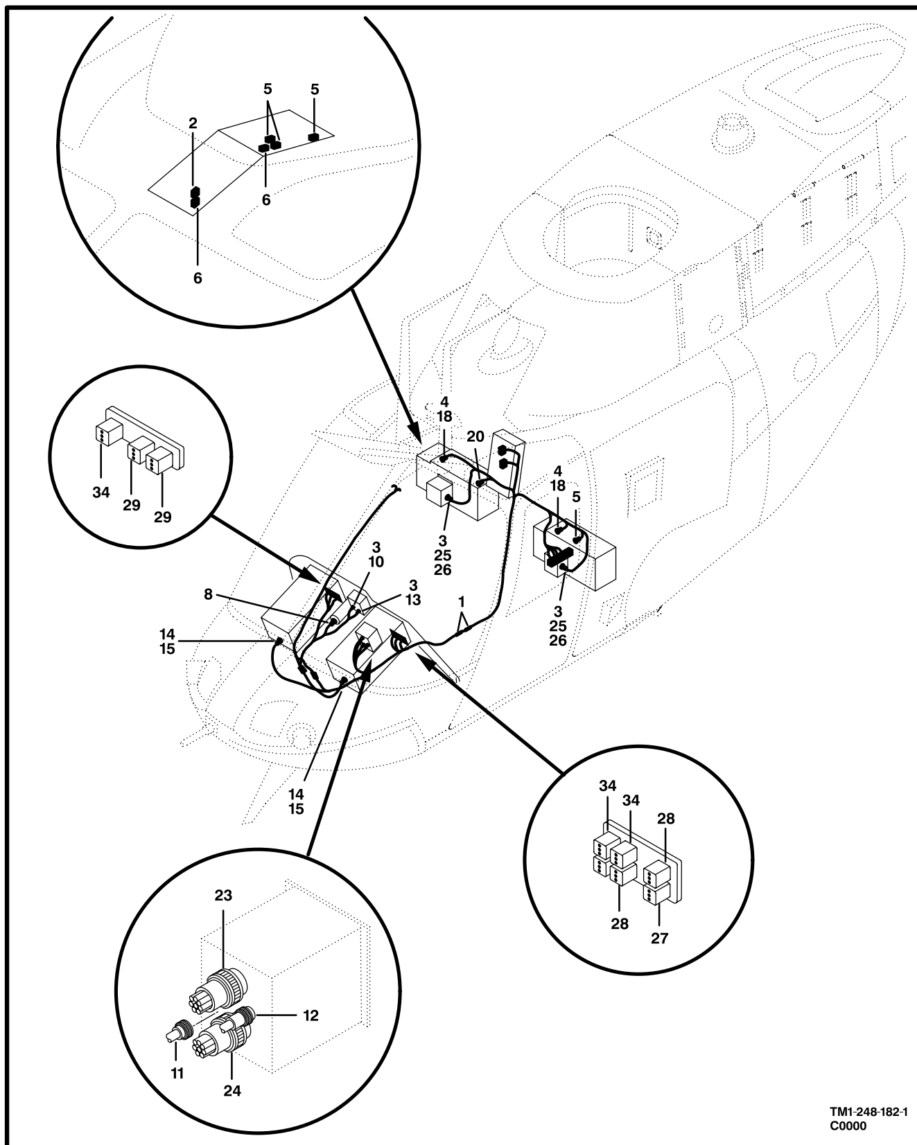
Figure 177. Cable Assembly,Control Display System (Sheet 1 of 2)
