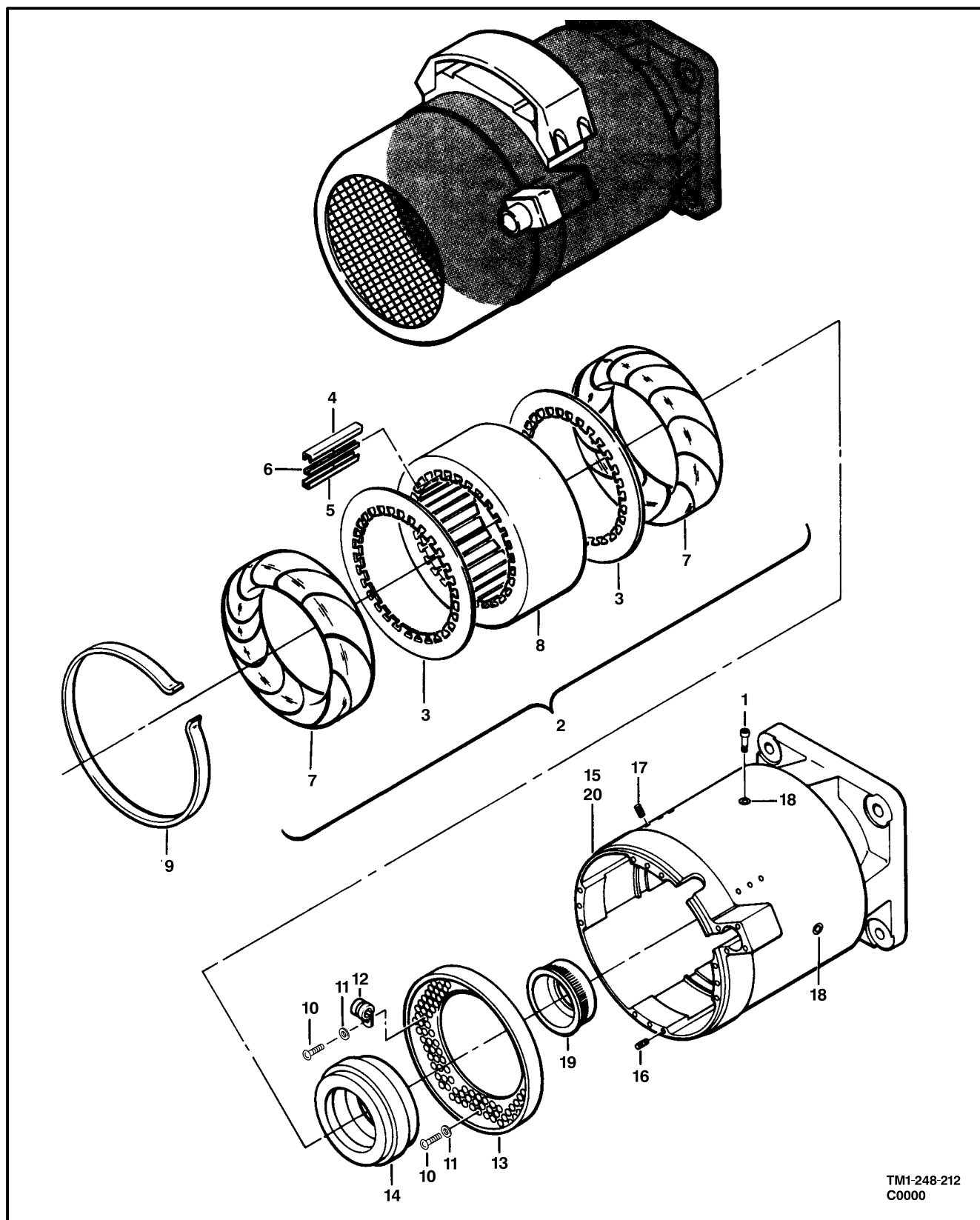
Figure 207. Housing Assembly
