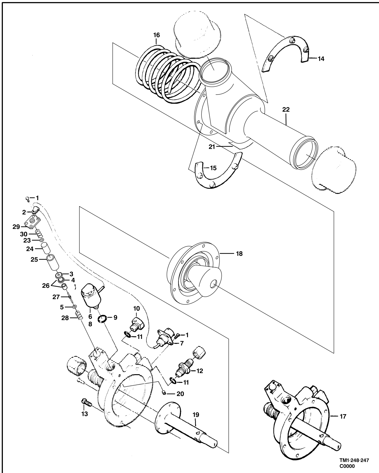
Figure 263. Mixing Valve Assembly
