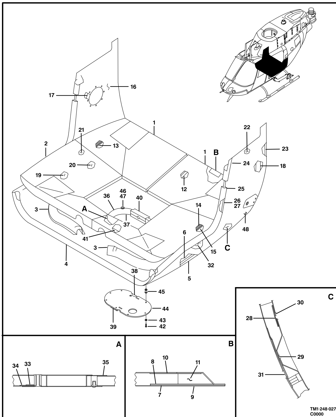
Figure 26. Support Installation, Fuel Cell
