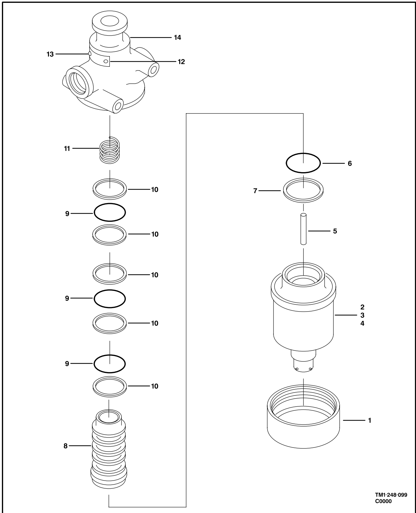
Figure 96. Valve,Solenoid
