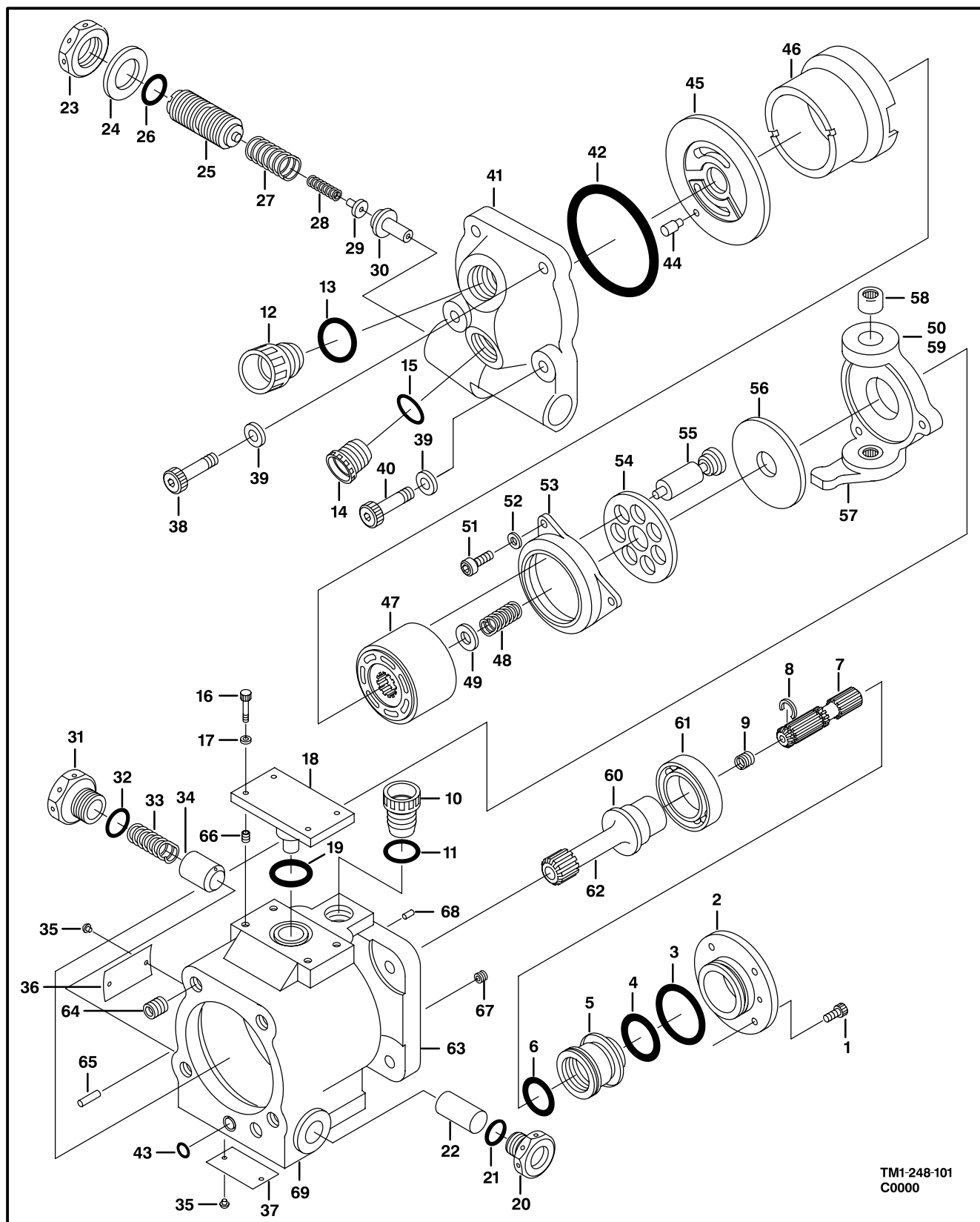
Figure 97. Pump Assembly,Hydraulic
