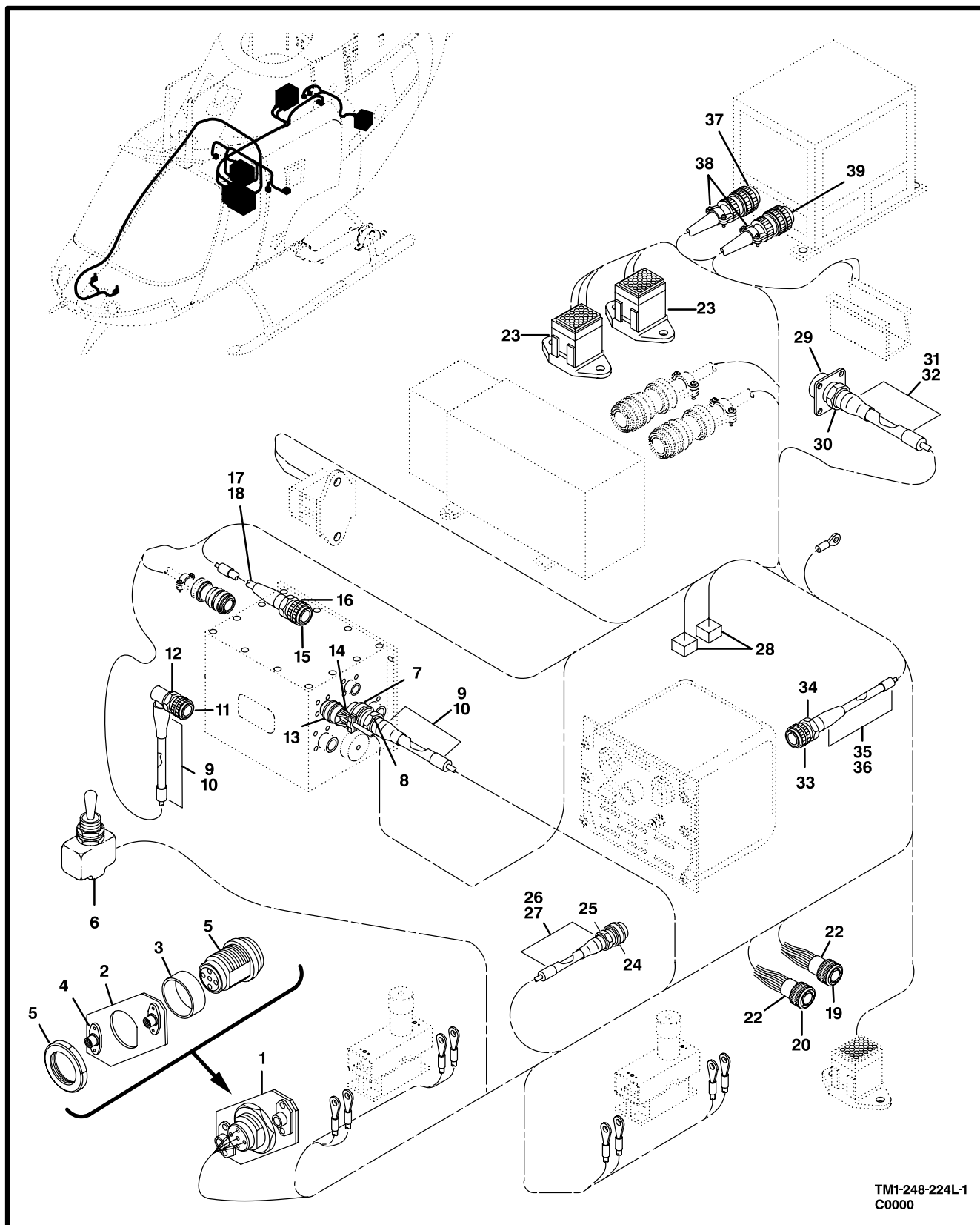
Figure 230. Cable Assembly, Intercom and ATH System (Sheet 1 of 2)
