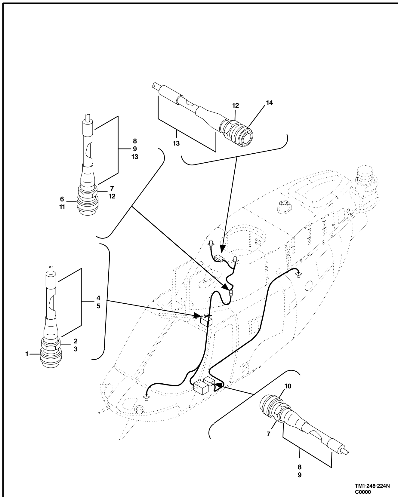
Figure 232. Cable Assembly,Radar Detector
