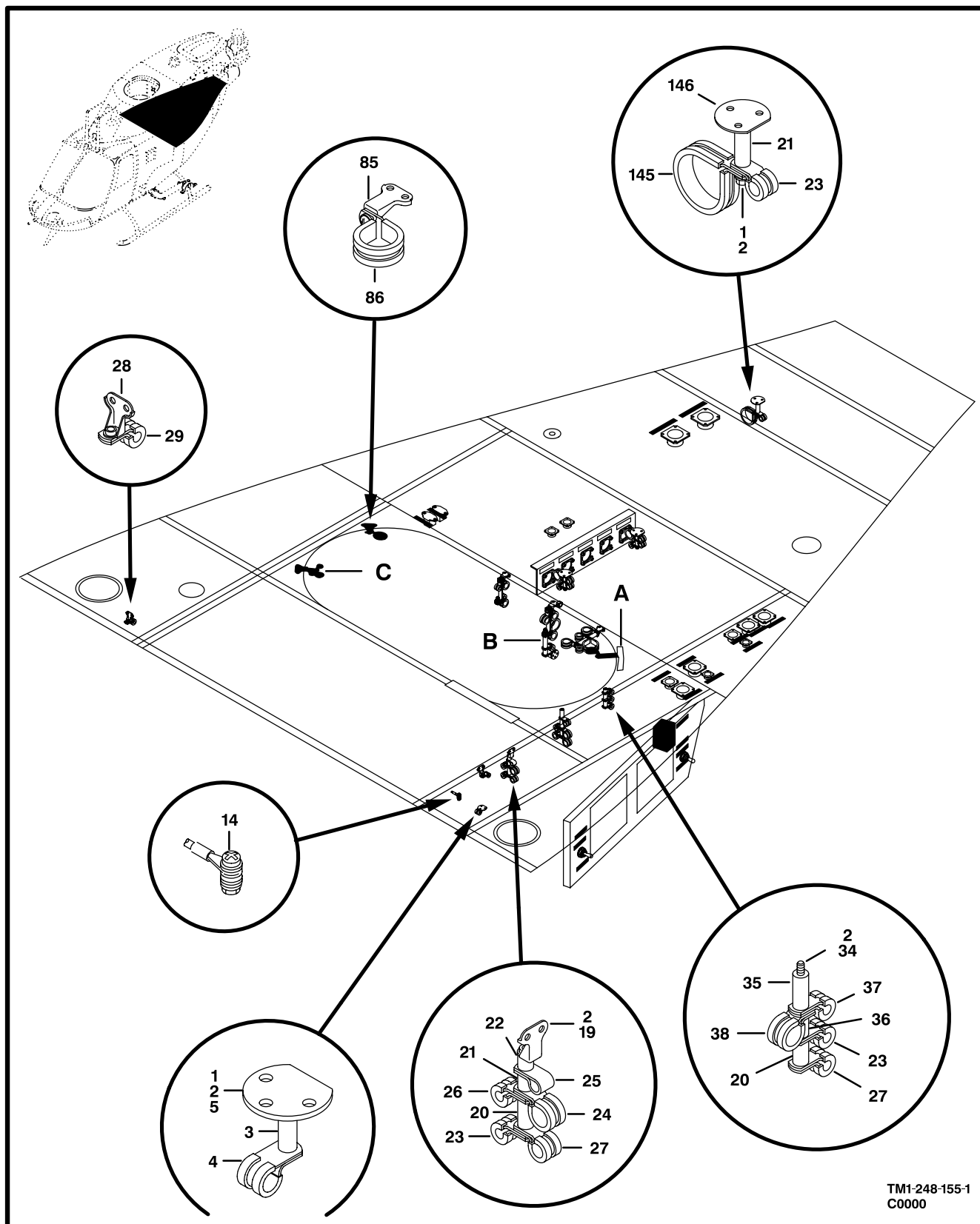
Figure 150. Electrical Installation, Canted Web (Sheet 1 of 5)
