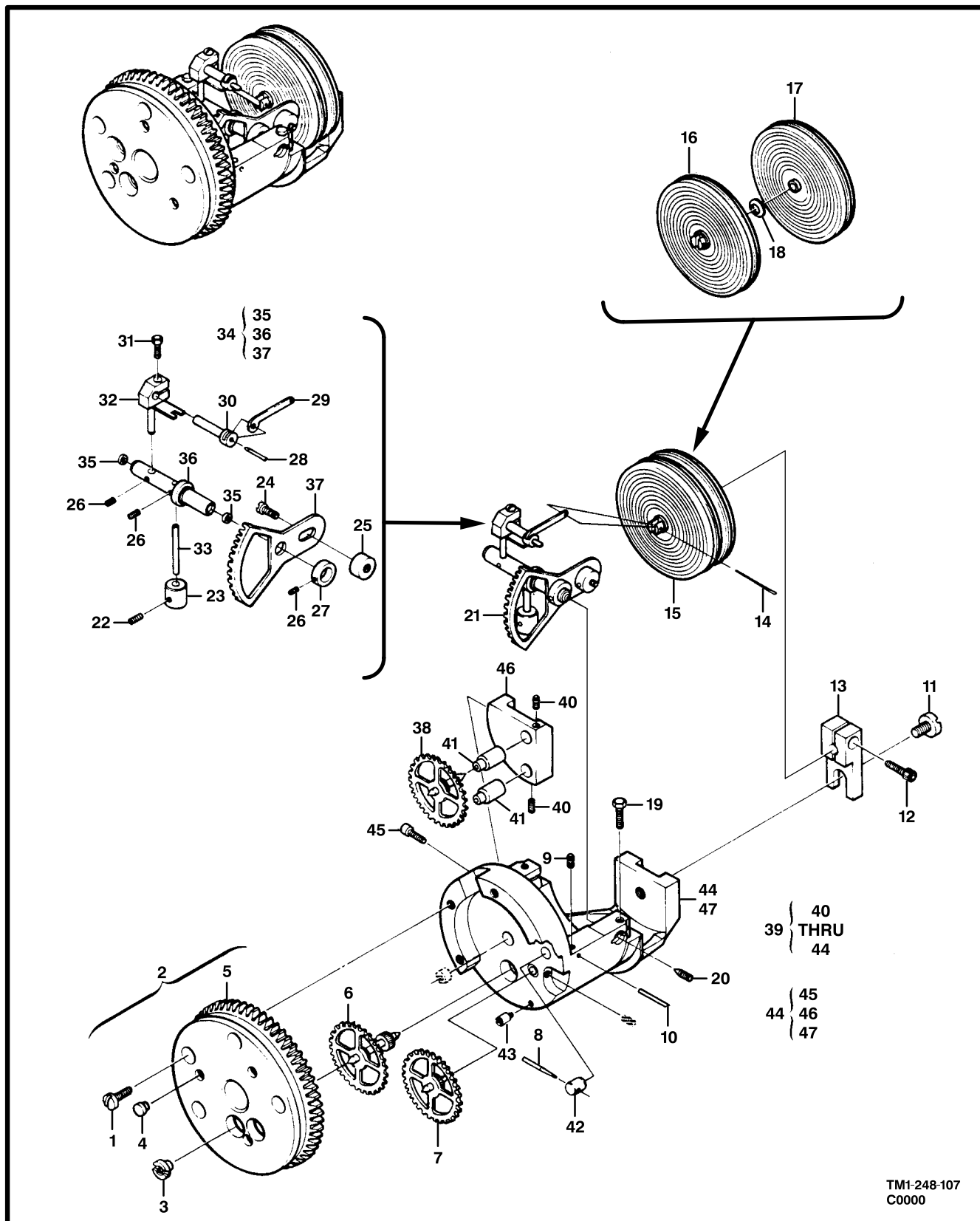
Figure 102. Mechanism Assembly, Altimeter
