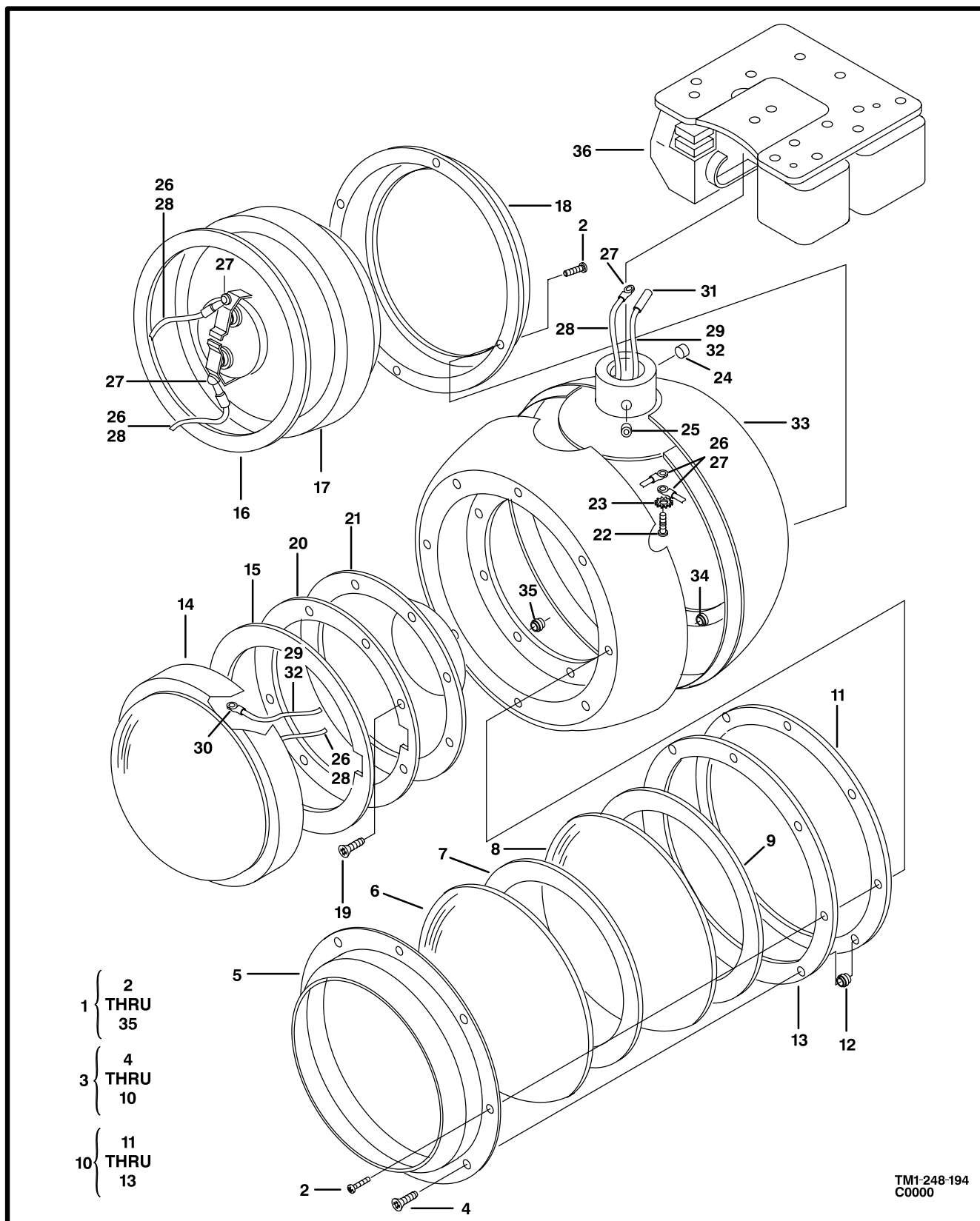
Figure 189. Searchlight,IR/White
