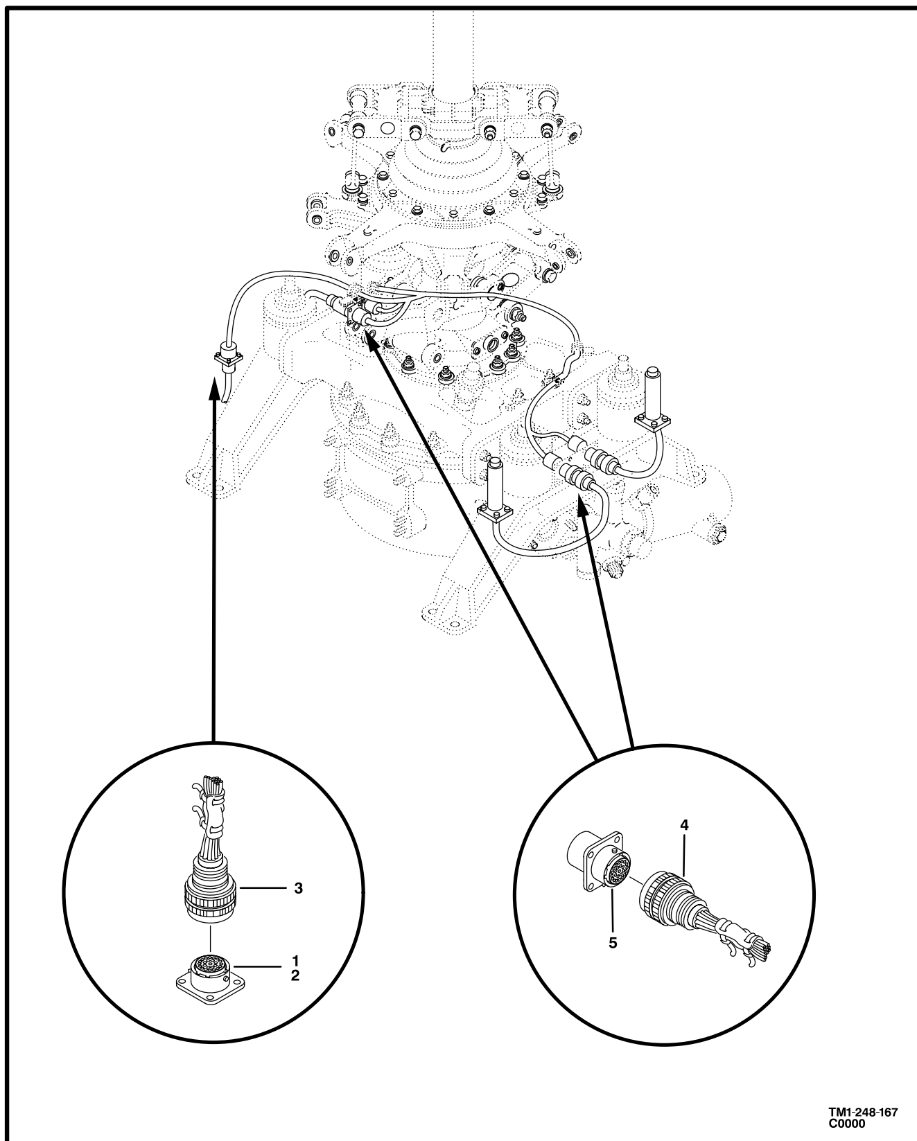
Figure 162. Electrical Installation, LVDT-TAMS
