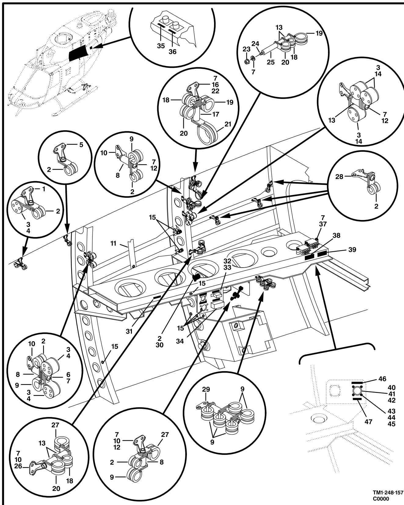
Figure 152. Electrical Installation, Canted Web (USBL EFF 95-0080 AND SUB)
