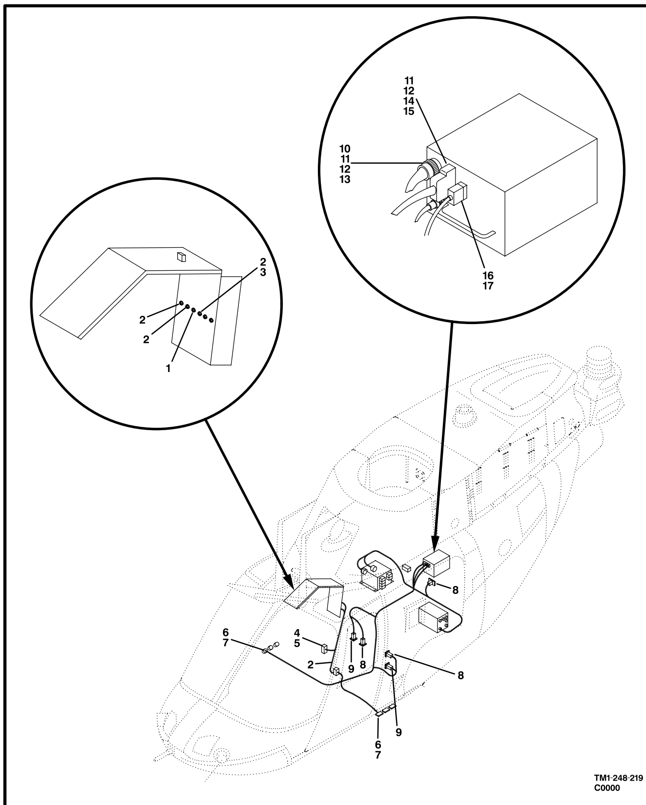
Figure 214. Cable Assembly, Hellfire
