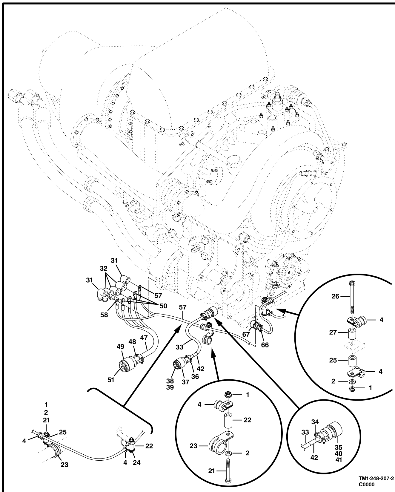
Figure 202. Electrical System, Power Plant (Sheet 2 of 3)
