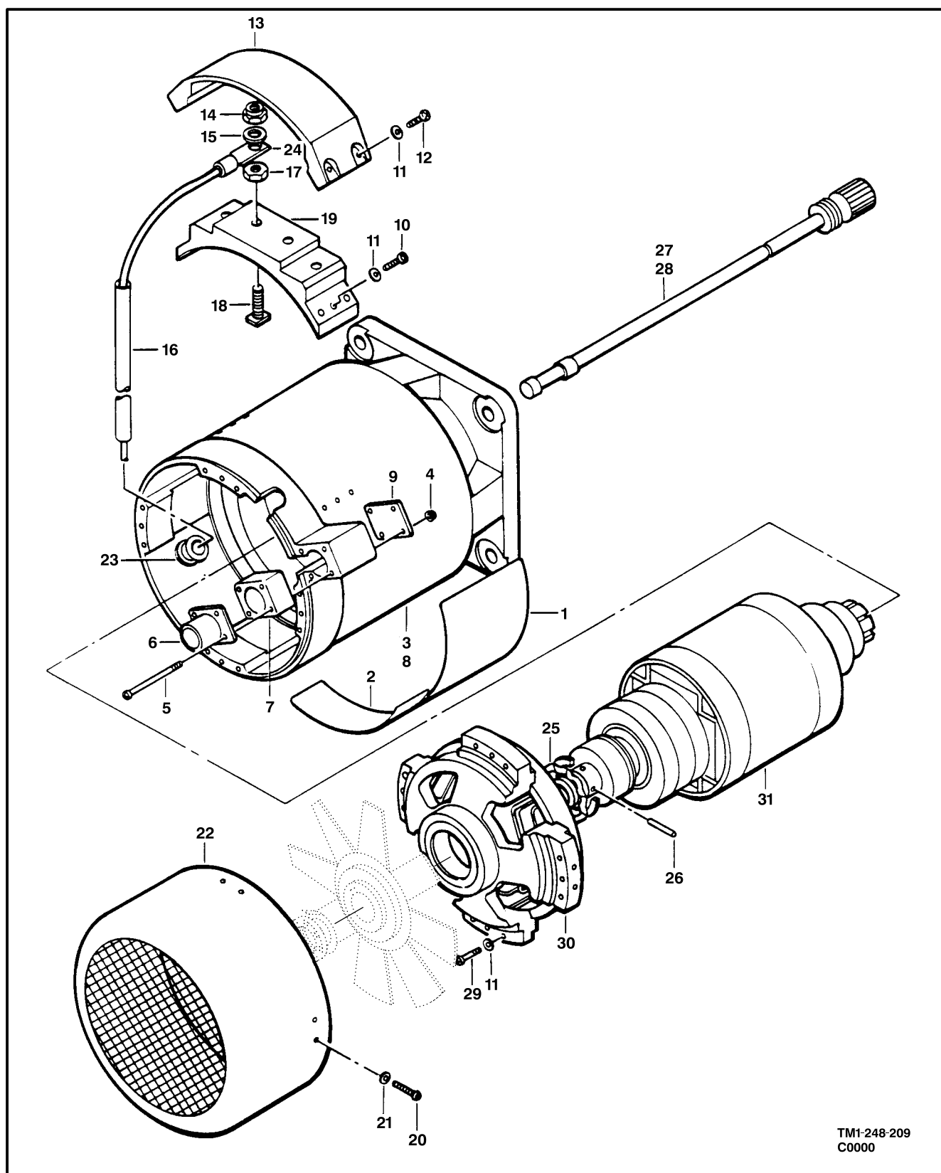
Figure 204. Generator Assembly
