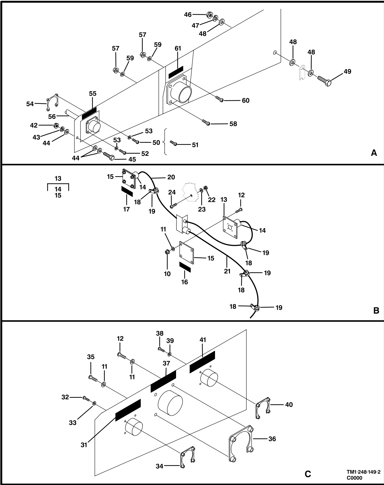
Figure 144. Electrical Installation (Sheet 2 of 2)
