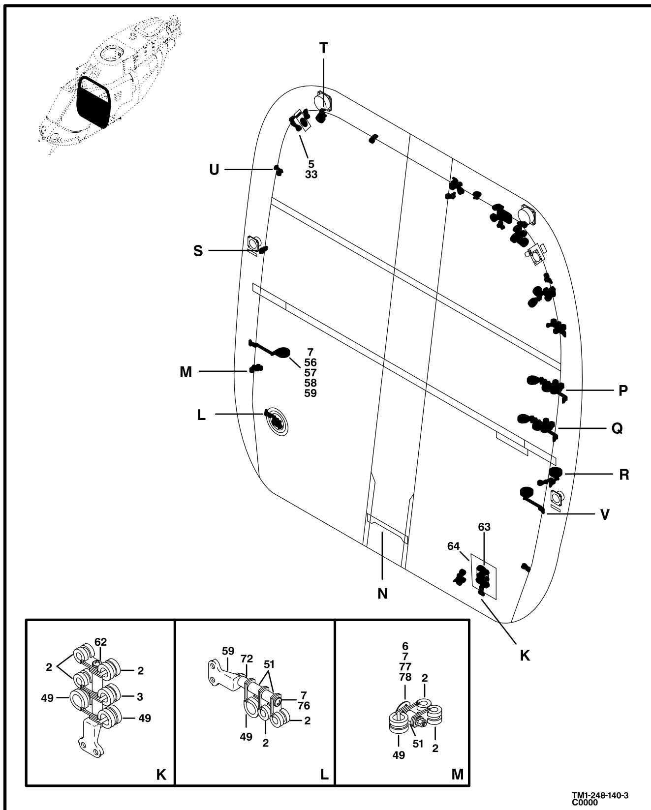
Figure 135. Electrical Installation,Bulkhead (Sheet 3 of 4)
