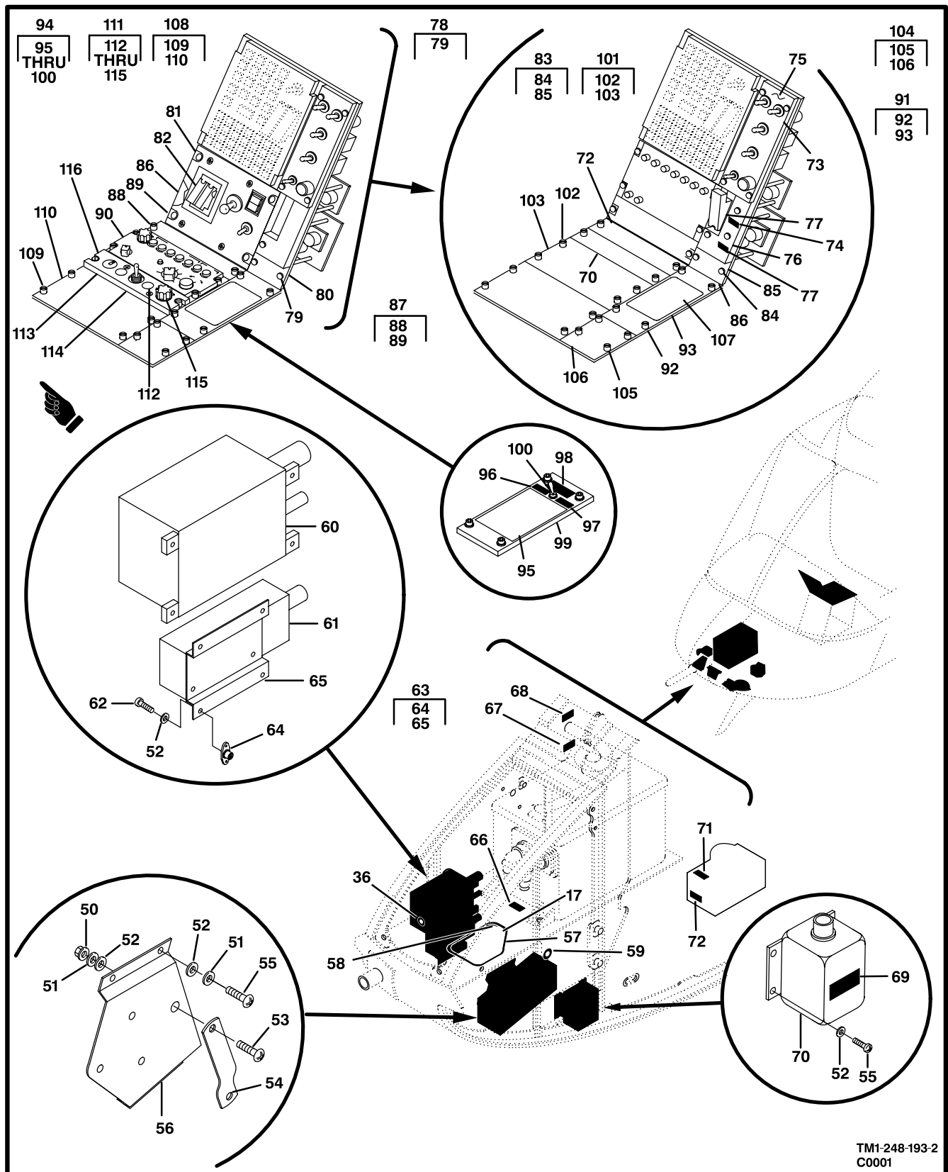
Figure 188. Electrical and Avionics Installation, Nose Compartment and Pedestal (Sheet 2 of 2)
