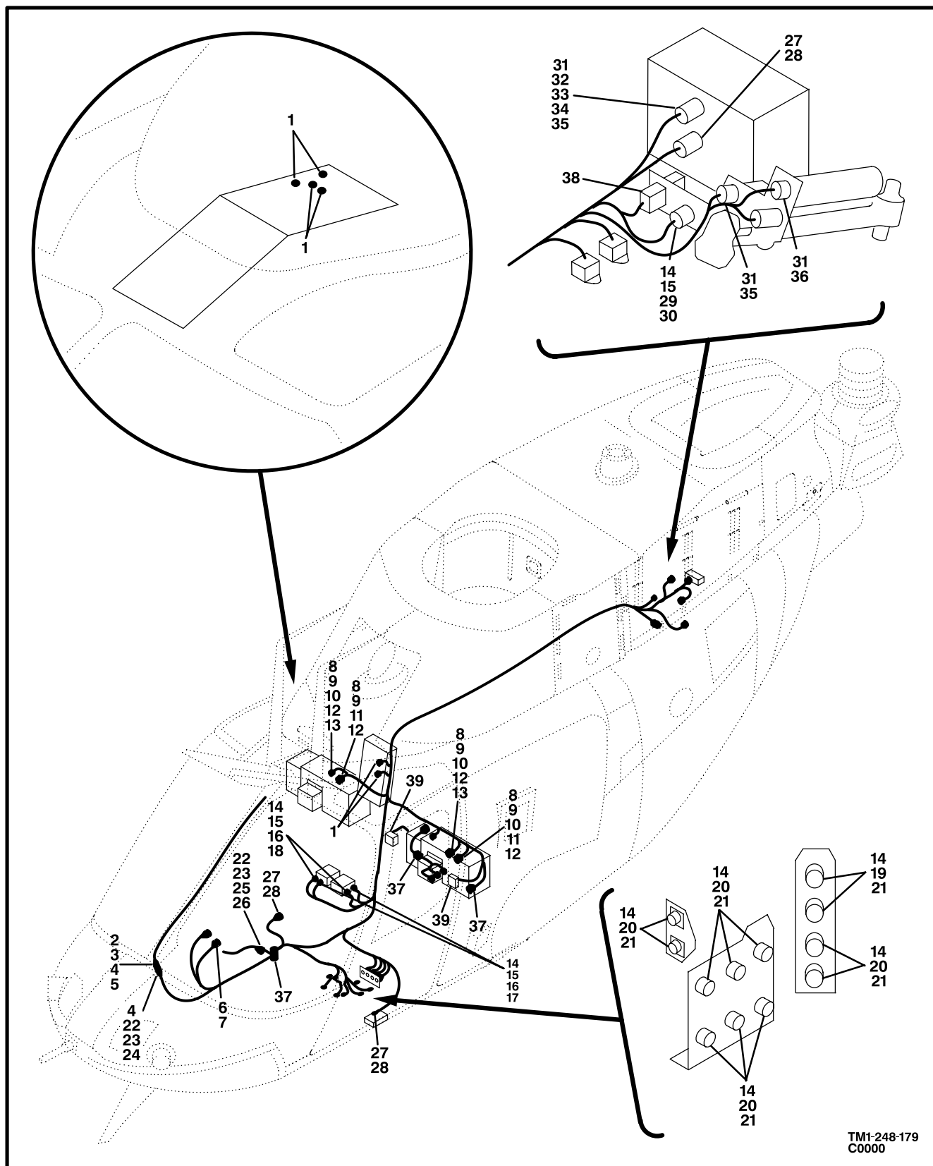
Figure 174. Cable Assembly, SCAS Hydraulic System
