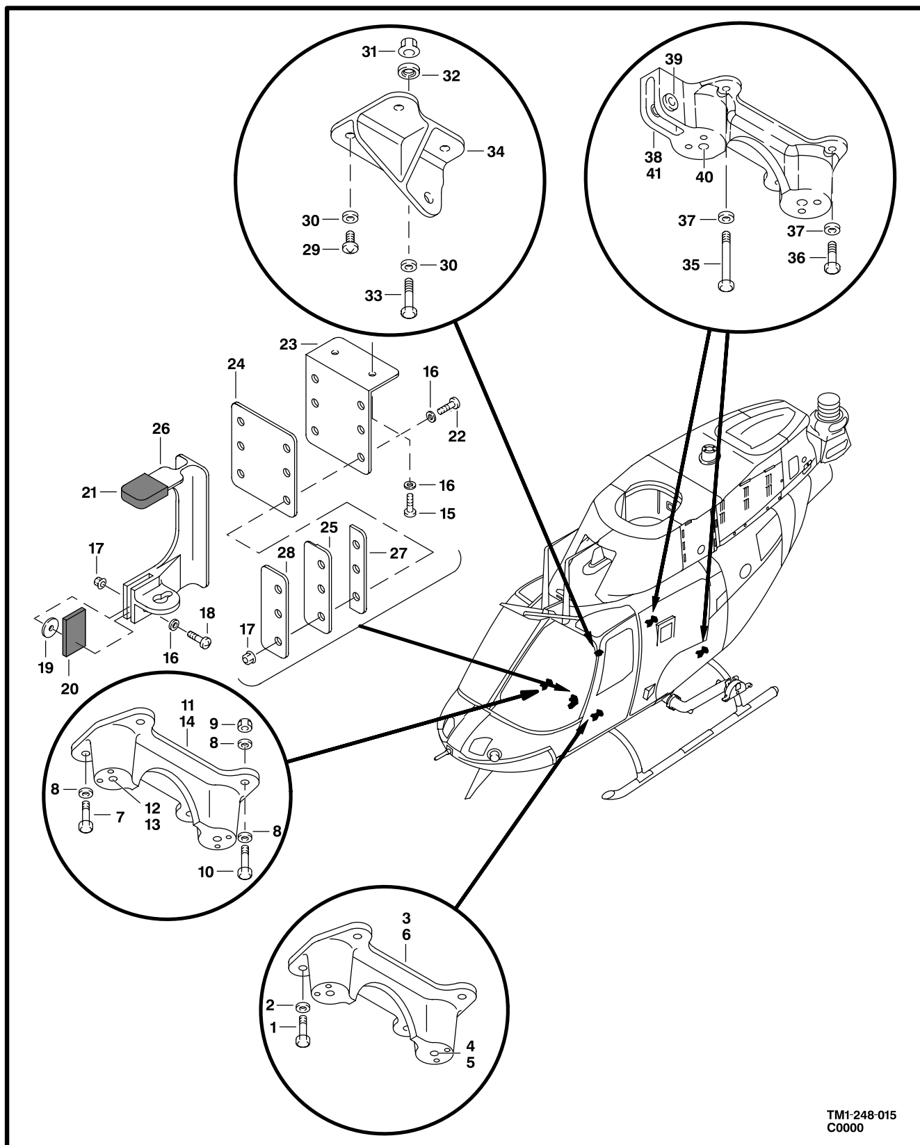
Figure 15. MOD-Support Installation,FWD,LH,Landing Gear
