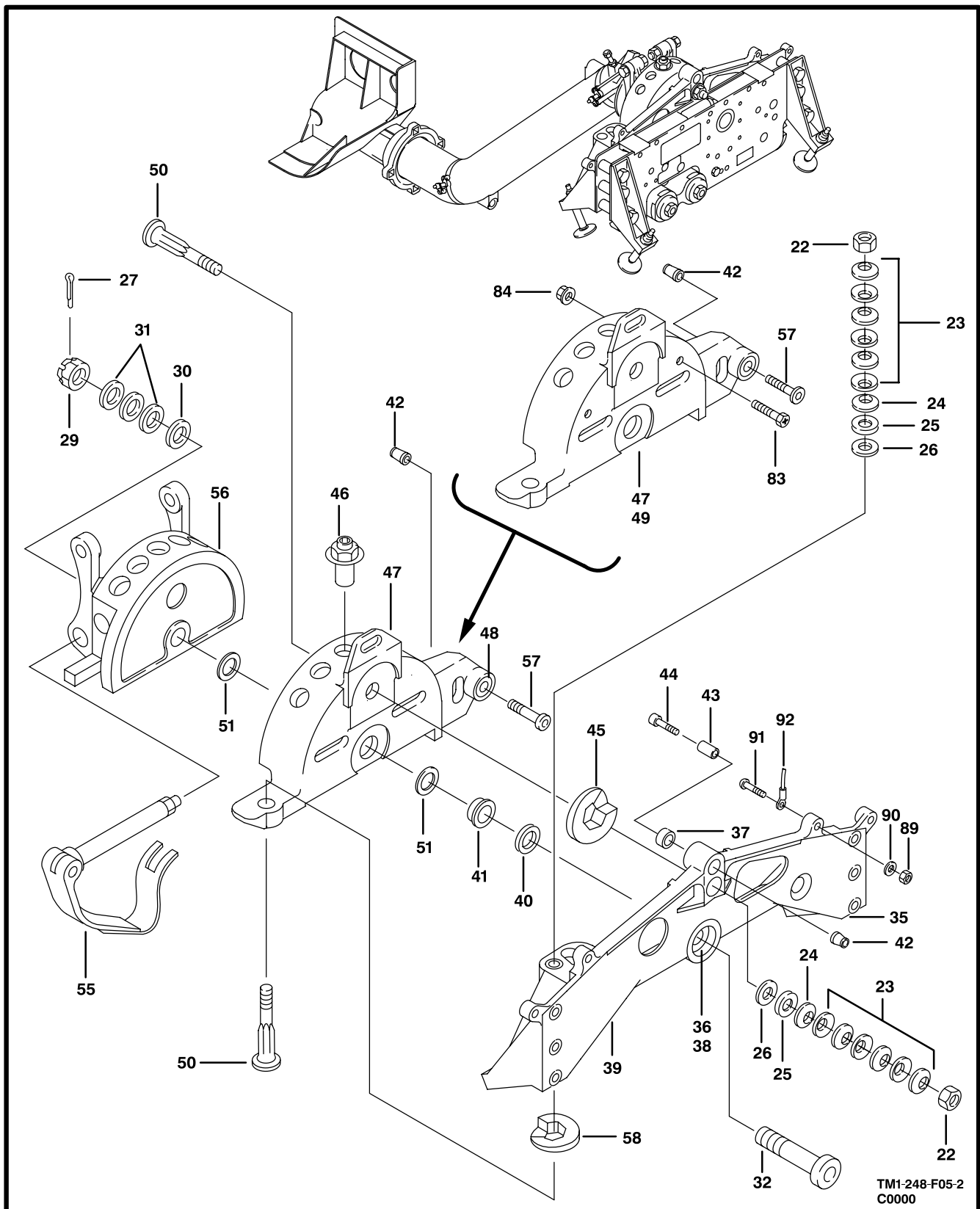
Figure F5. Universal Pylon Installation (Sheet 2 of 4)
