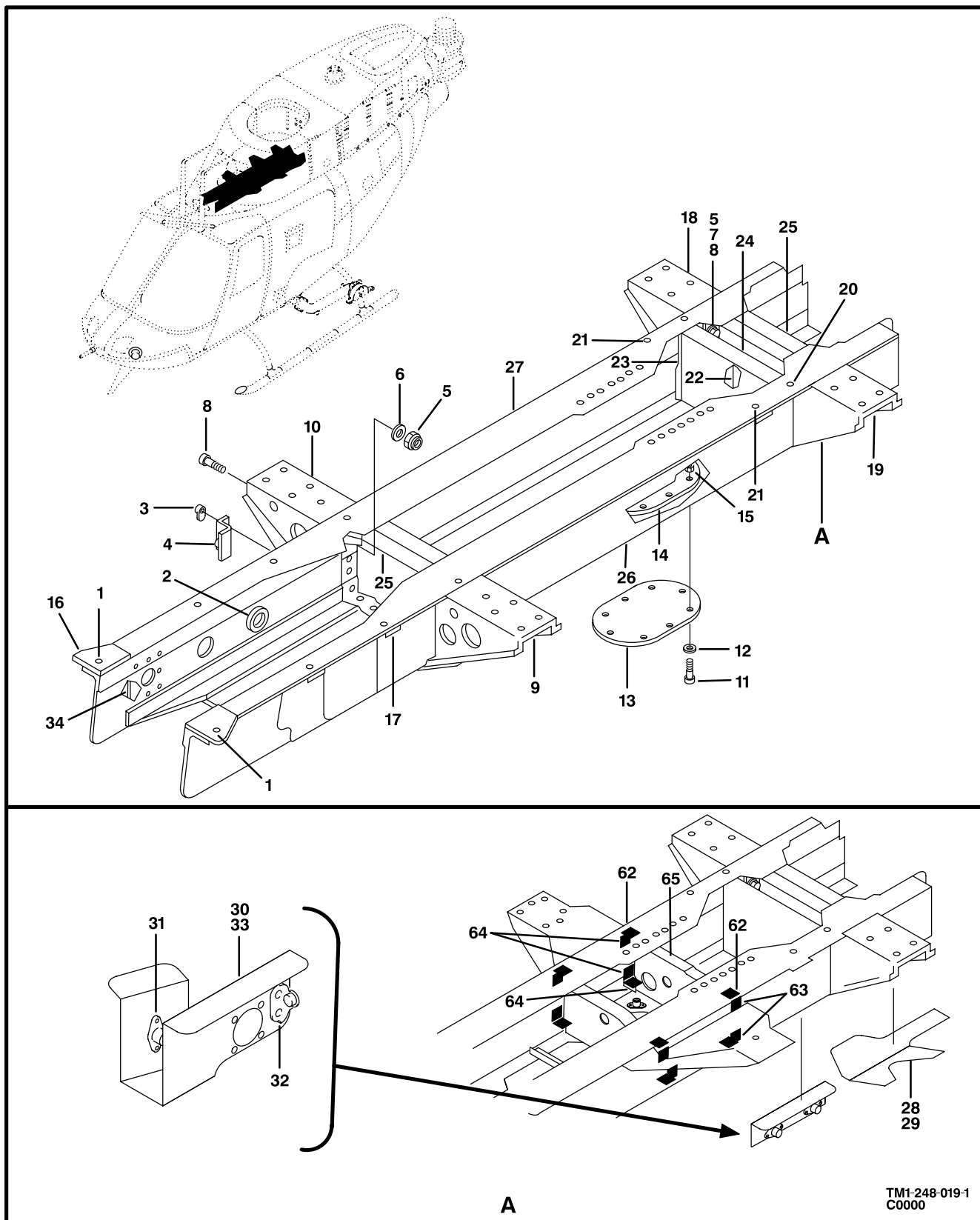
Figure 19. Beam Installation,Upper,Cabin Roof (Sheet 1 of 2)
