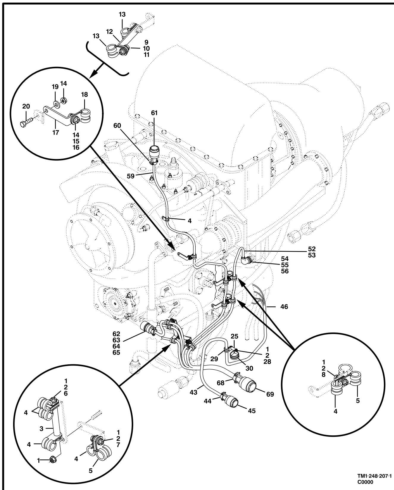
Figure 202. Electrical System, Power Plant (Sheet 1 of 3)
