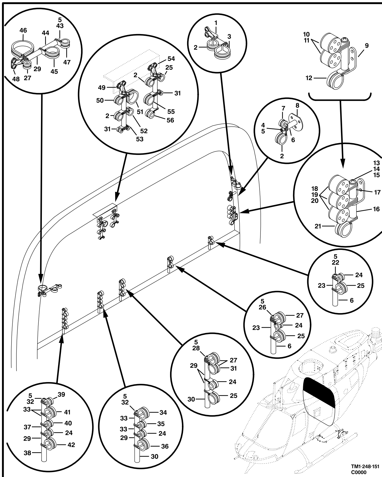
Figure 146. Electrical Installation, Bulkhead
