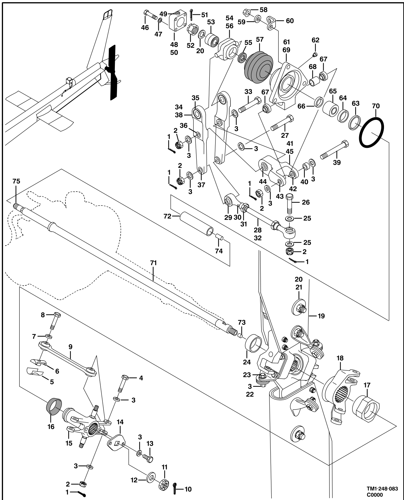
Figure 82. Tail Rotor Installation
