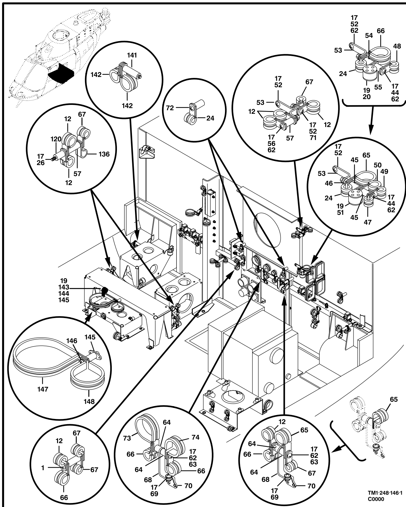
Figure 141. Electrical Installation,Bulkhead (Sheet 1 of 4)
