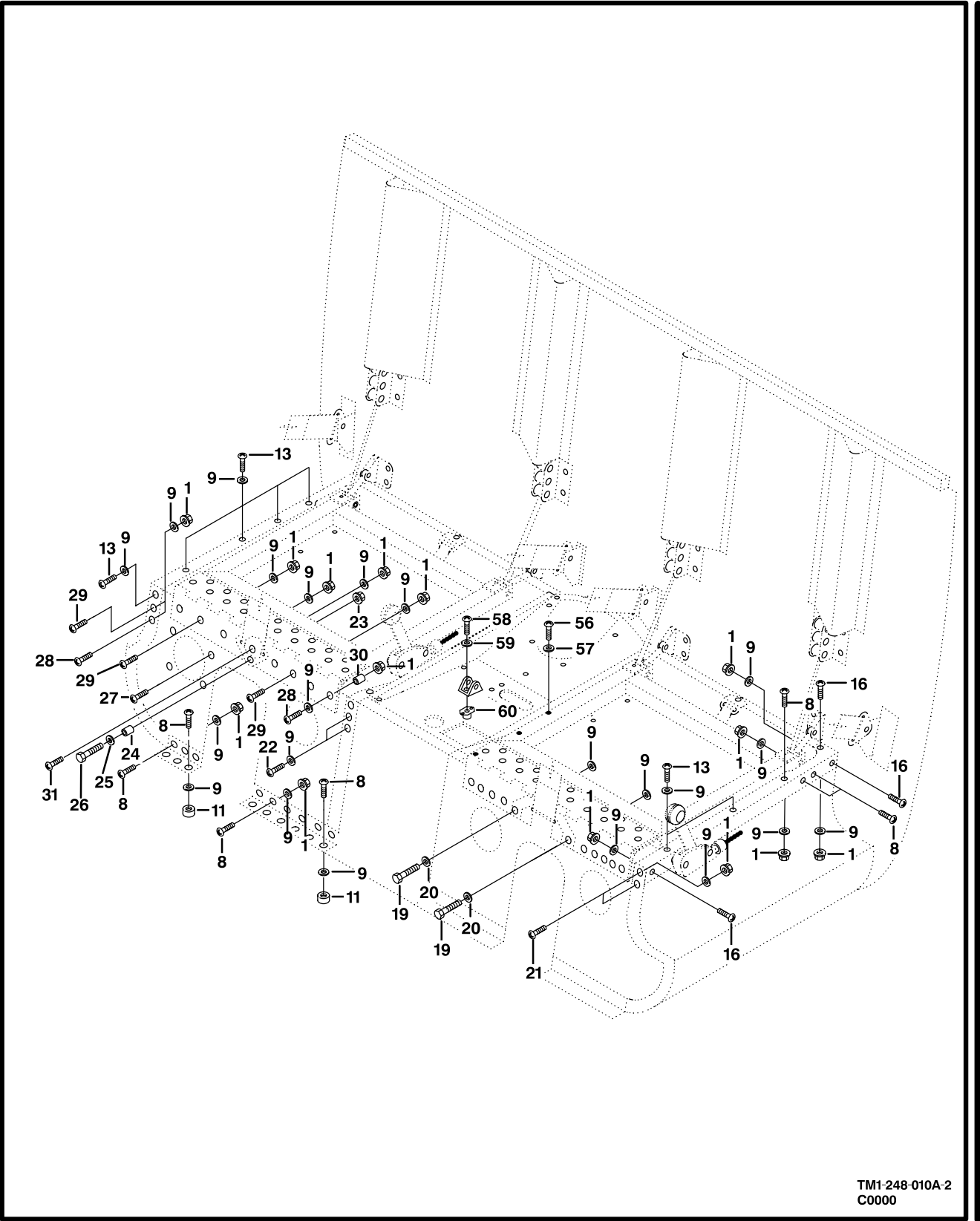
Figure 10A. Crewseat Installation, Energy Attenuating (Sheet 2 of 3)
