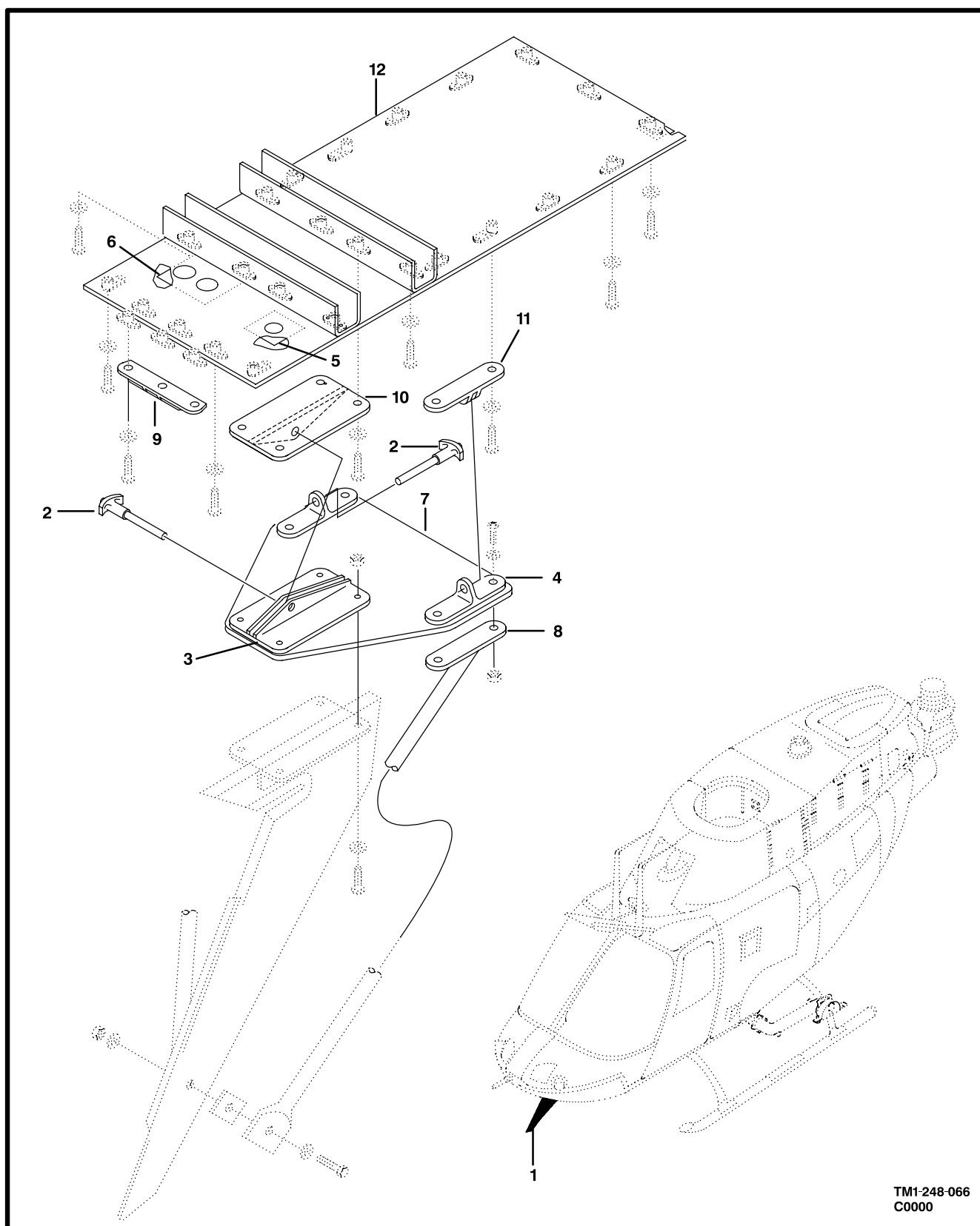
Figure 65. MOD-Wire Cutter
