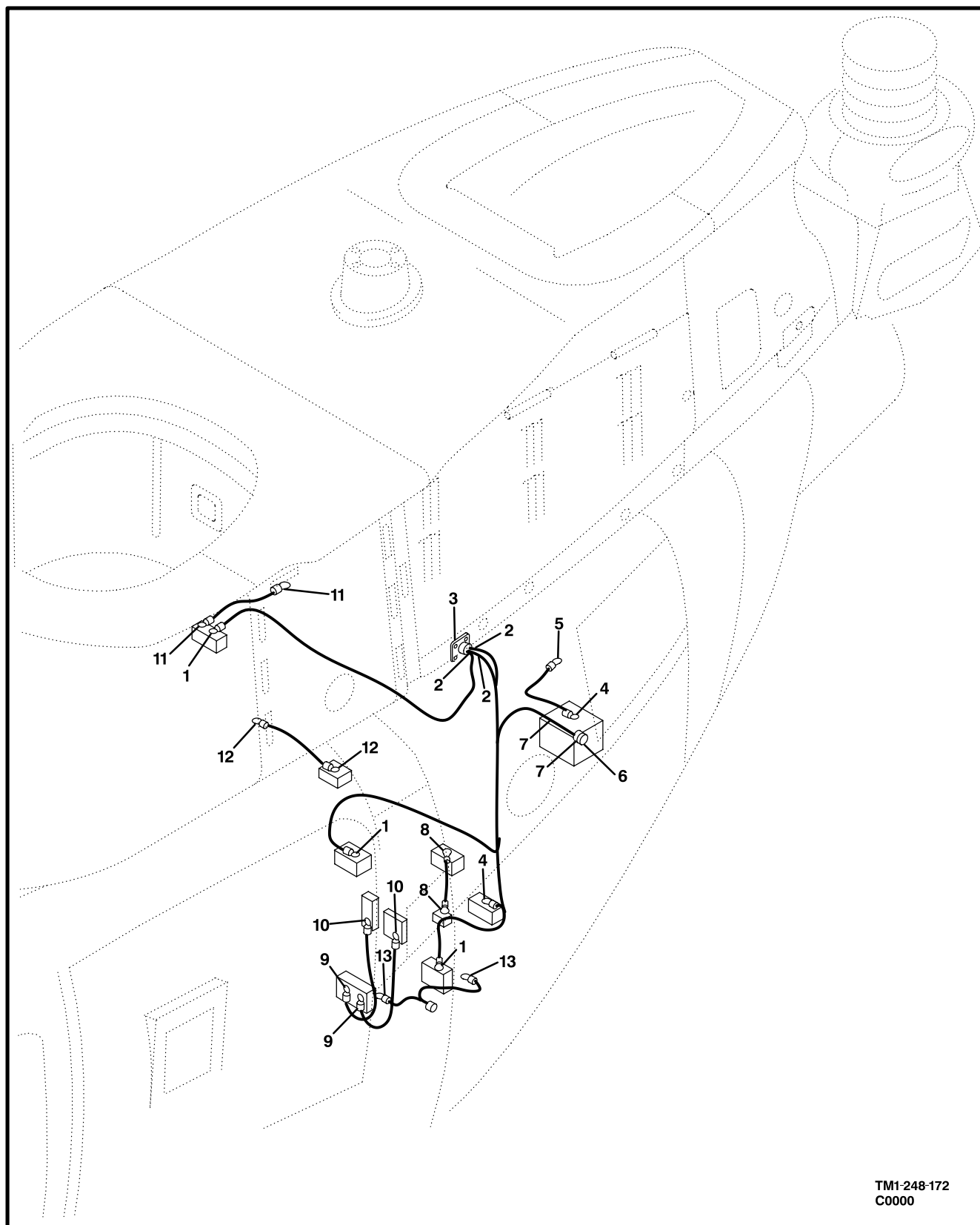
Figure 167. Cable Assembly,DC Power System
