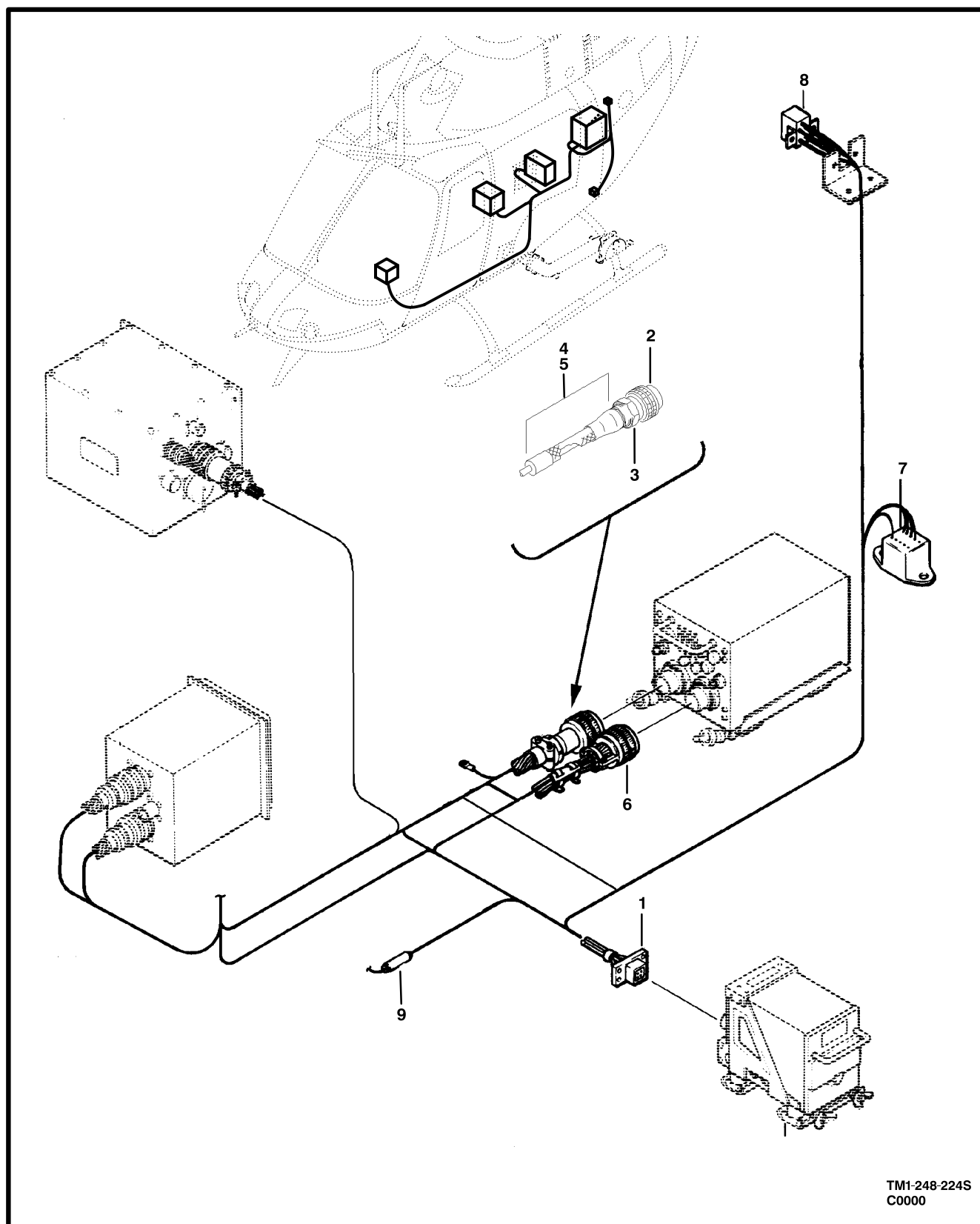
Figure 236. Cable Assembly,IFF System
