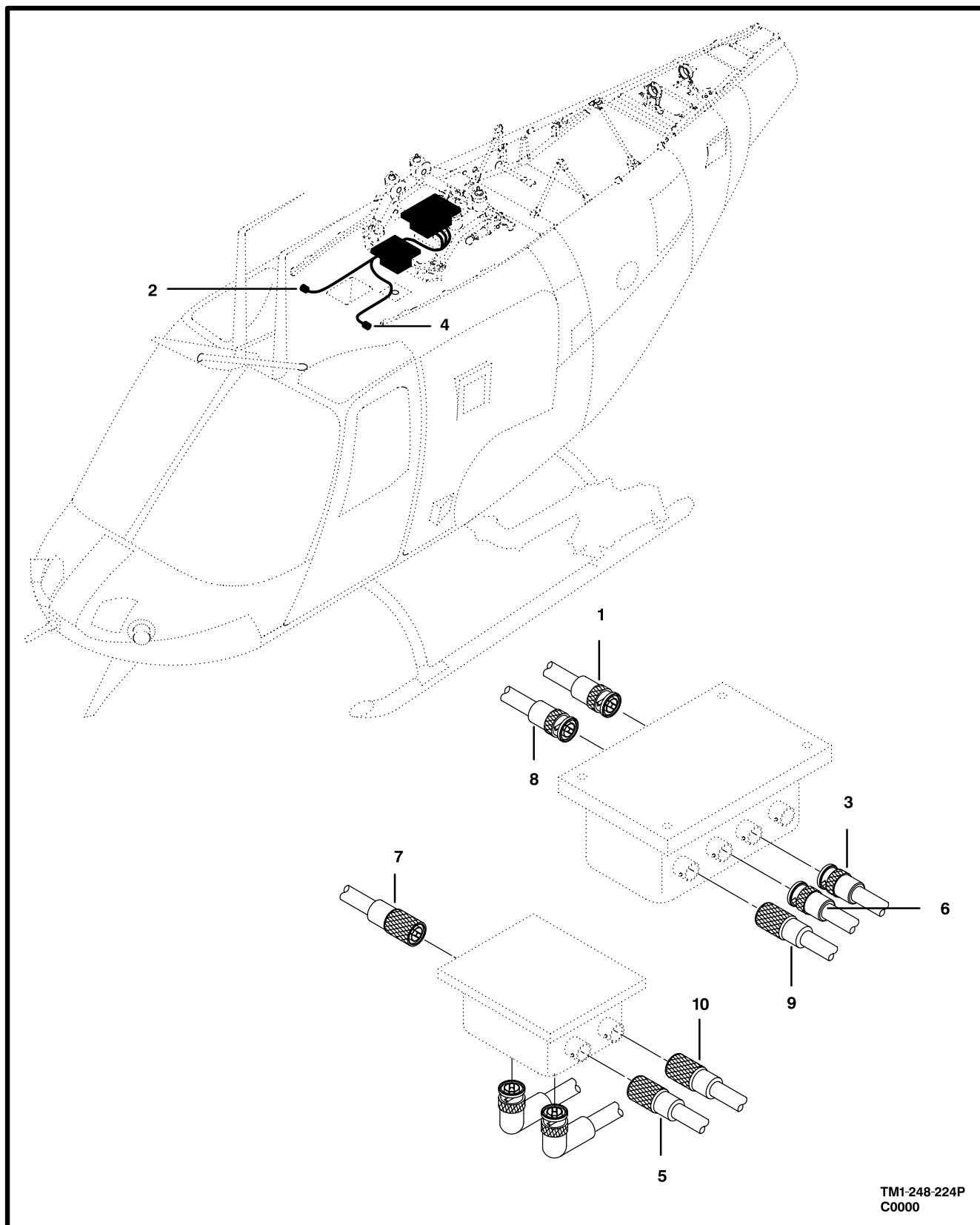
Figure 233. Cable Assembly, No. 2 VHF-FM Communication System
