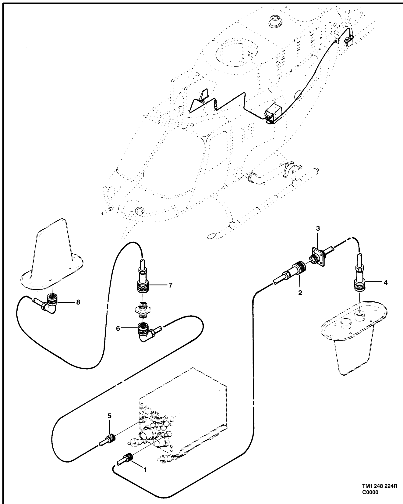
Figure 235. Cable Assembly,IFF System
