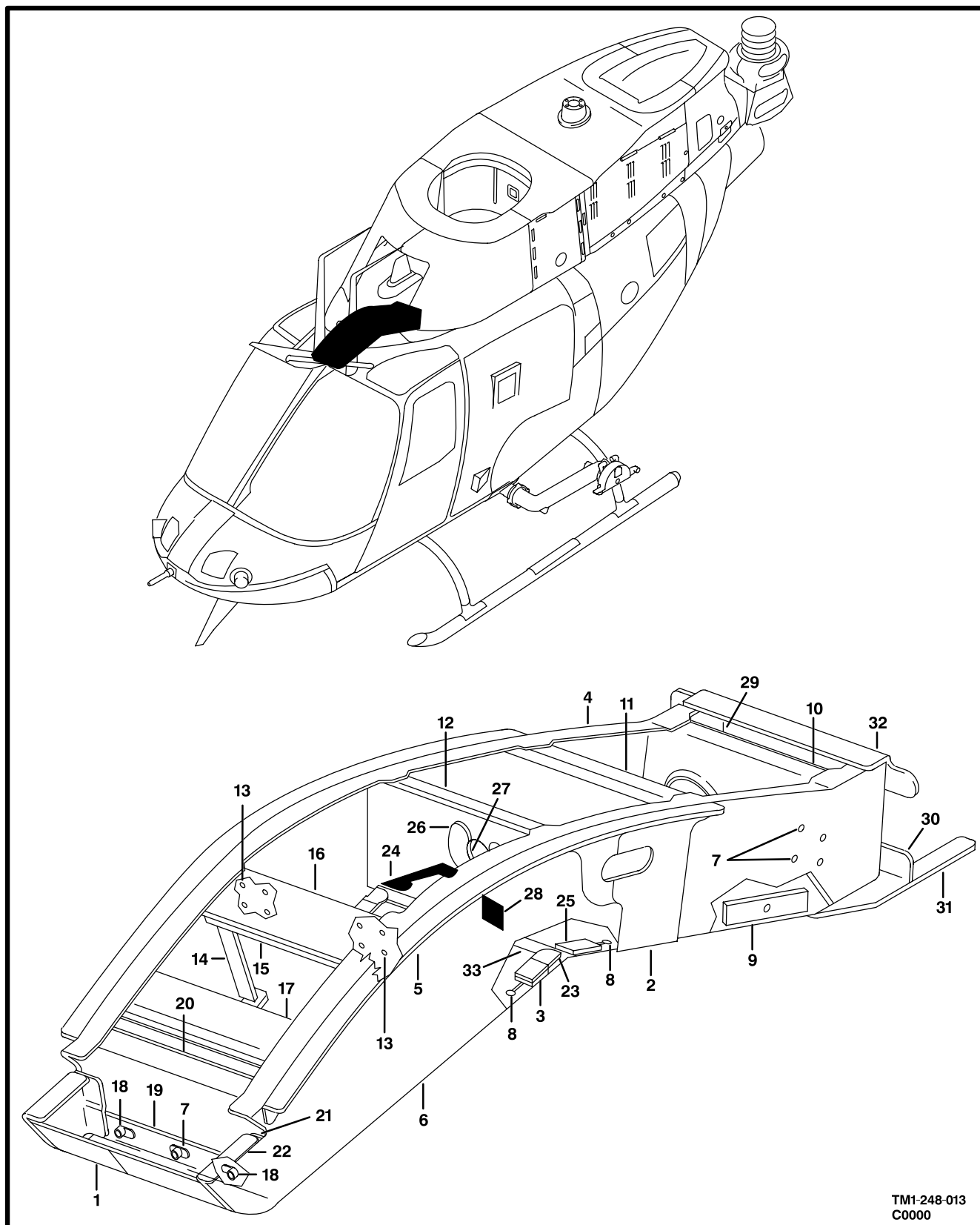
Figure 13. Console Installation, Overhead
