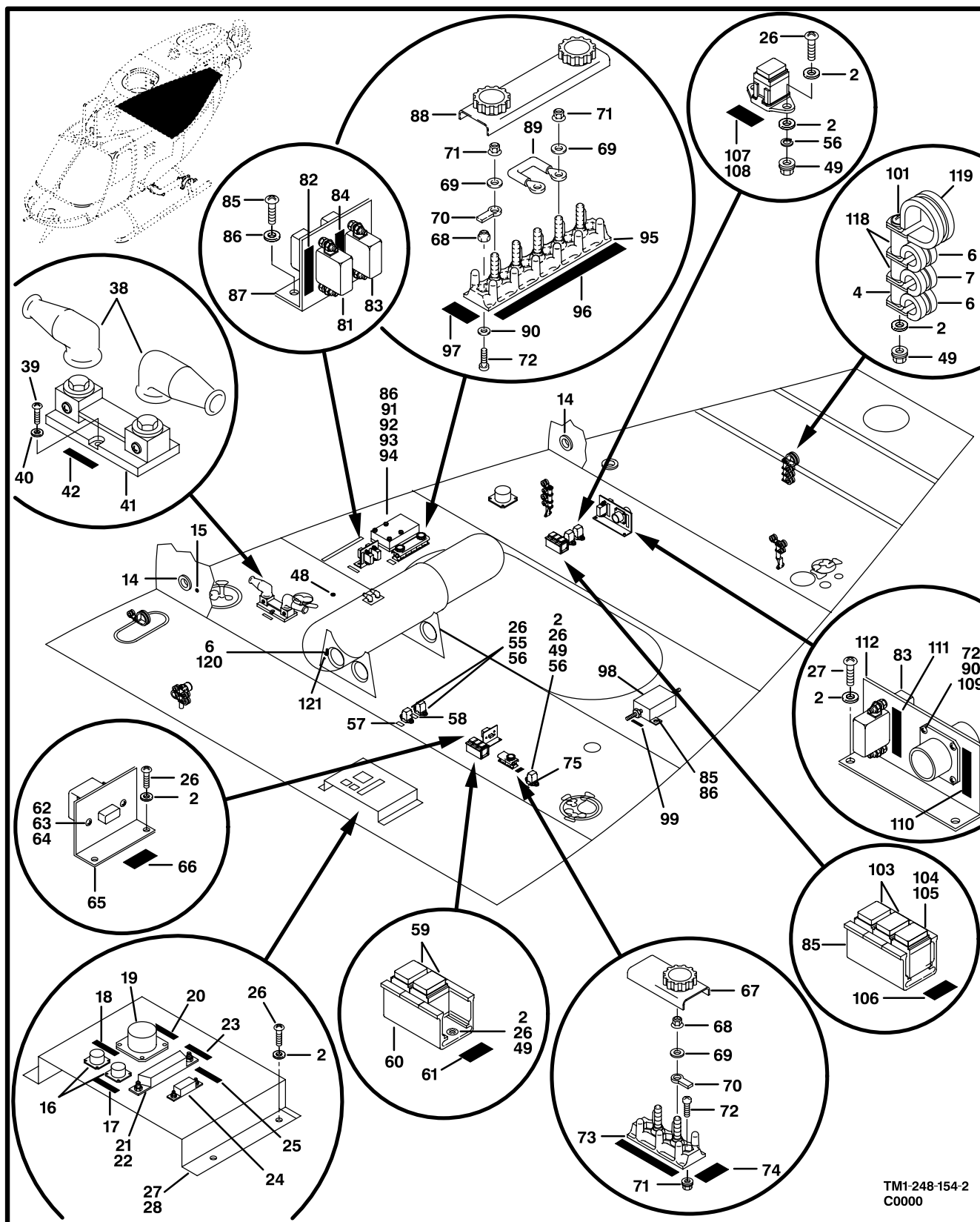
Figure 149. Electrical Installation, Canted Web (Sheet 2 of 2)
