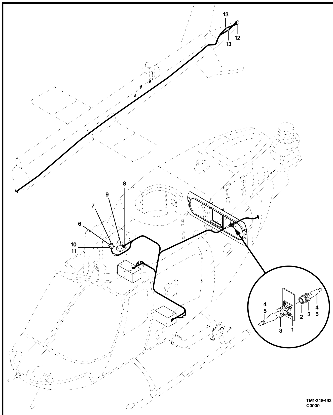
Figure 187. Cable Assembly,SCAS And Hydtaulic System
