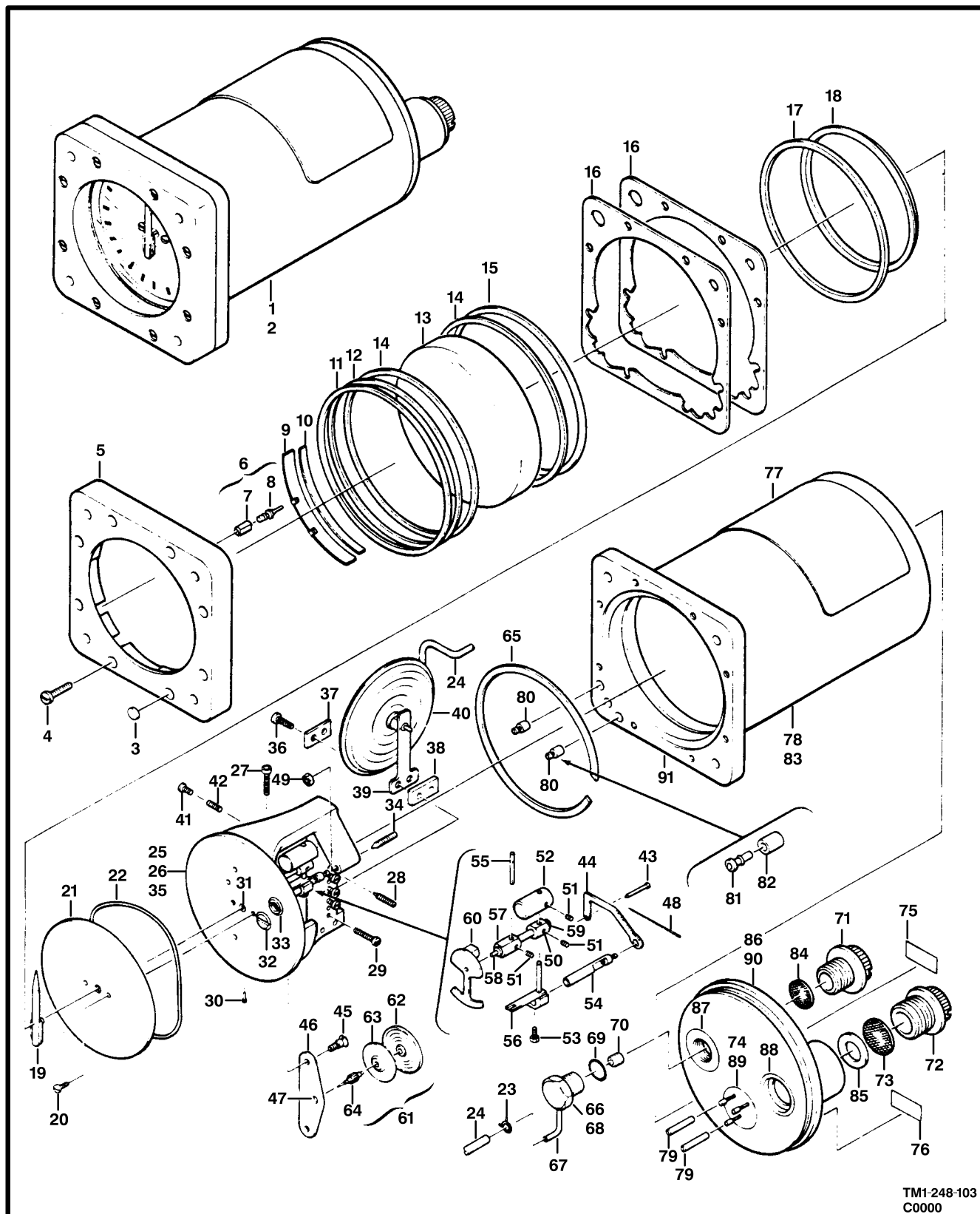
Figure 99. Indicator,Airspeed
