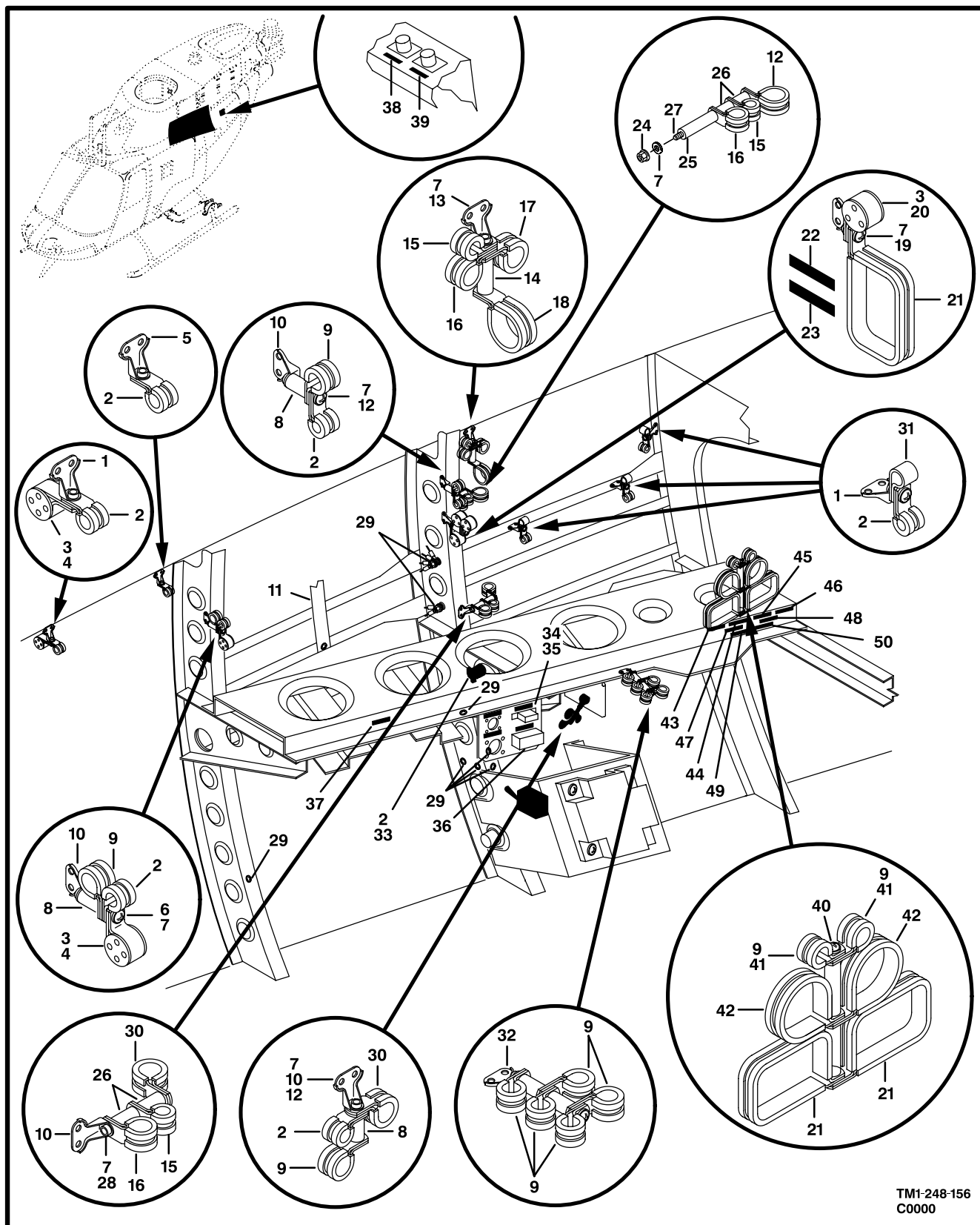
Figure 151. Electrical Installation, Canted Web (USBL EFF 89-0112 THRU 95-0079)
