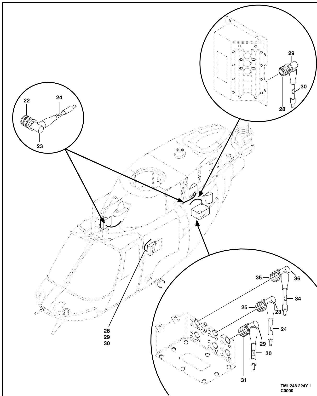
Figure 242. Cable Assembly, Laser and Radar Warning System (Sheet 1 of 2)
