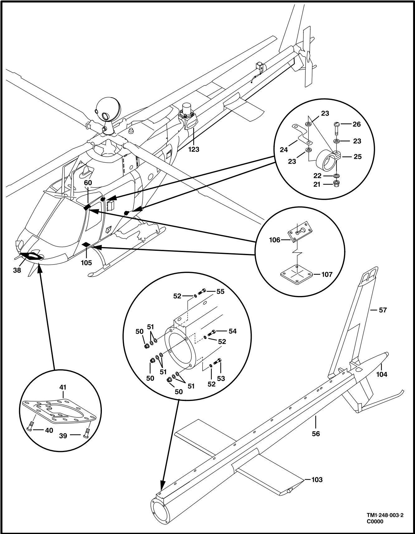
Figure 3. Fuselage Assembly (Sheet 2 of 4)
