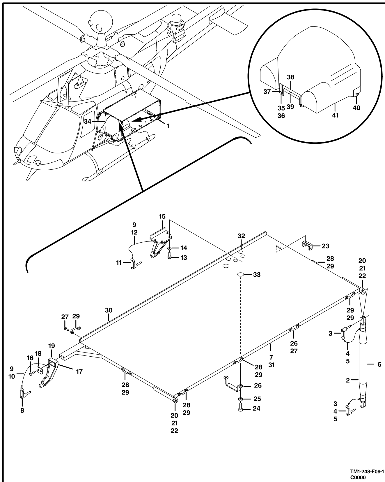
Figure F9. Aux Equipment Kit (Sheet 1 of 2)
