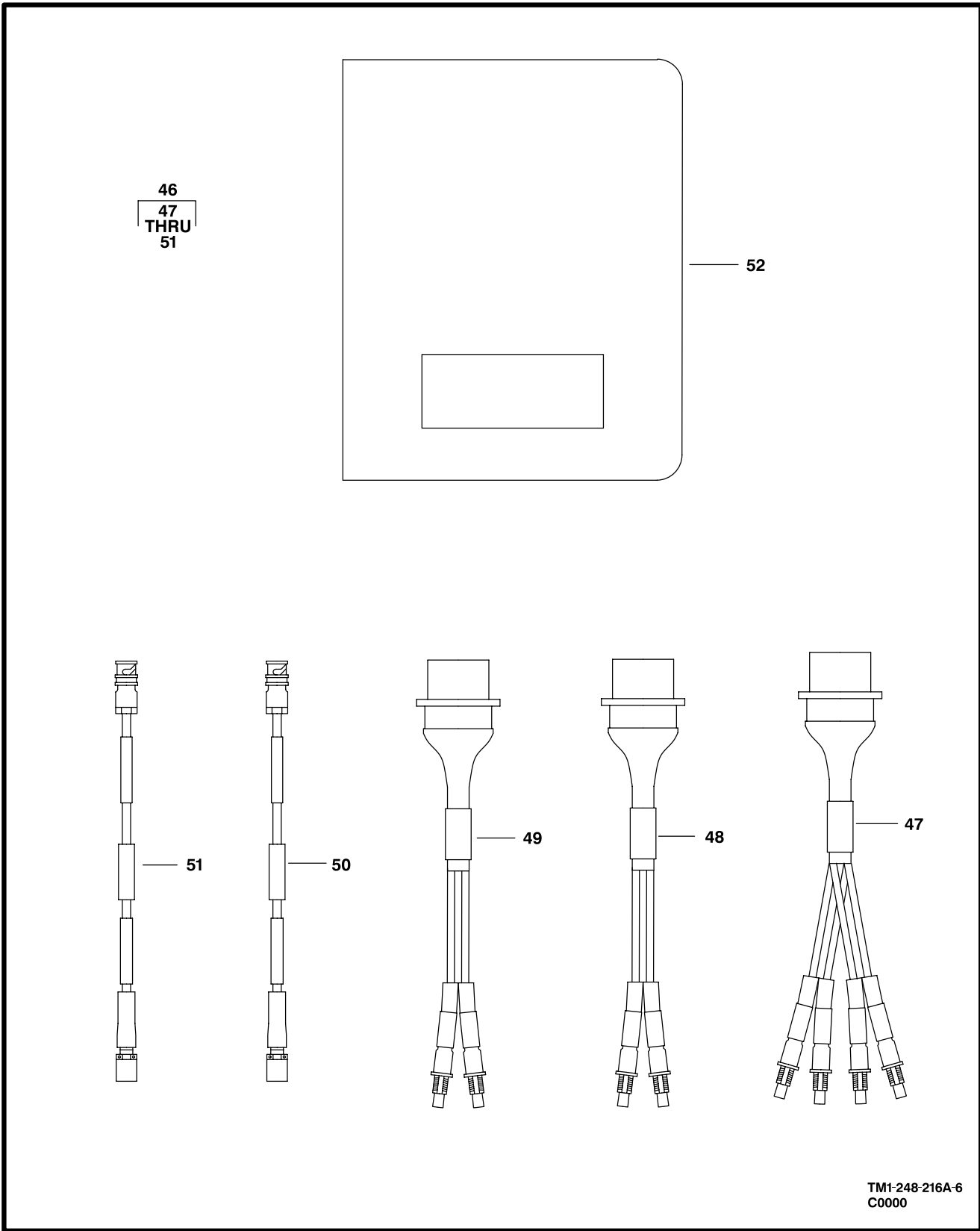
Figure 216A. Kit, Tester/Analyzer Set (Sheet 10 of 13)
