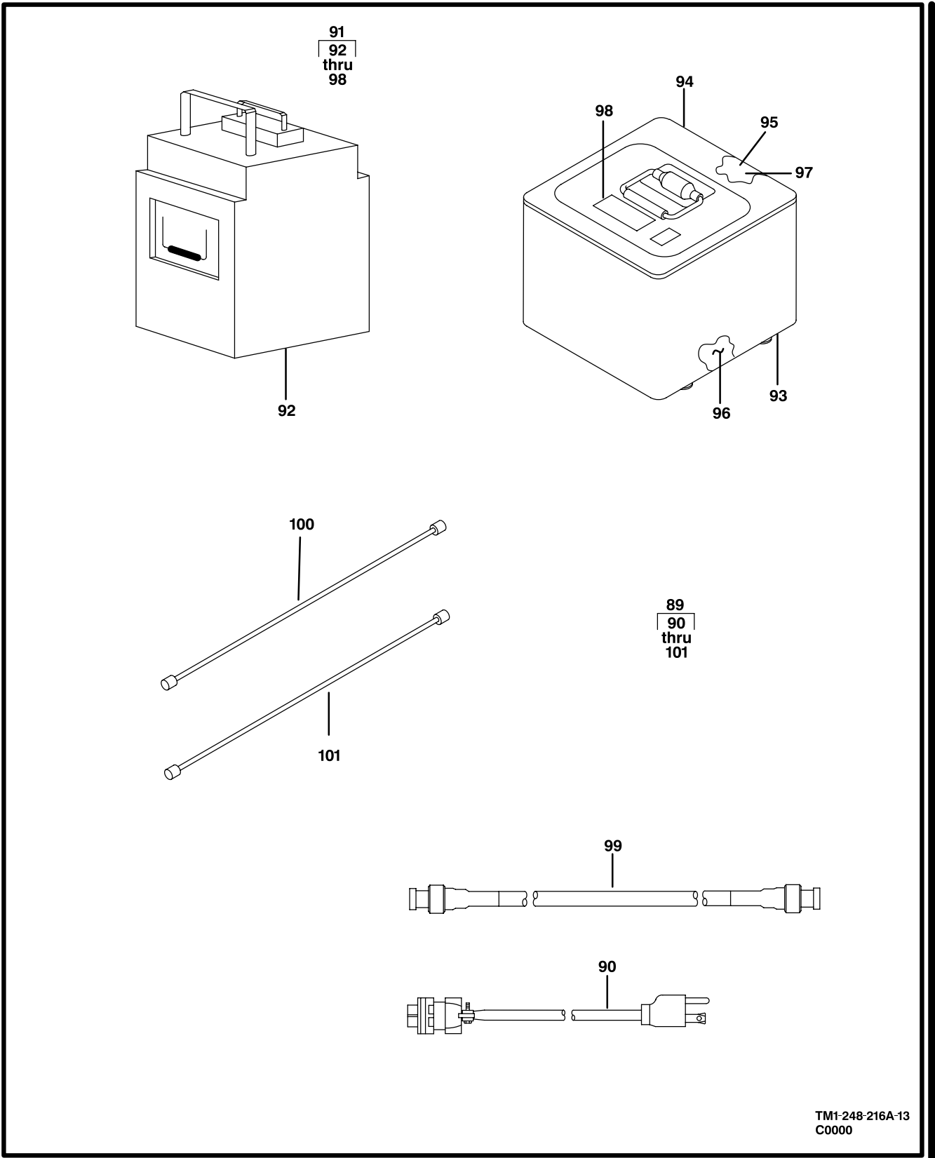
Figure 216A. Kit, Tester/Analyzer Set (Sheet 5 of 13)
