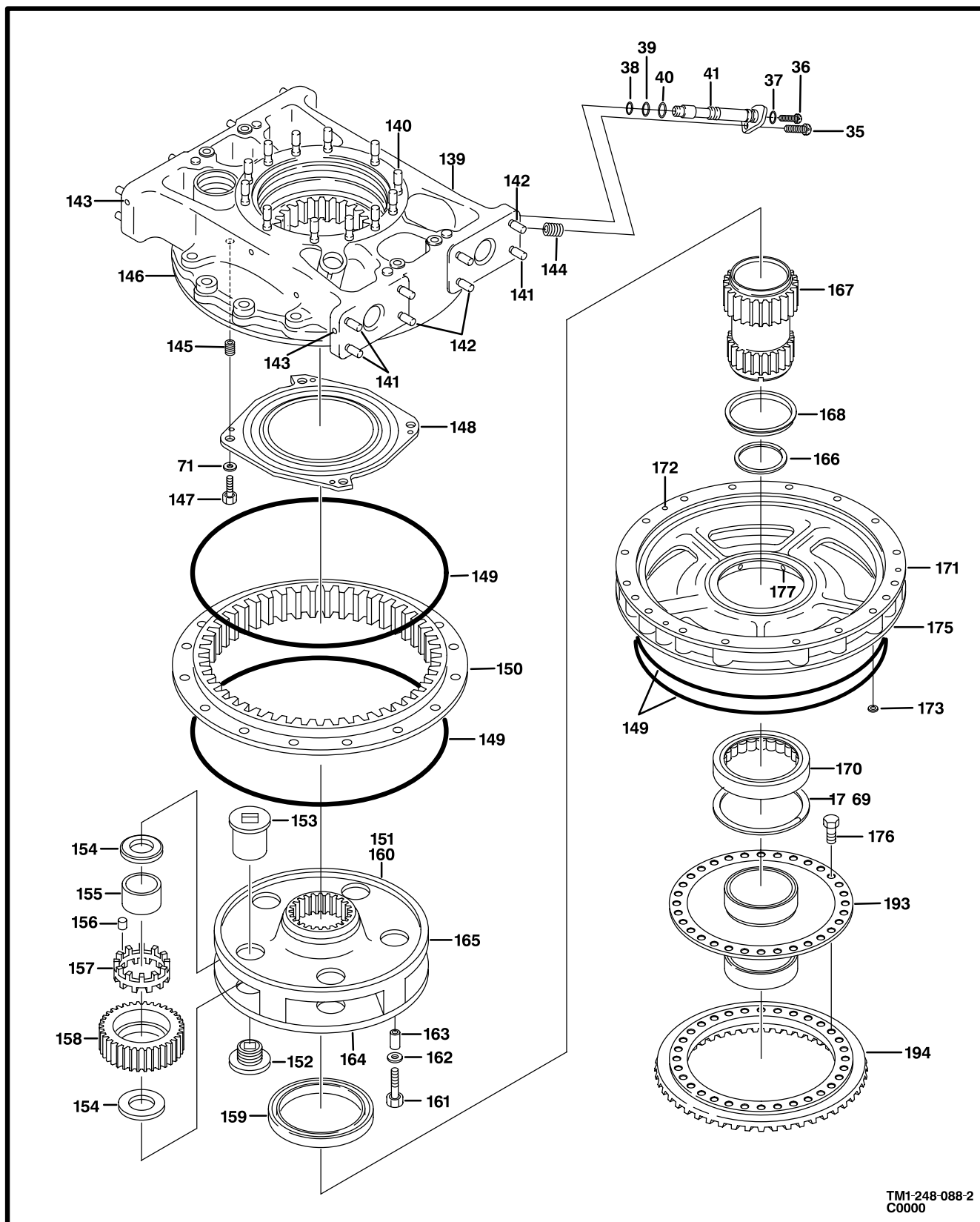
Figure 86. Transmission and Mast Assembly (Sheet 2 of 4)
