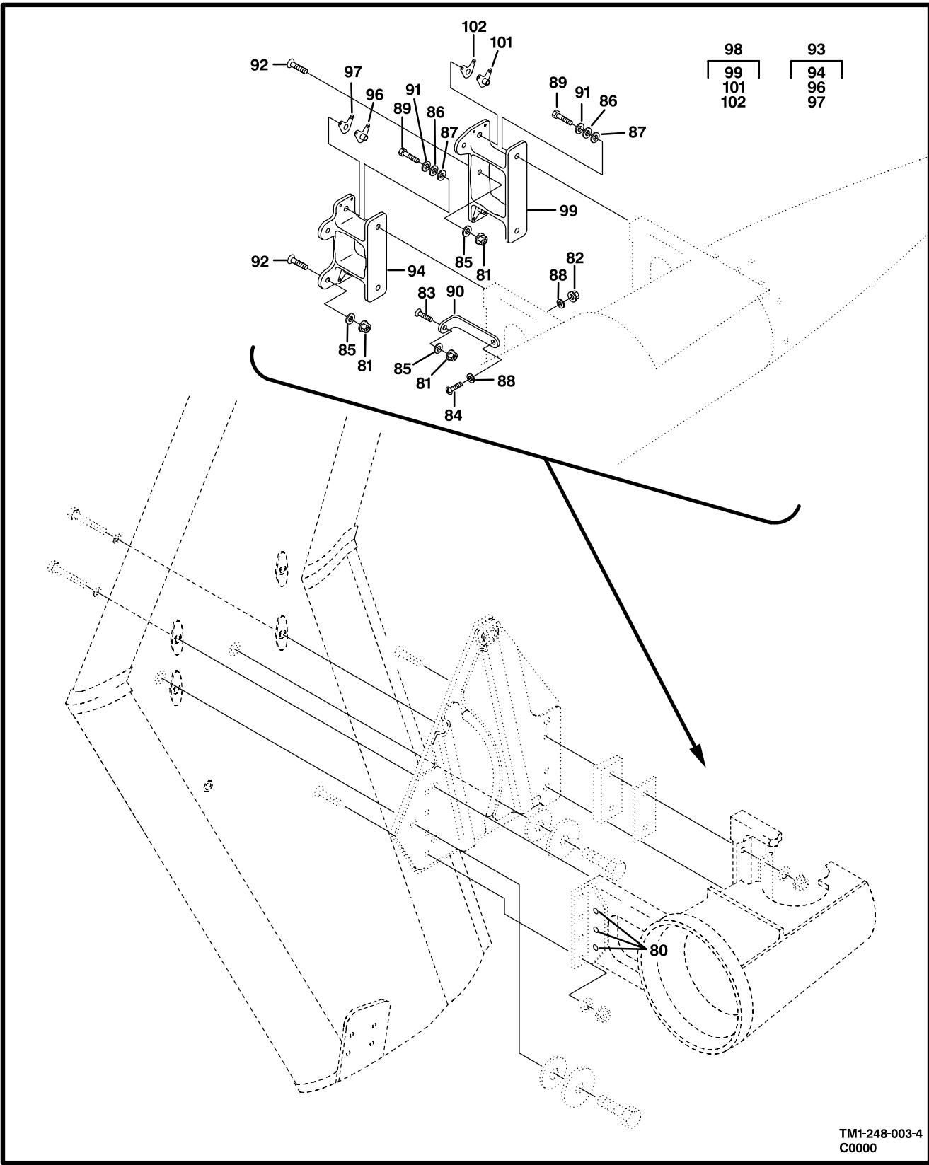
Figure 3. Fuselage Assembly (Sheet 4 of 4)
