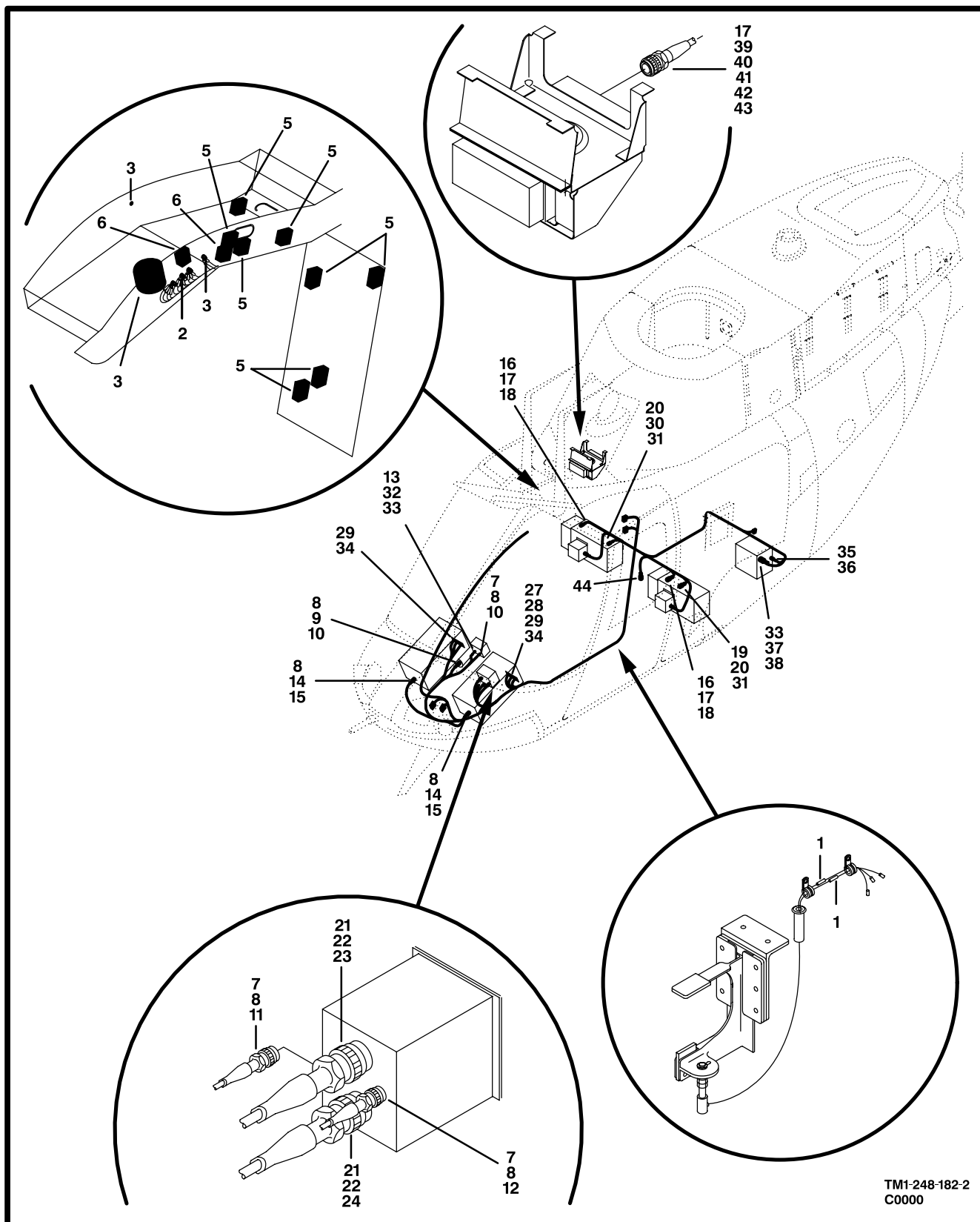
Figure 177. Cable Assembly,Control Display System (Sheet 2 of 2)
