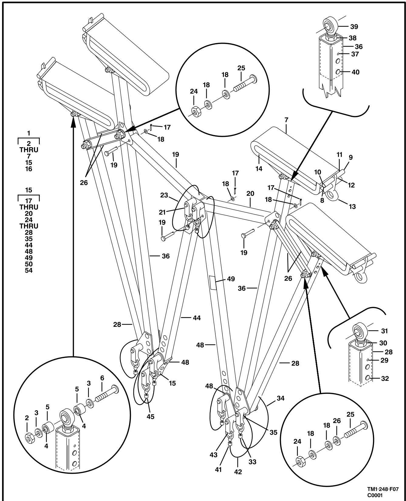
Figure F6. Flyaway Items
