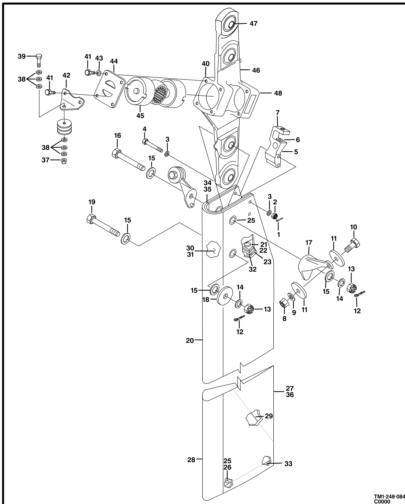
Figure 83. Hub and Blade Assembly
