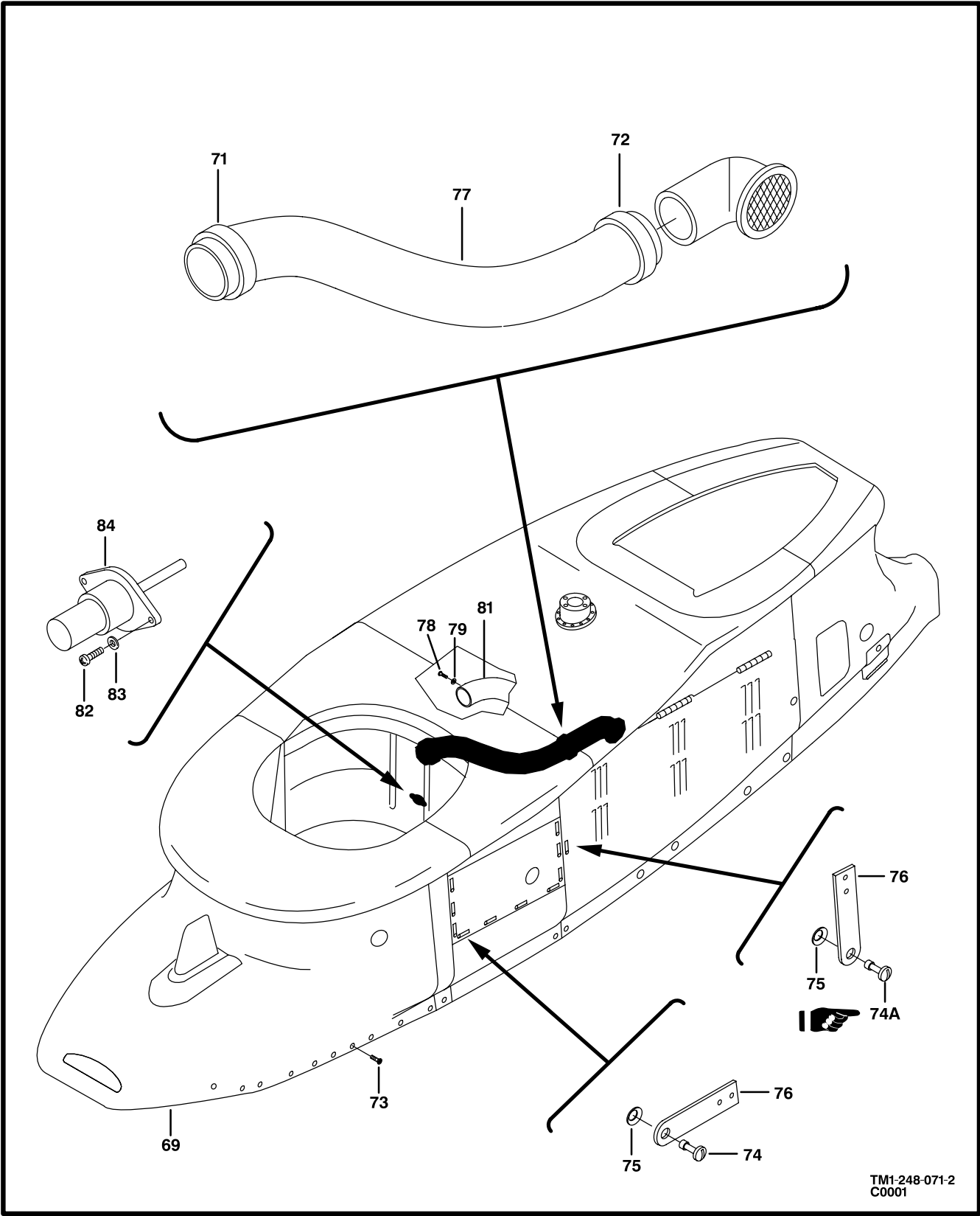
Figure 69. Power Plant Installation (Sheet 2 of 2)
