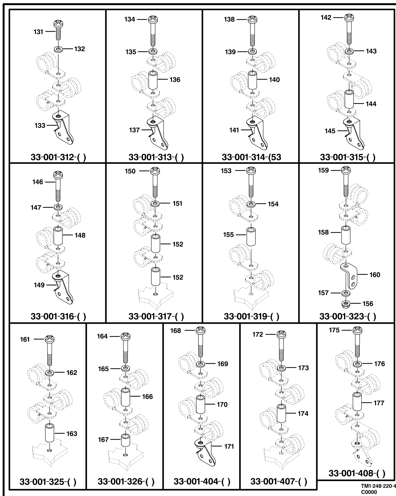
Figure 215. Support Installations (Sheet 4 of 5)
