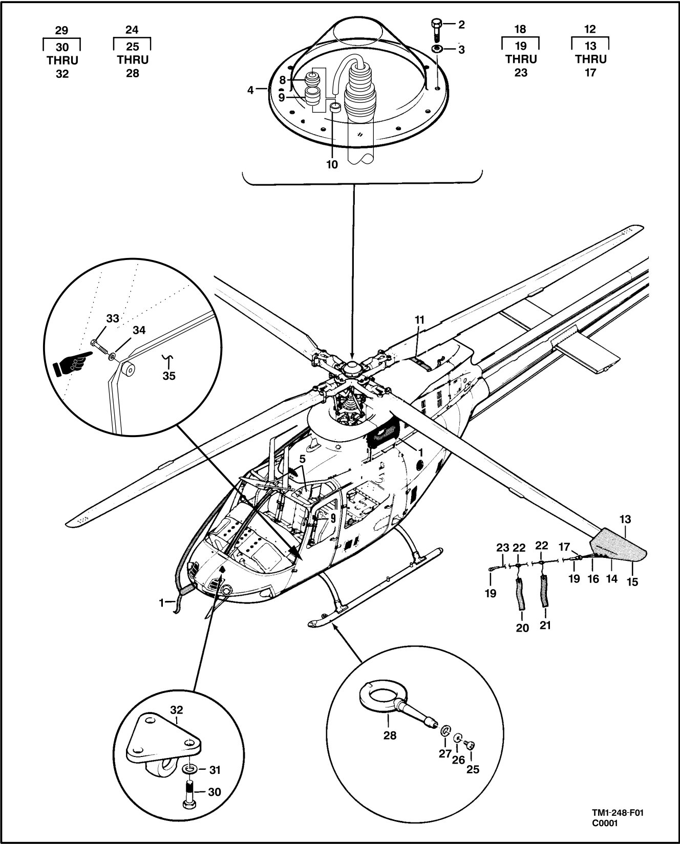
Figure F1. Flyaway Items
