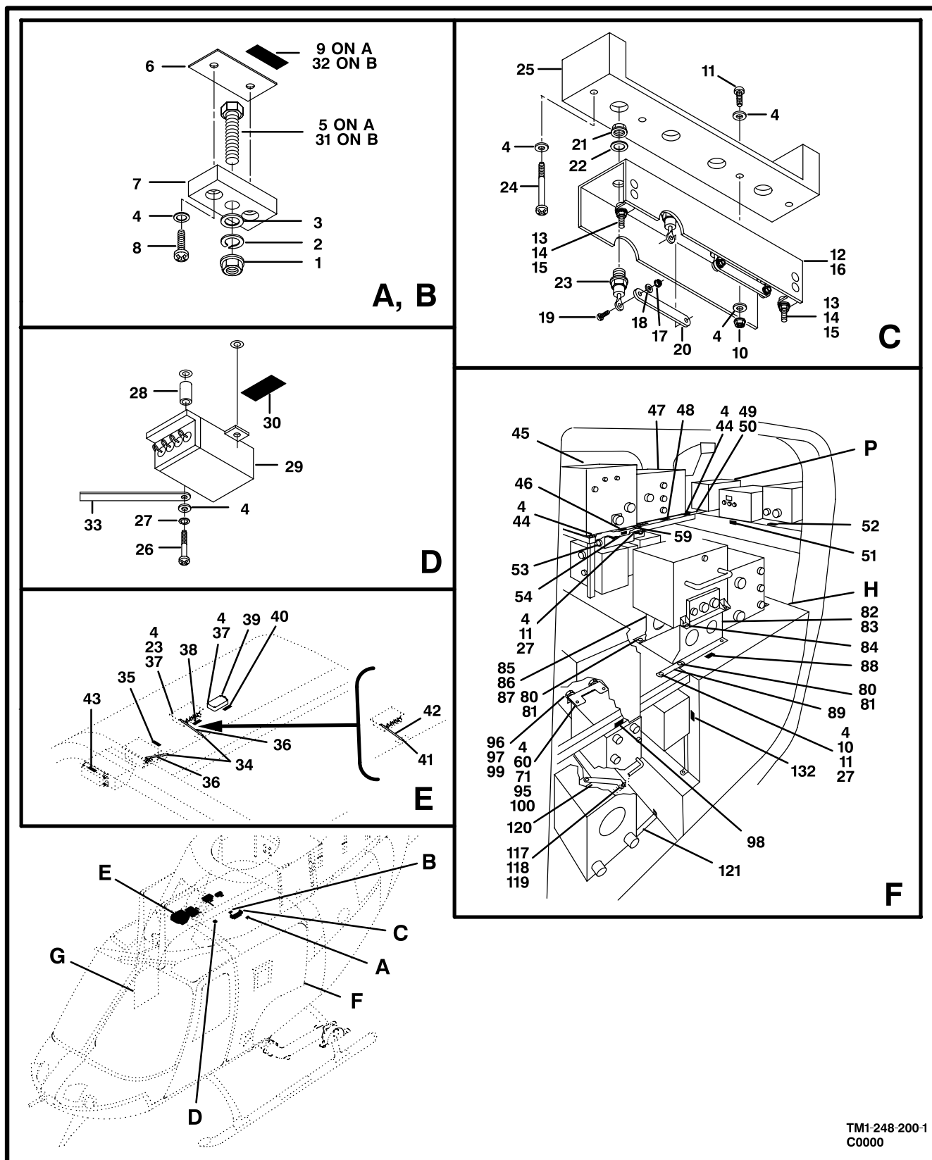
Figure 195. Electrical And Avionics Installation, AFT Cabin (Sheet 1 of 2)
