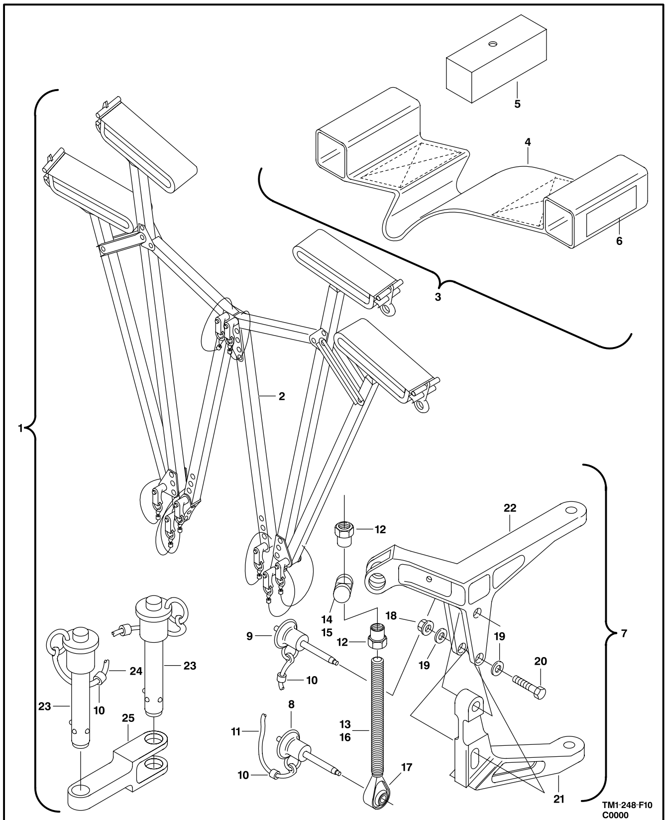
Figure F8. Rack Assembly, Blade Fold
