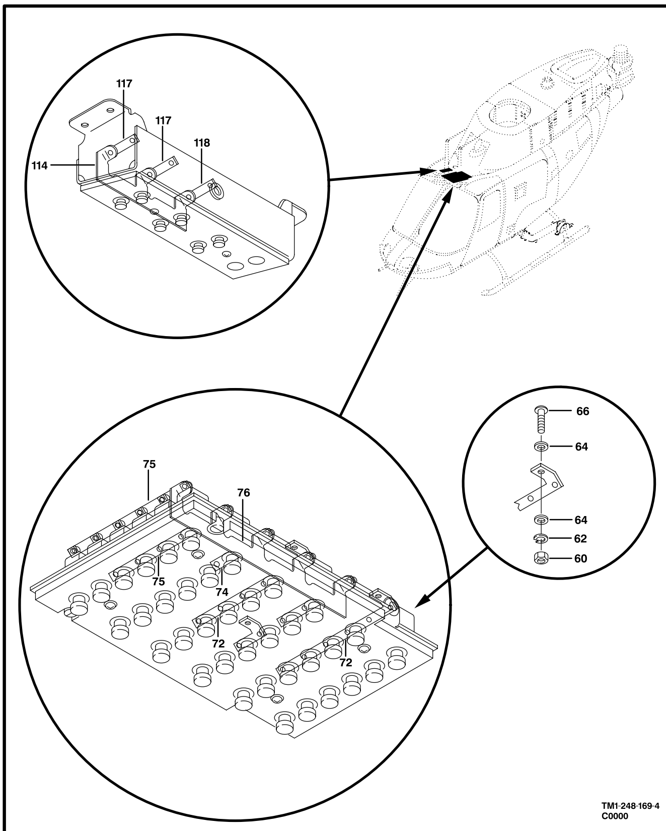
Figure 164. Console Installation, Overhead Electrical (Sheet 4 of 4)
