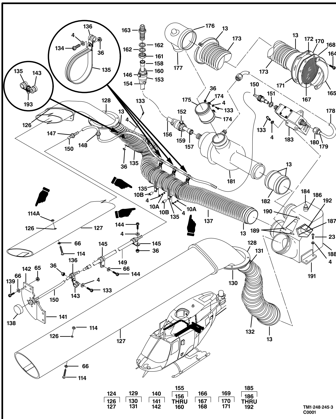
Figure 261. Environmental Control System (Sheet 3 of 3)
