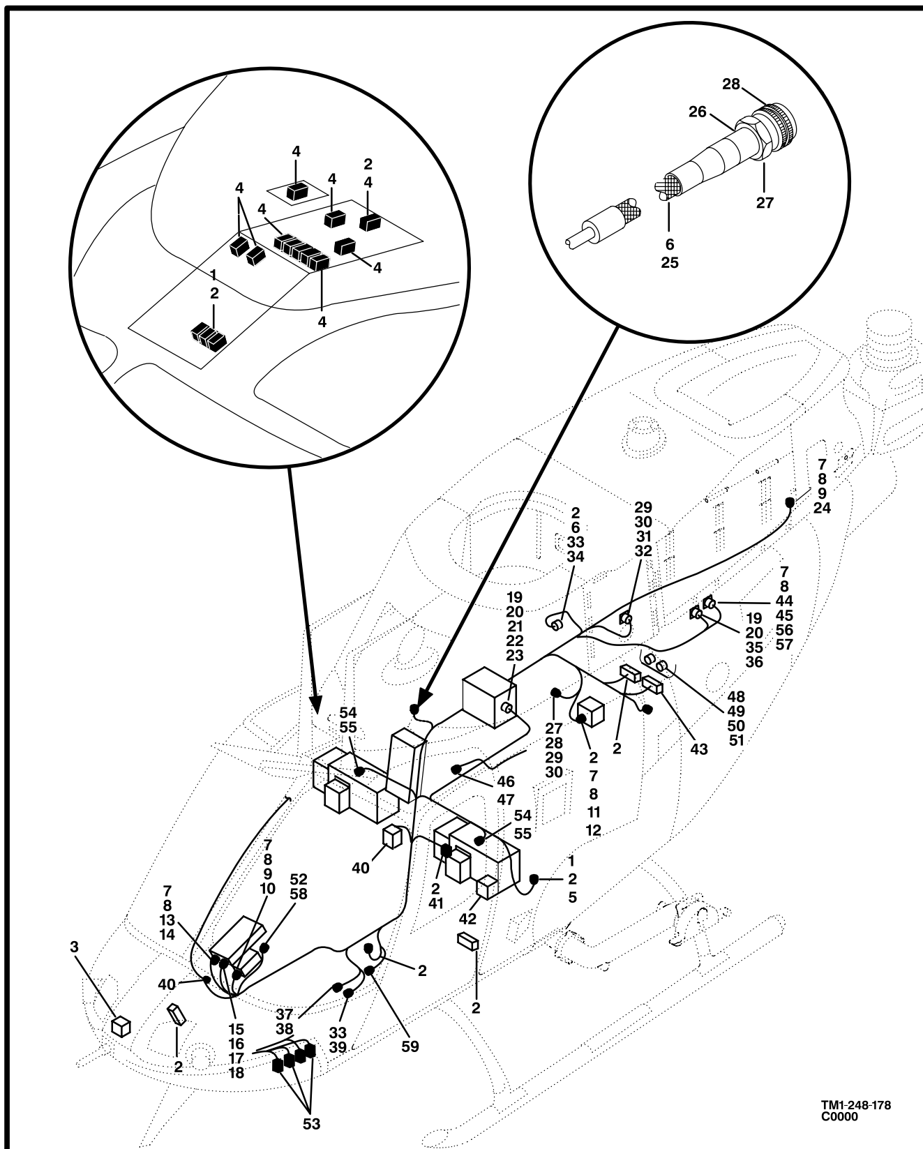
Figure 173. Cable Assembly, Power Plant and Transmission
