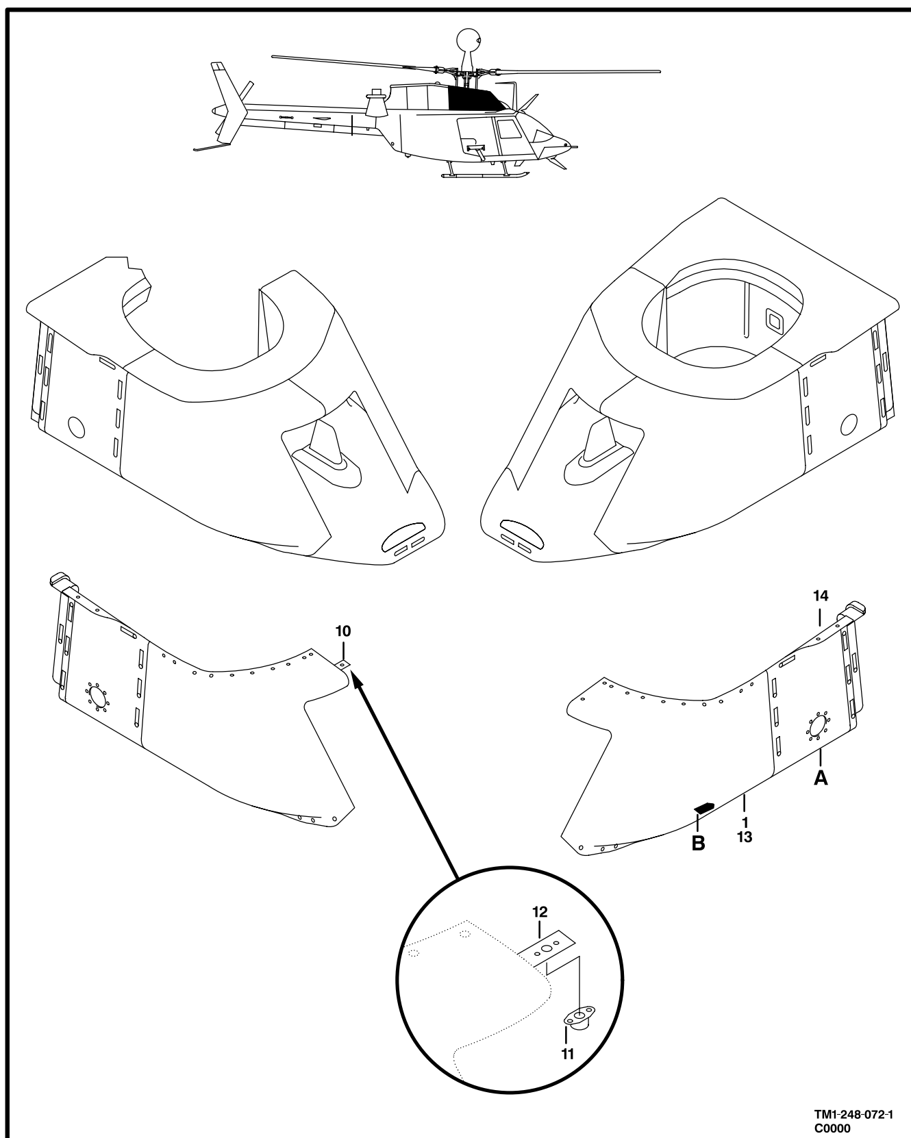
Figure 70. Shield Assembly (Sheet 1 of 2)
