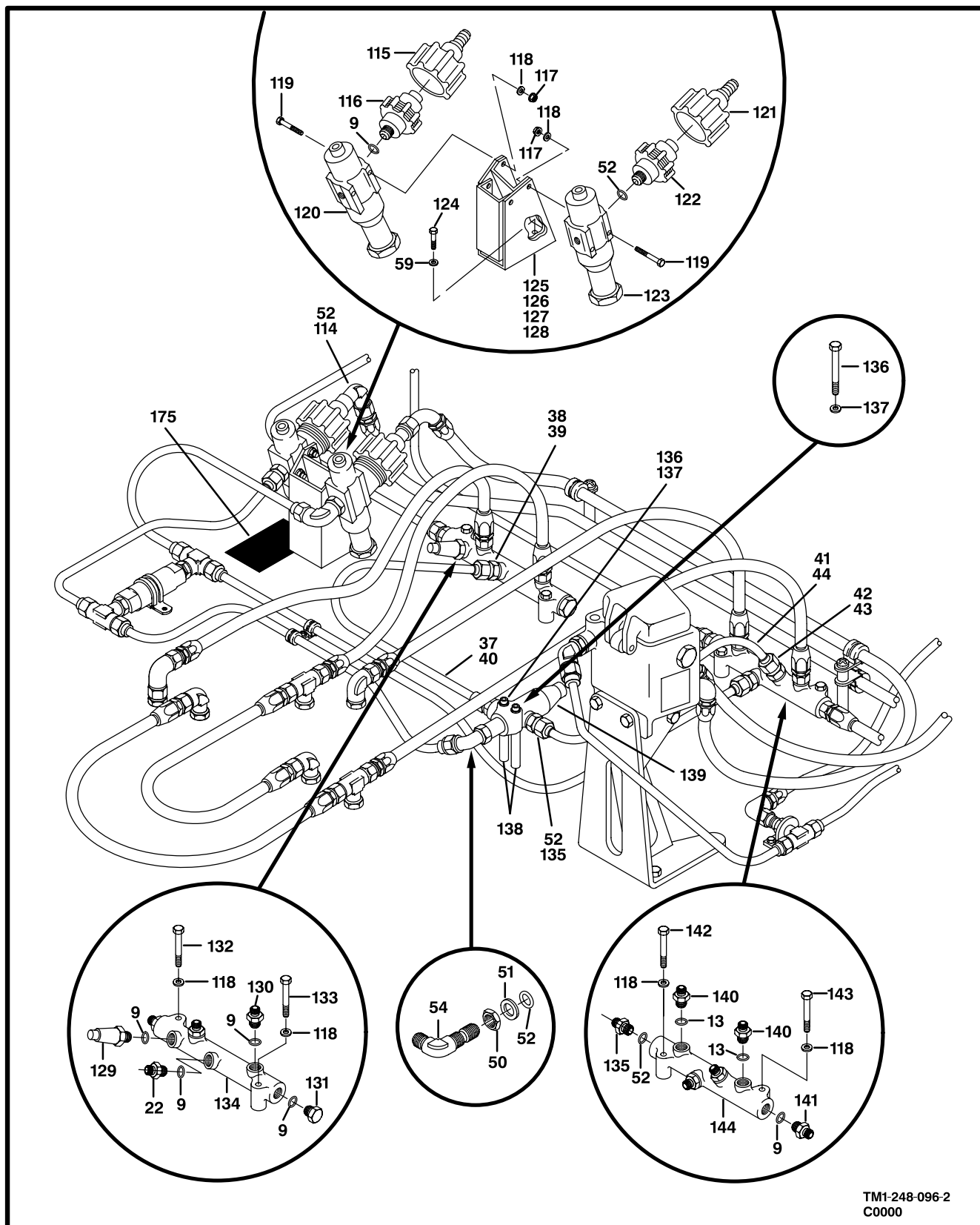
Figure 93. Hydraulic System Installation, Flight Controls (Sheet 2 of 3)
