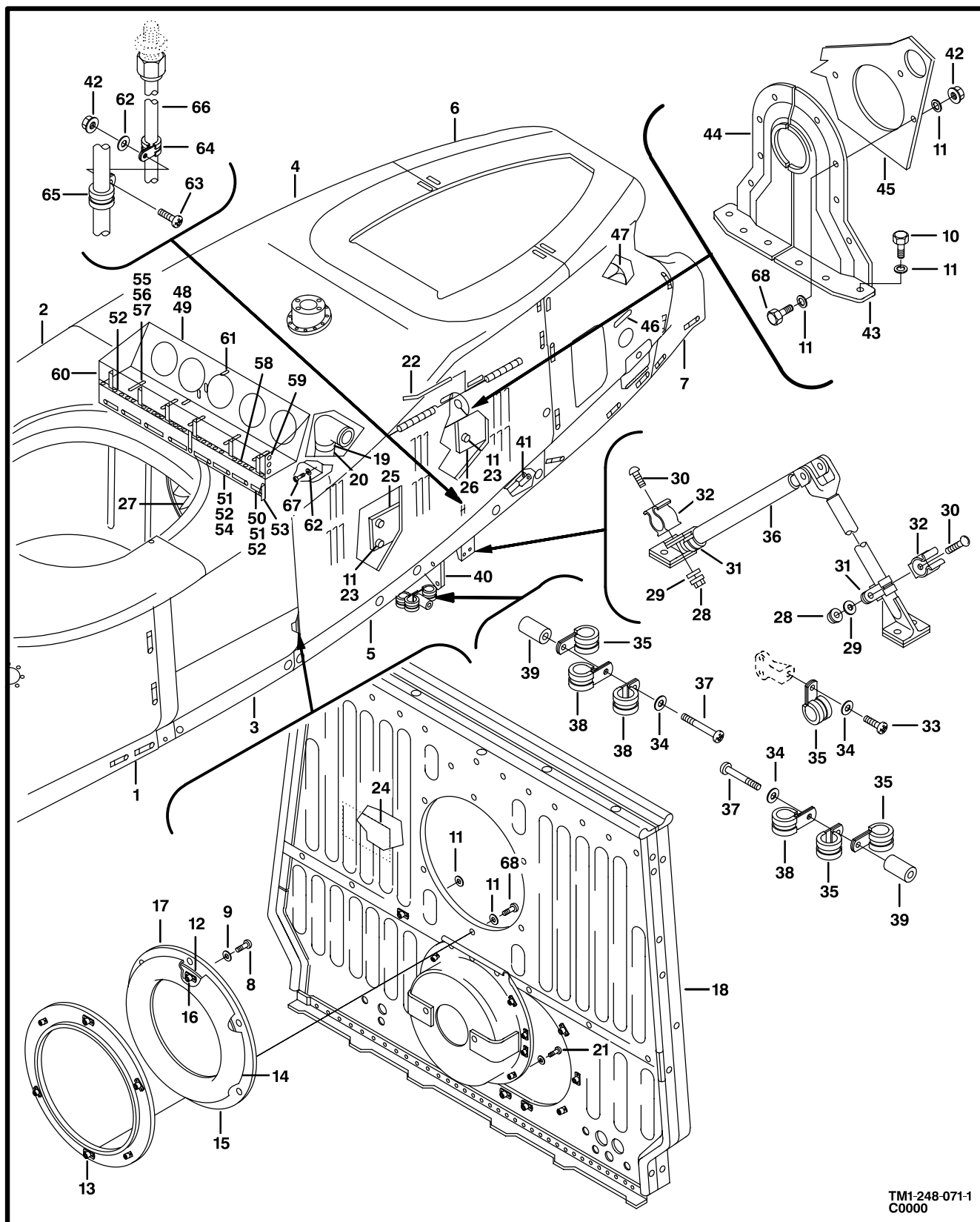
Figure 69. Power Plant Installation (Sheet 1 of 2)
