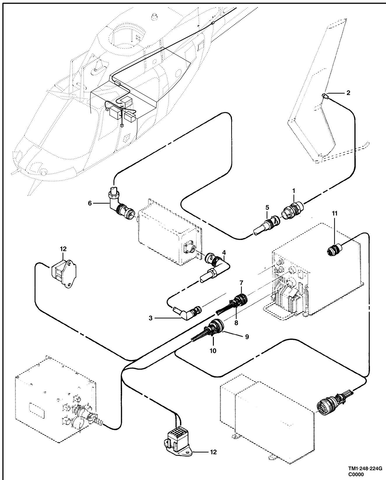
Figure 225. Cable Assembly,VHF-AM Communication System
