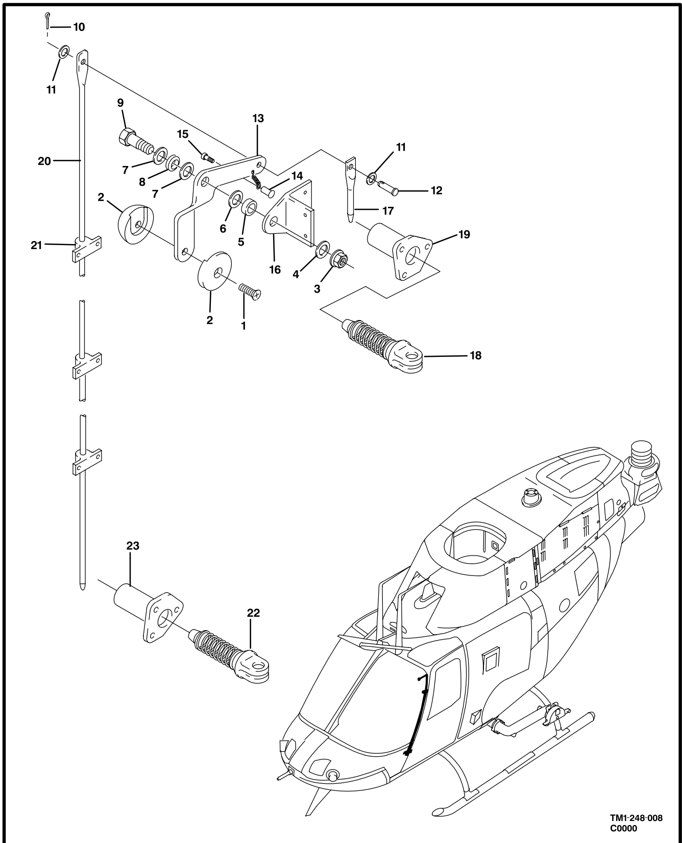
Figure 8. Jettison Mechanism Installation, Crew Door
