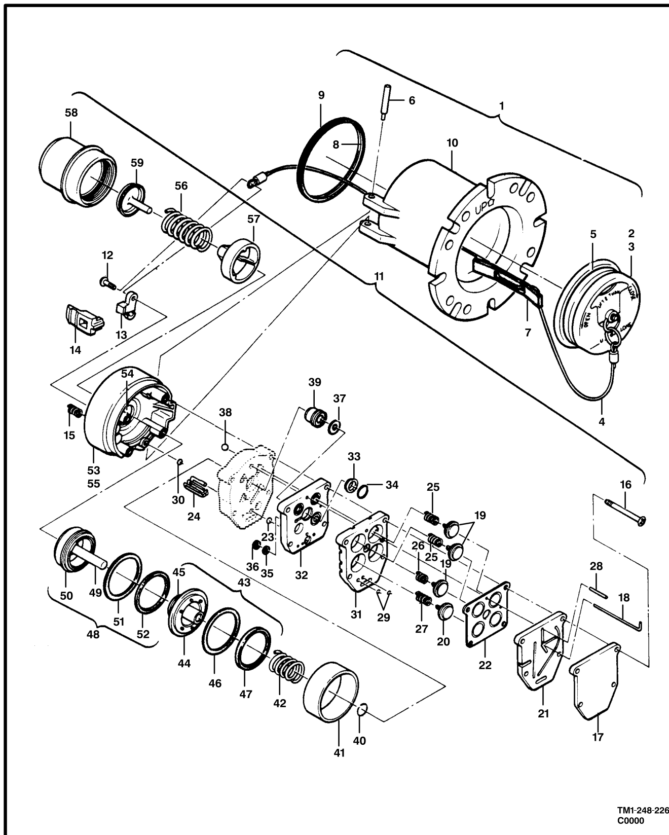
Figure 244. Receiver, Refueling
