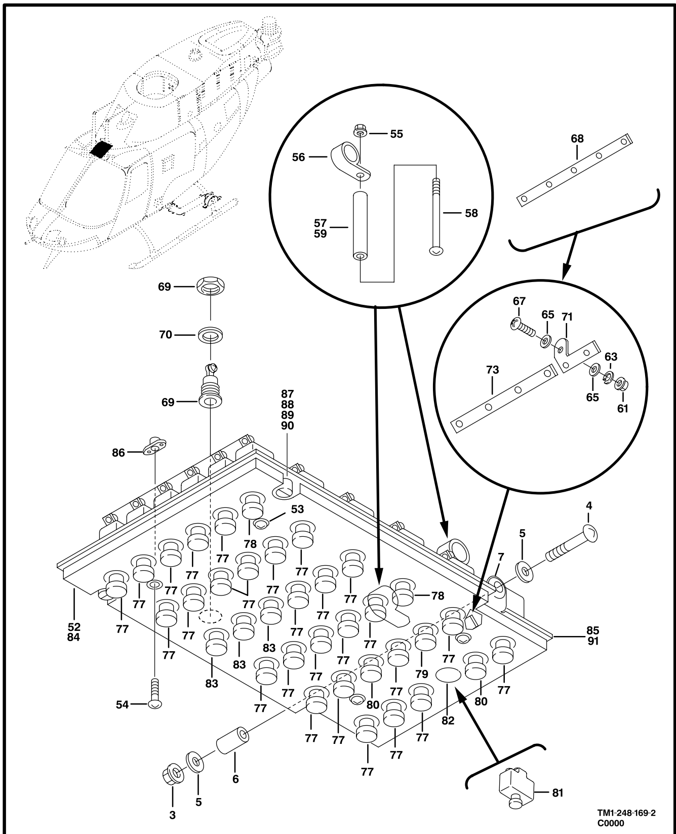
Figure 164. Console Installation, Overhead Electrical (Sheet 2 of 4)
