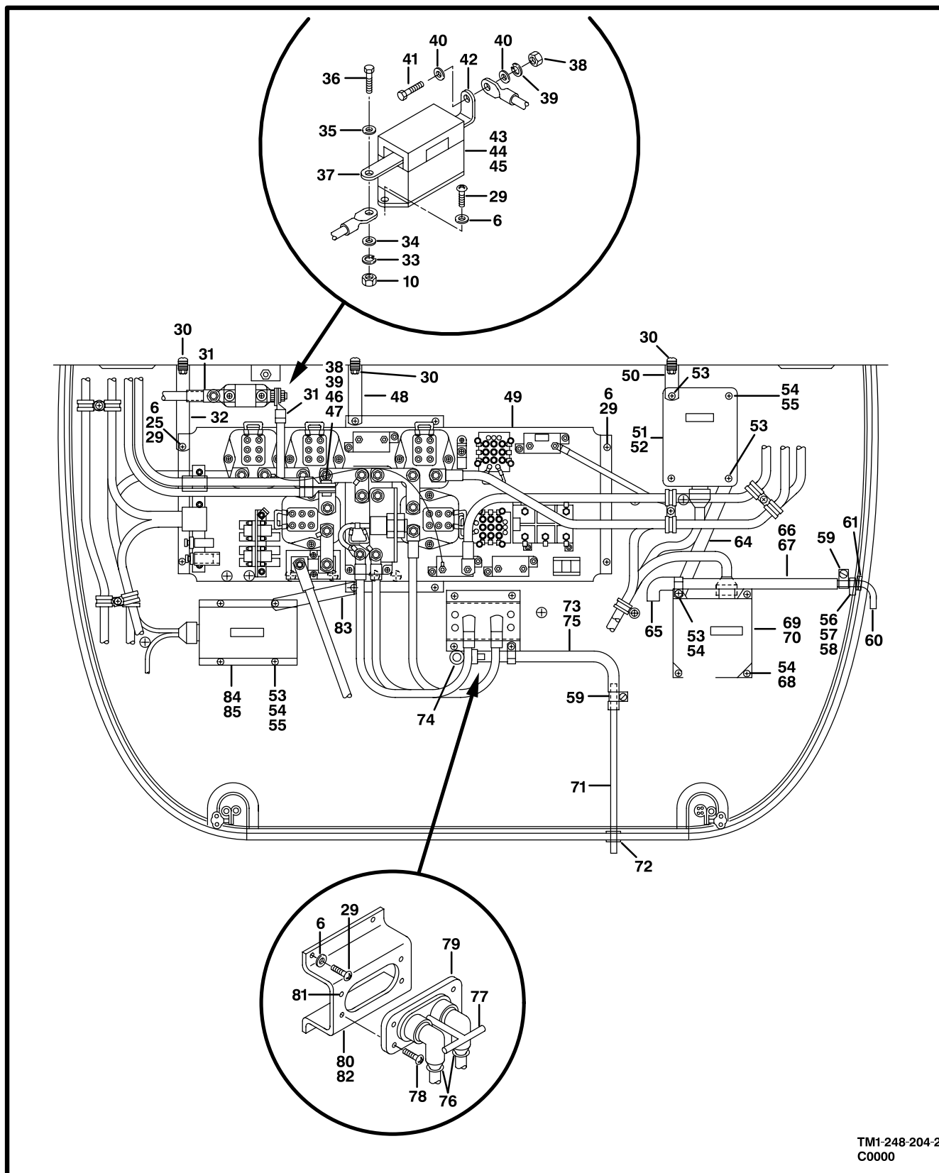
Figure 199. Electrical Assembly, Avionics Installation, AFT Cabin (Sheet 2 of 5)
