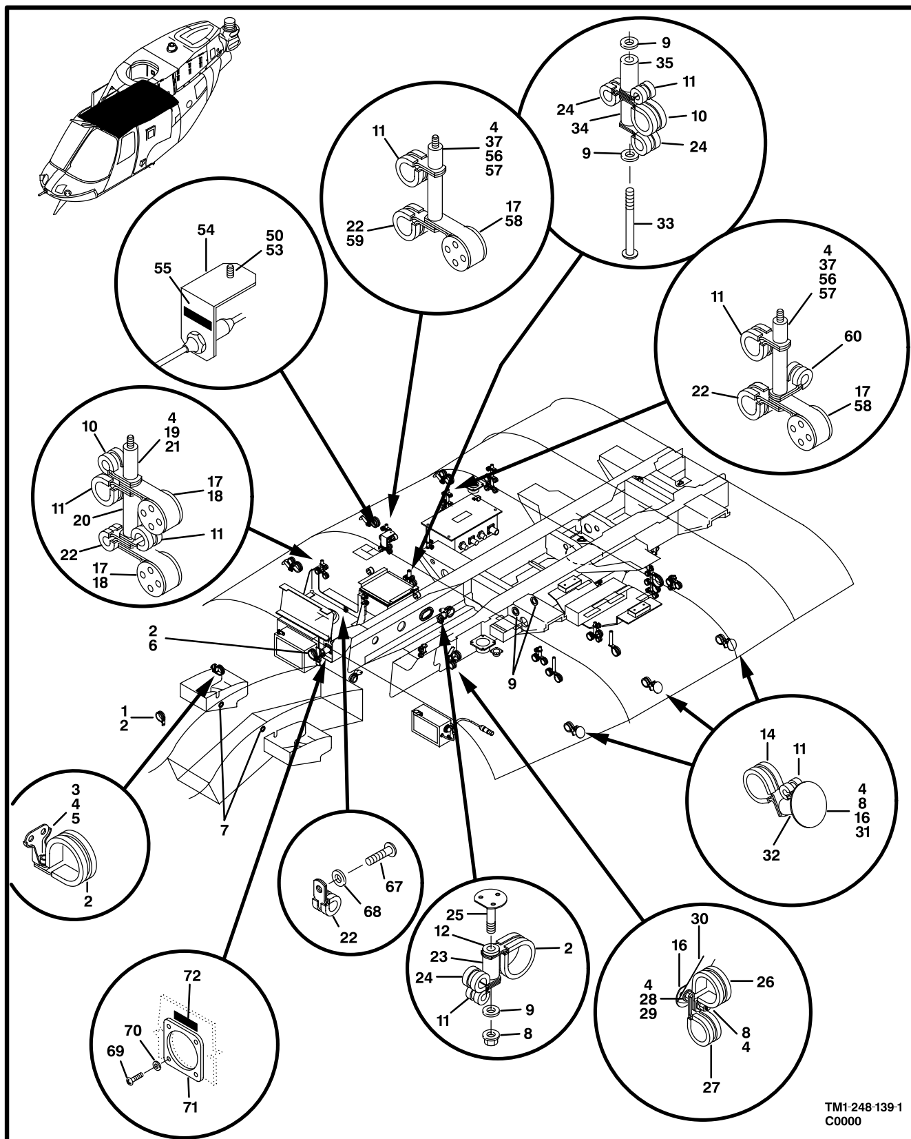
Figure 134. Electrical Installation,Bulkhead (Sheet 1 of 2)
