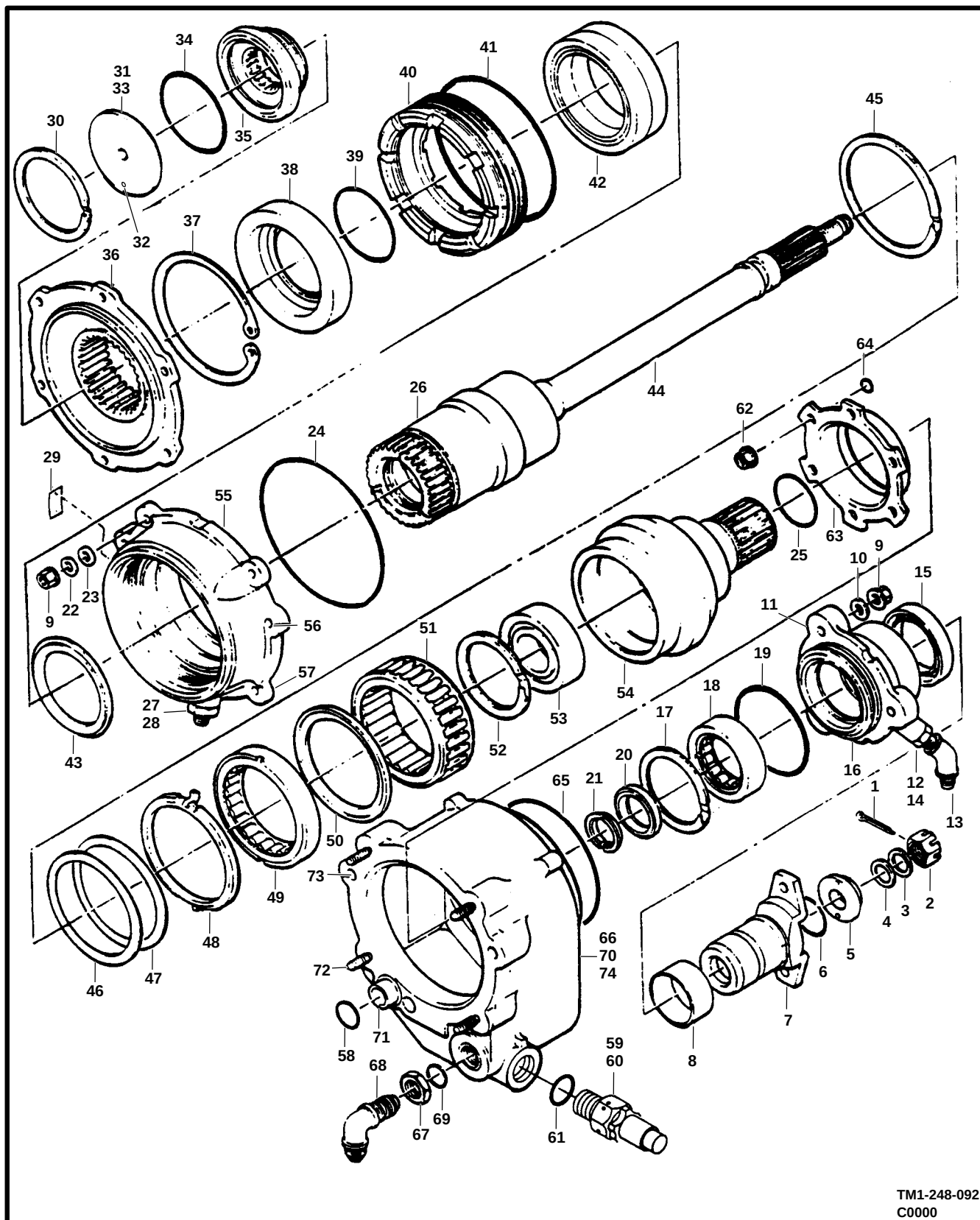
Figure 89. Freewheeling Installation
