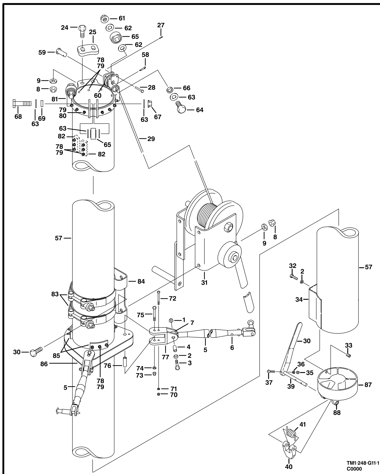
Figure G6. Hoist Installation, Mast Mounted Sight (Sheet 1 of 2)
