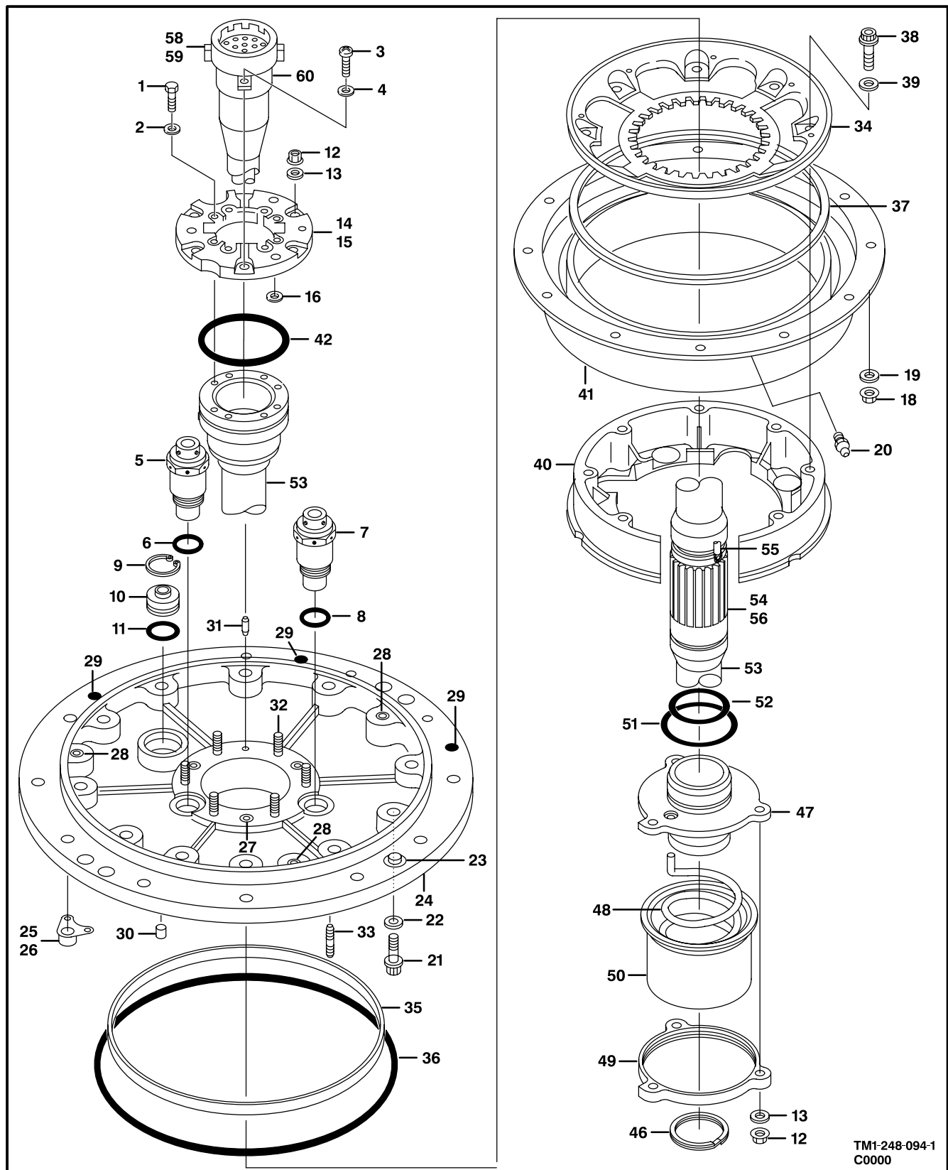
Figure 91. Torquemeter Installation (Sheet 1 of 2)
