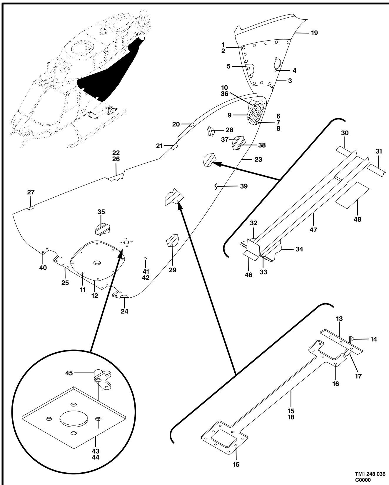
Figure 35. Antenna Access Door
