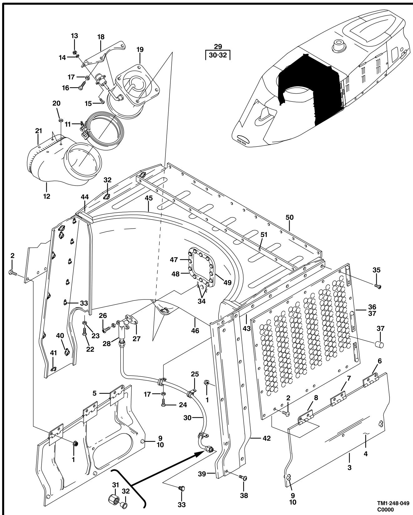
Figure 49. Induction System
