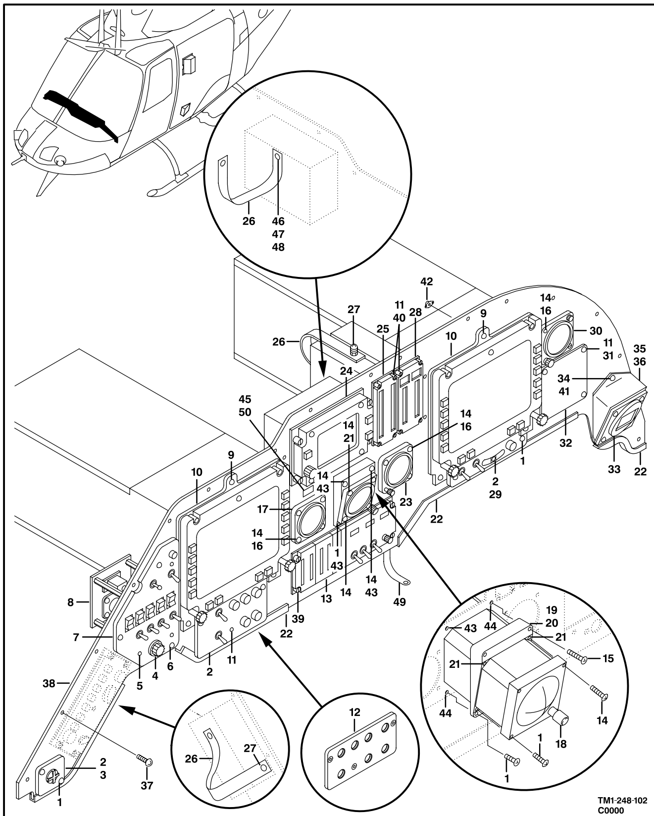
Figure 98. Instrument Panel Installation
