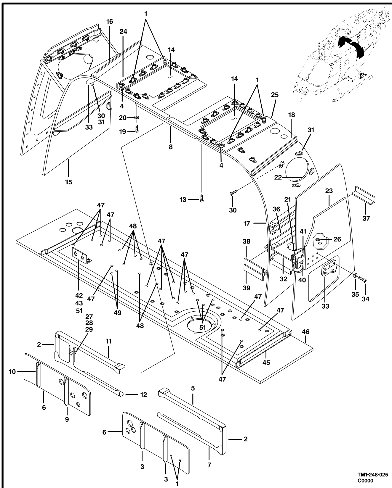
Figure 24. MOD-Closure,AFT
