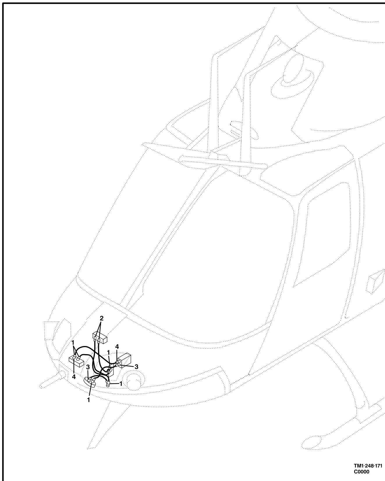
Figure 166. Cable Assembly,DC Power System
