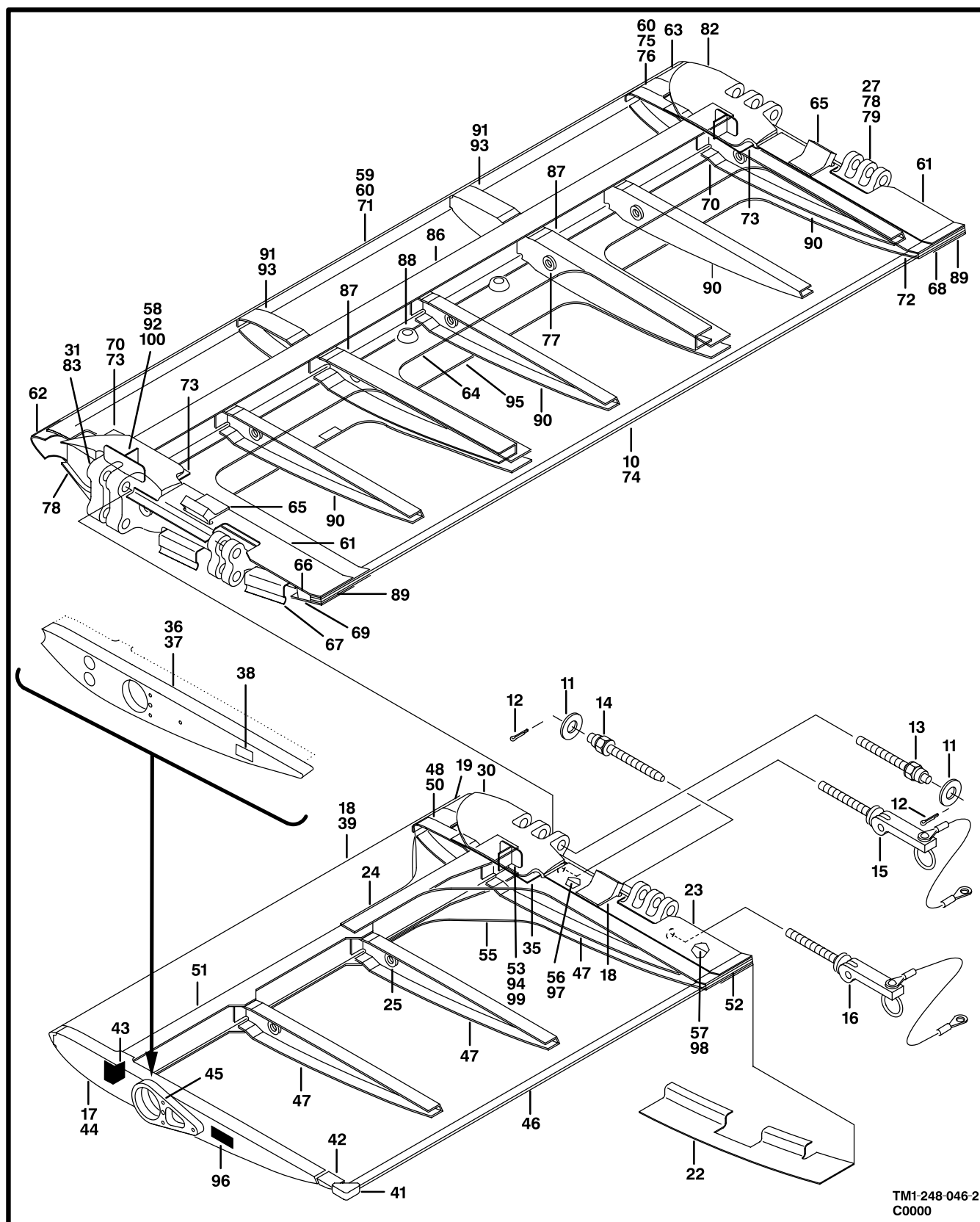
Figure 46. Stabilizer Installation, Horizontal (Sheet 2 of 3)
