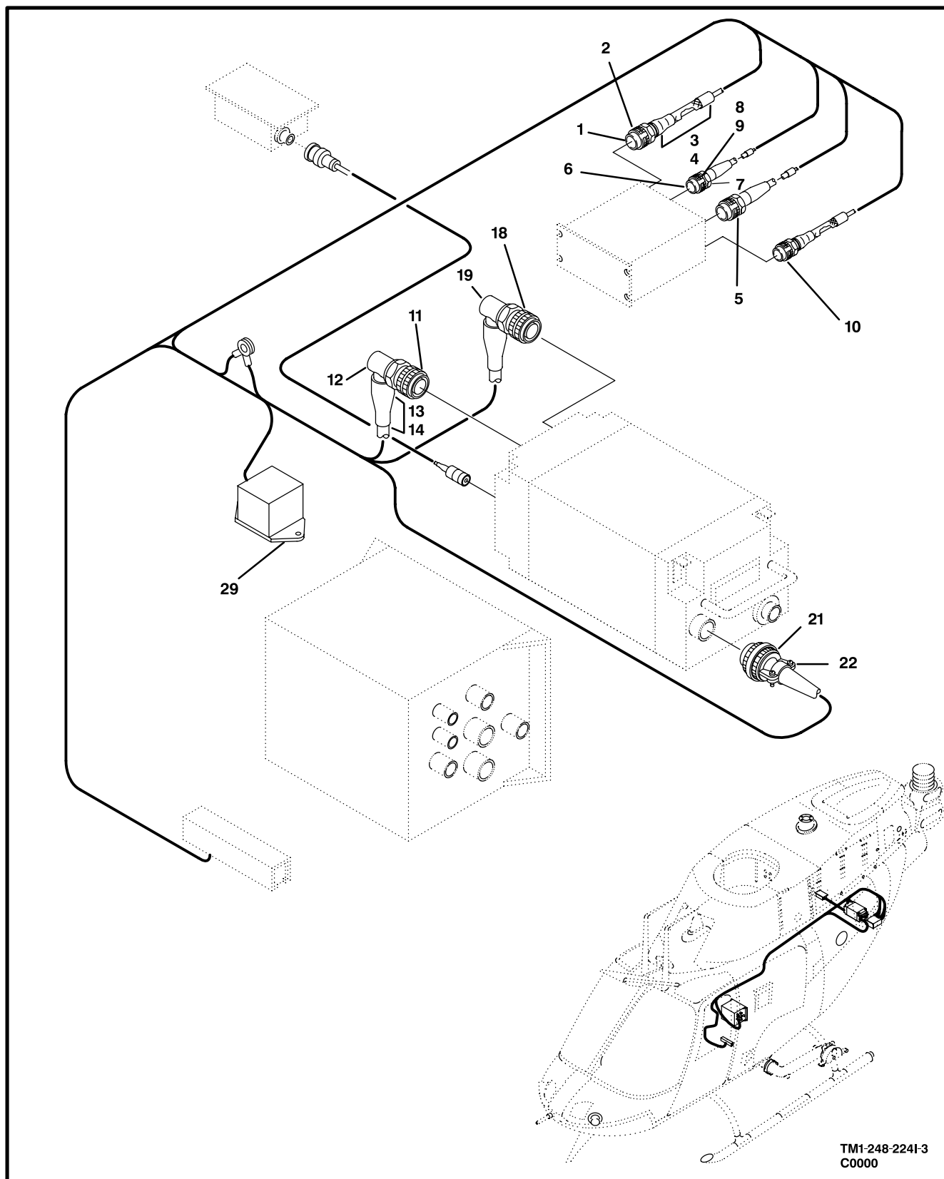
Figure 227. Cable Assembly, NO. 2 VHF-FM Communication System (Sheet 3 of 3)
