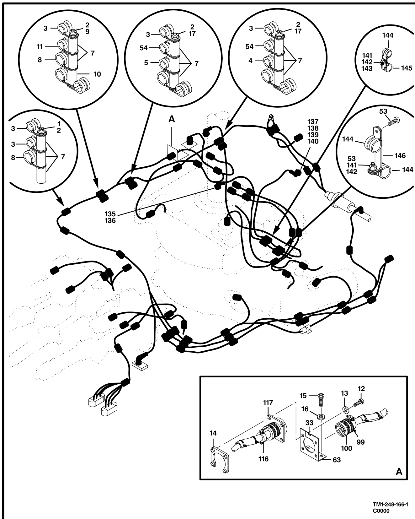
Figure 161. Electrical Installation, Mast Mounted Sight (Sheet 1 of 6)
