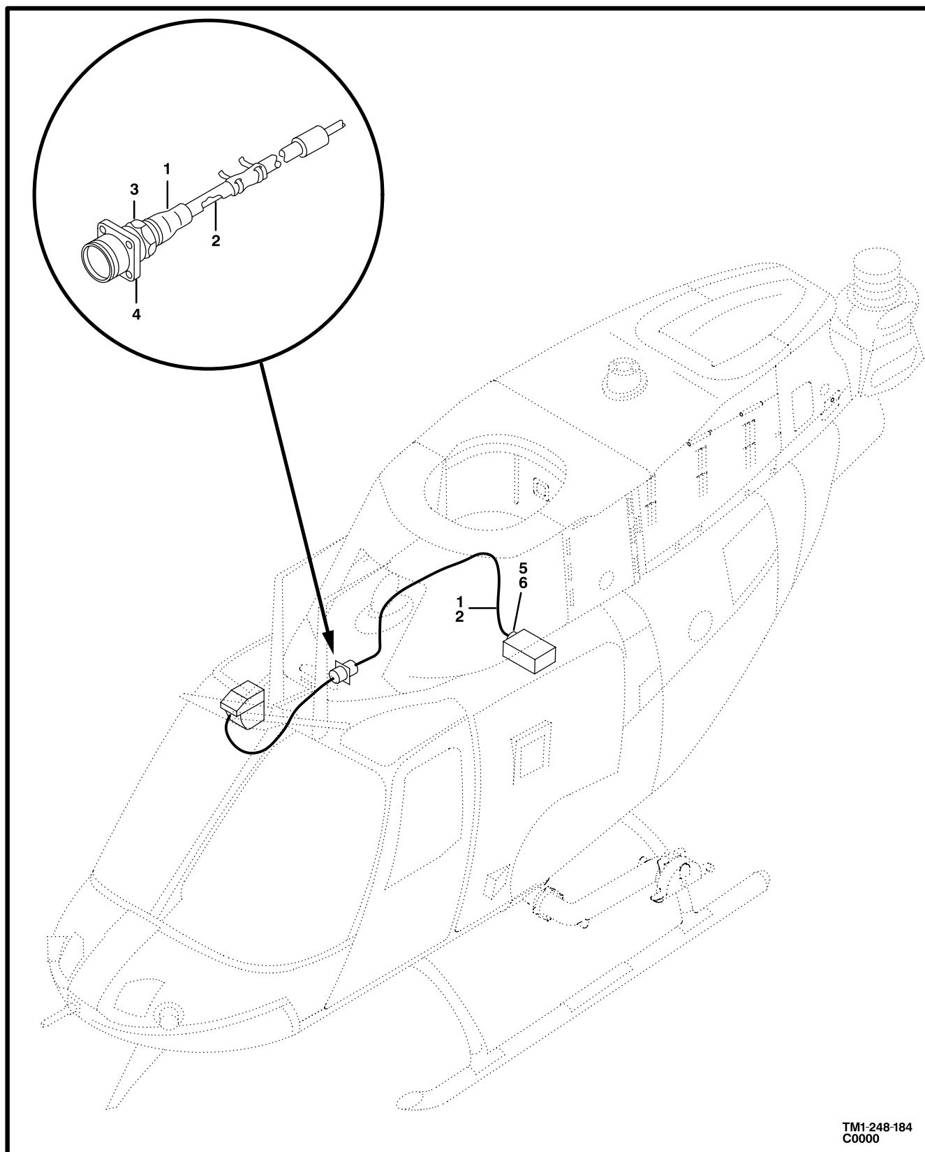
Figure 179. Cable Assembly, ATAS
