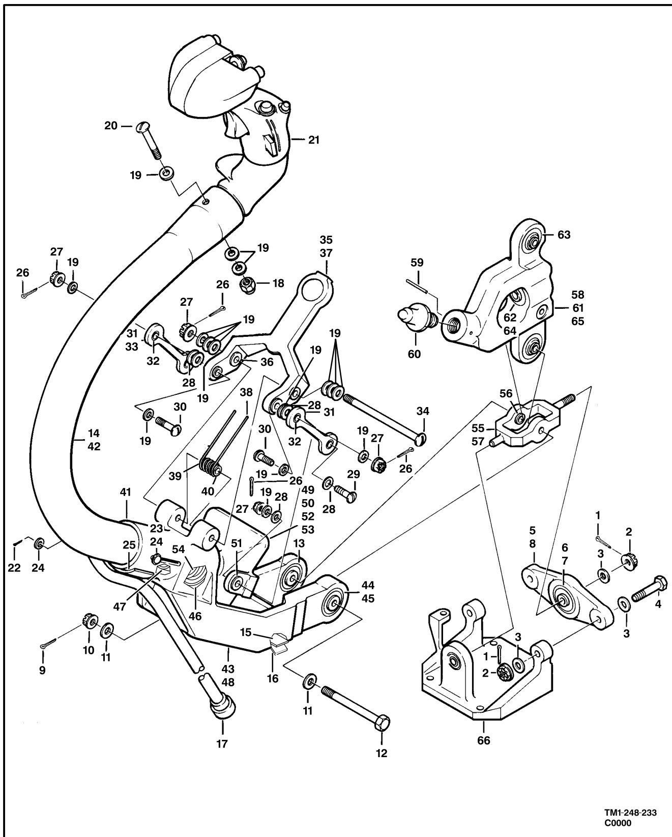
Figure 251. Stick Assembly, Copilot, Cyclic
