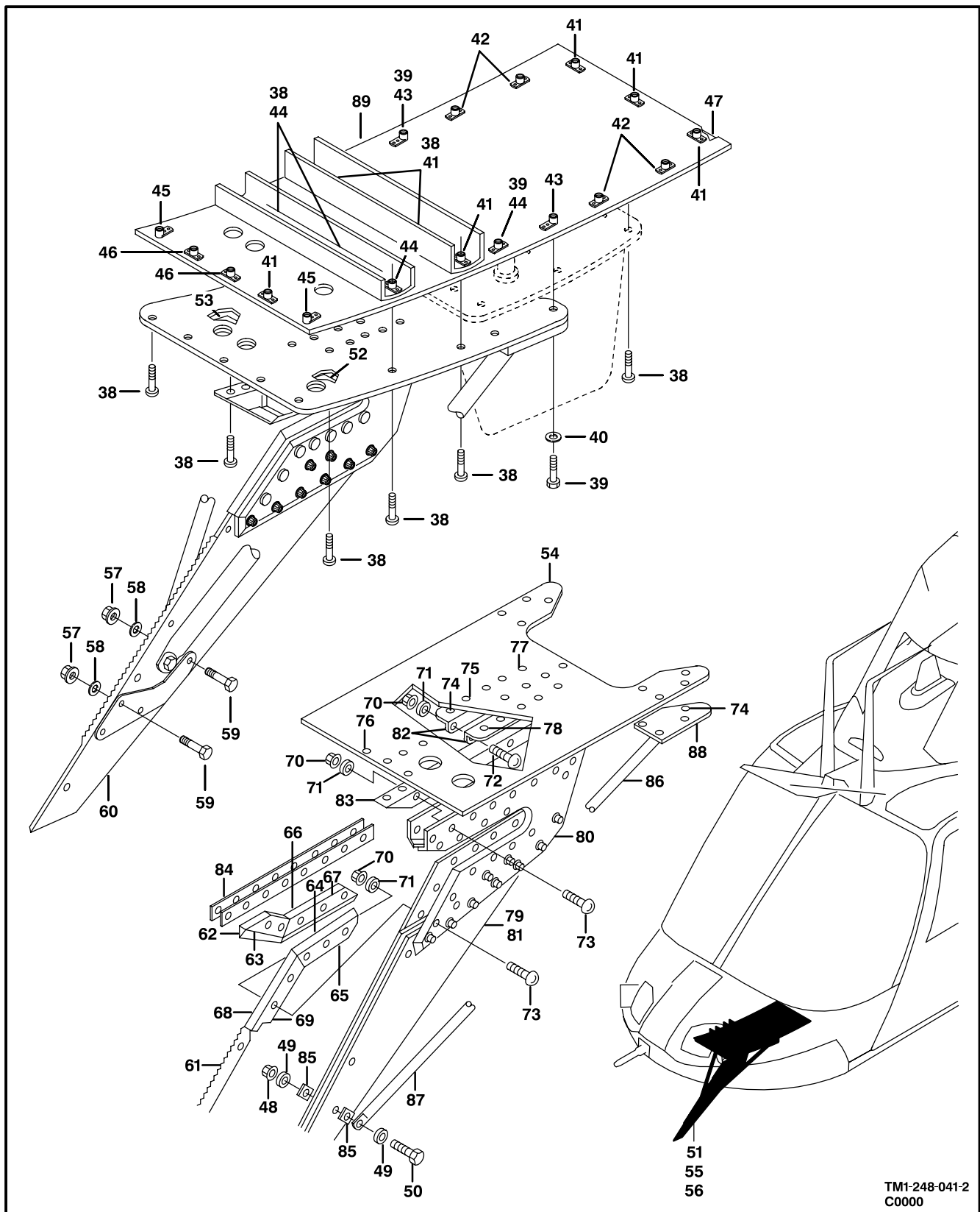
Figure 40. Wire Cutter Installation (Sheet 2 of 2)
