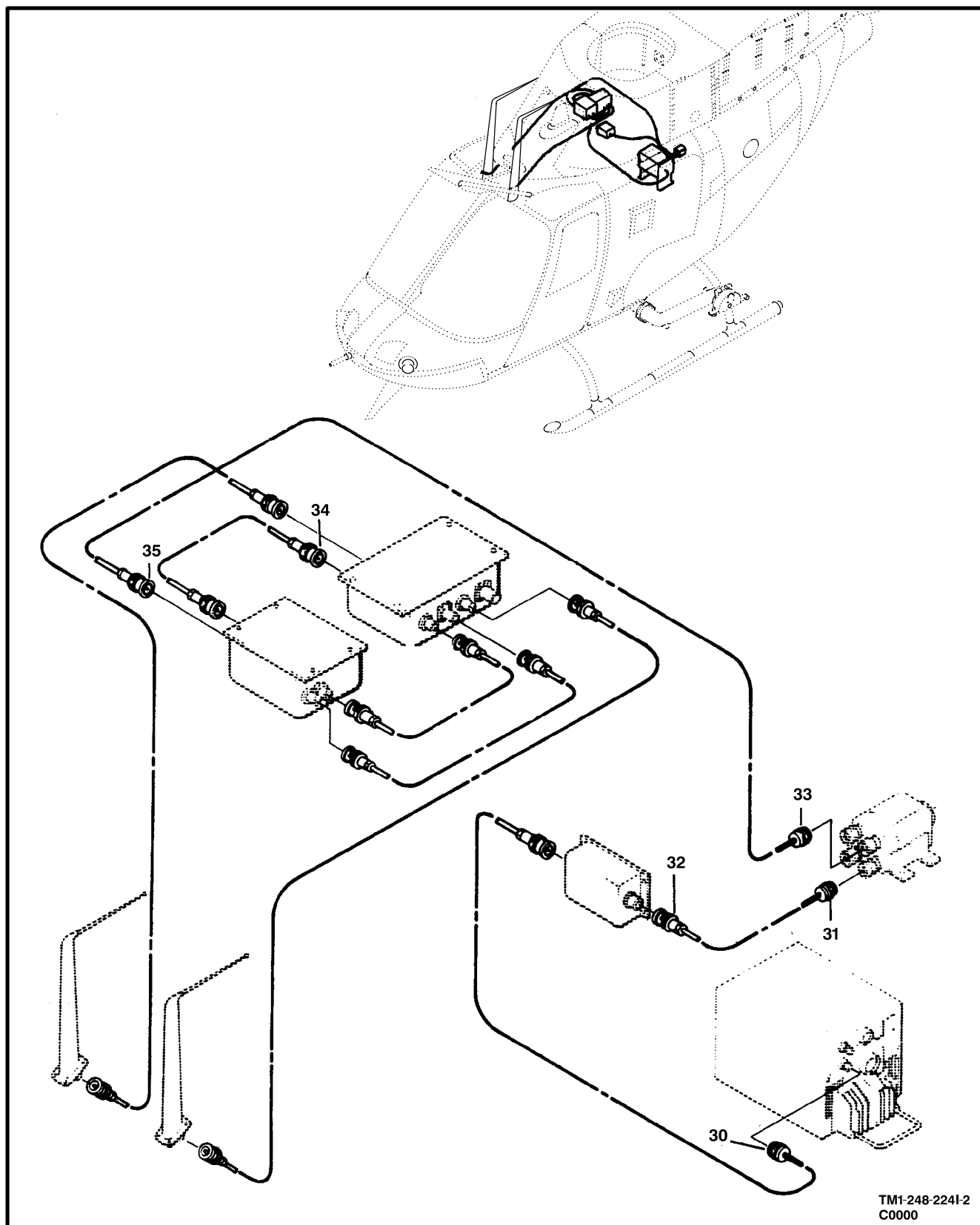
Figure 227. Cable Assembly, NO. 2 VHF-FM Communication System (Sheet 2 of 3)
