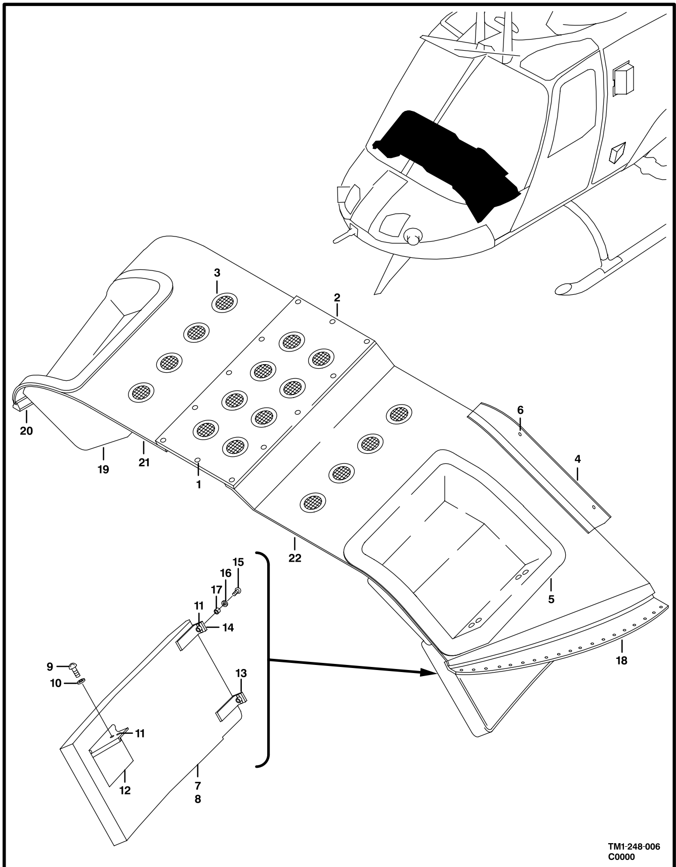
Figure 6. Shroud Installation
