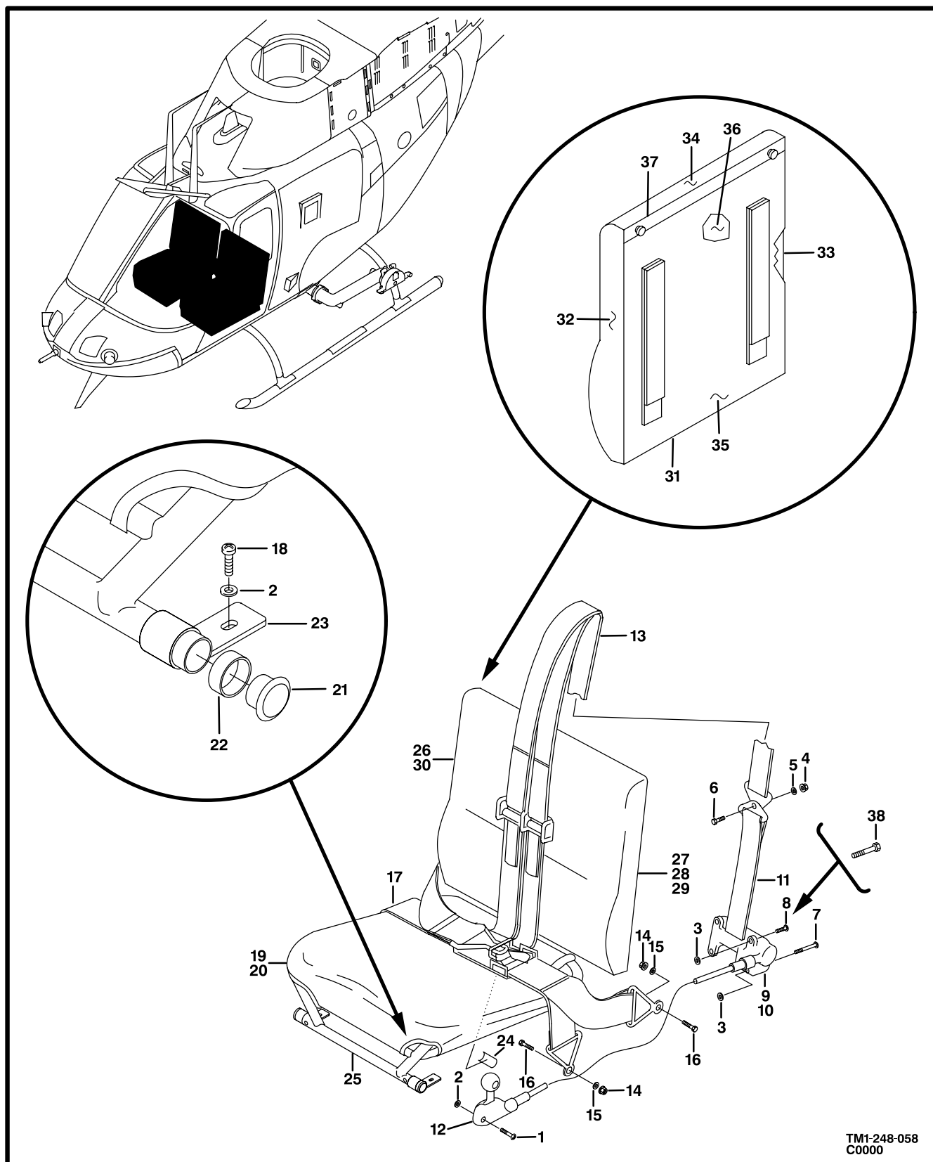
Figure 57. Seat and Restraint Assembly (Sheet 1 of 2)
