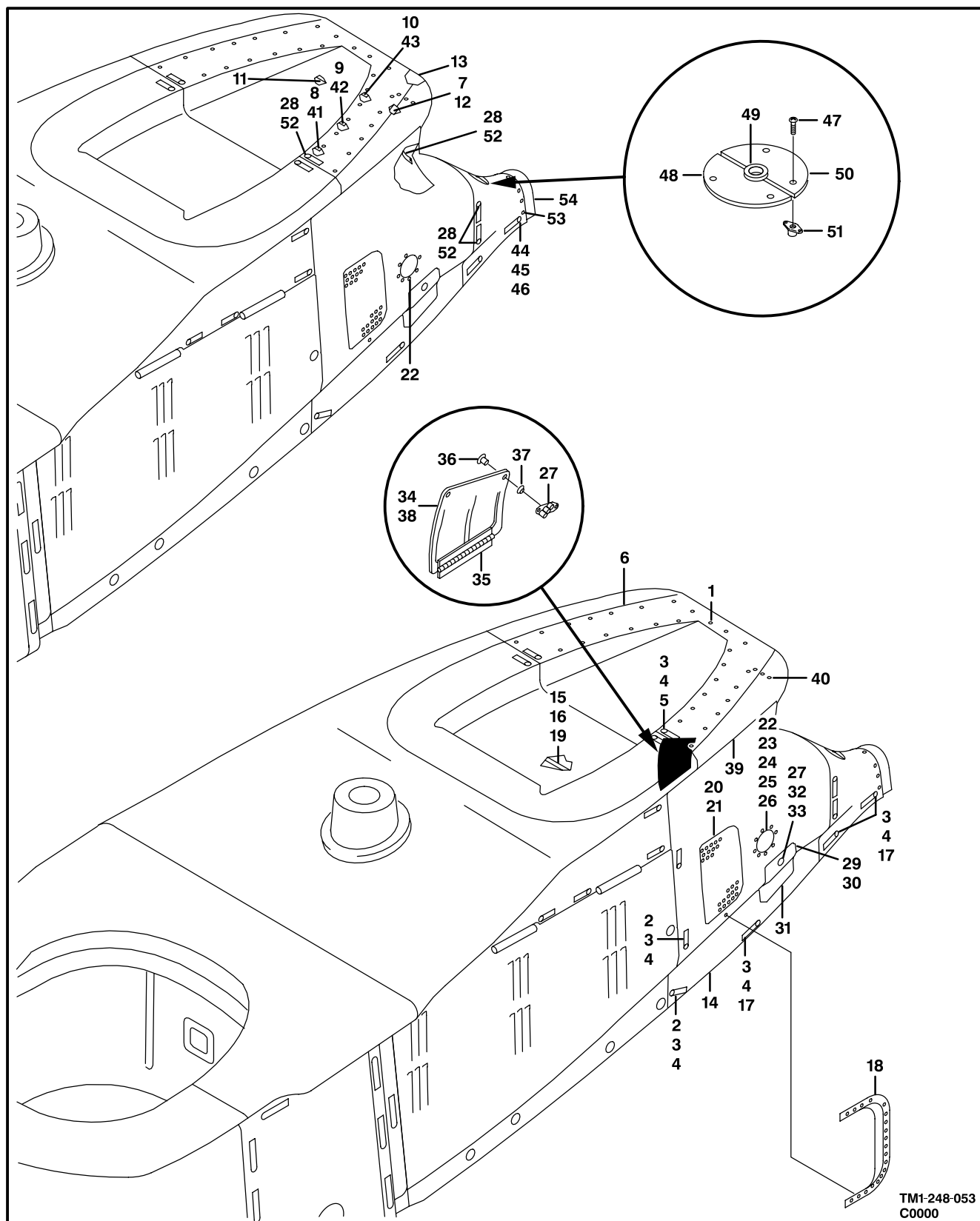
Figure 52. Fairing Assembly,AFT
