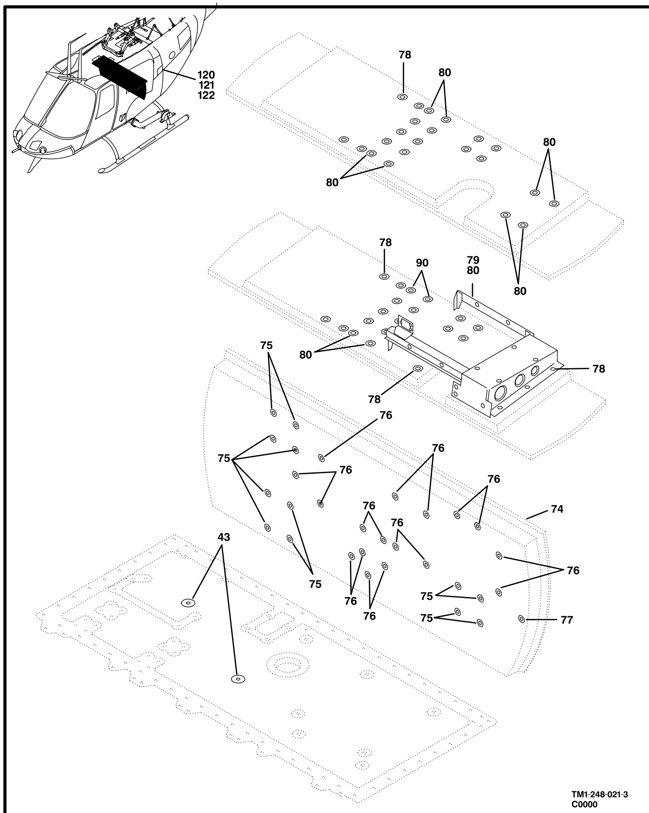
Figure 21. MOD-Fuel Cavity (Sheet 3 of 4)
