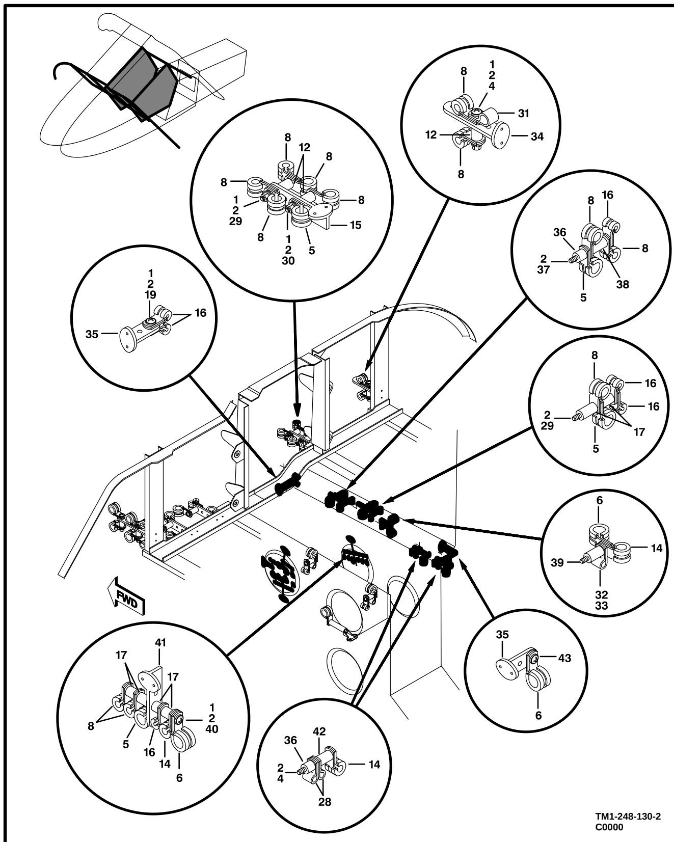
Figure 125. Electrical Installation,Nose (Sheet 2 of 2)
