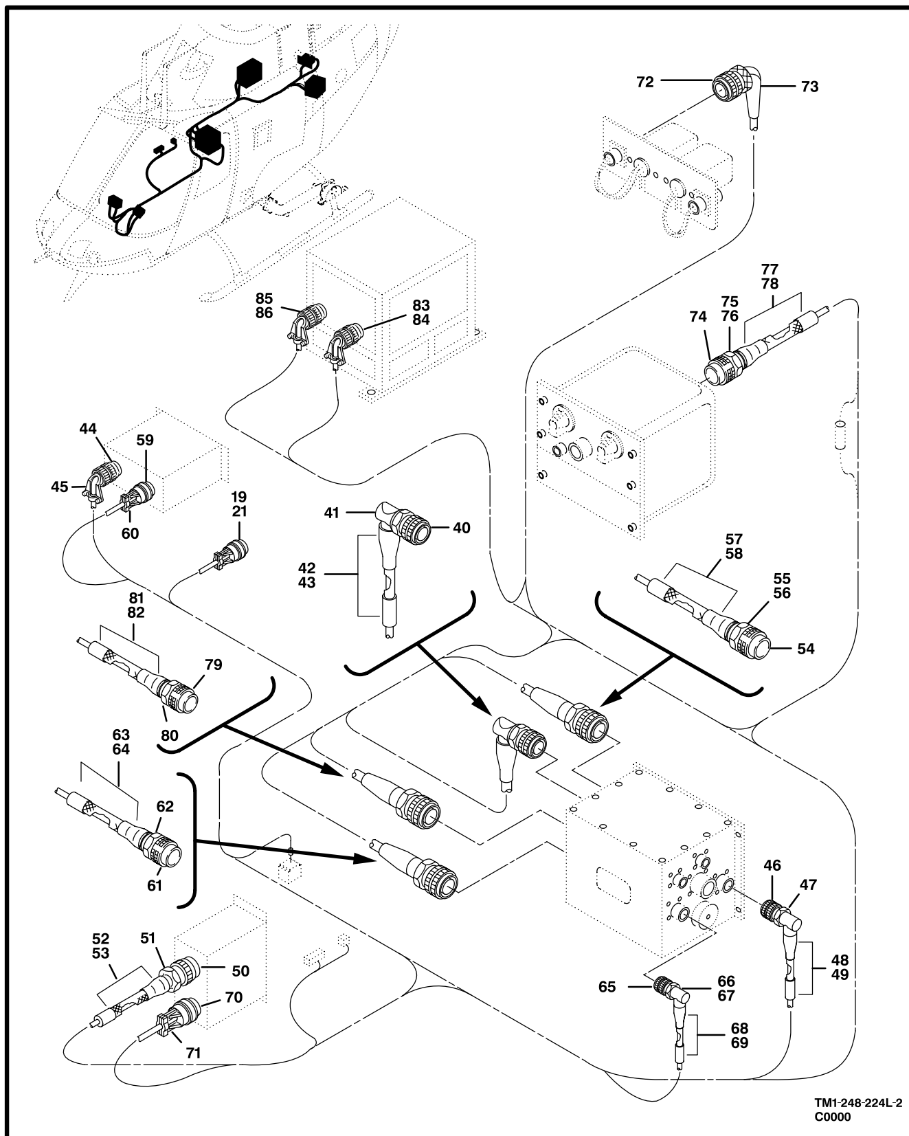
Figure 230. Cable Assembly, Intercom and ATH System (Sheet 2 of 2)
