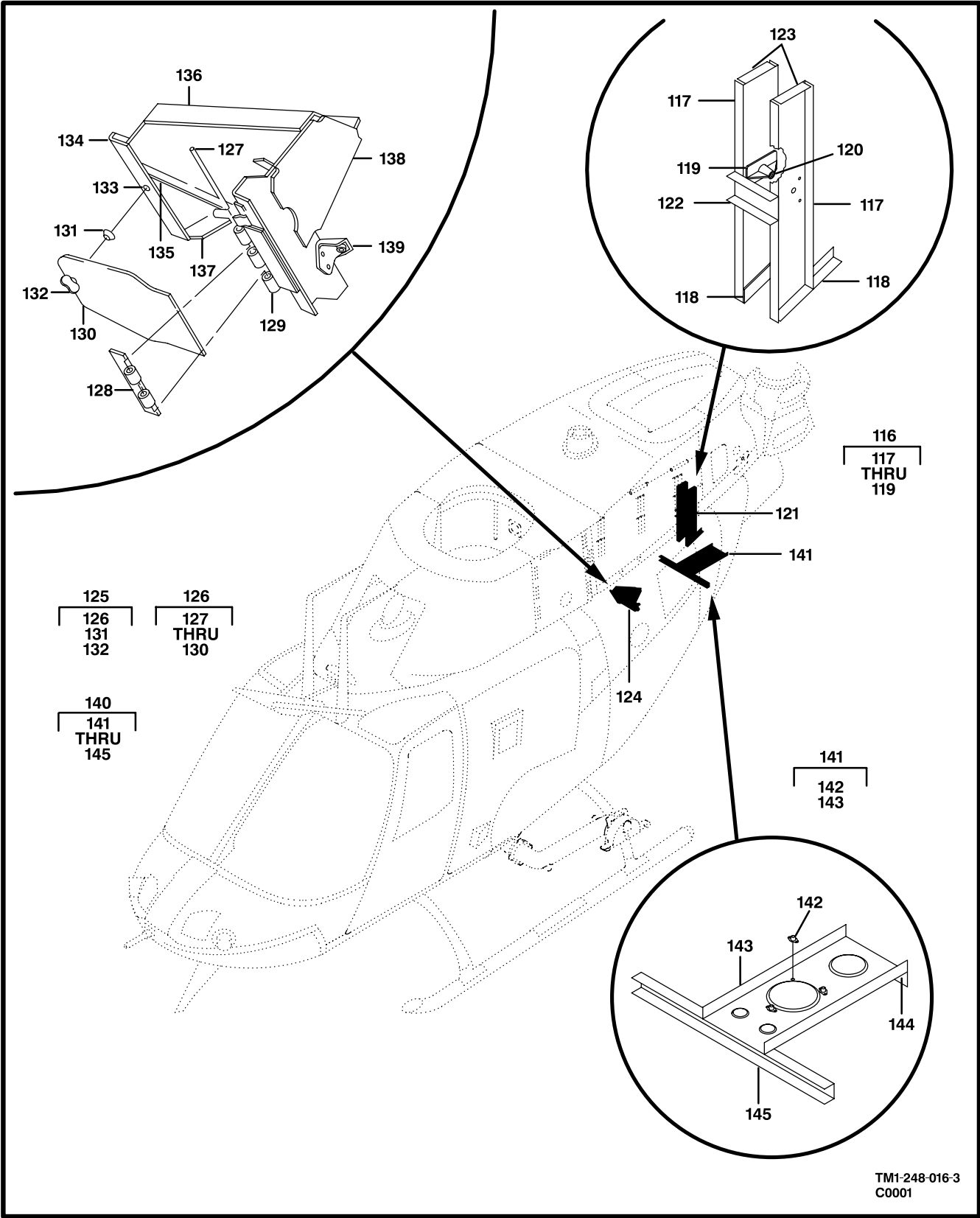
Figure 16. MOD-Roof,AFT (Sheet 3 of 4)
