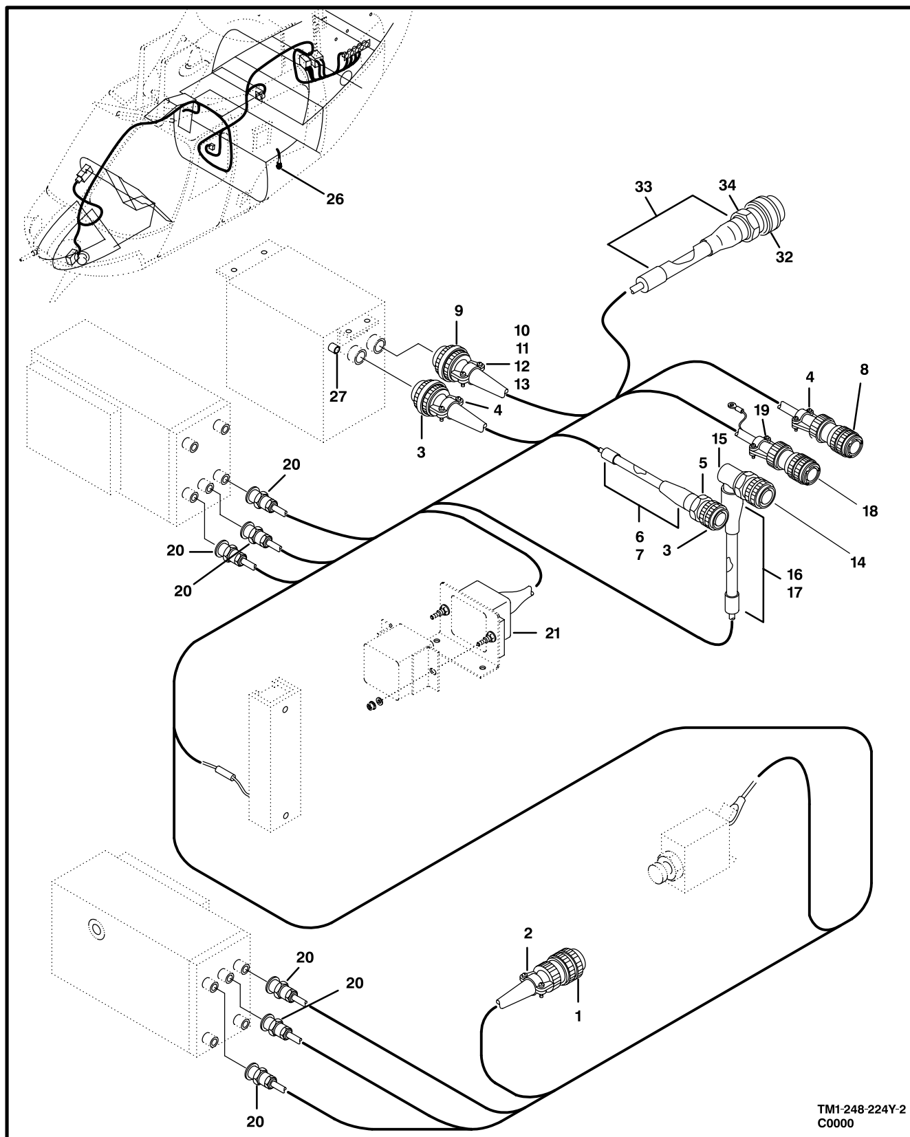
Figure 242. Cable Assembly, Laser and Radar Warning System (Sheet 2 of 2)
