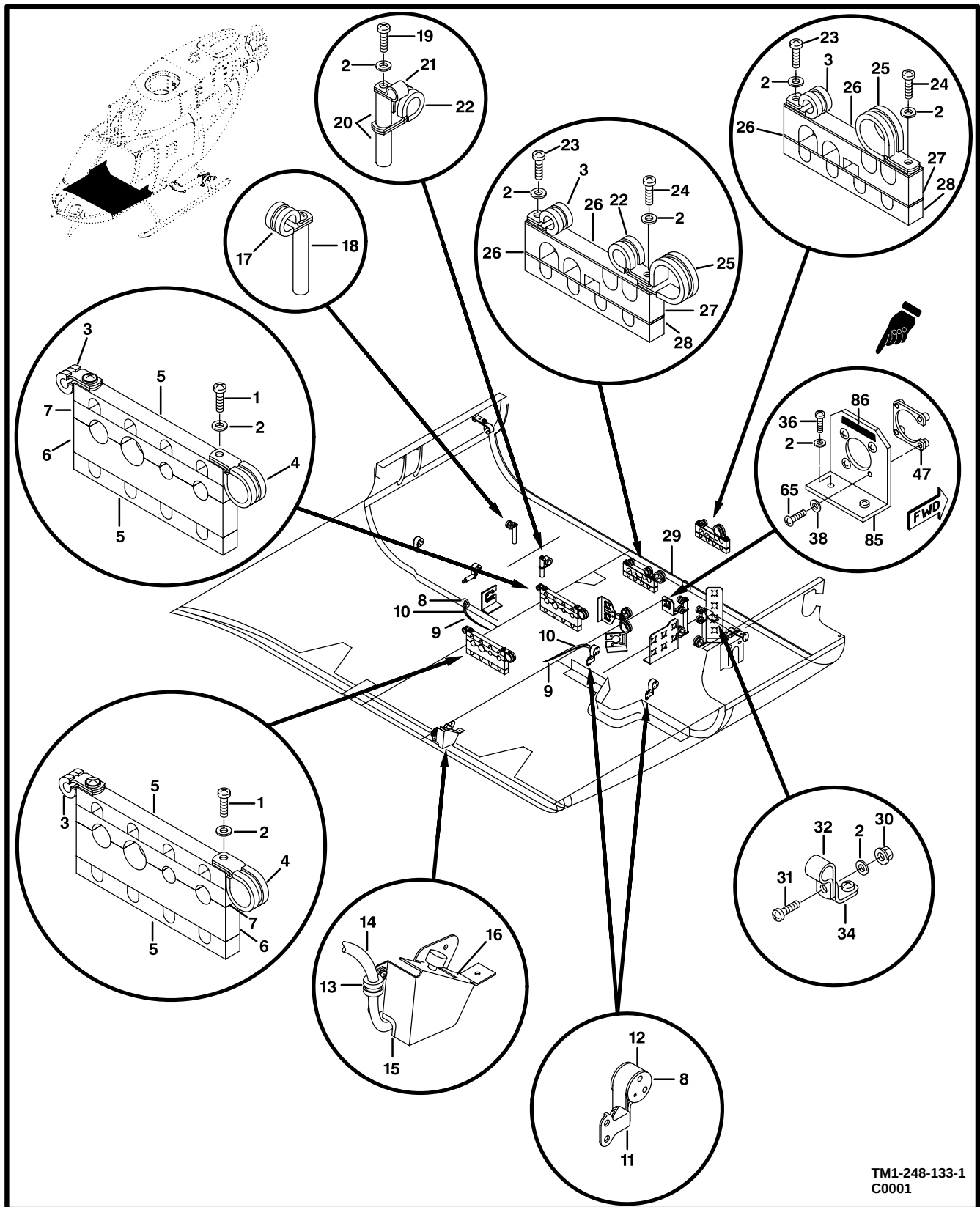
Figure 128. Electrical Installation, Shell (Sheet 1 of 2)
