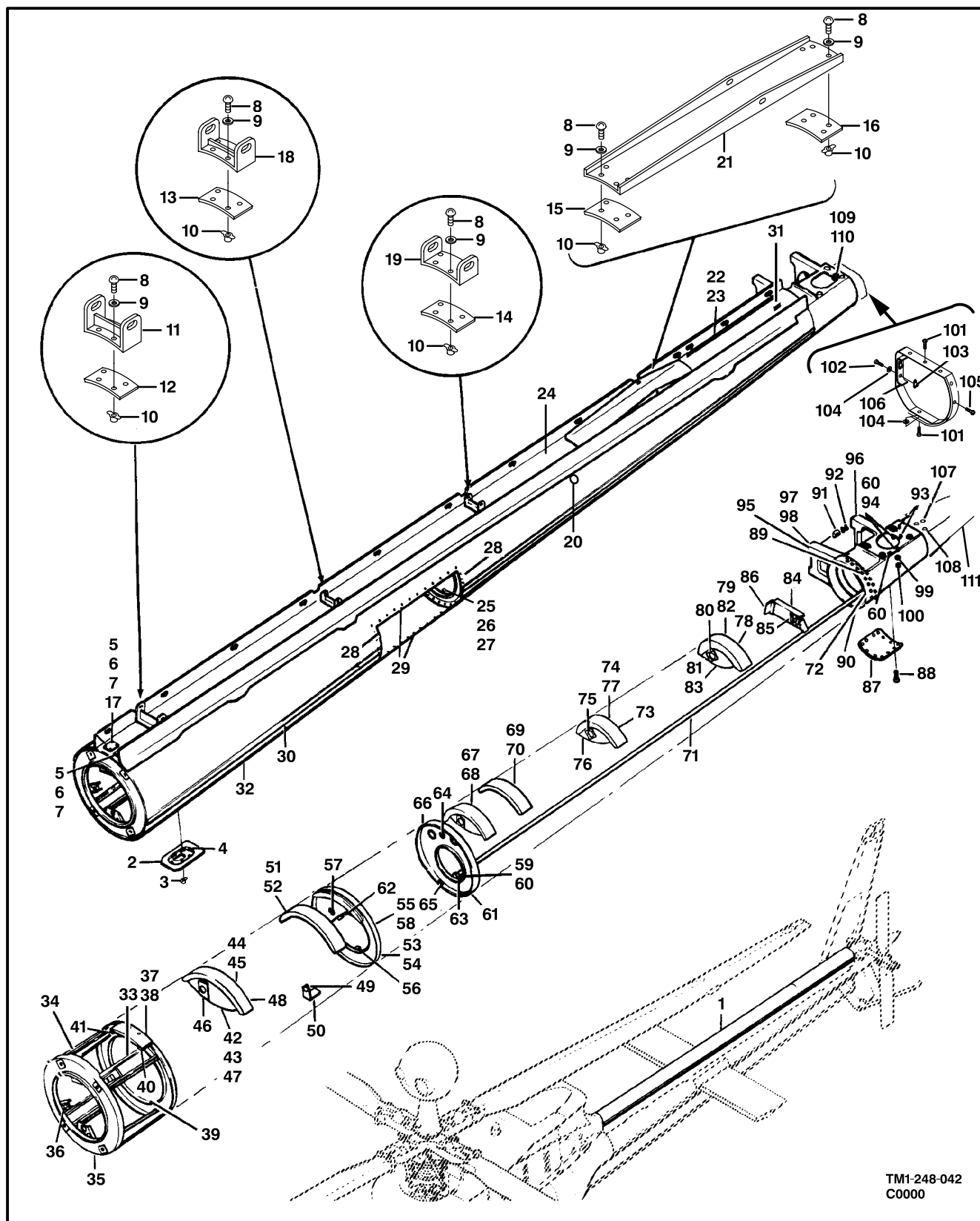
Figure 41. Tailboom Installation
