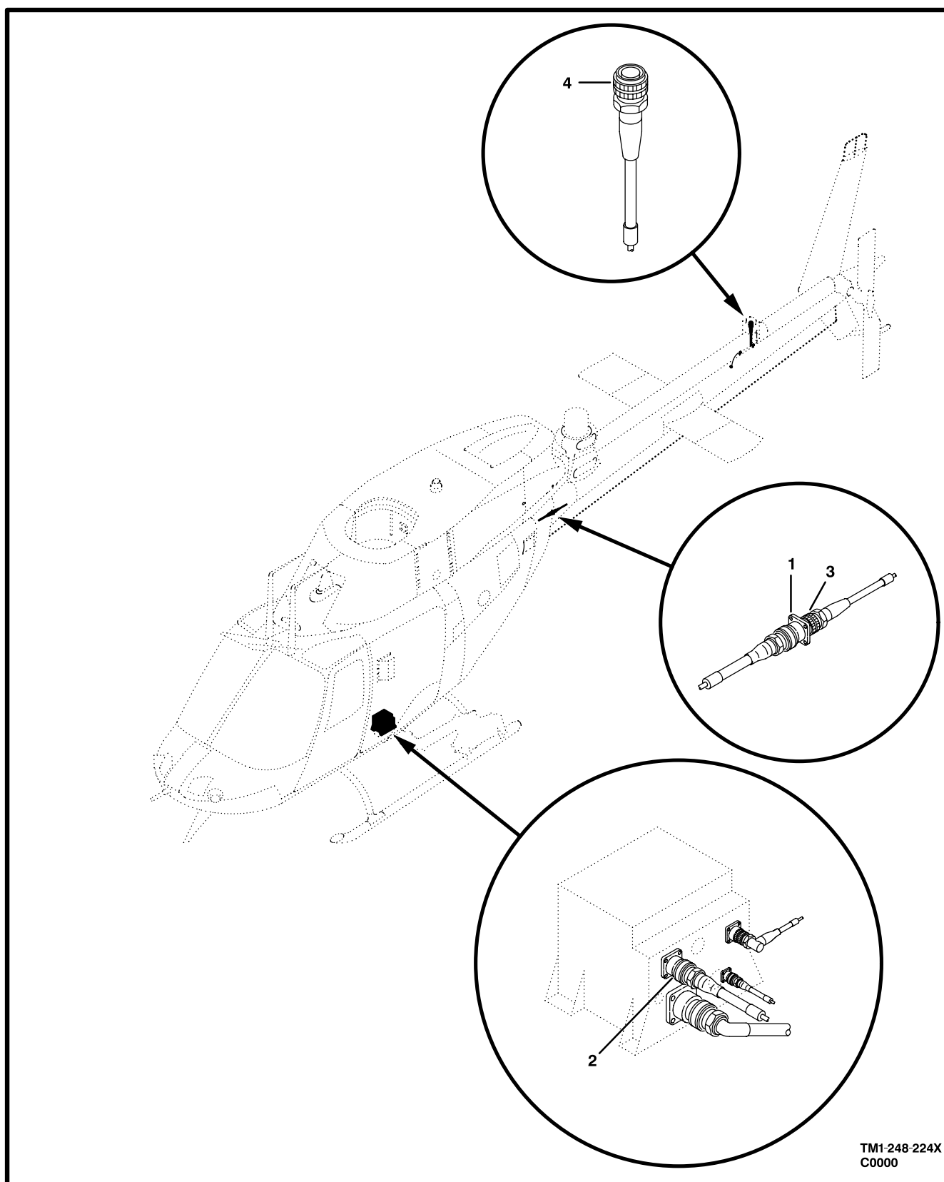
Figure 241. Cable Assembly,EGI
