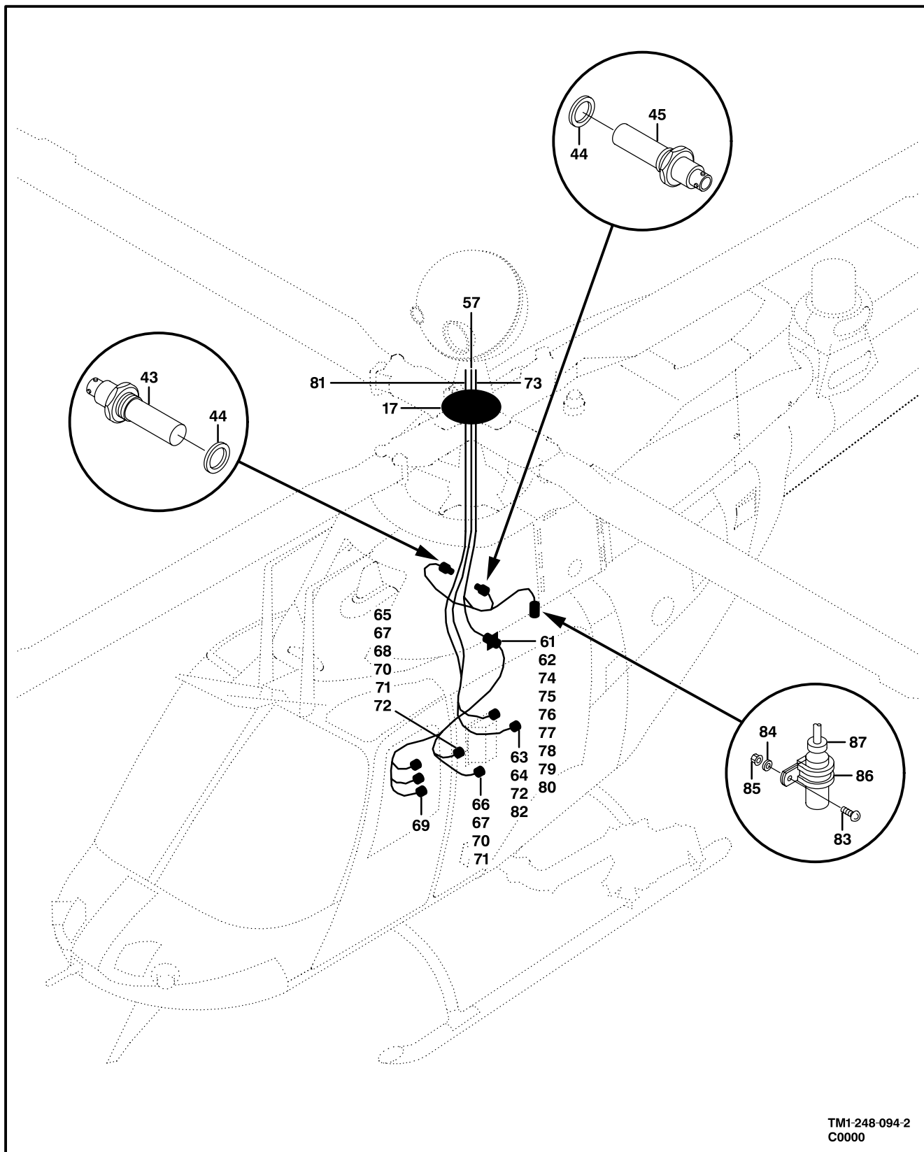
Figure 91. Torquemeter Installation (Sheet 2 of 2)
