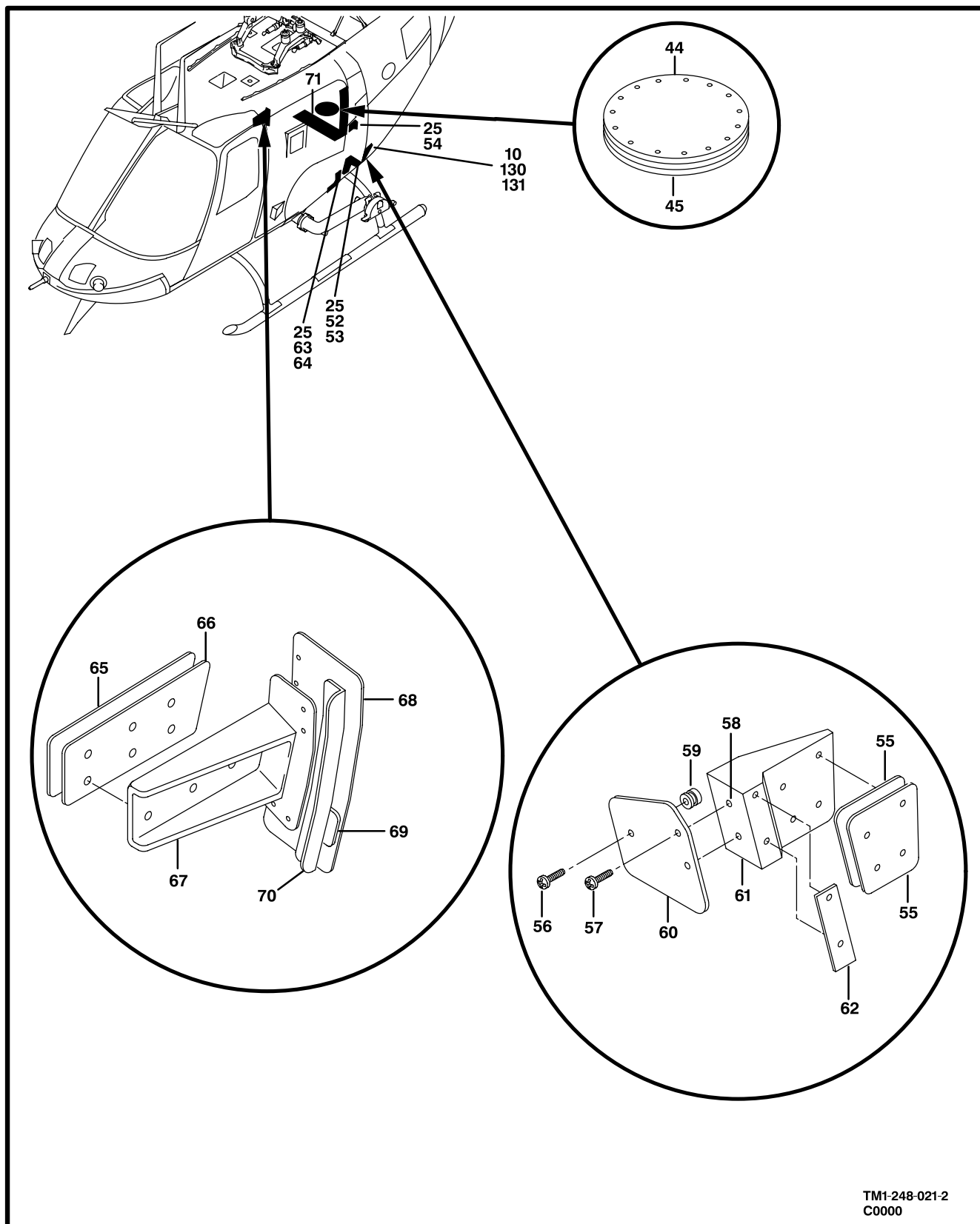
Figure 21. MOD-Fuel Cavity (Sheet 2 of 4)
