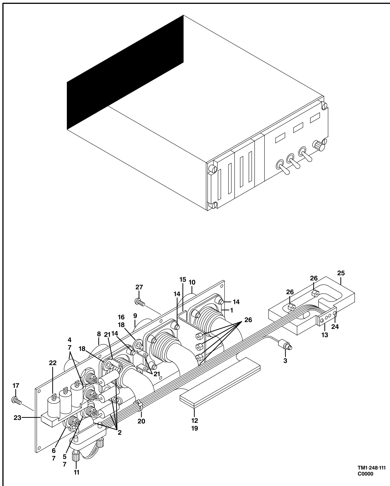
Figure 106. Plate,Rear Subassembly
