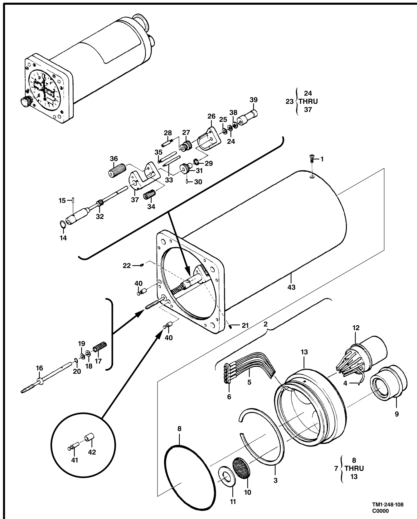
Figure 103. Case Assembly, 2 Inch Altimeter
