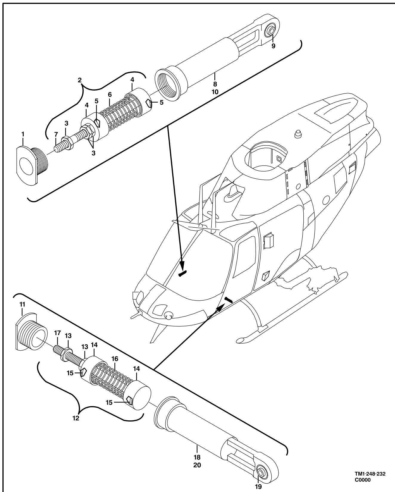
Figure 250. Force Gradient
