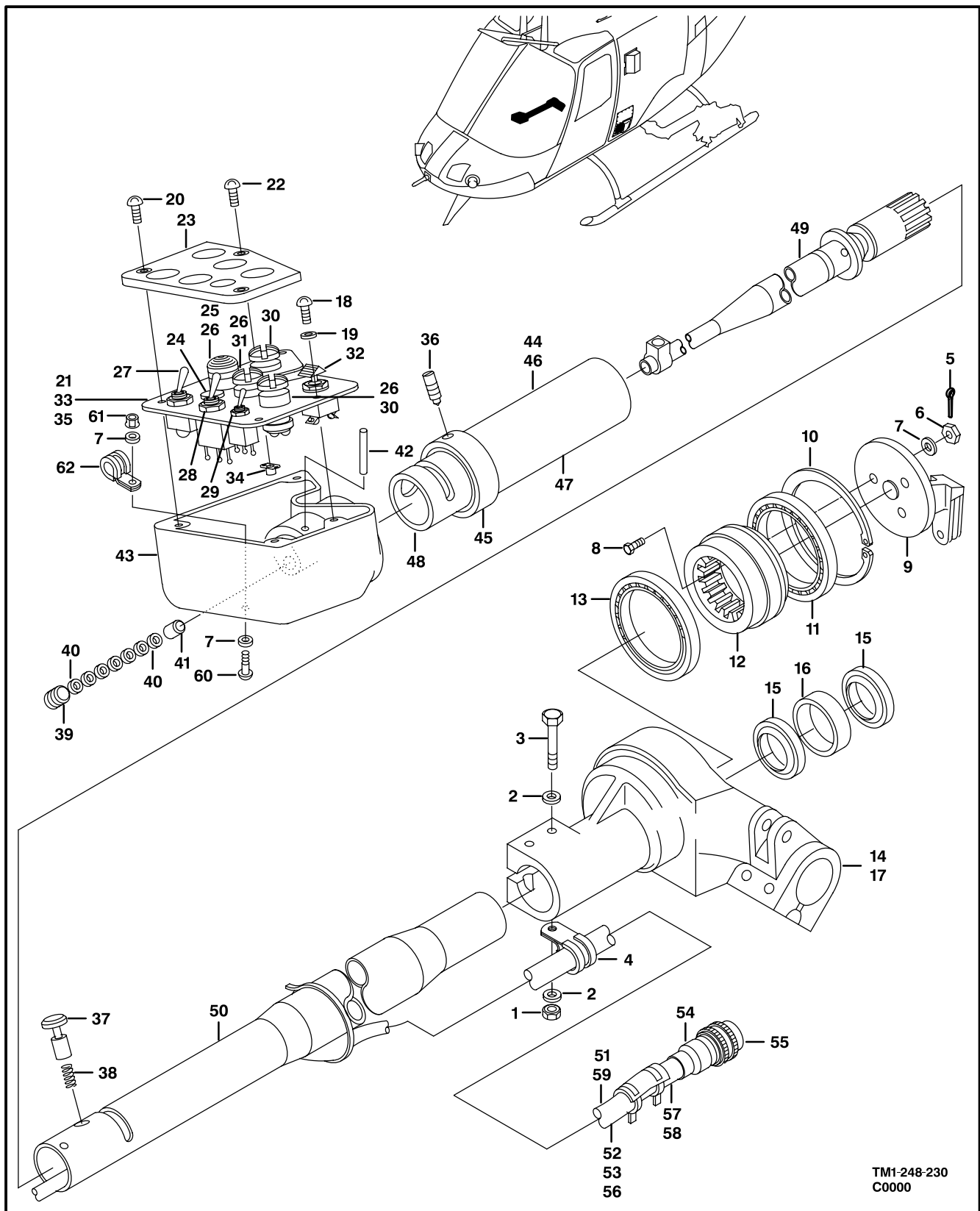
Figure 248. Stick Assembly, Pilot
