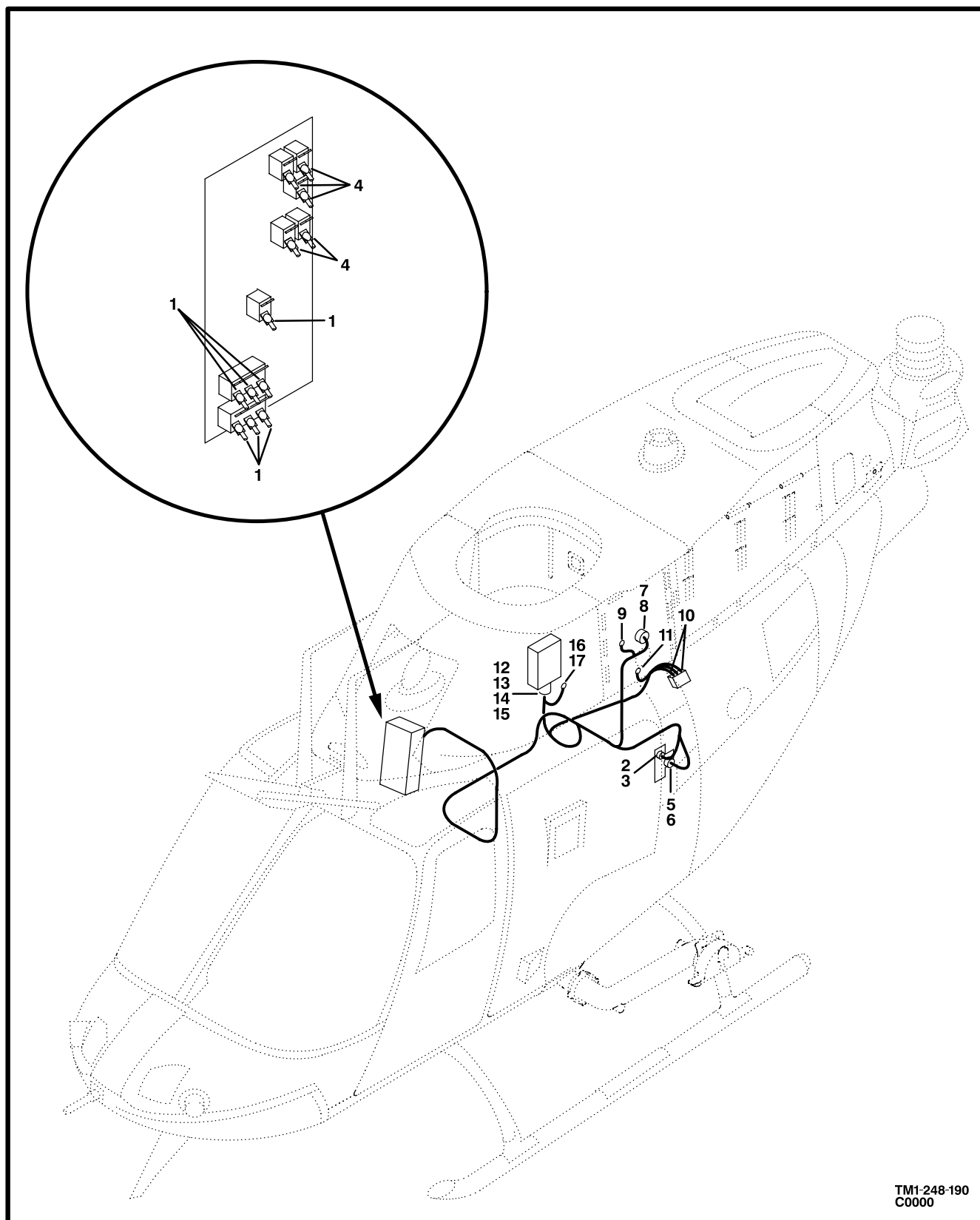
Figure 185. Cable Assembly, AC Power System
