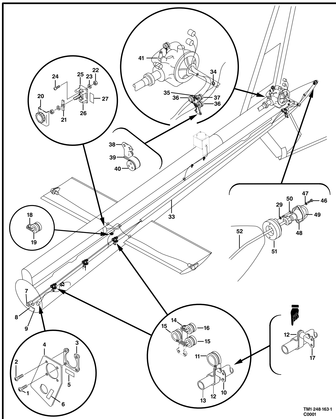
Figure 158. Electrical Installation, Tailboom (Sheet 1 of 2)
