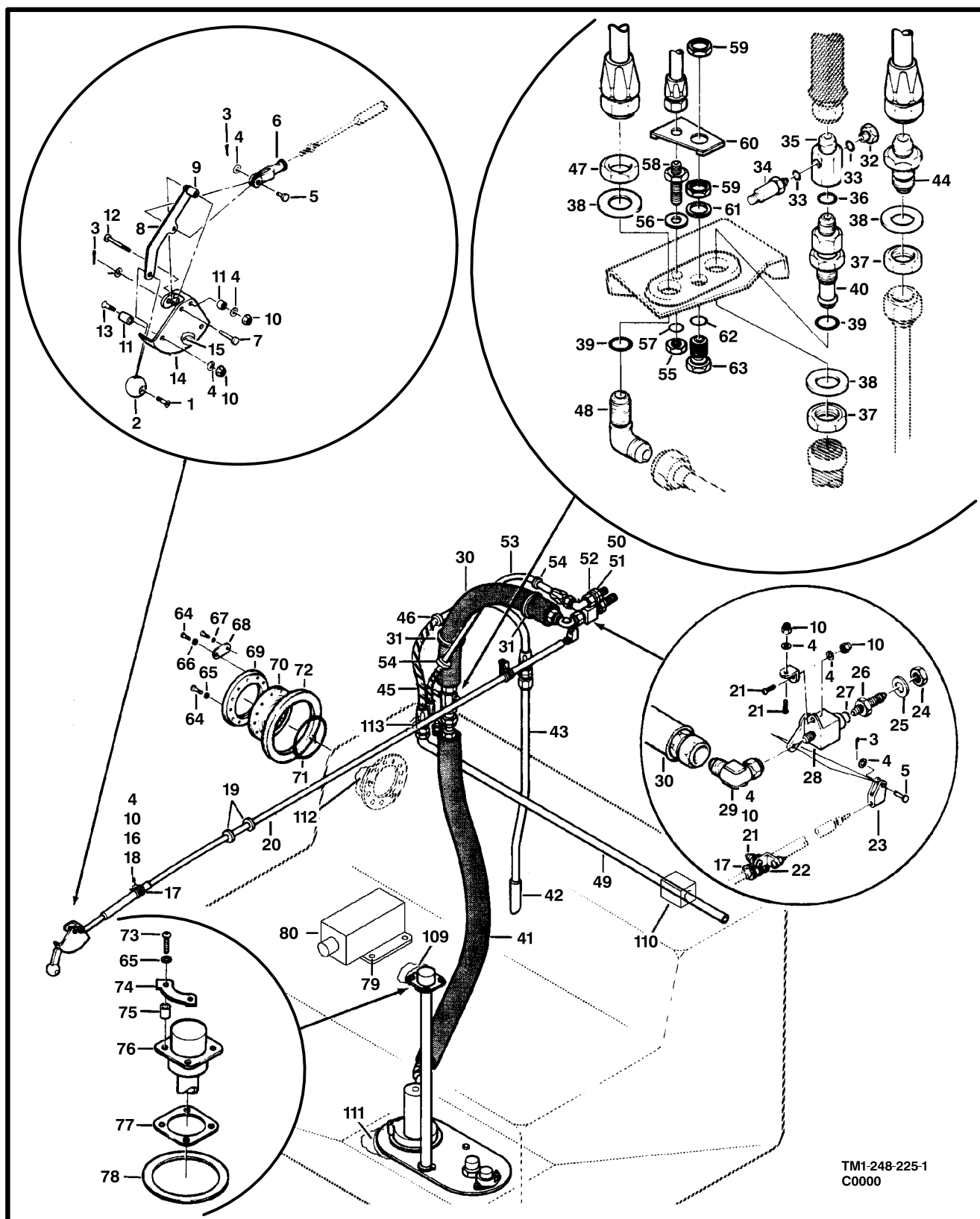
Figure 243. Fuel System Installation (Sheet 1 of 2)
