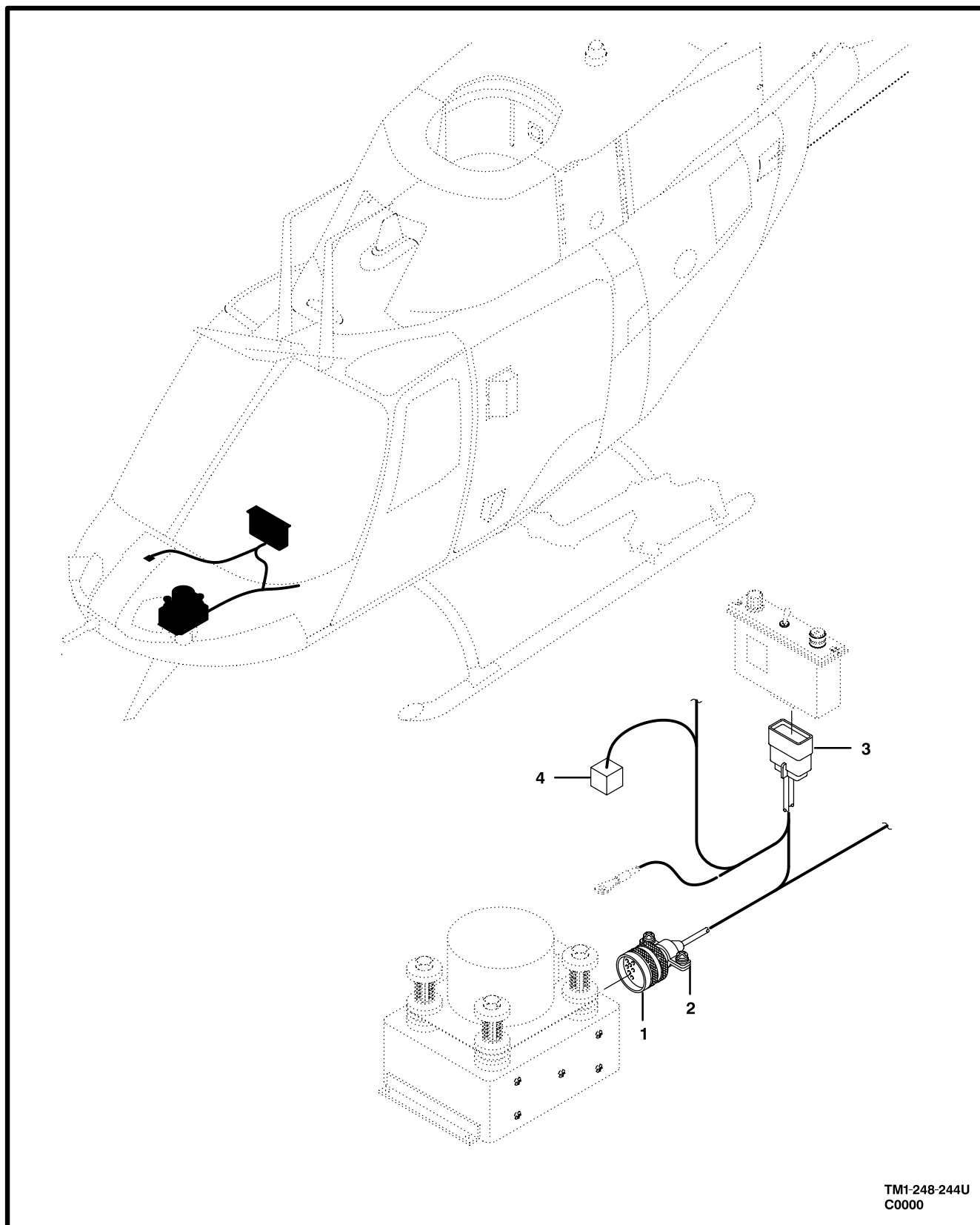
Figure 238. Cable Assembly, Directional Gyro
