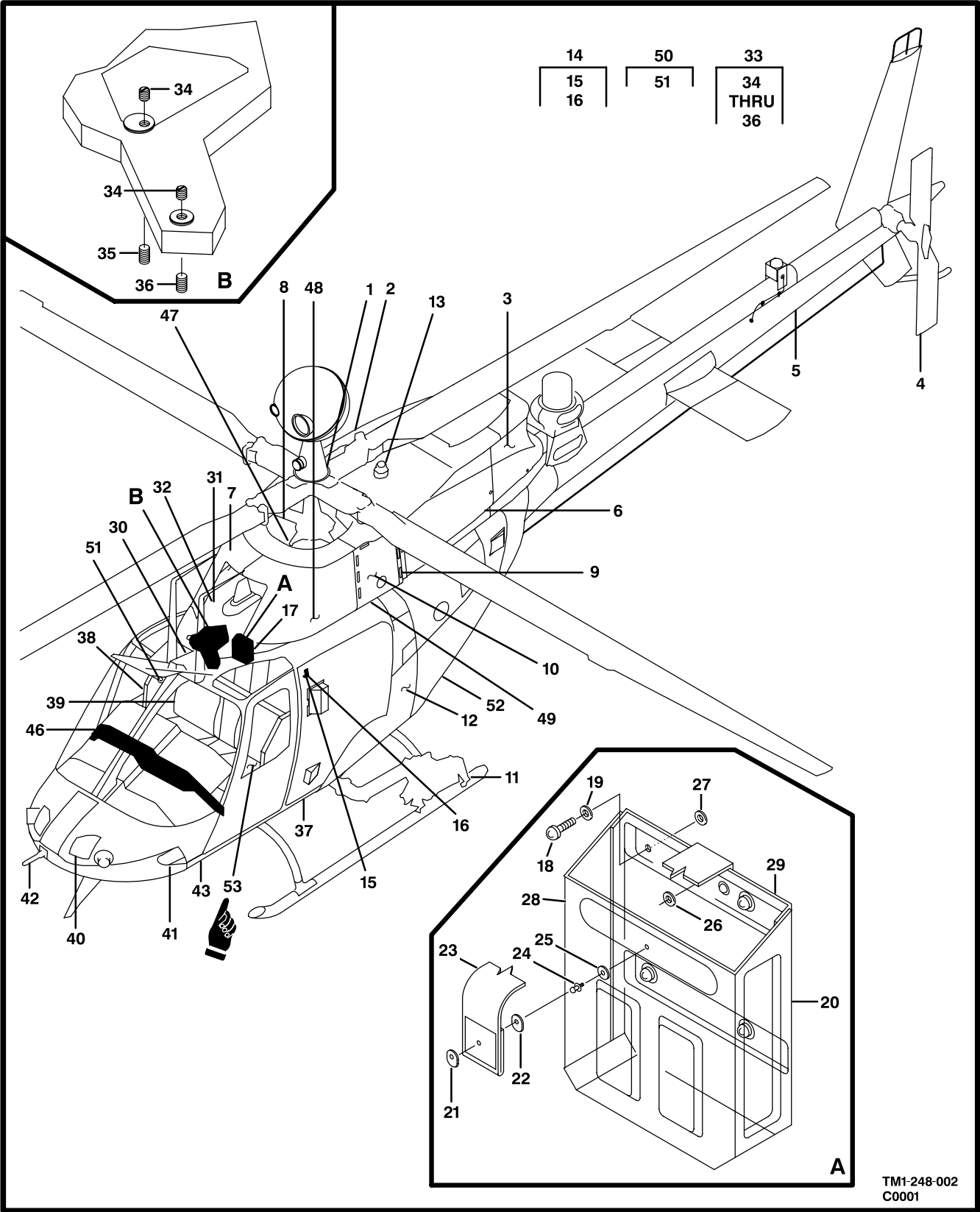
Figure 2. Helicopter Assembly
