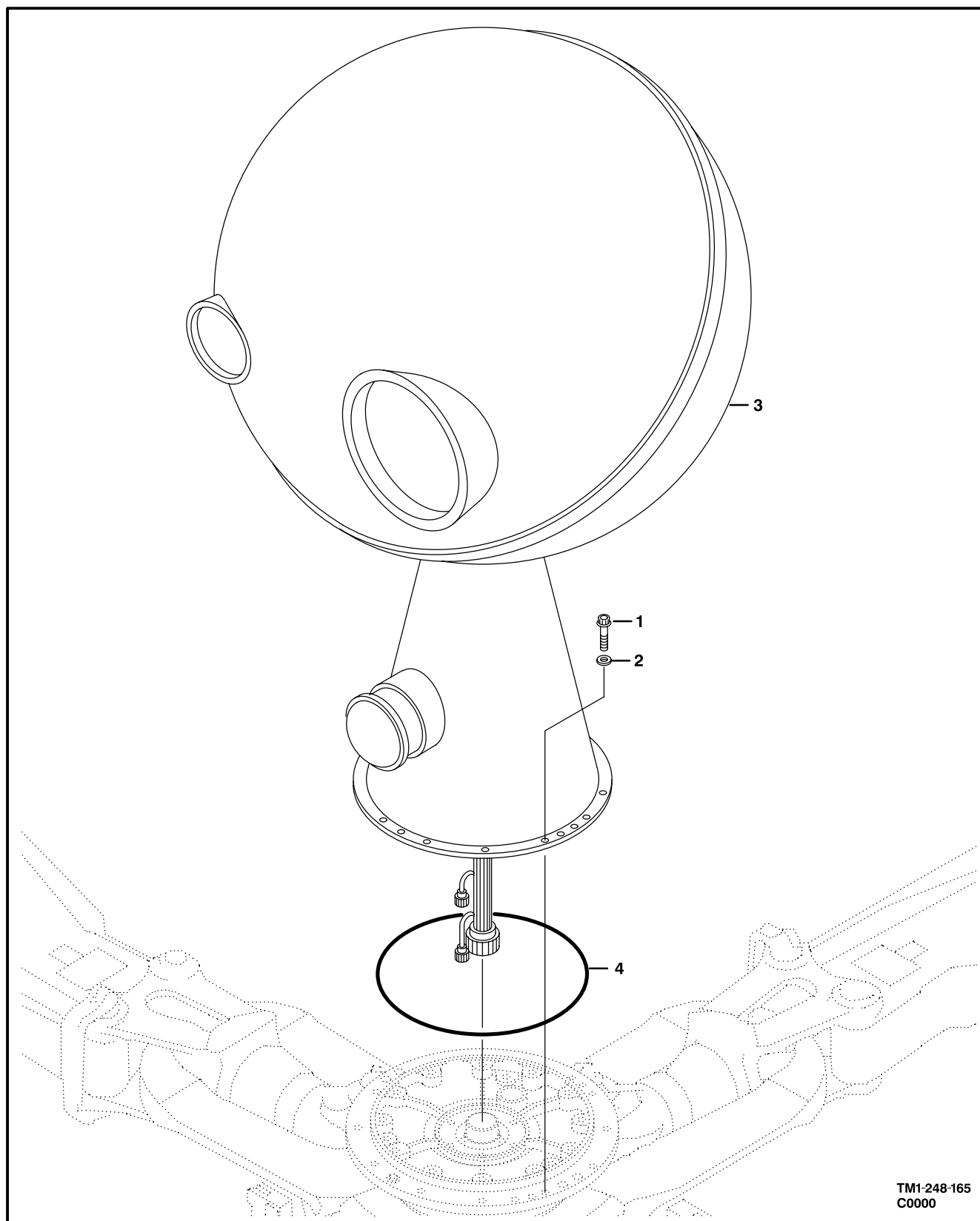
Figure 160. Electrical Installation, Mast Mounted Sight
