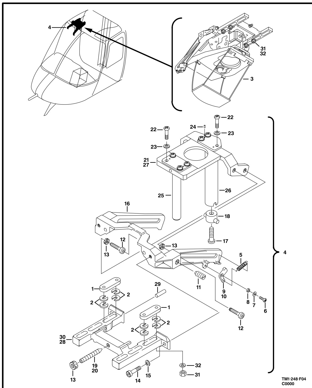
Figure F4. Missile Sight Subsystem Installation
