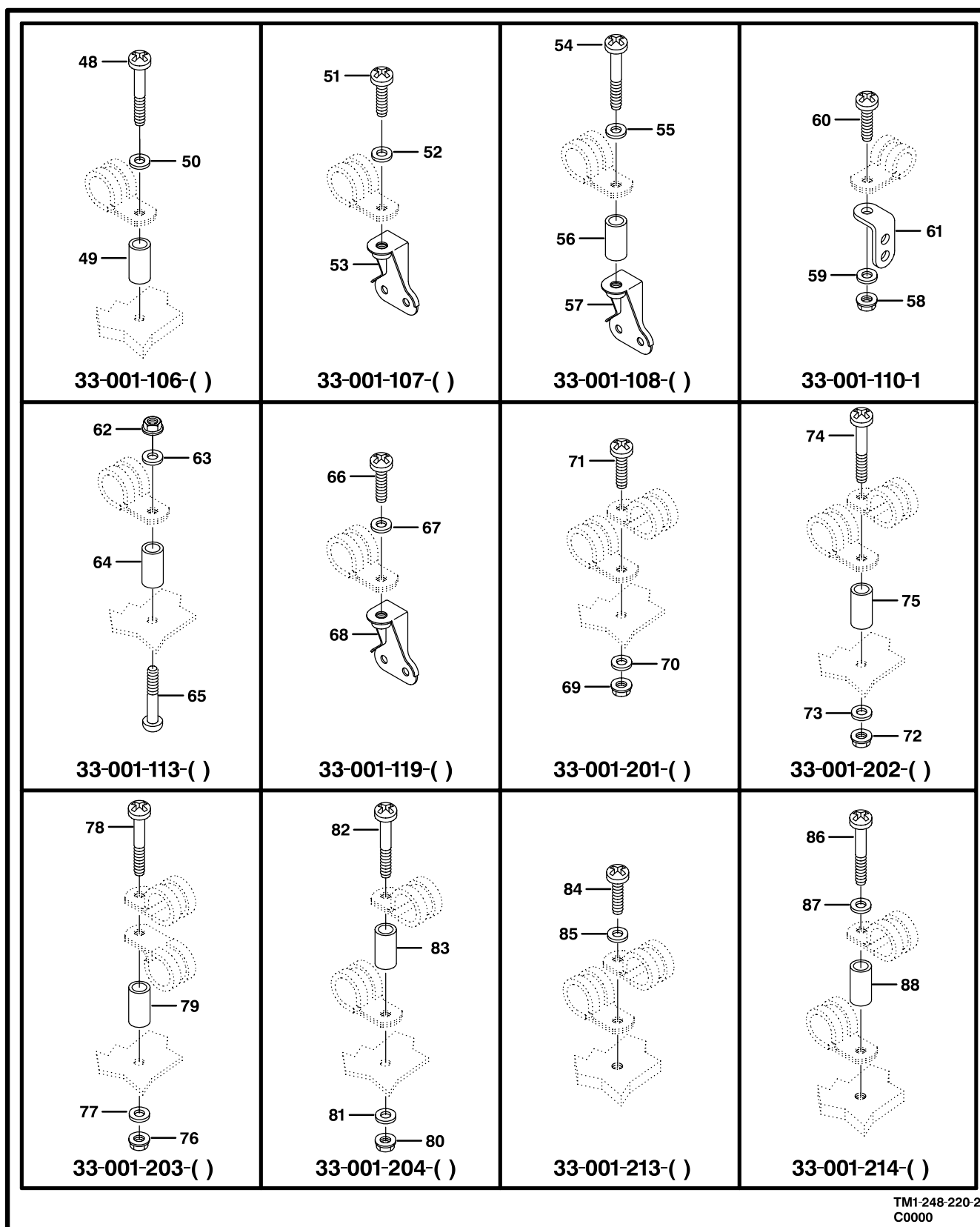
Figure 215. Support Installations (Sheet 2 of 5)
