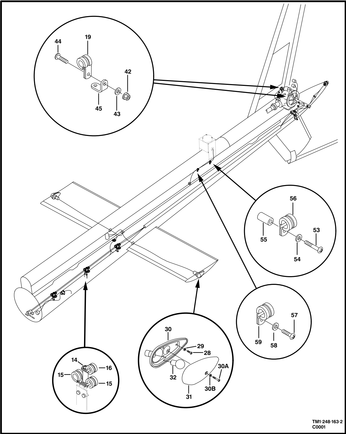
Figure 158. Electrical Installation,Tailboom (Sheet 2 of 2)
