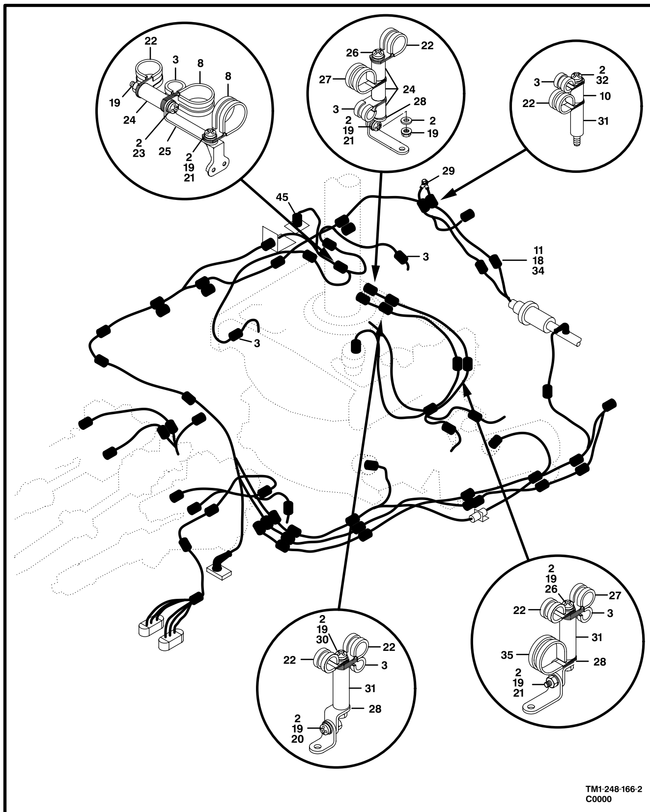
Figure 161. Electrical Installation, Mast Mounted Sight (Sheet 2 of 6)
