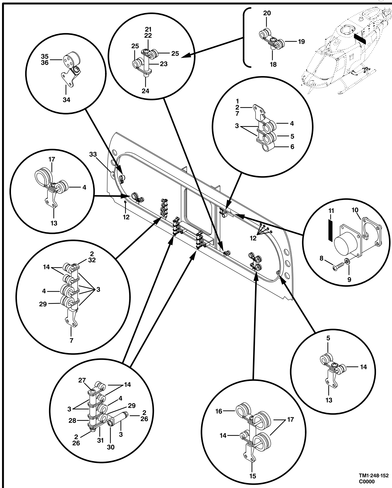
Figure 147. Electrical Installation,Bulkhead
