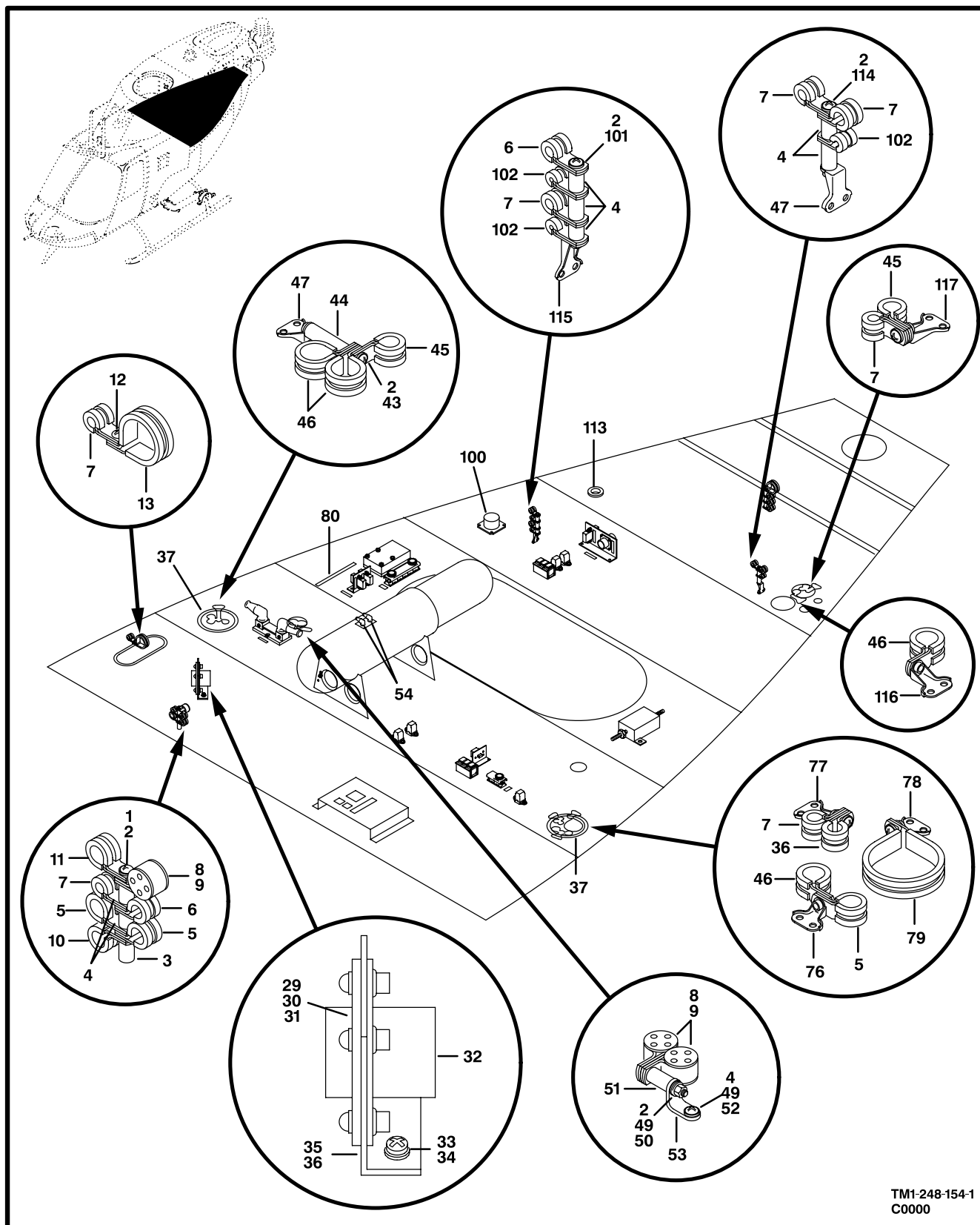
Figure 149. Electrical Installation, Canted Web (Sheet 1 of 2)
