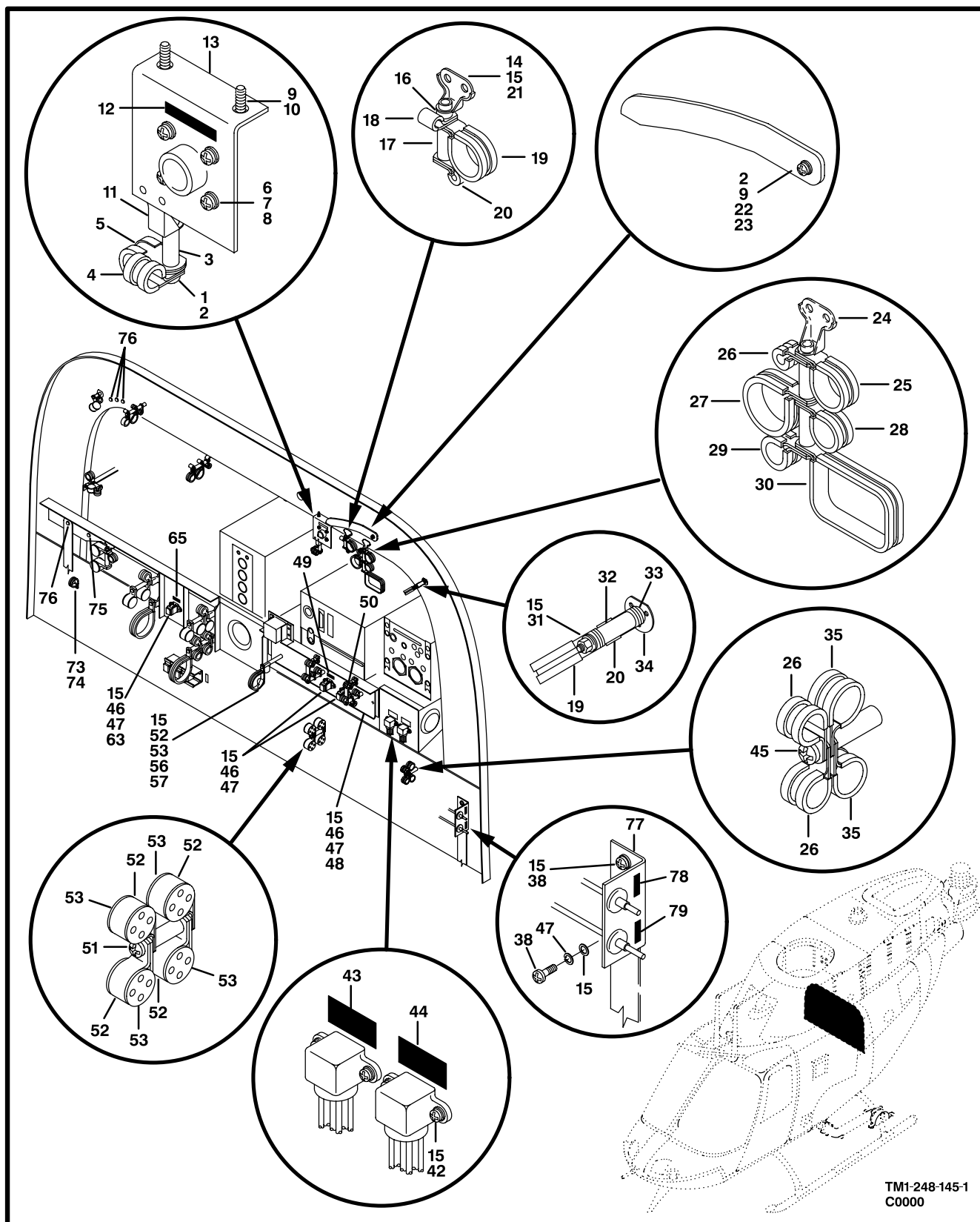
Figure 140. Electrical Installation, Bulkhead (Sheet 1 of 3)
