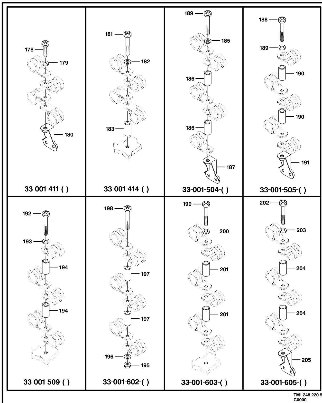
Figure 215. Support Installations (Sheet 5 of 5)
