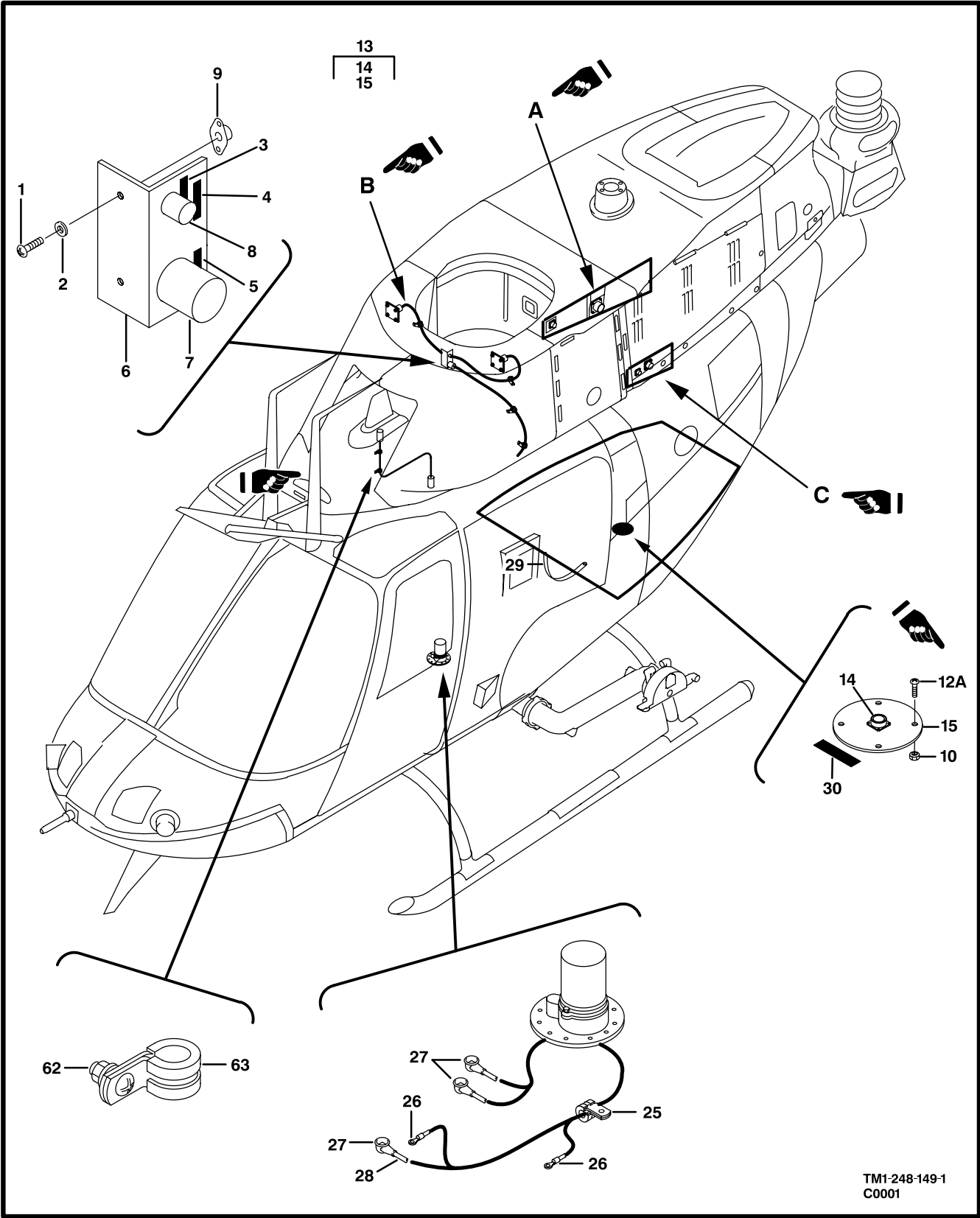
Figure 144. Electrical Installation (Sheet 1 of 2)
