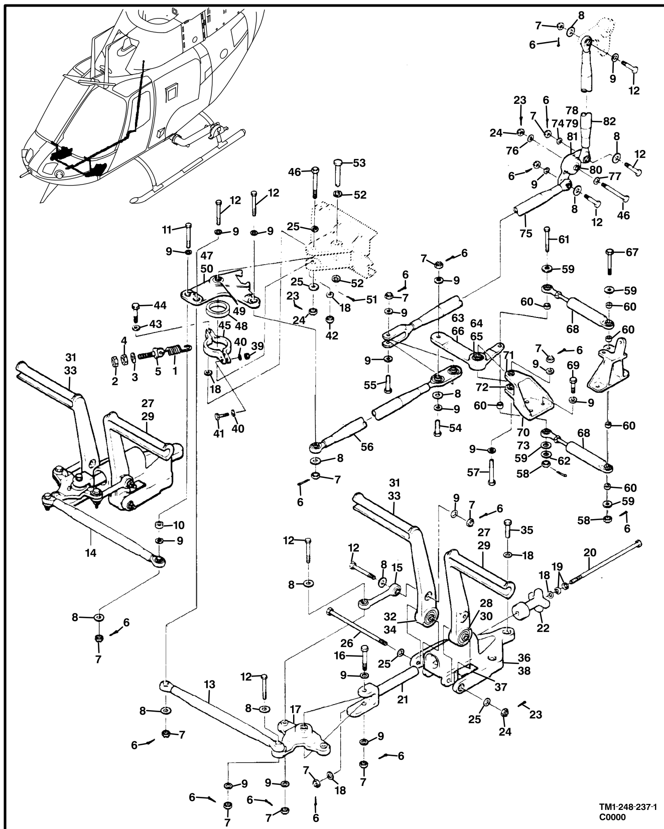
Figure 255. Controls Installation, Directional (Sheet 1 of 2)
