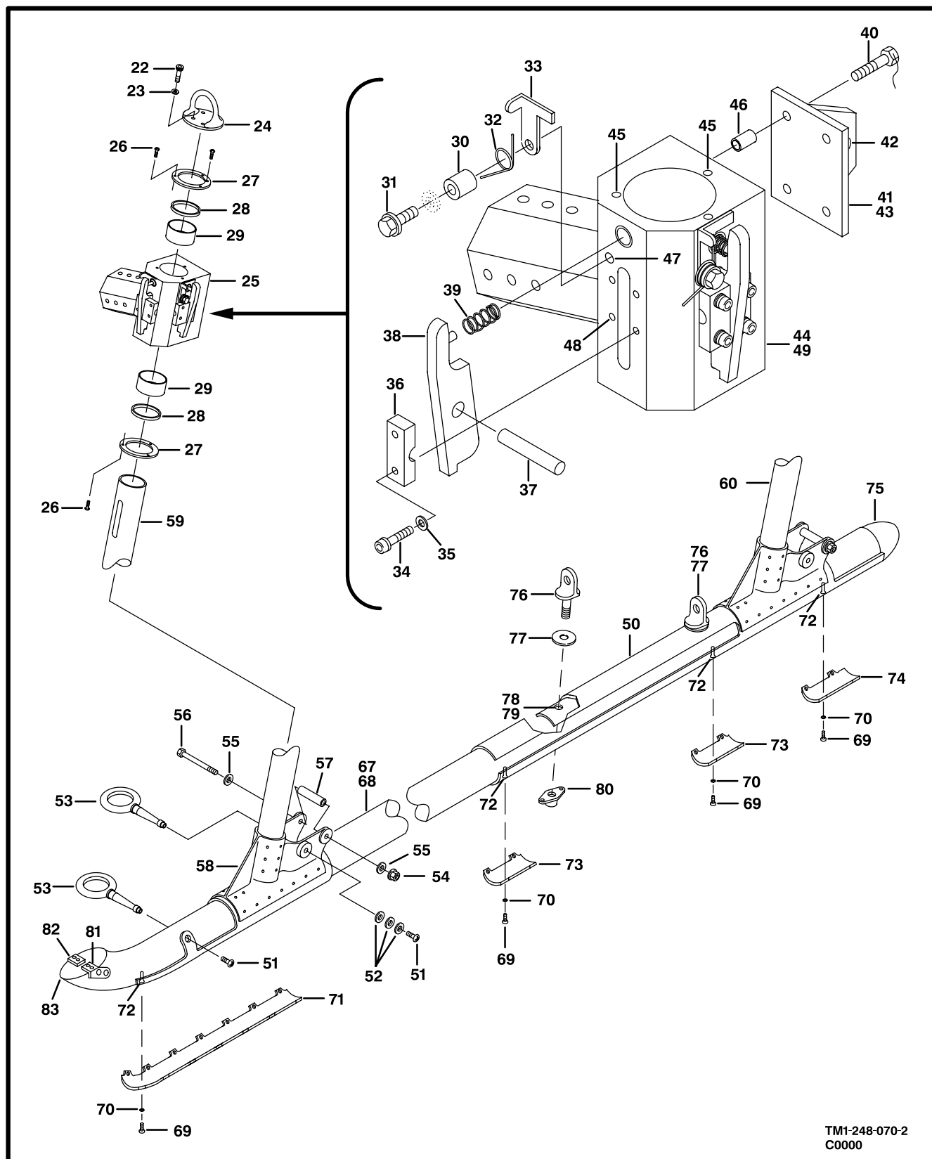
Figure 68. Landing Gear Installation (Sheet 2 of 2)
