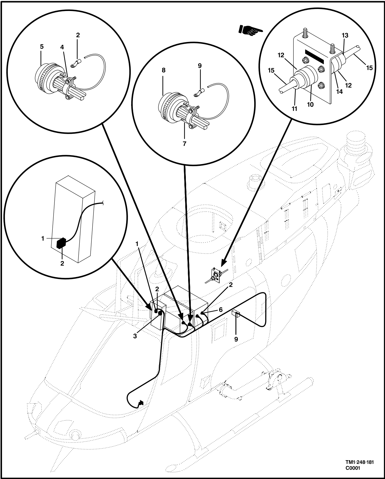
Figure 176. Cable Assembly,Mast Mounted Sight
