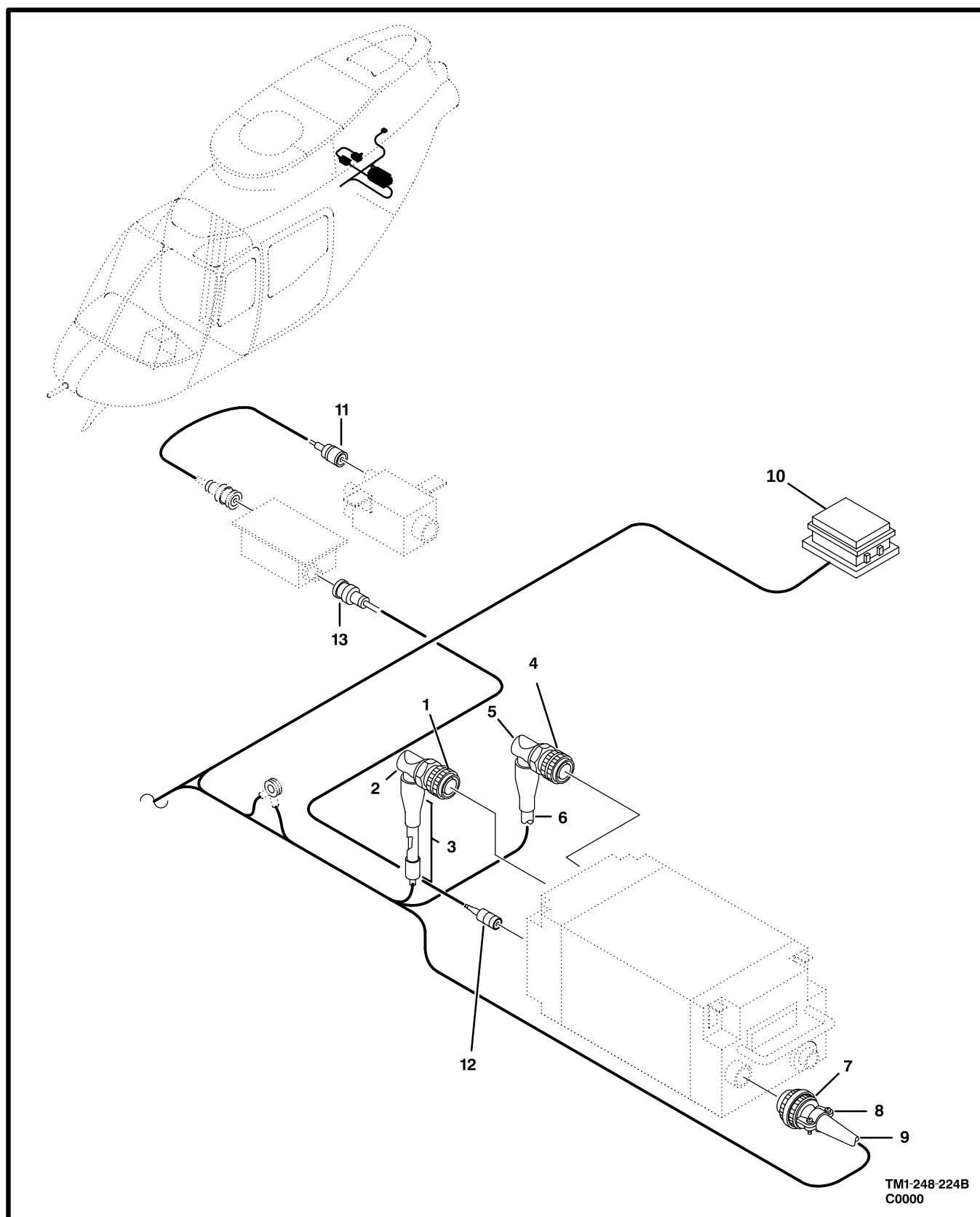
Figure 220. Cable Assembly, No. 2 VHF-FM Communication System
