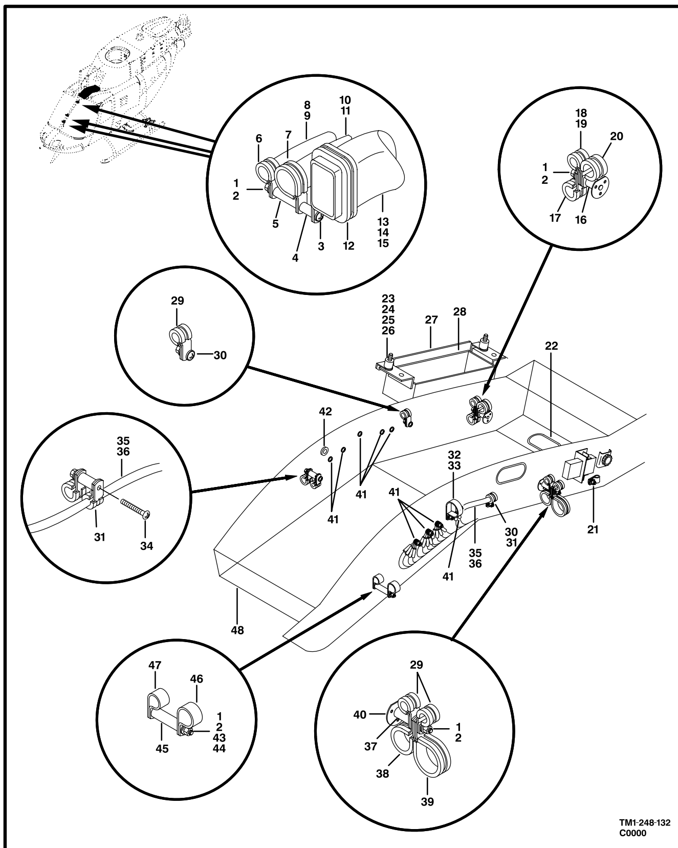
Figure 127. Electrical Installation, Console
