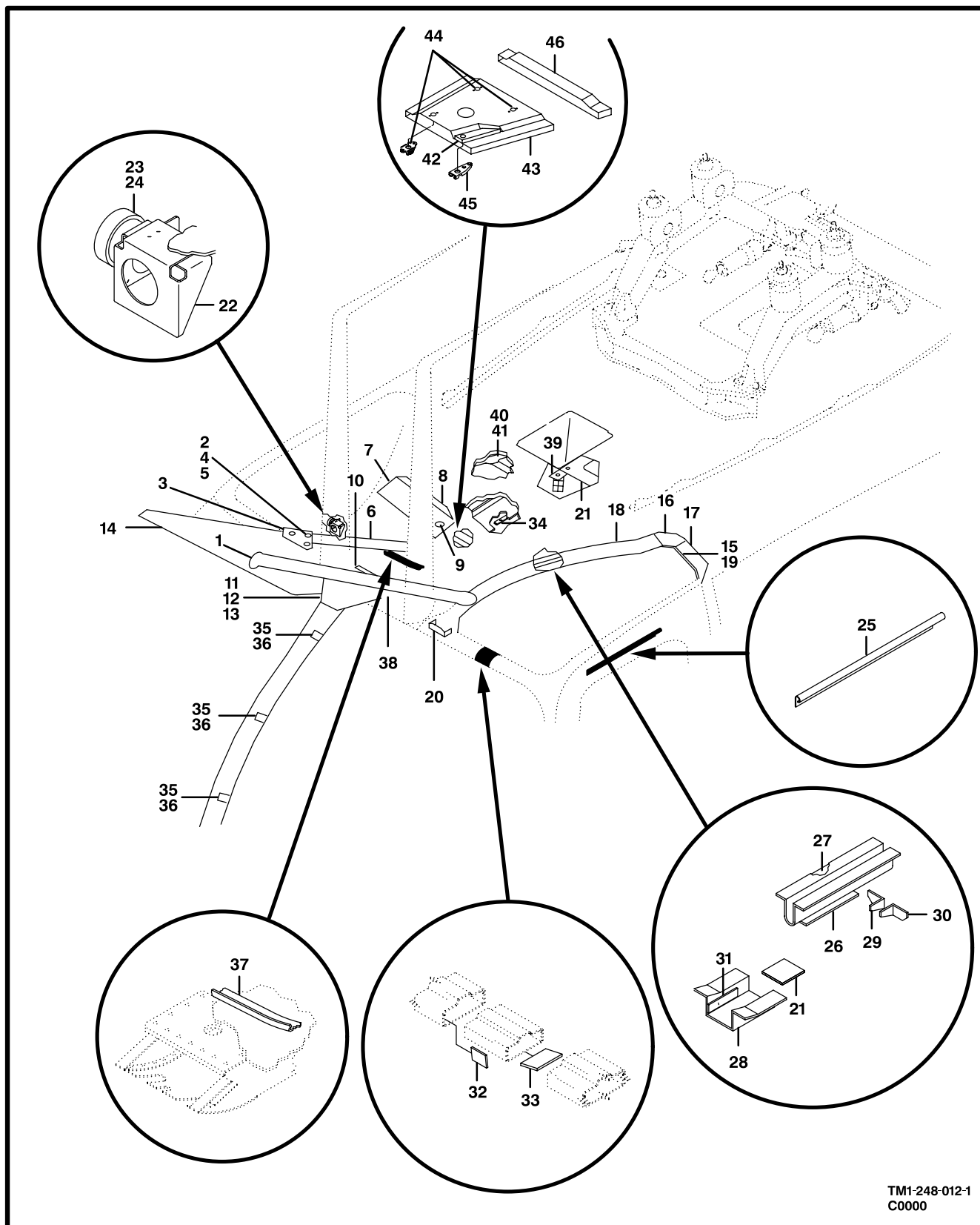
Figure 12. MOD-Roof,FWD (Sheet 1 of 2)
