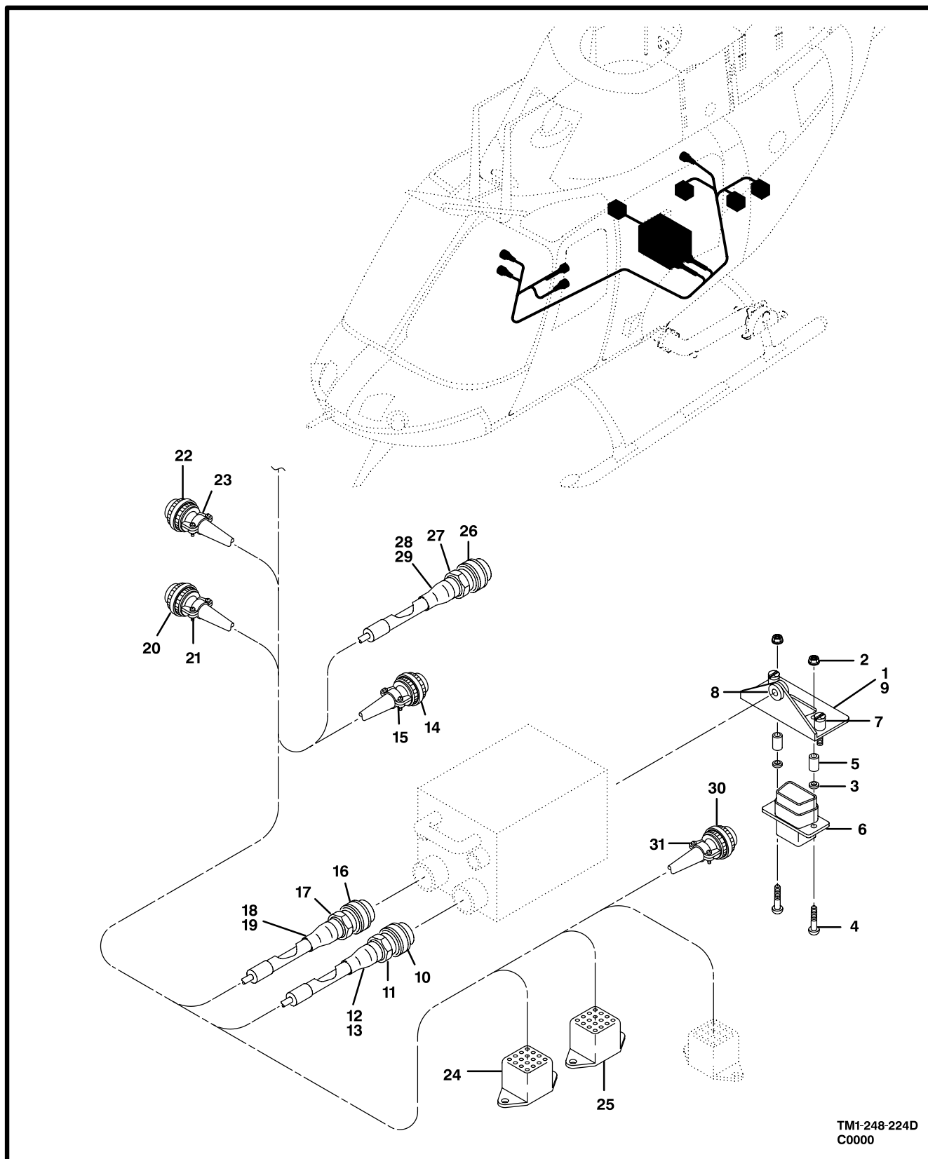
Figure 222. Cable Assembly, UHF-FM Communication System
