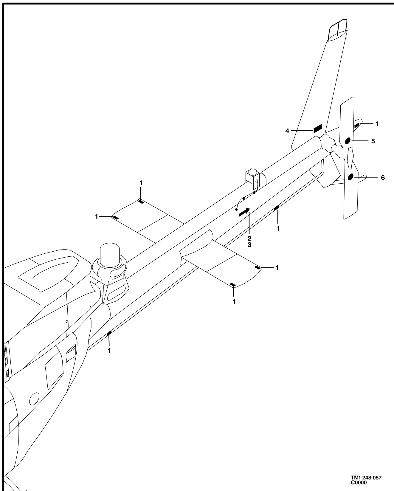
Figure 56. Markings Installation,AFT
