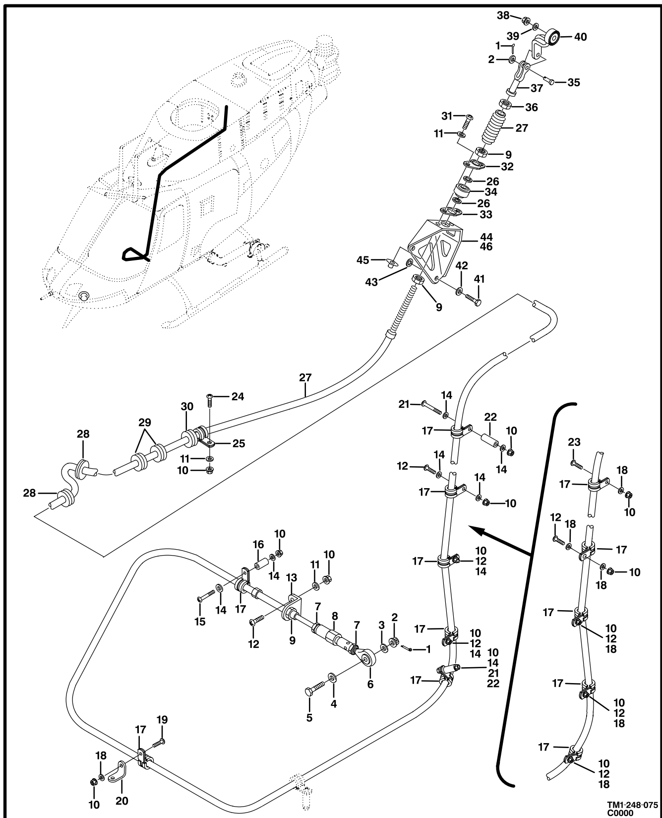
Figure 74. Engine Control Installation
