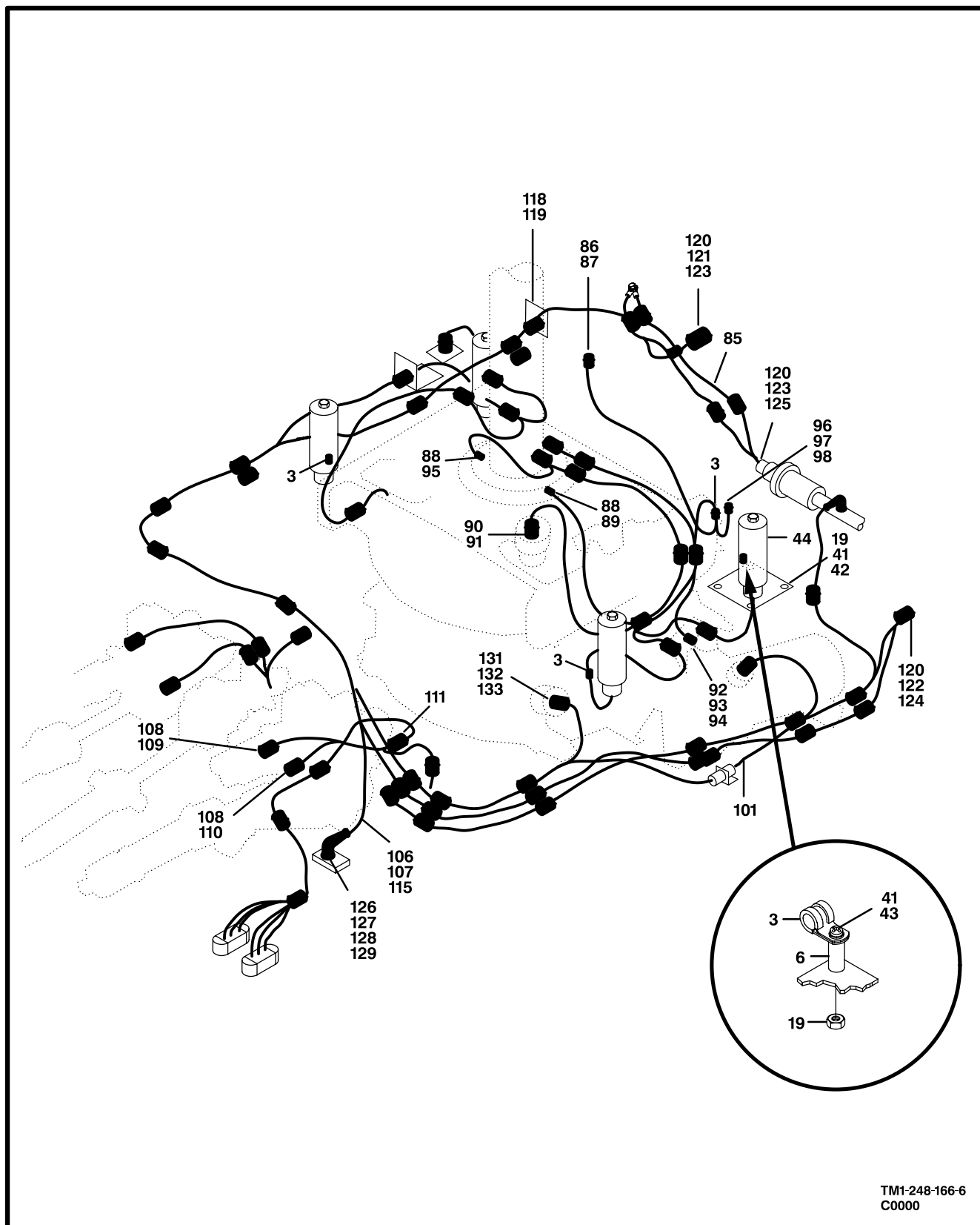
Figure 161. Electrical Installation, Mast Mounted Sight (Sheet 6 of 6)
