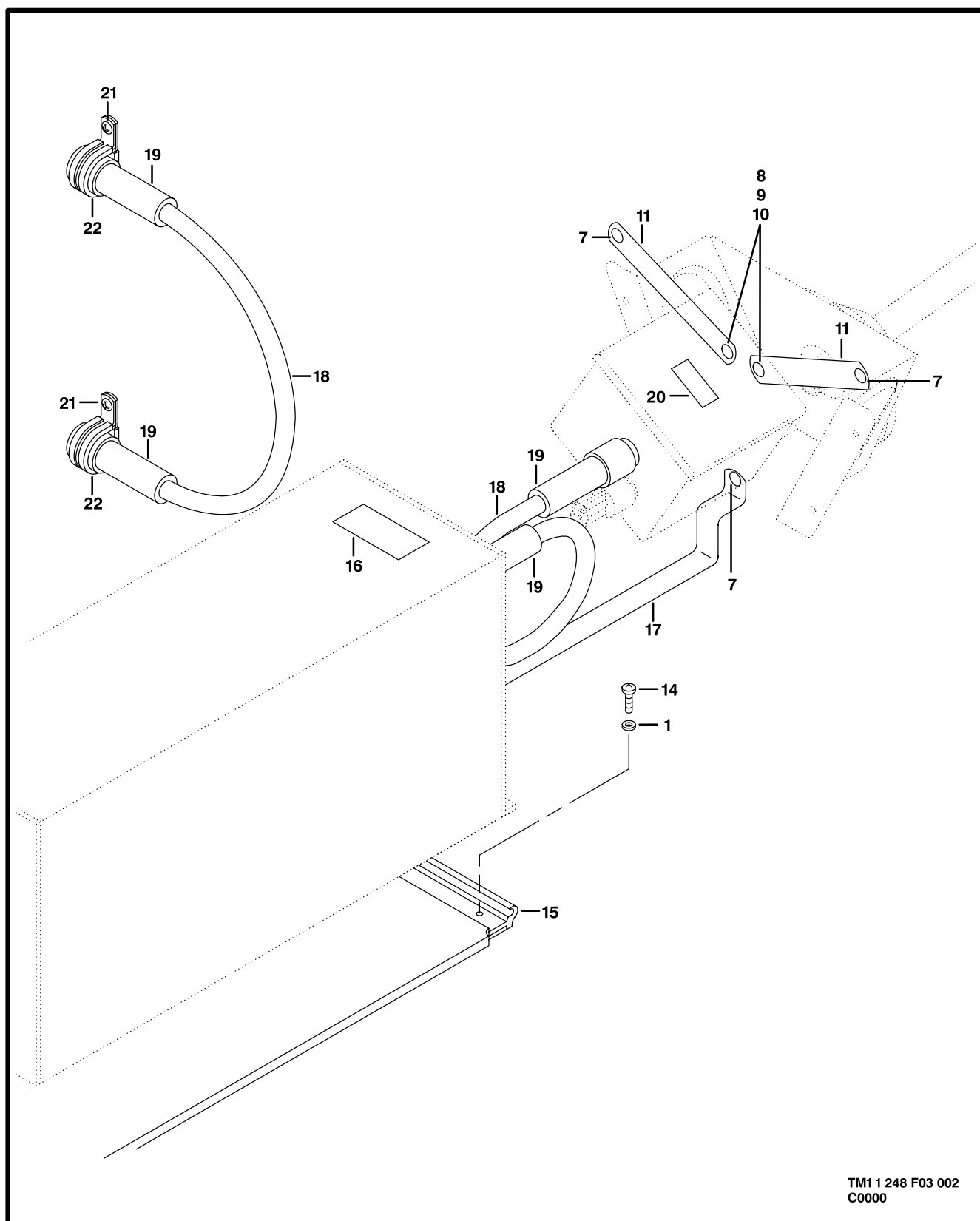
Figure F3. HF Antenna Installation (Sheet 2 of 2)
