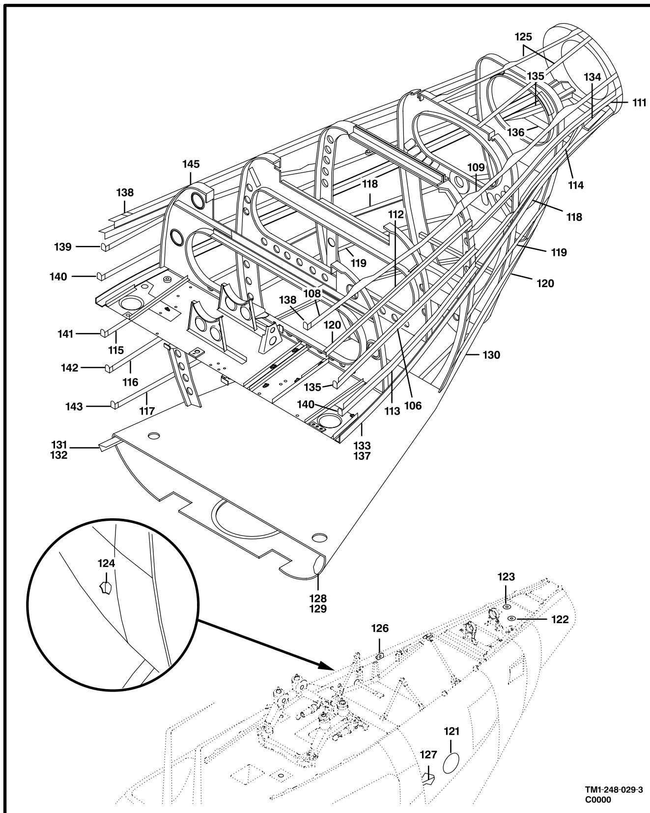
Figure 28. Fuselage Assembly,AFT (Sheet 3 of 3)
