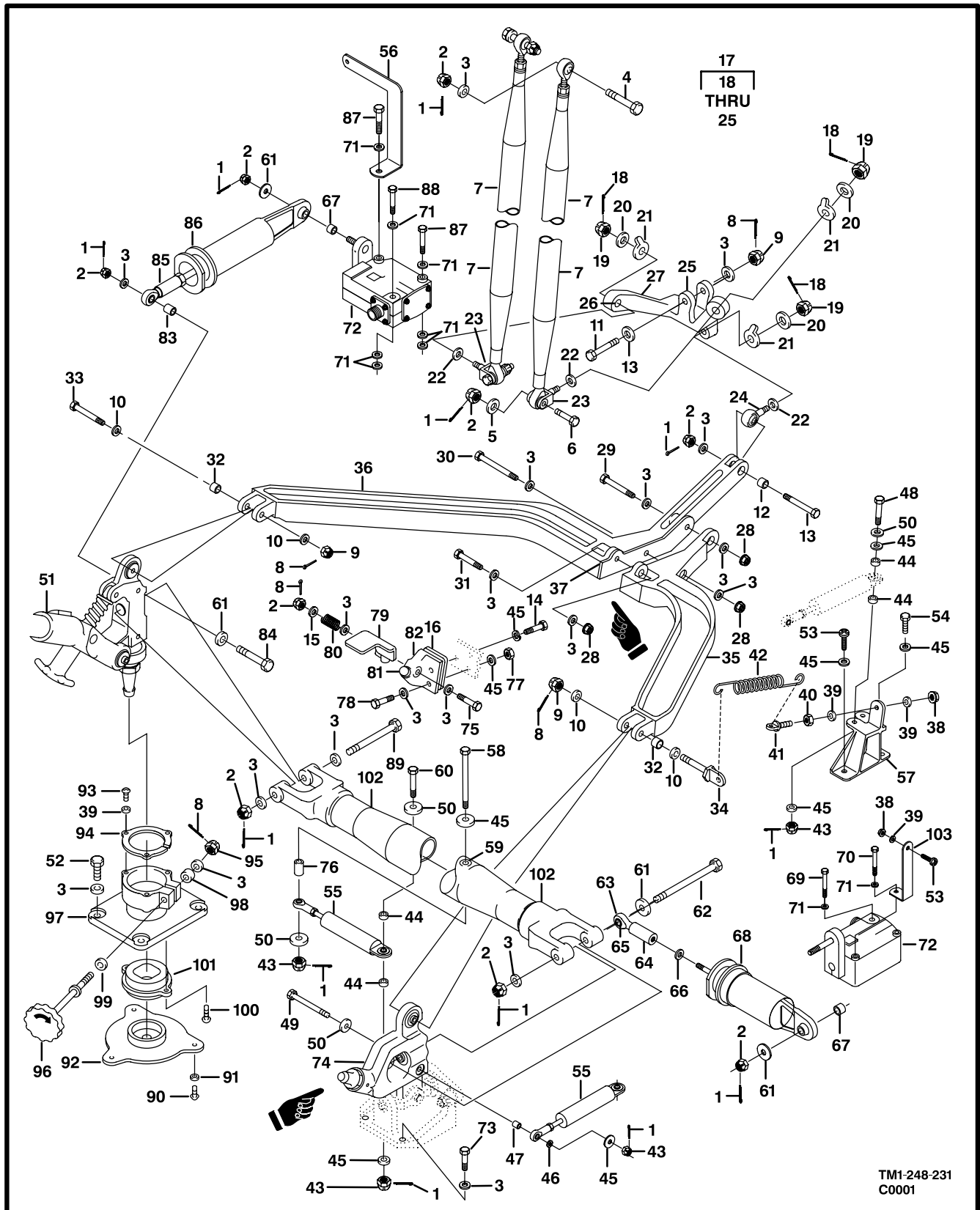
Figure 249. Controls Installation,Cyclic
