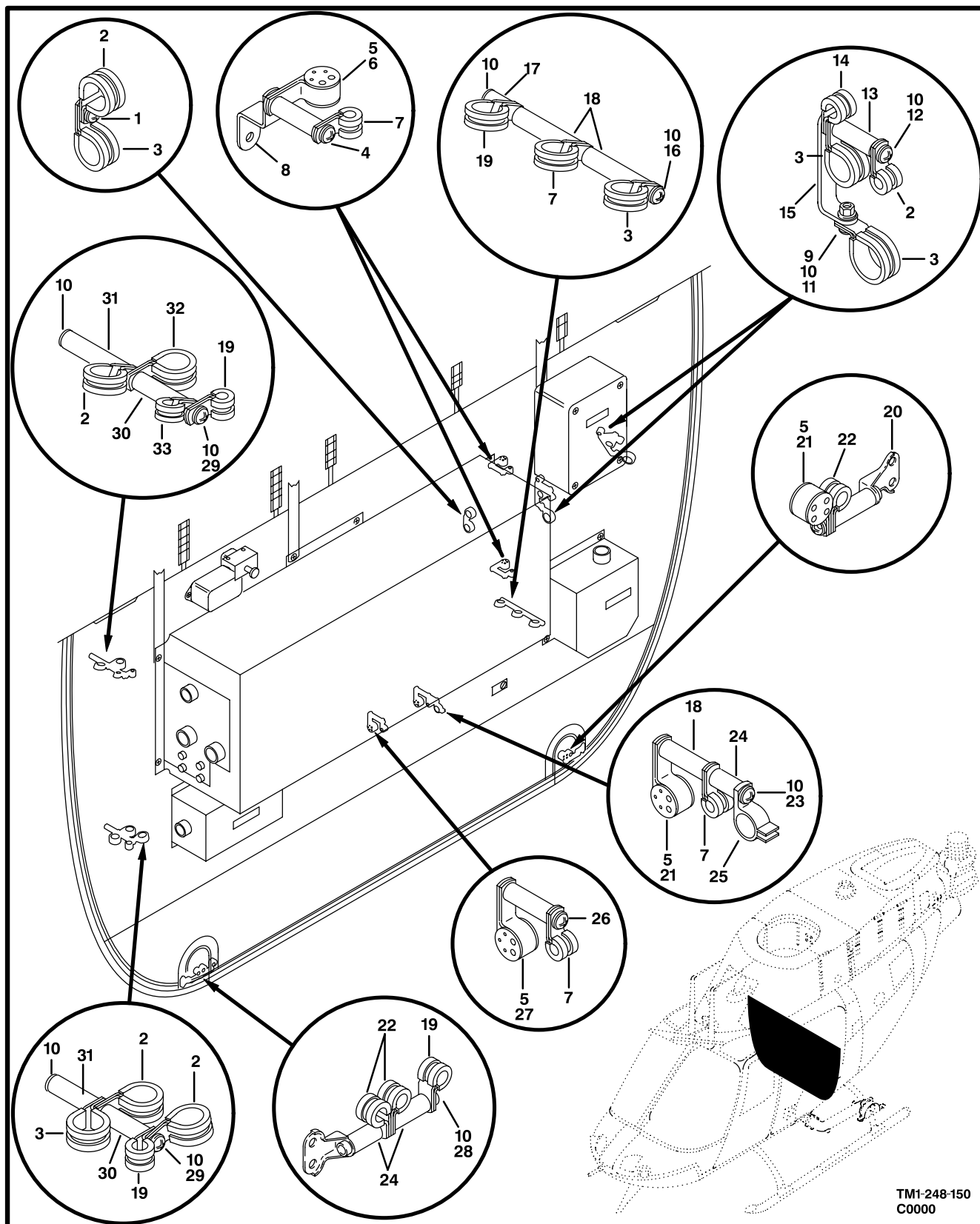
Figure 145. Electrical Installation, Bulkhead
