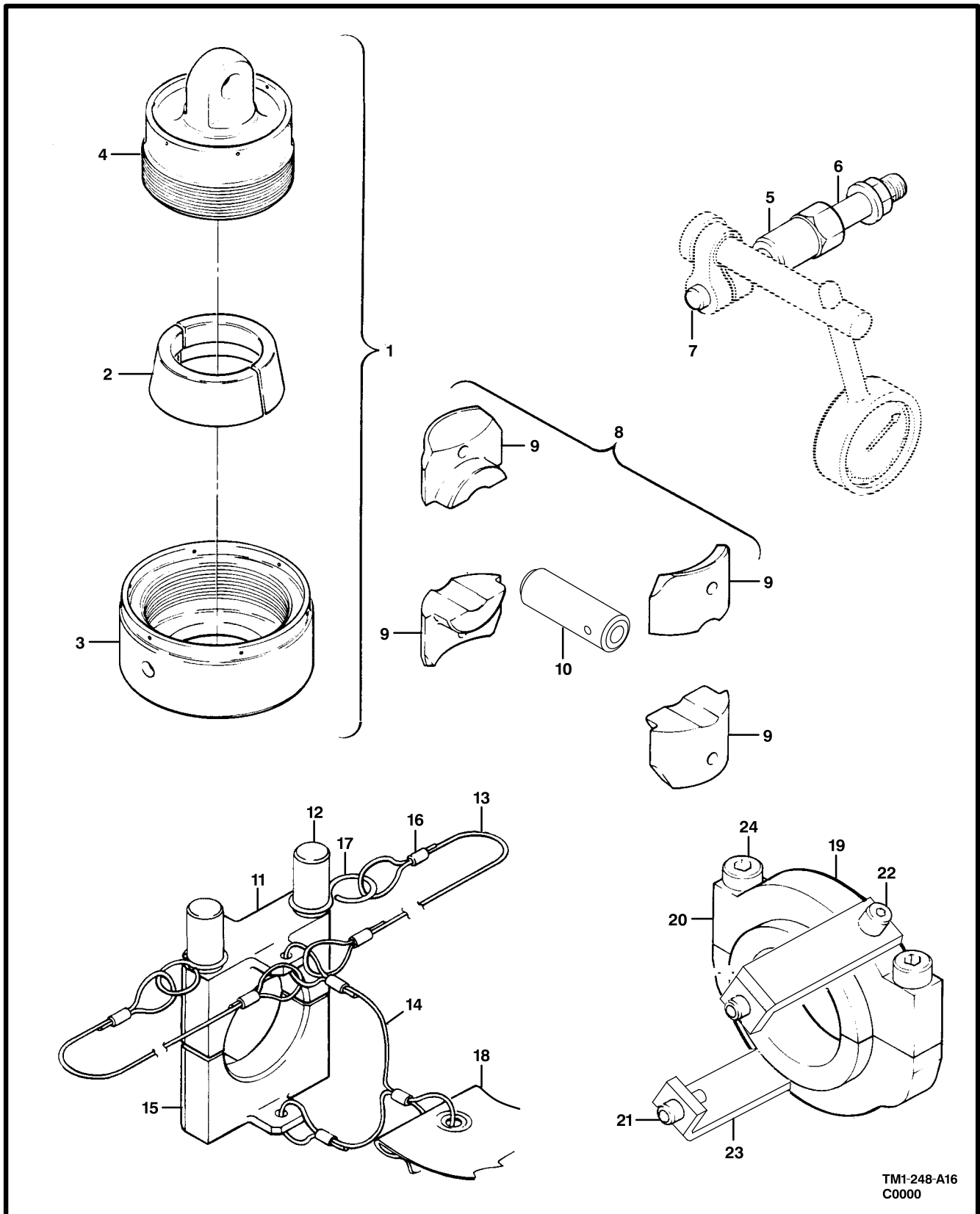
Figure A15. Airframe Tools
