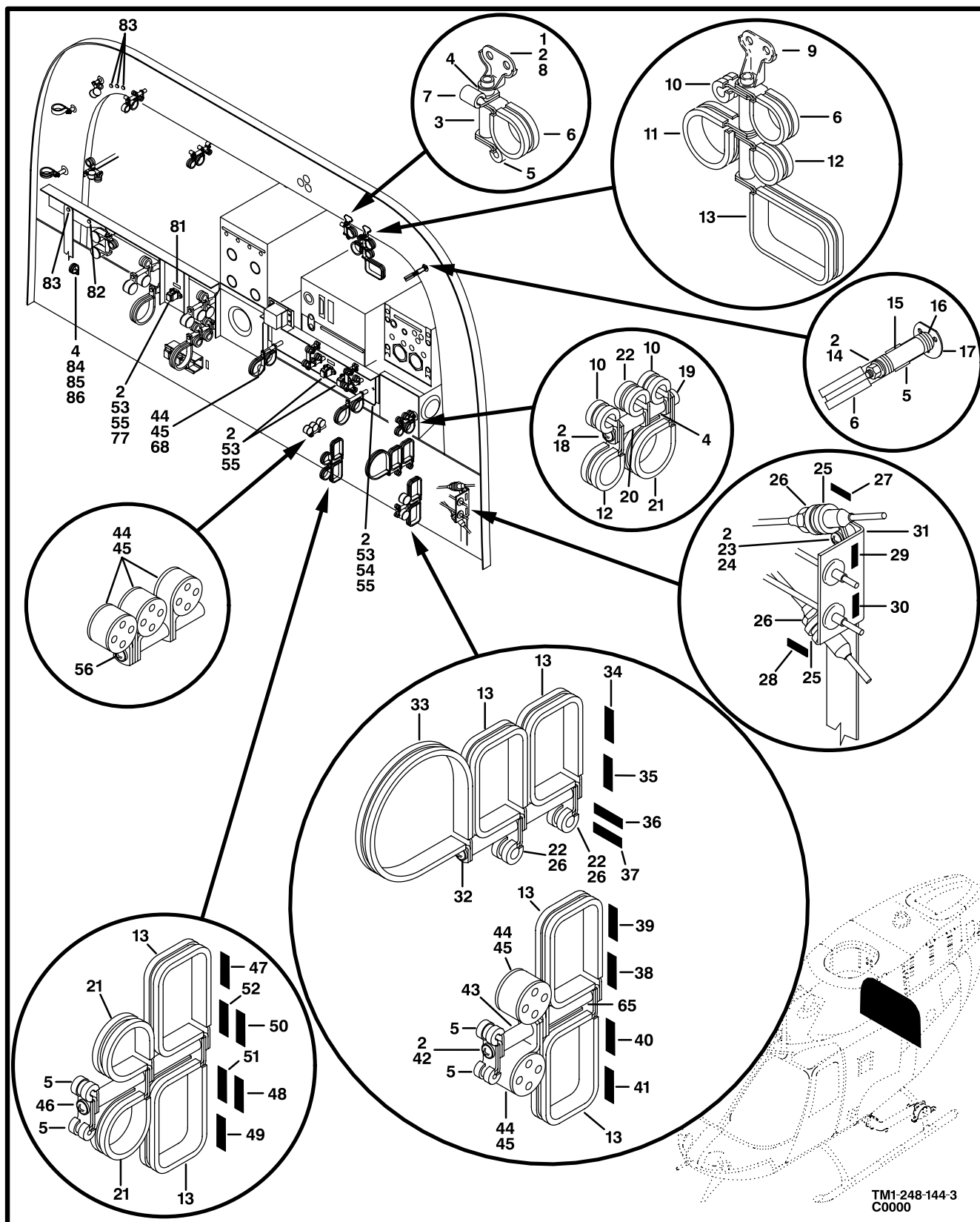
Figure 139. Electrical Installation, Bulkhead (Sheet 3 of 3)
