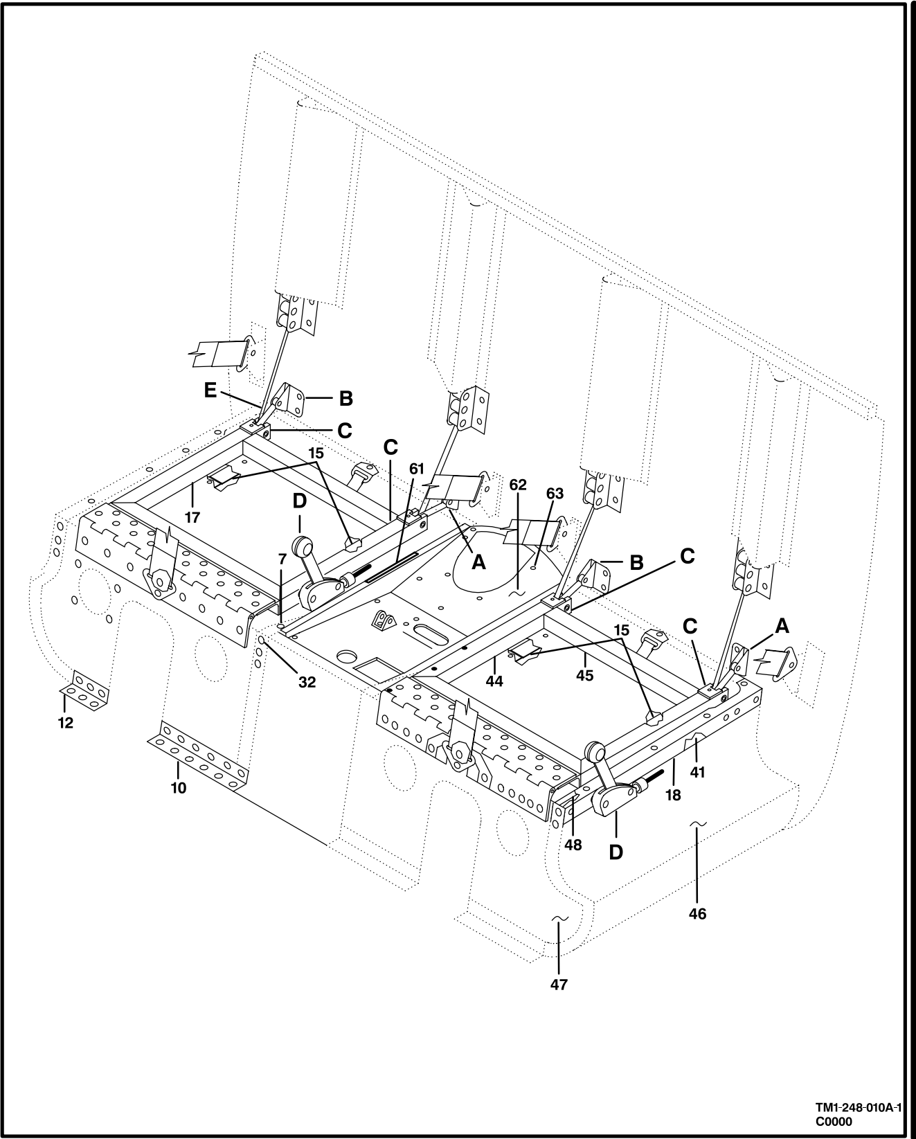
Figure 10A. Crewseat Installation, Energy Attenuating (Sheet 1 of 3)
