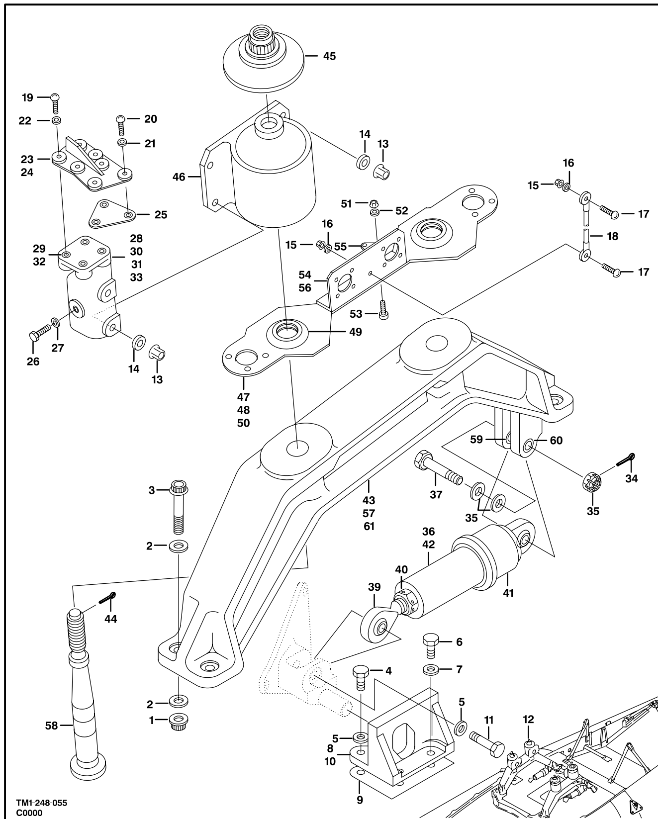
Figure 54. Pylon Mount Installation
