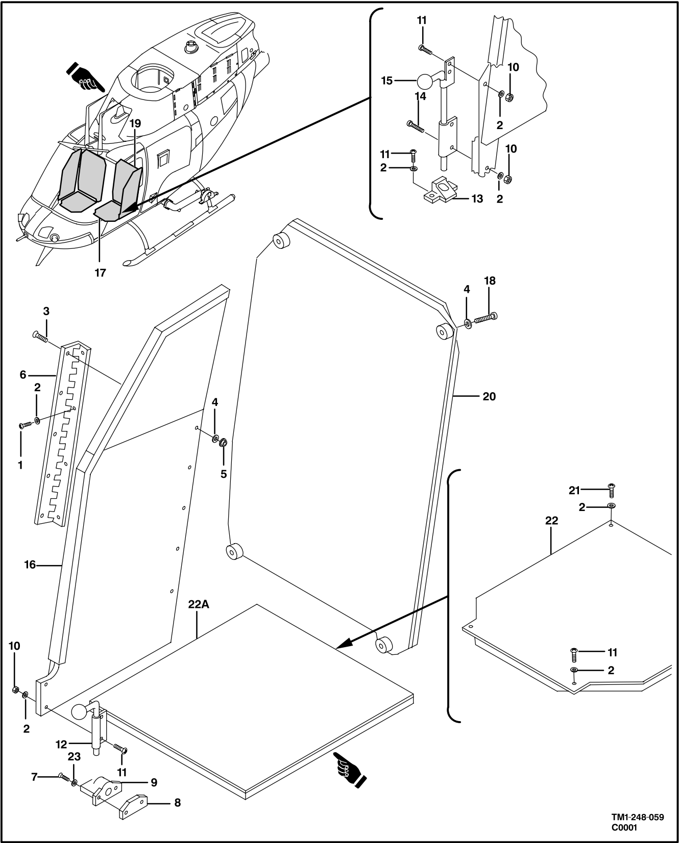
Figure 58. Armor Installation
