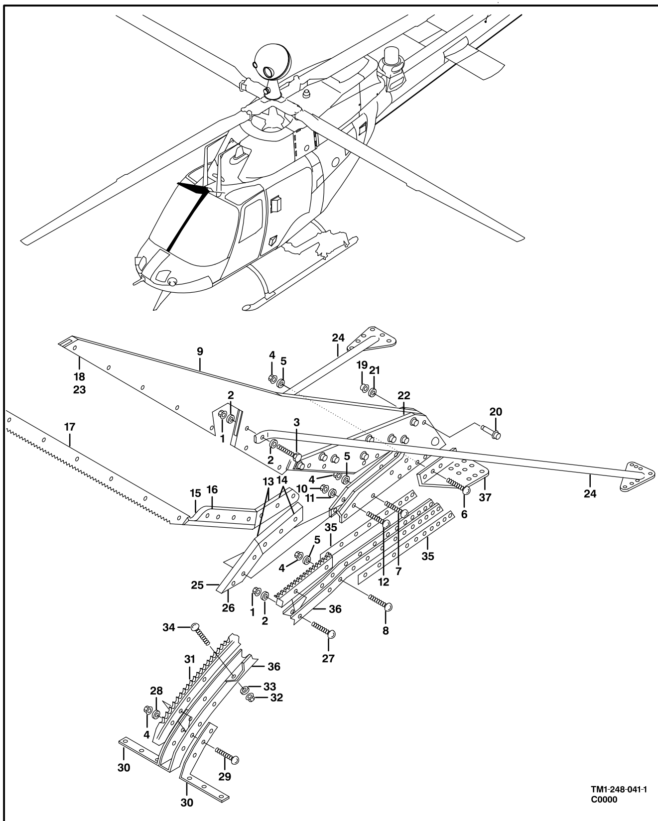
Figure 40. Wire Cutter Installation (Sheet 1 of 2)
