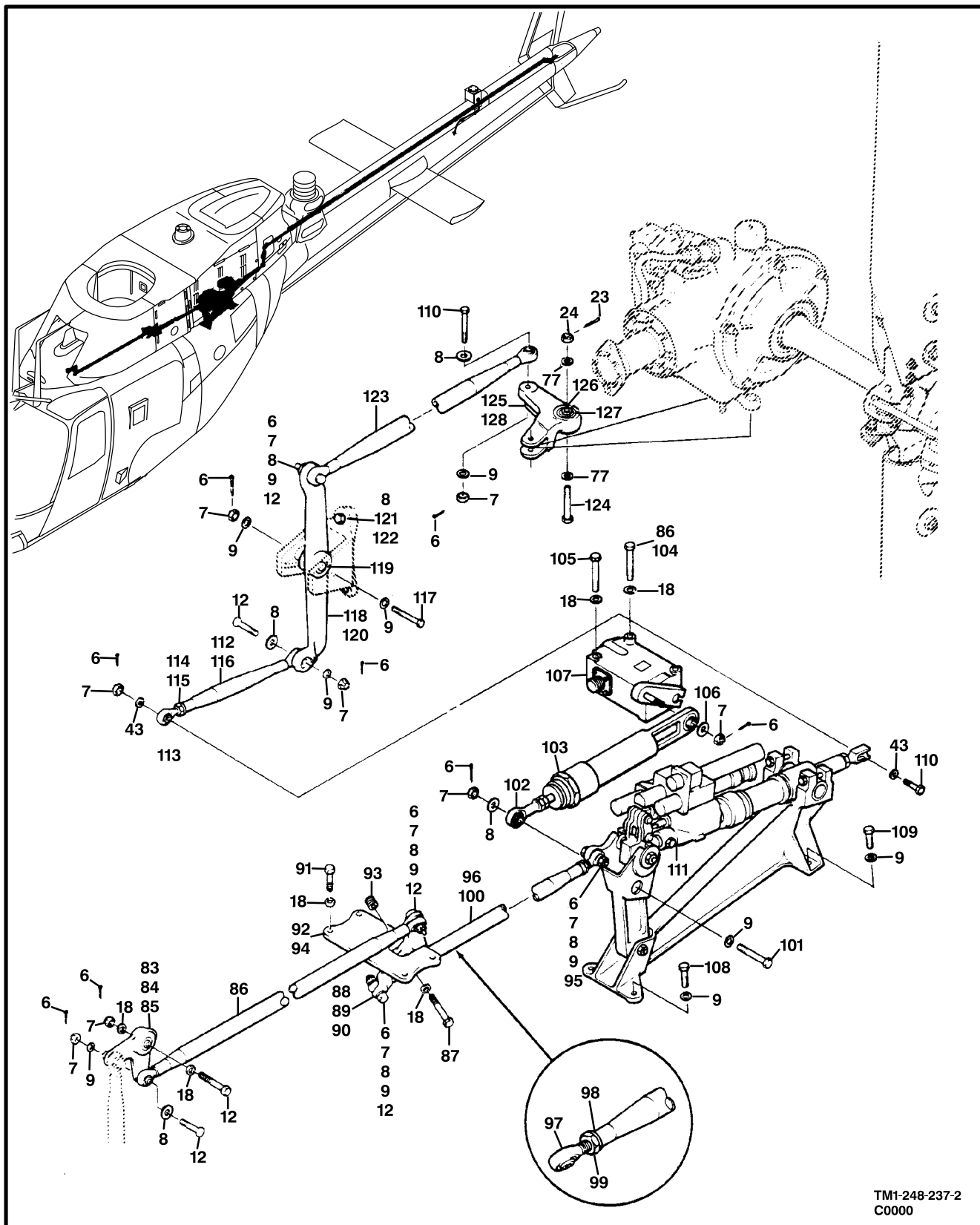
Figure 255. Controls Installation, Directional (Sheet 2 of 2)
