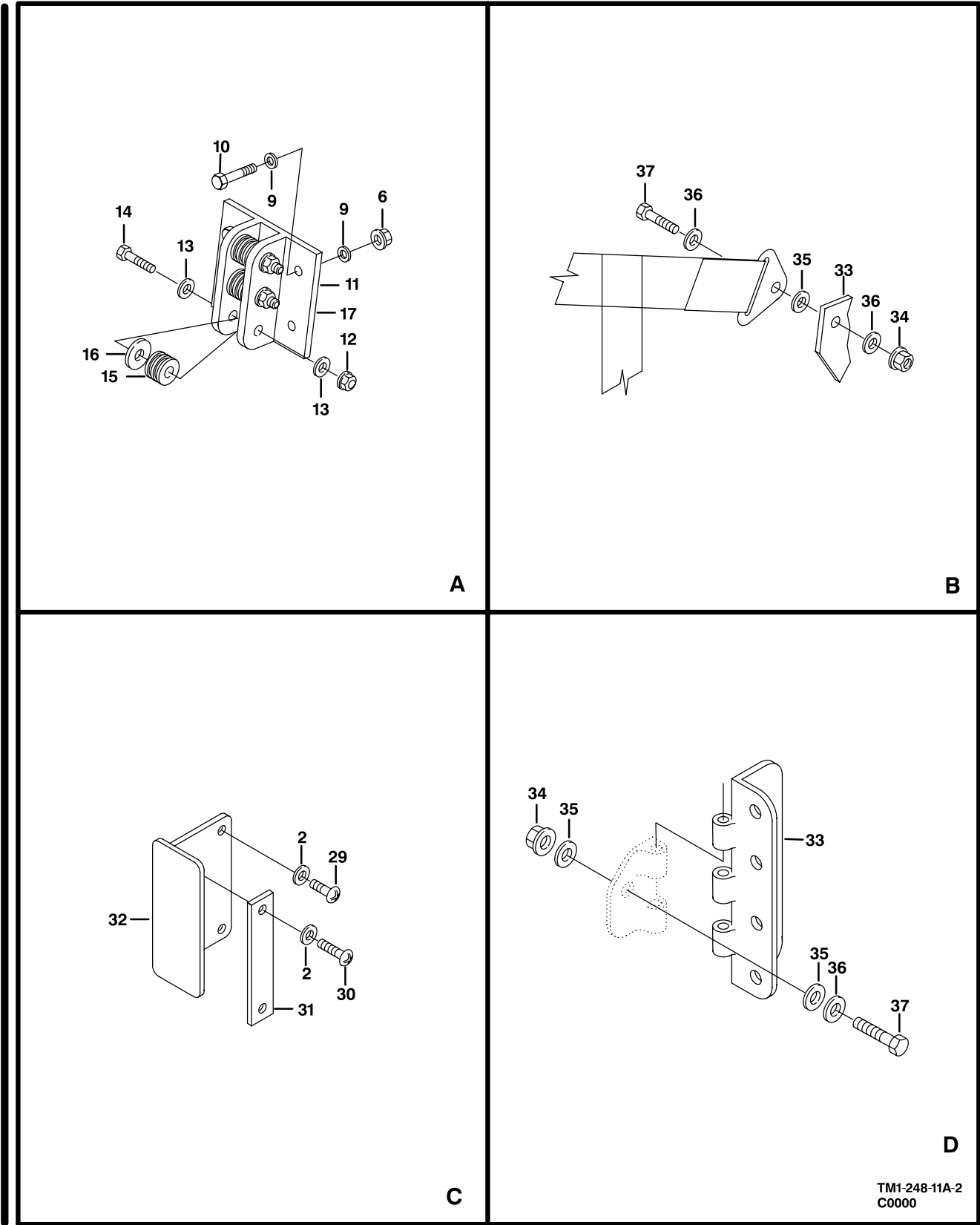
Figure 11A. CrewSeat Installation, Energy Attenuating (Sheet 2 of 2)
