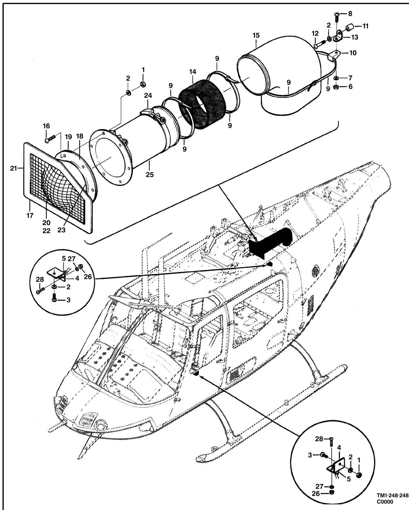
Figure 264. Avionics Cooling System
