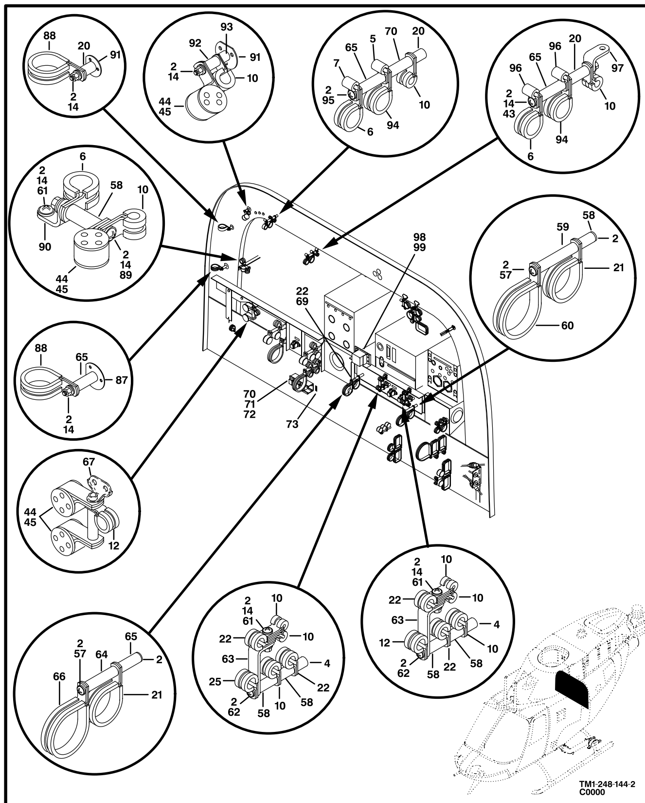
Figure 139. Electrical Installation, Bulkhead (Sheet 2 of 3)
