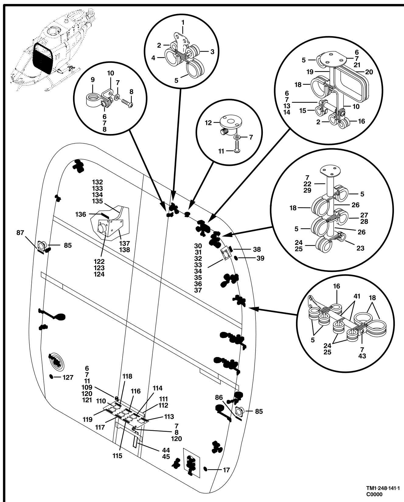
Figure 136. Electrical Installation,Bulkhead (Sheet 1 of 4)
