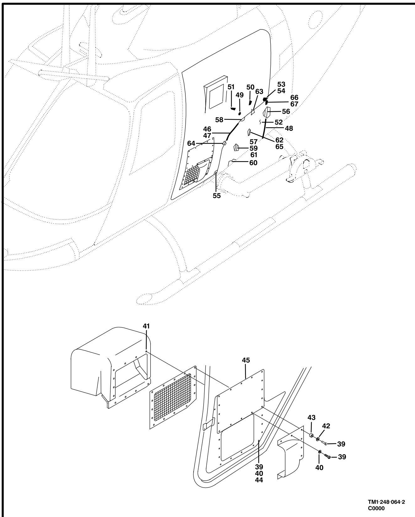
Figure 63. MOD-Fuselage Structure (Sheet 2 of 2)
