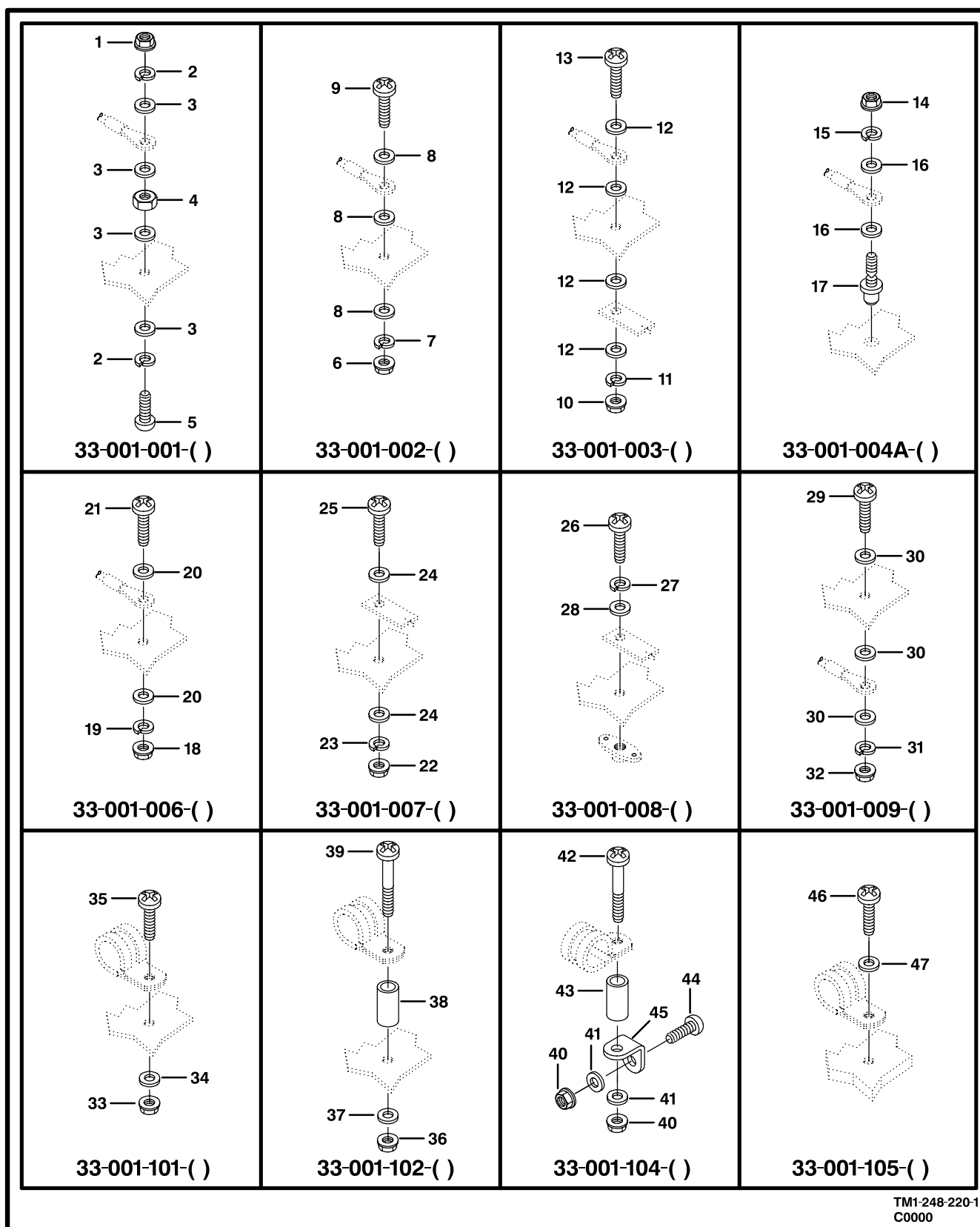
Figure 215. Support Installations (Sheet 1 of 5)
