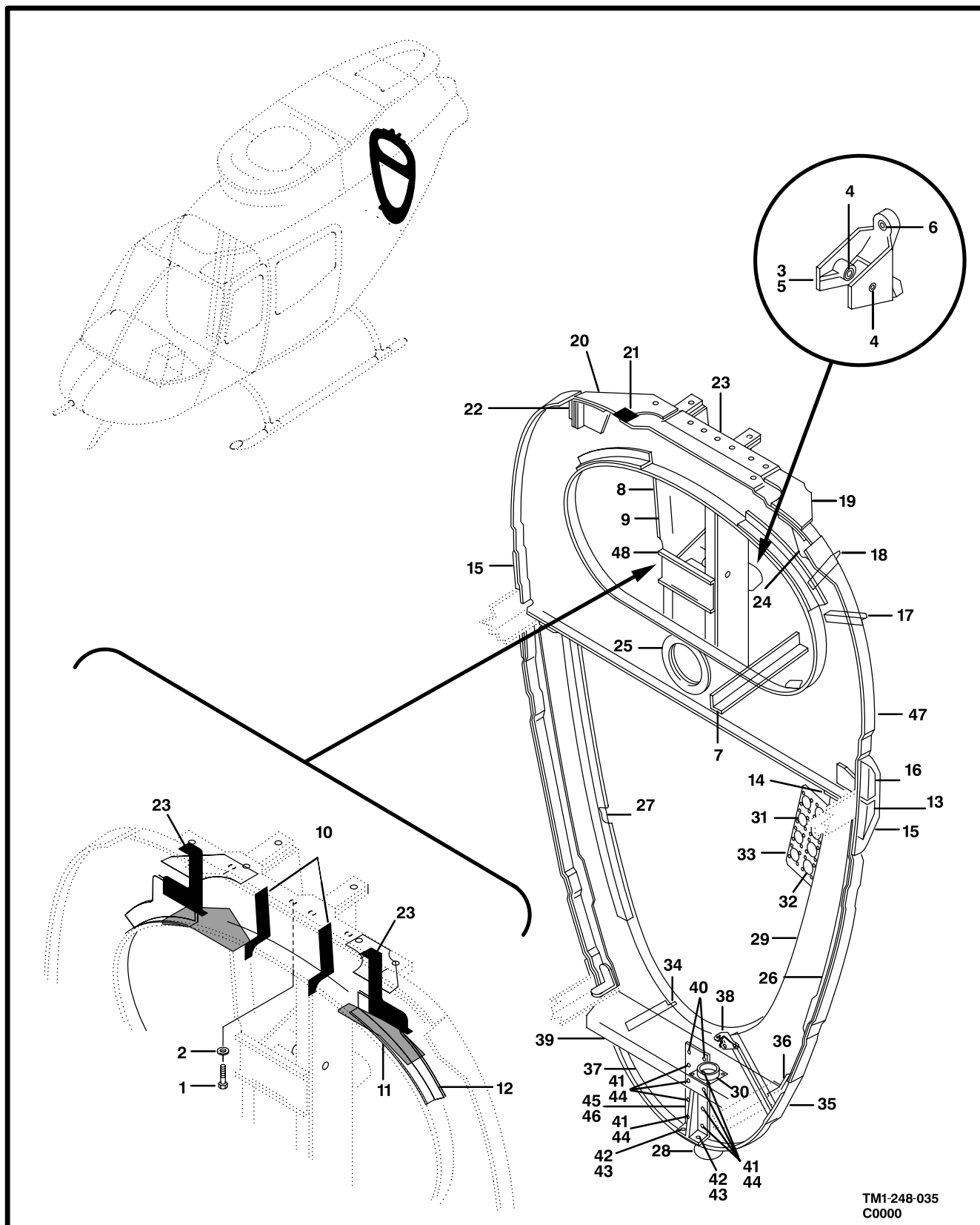
Figure 34. Frame Installation
