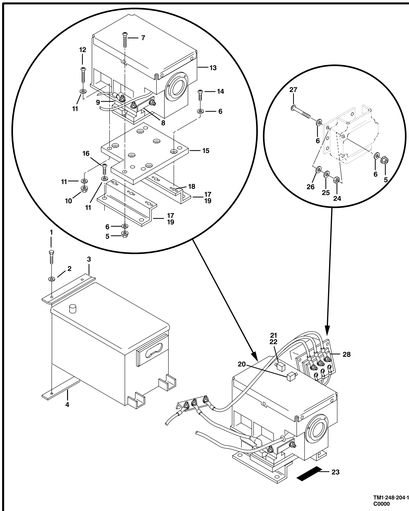
Figure 199. Electrical Assembly, Avionics Installation, AFT Cabin (Sheet 1 of 5)
