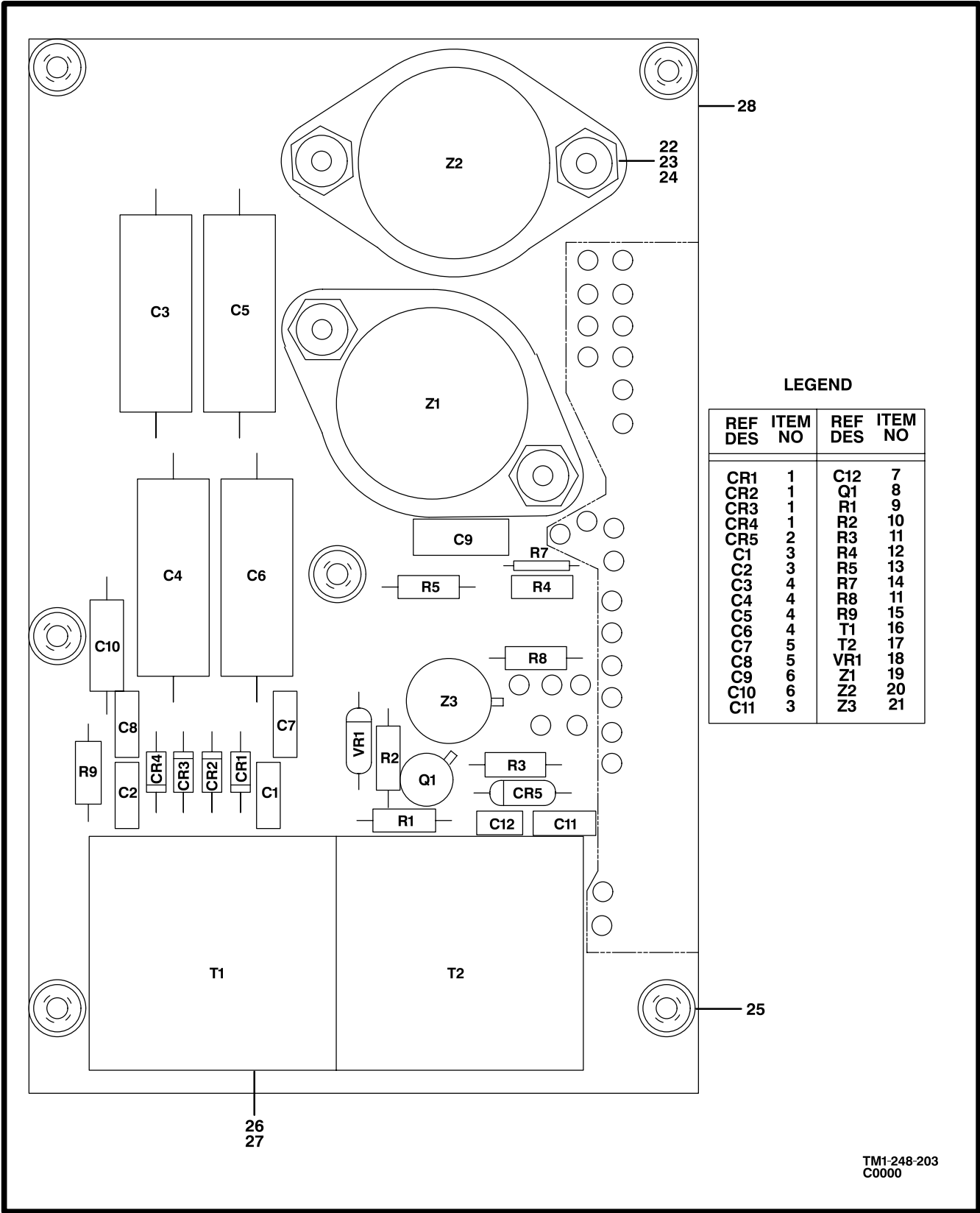
Figure 198. Printed Wiring Assembly,Power Supply,TAMS
