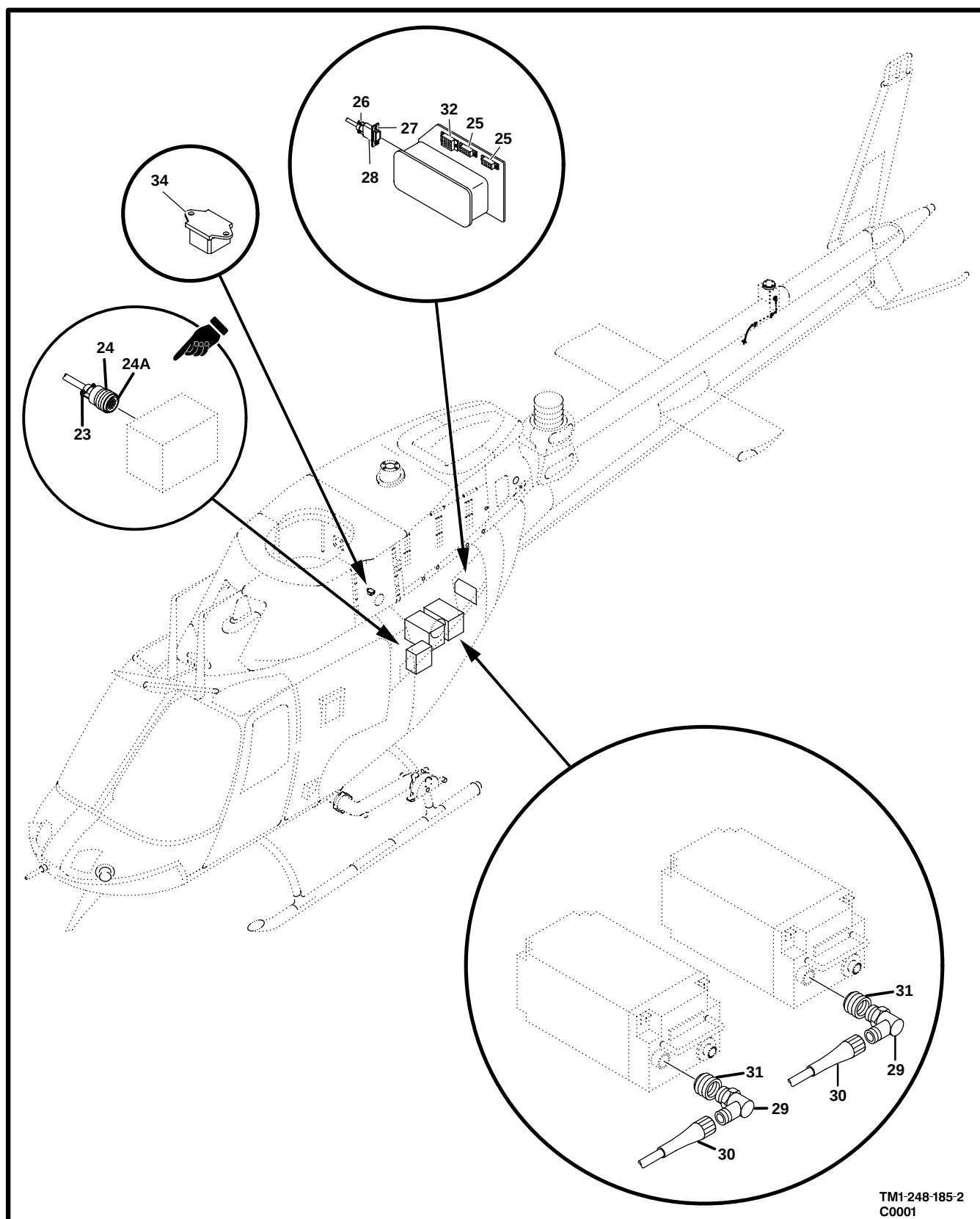
Figure 180. Cable Assembly, Lighting System (Sheet 2 of 2)
