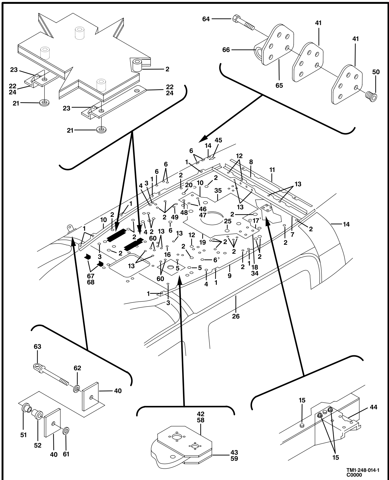
Figure 14. Shell Assembly (Sheet 1 of 2)
