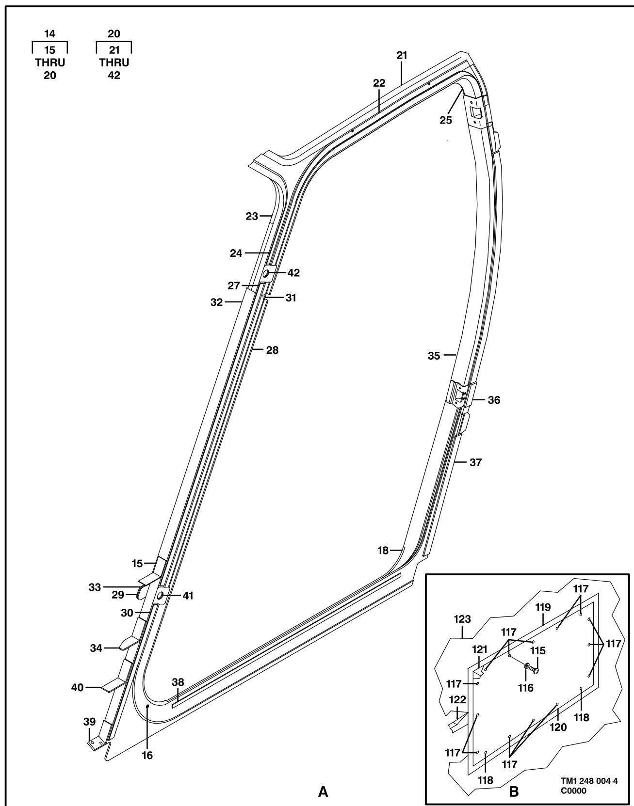
Figure 4. Structure Assembly,Fuselage (Sheet 4 of 4)
