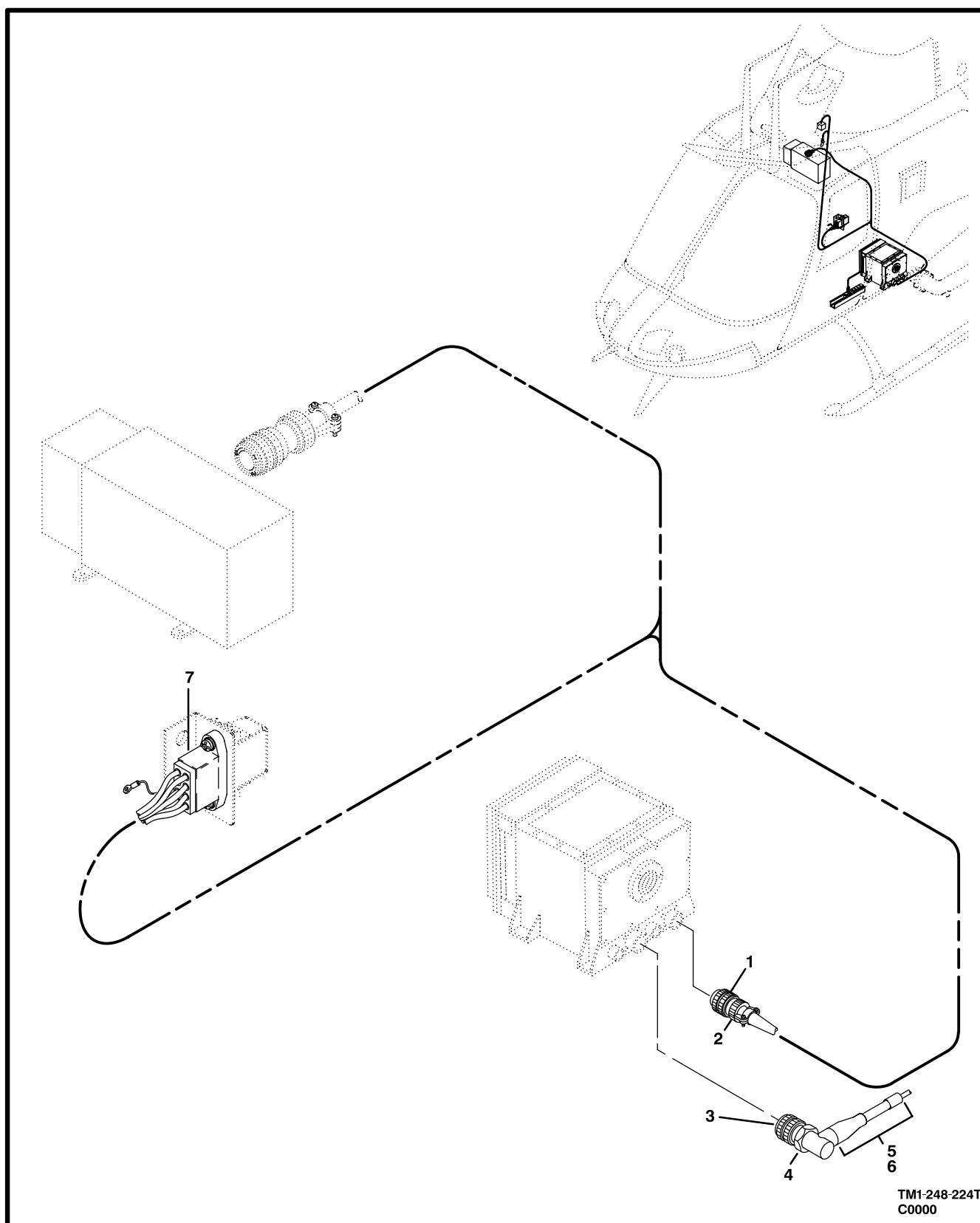
Figure 237. Cable Assembly,Attitude Heading Reference System
