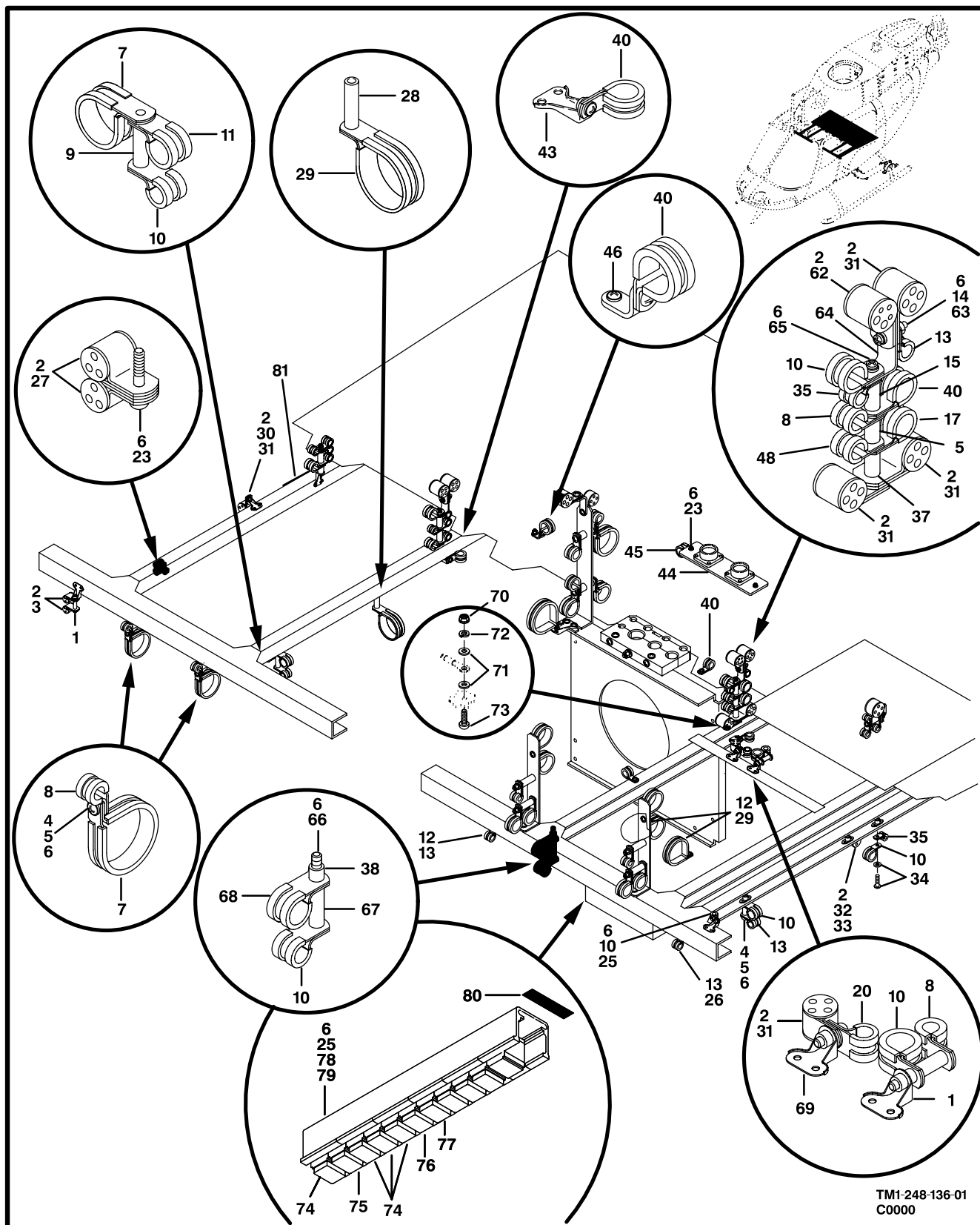
Figure 131. Electrical Installation, Shelf (Sheet 1 of 2)
