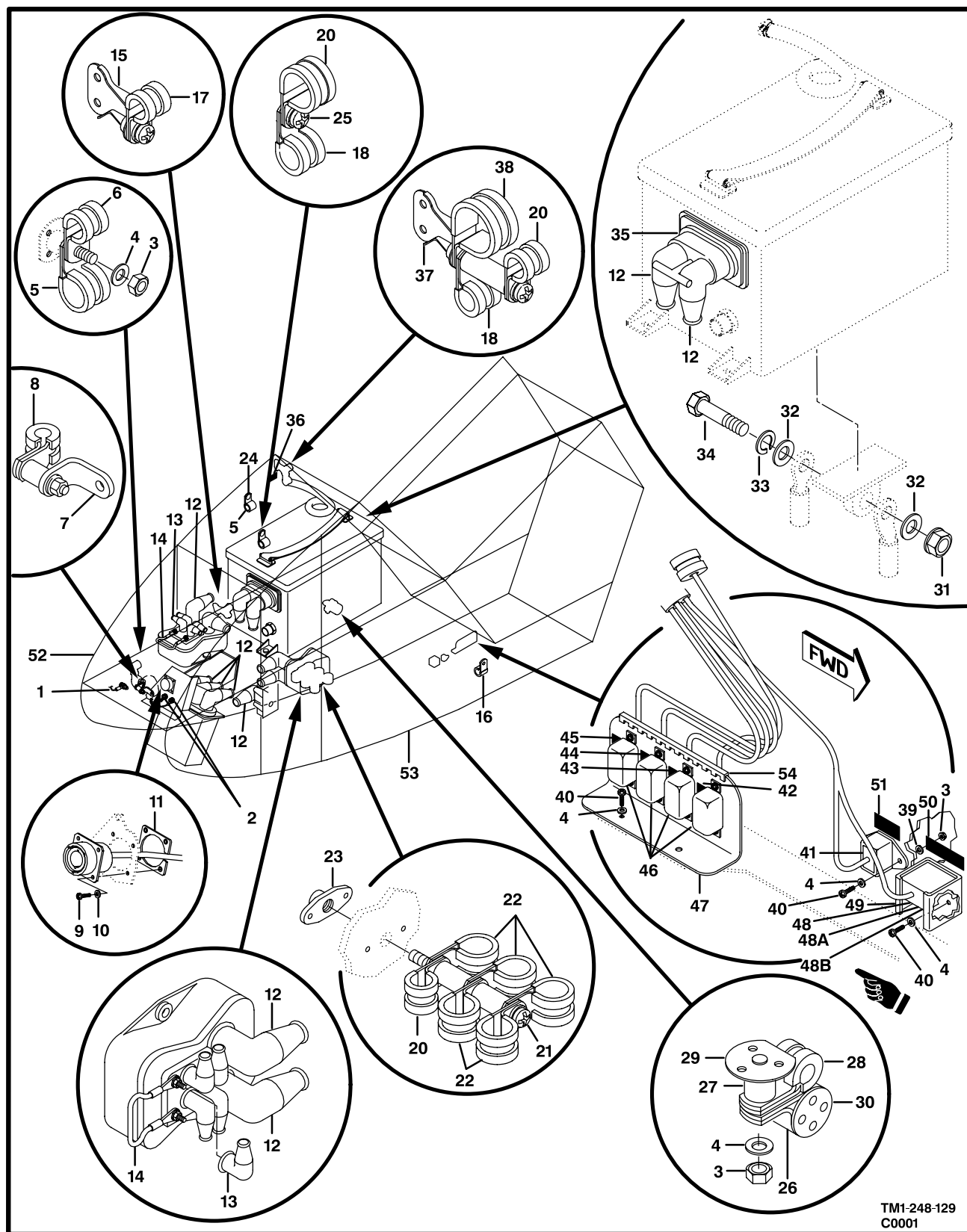
Figure 124. Electrical Installation,Nose
