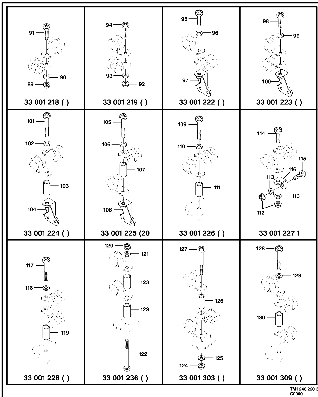
Figure 215. Support Installations (Sheet 3 of 5)
