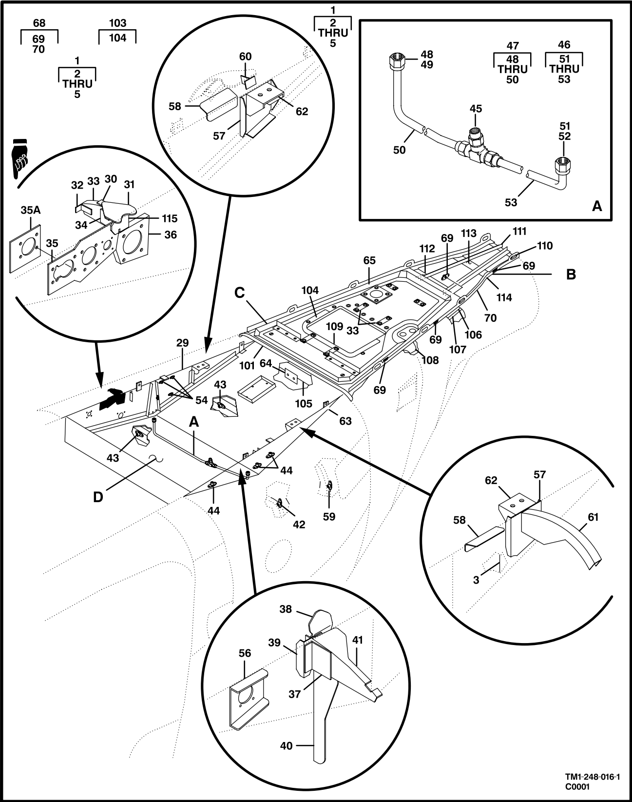
Figure 16. MOD-Roof,AFT (Sheet 1 of 4)
