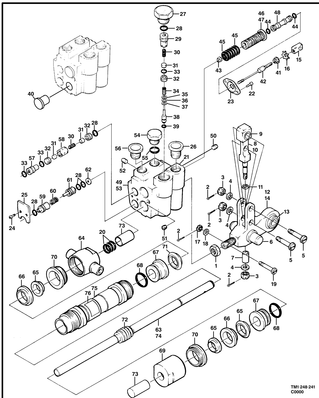
Figure 258. Servo Actuator,Hydraulic Flight Control
