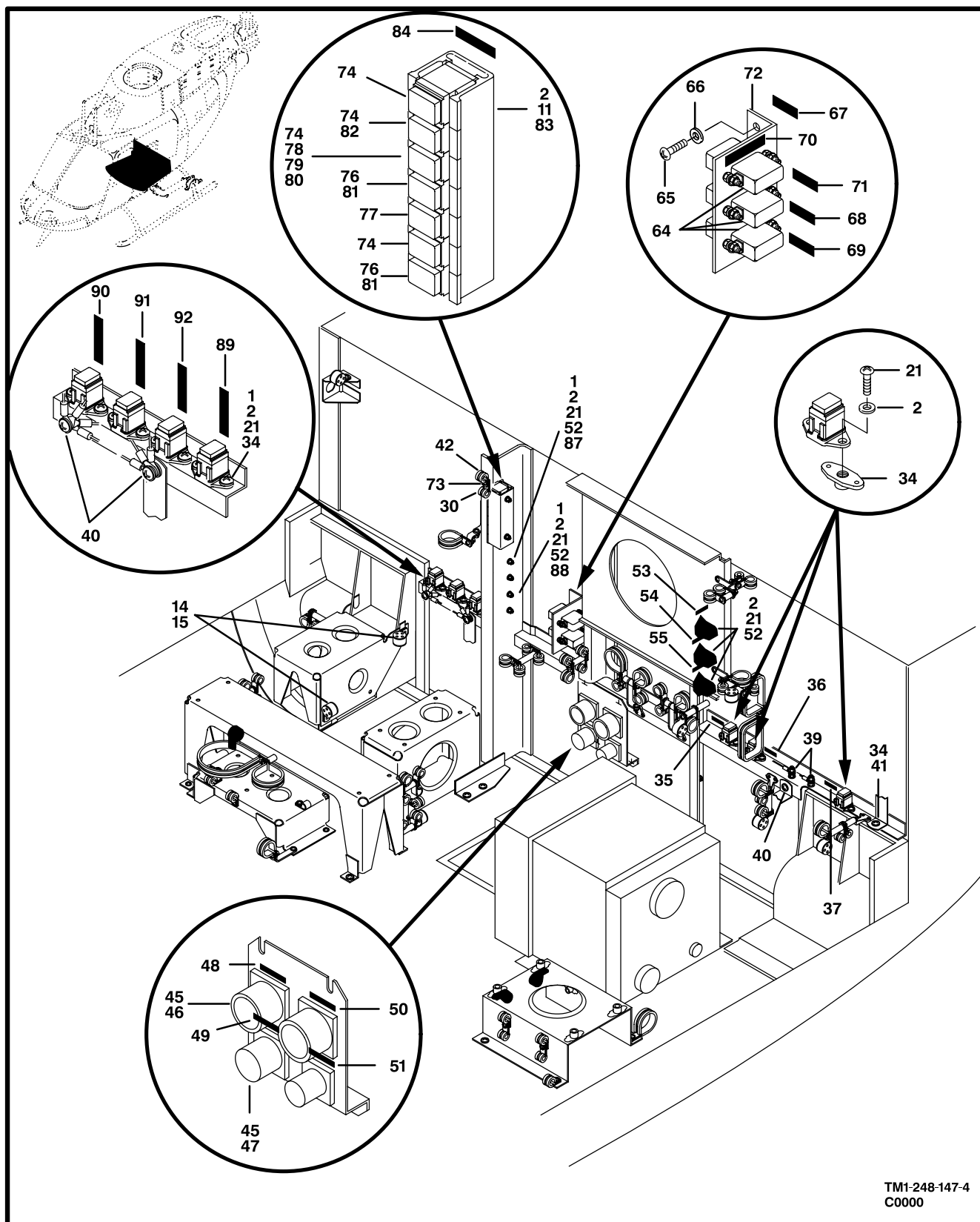
Figure 142. Electrical Installation, Bulkhead (Sheet 4 of 5)
