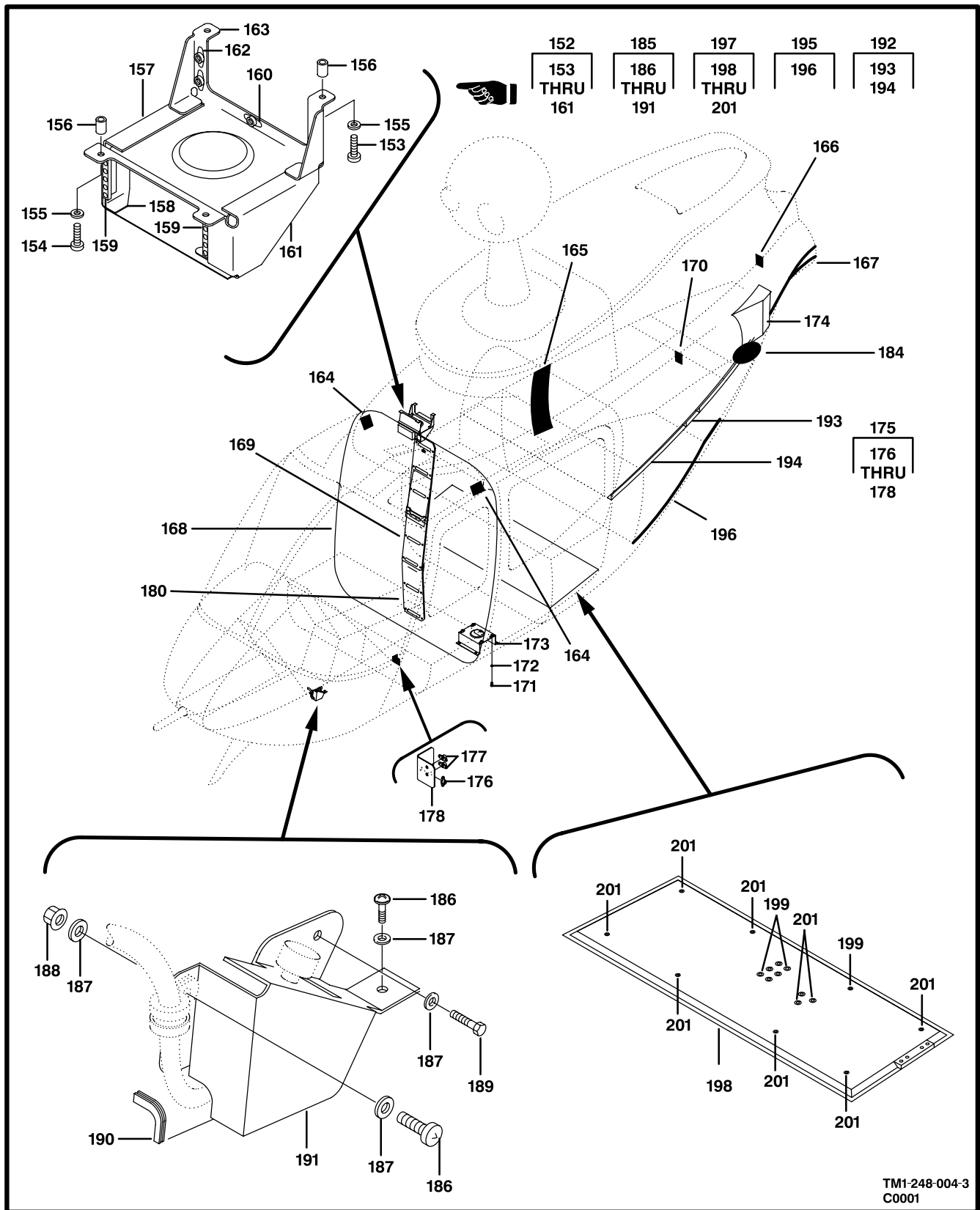
Figure 4. Structure Assembly, Fuselage (Sheet 3 of 4)
