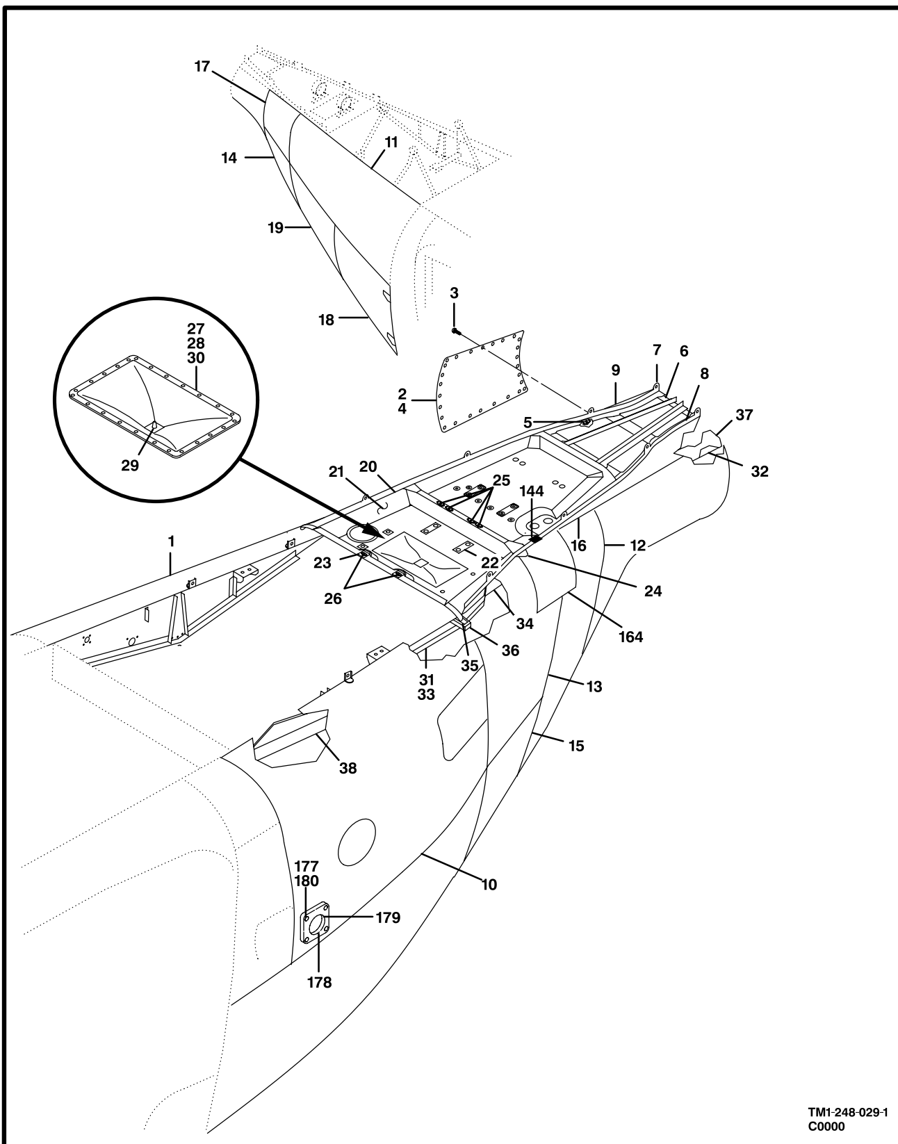
Figure 28. Fuselage Assembly, AFT (Sheet 1 of 3)
