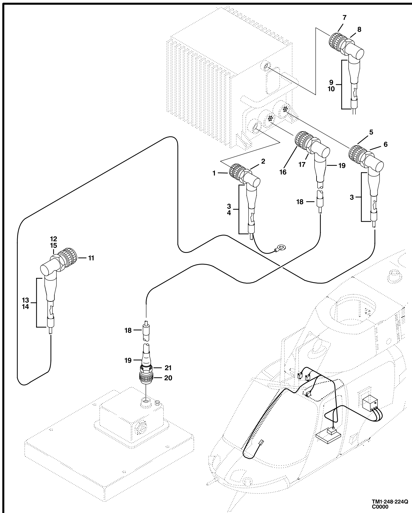
Figure 234. Cable Assembly, Doppler NAV System
