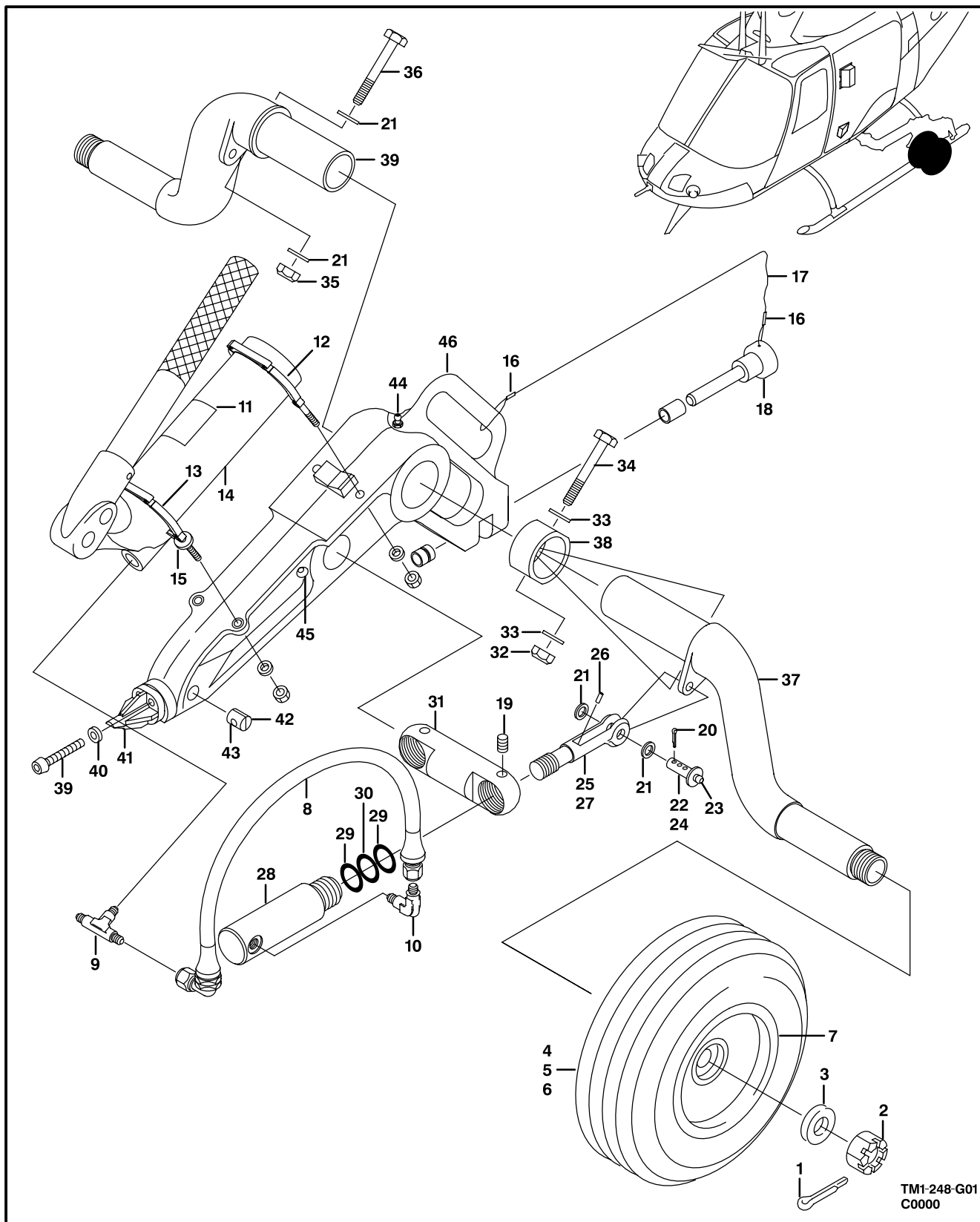
Figure G1. Truck, Handling Wheel
