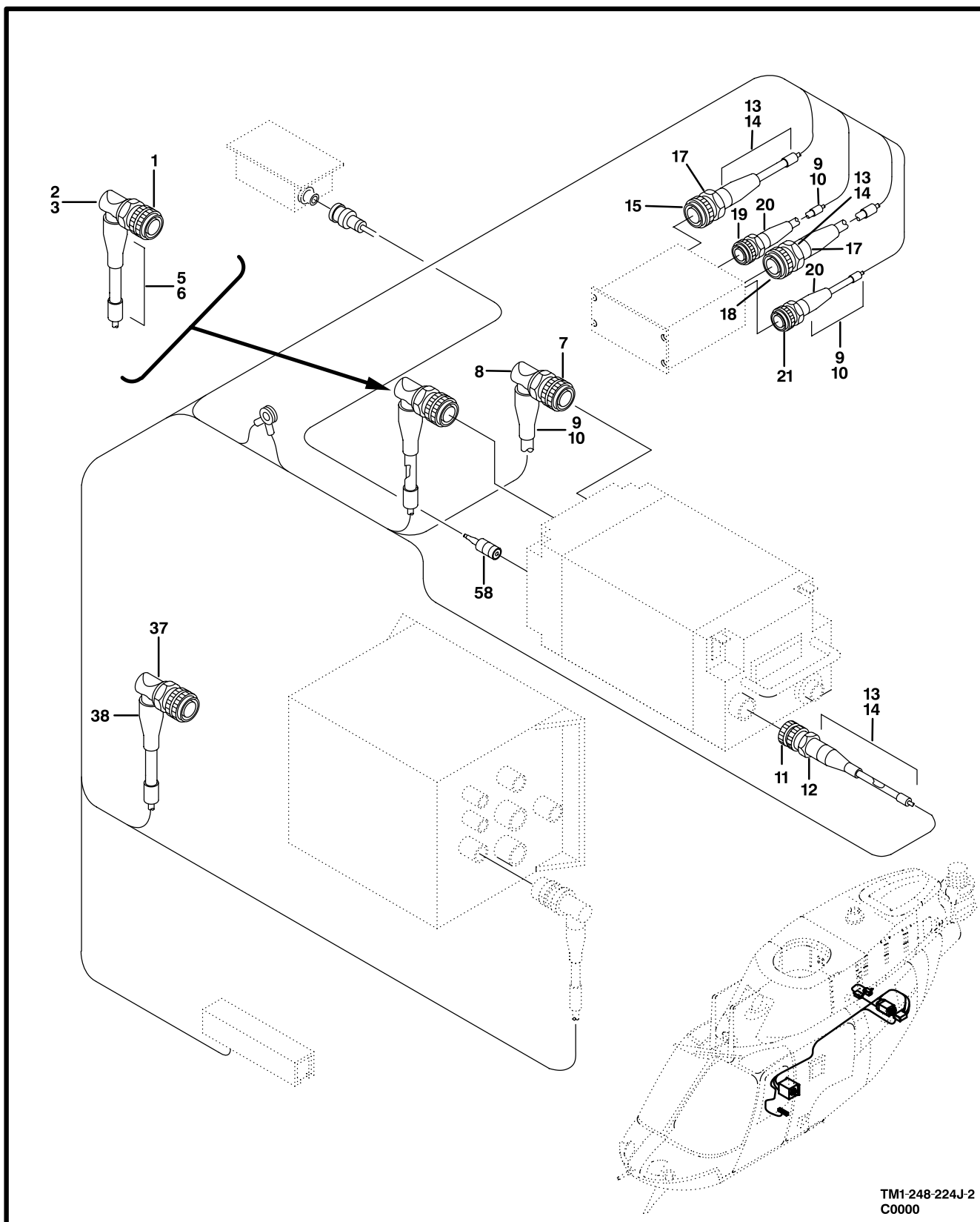
Figure 228. Cable Assembly,VHF-FM Communication System (Sheet 2 of 2)
