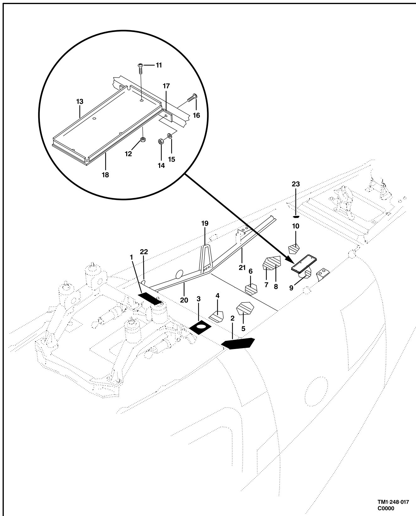
Figure 17. Pan Assembly
