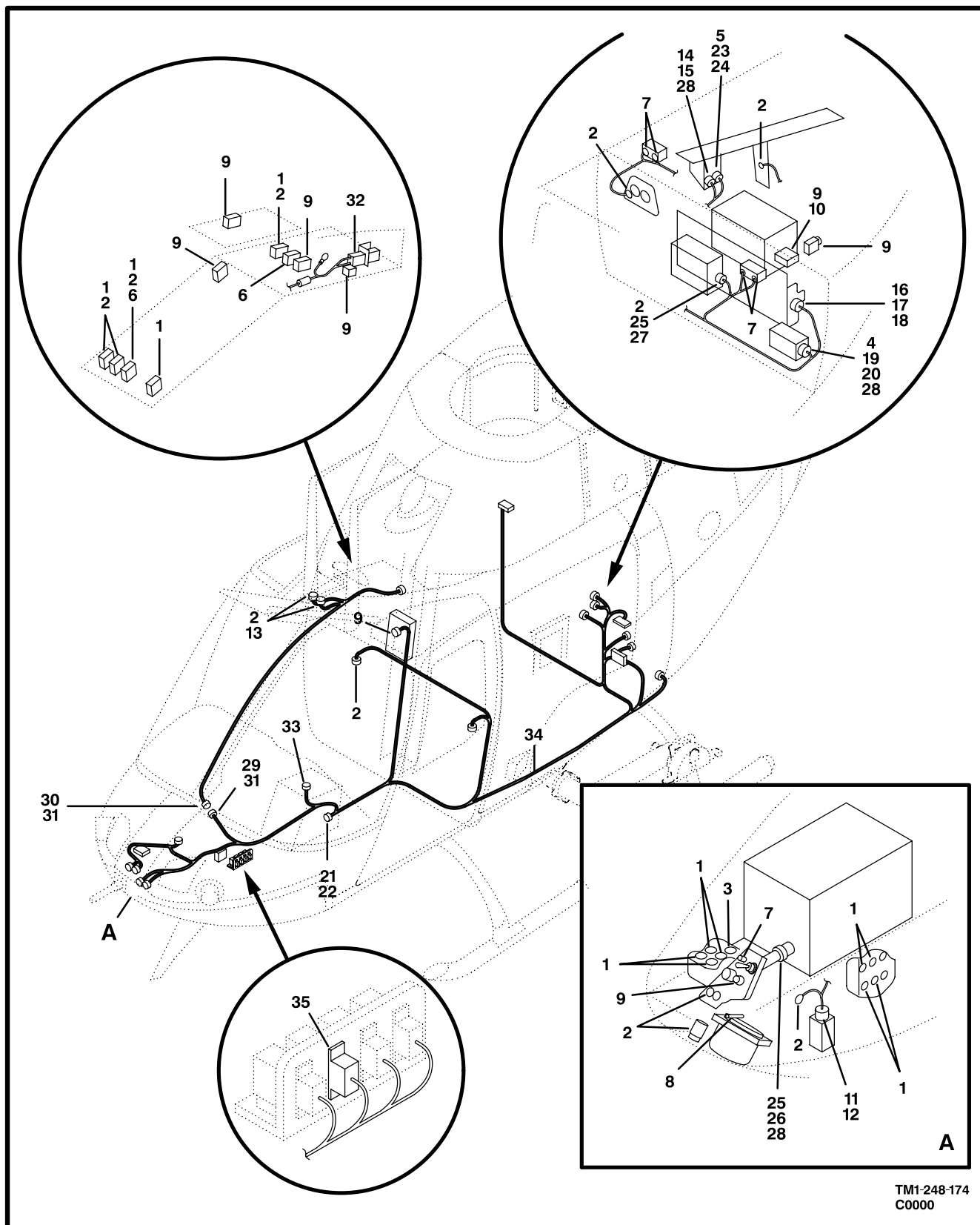
Figure 169. Cable Assembly, DC Power System
