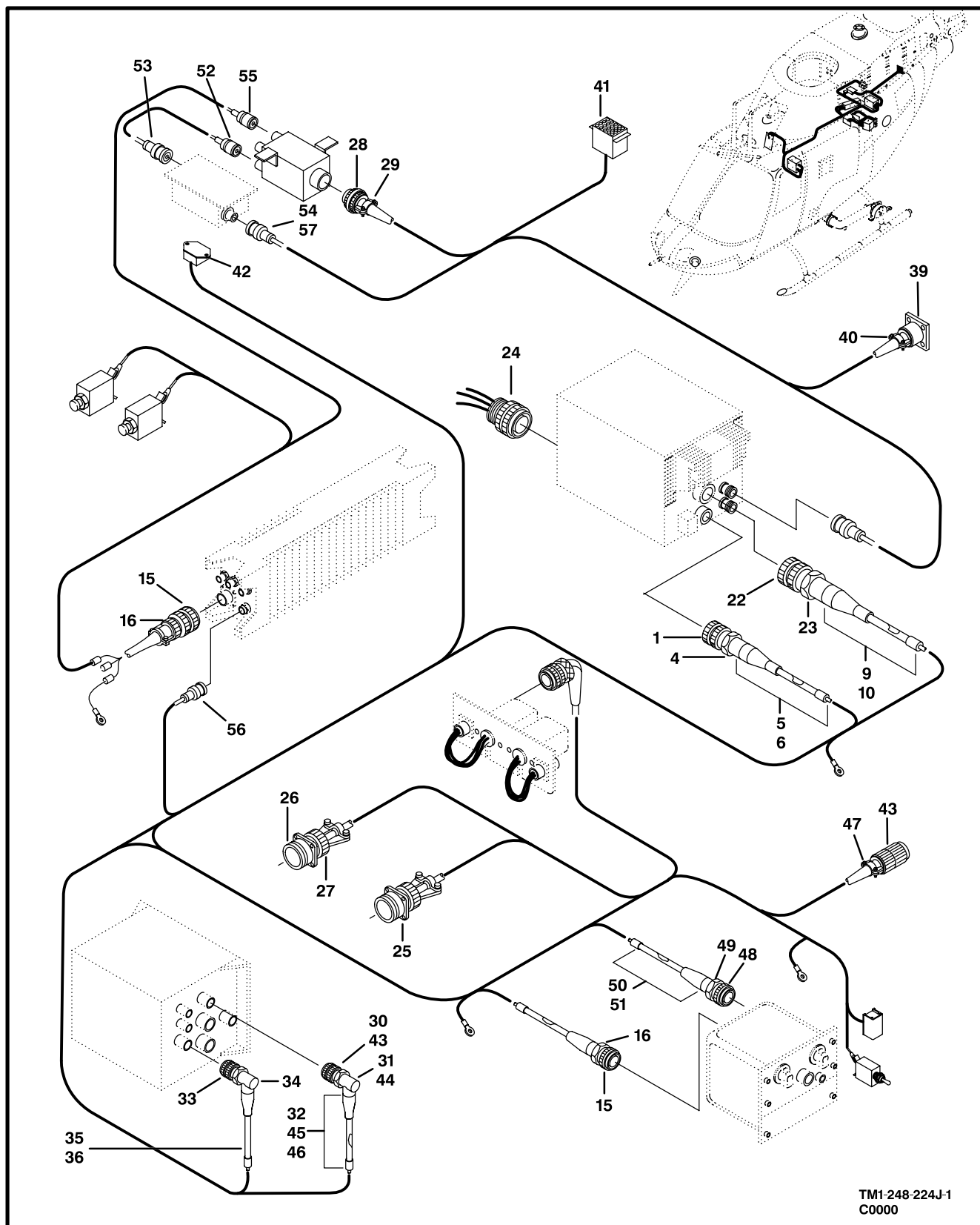
Figure 228. Cable Assembly,VHF-FM Communication System (Sheet 1 of 2)
