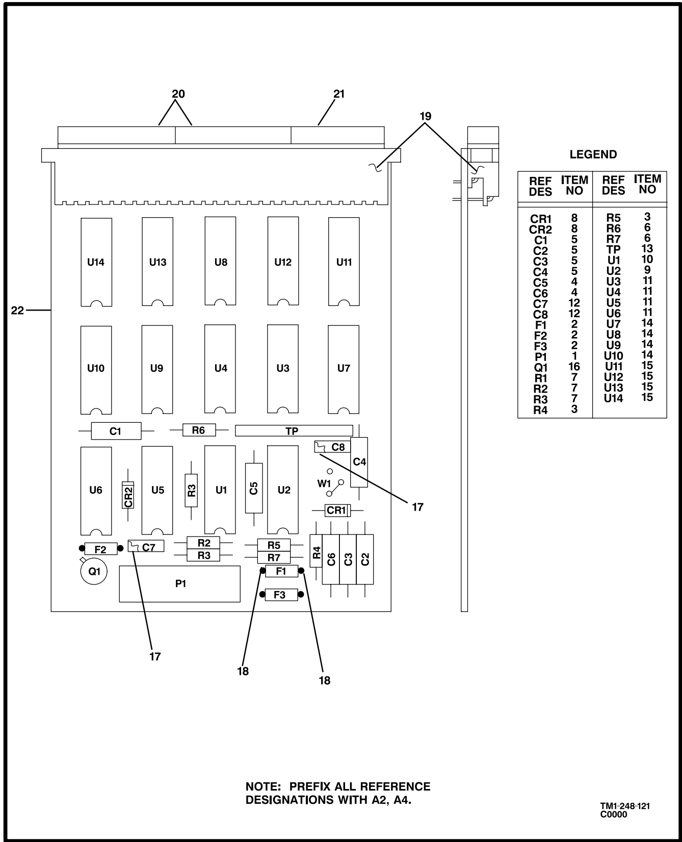
Figure 116. Driver, 28 Lamp
