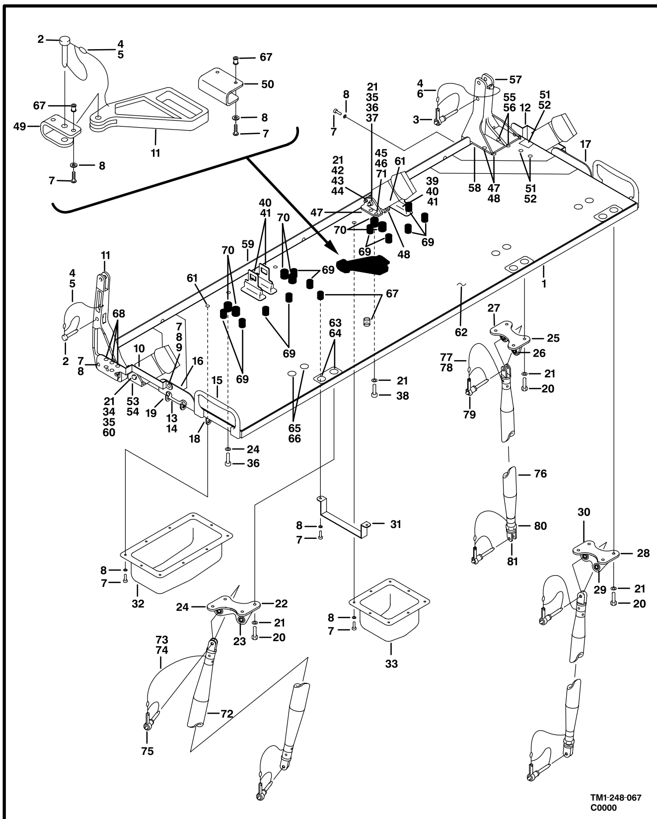
Figure 66. Kit, Seat/Cargo
