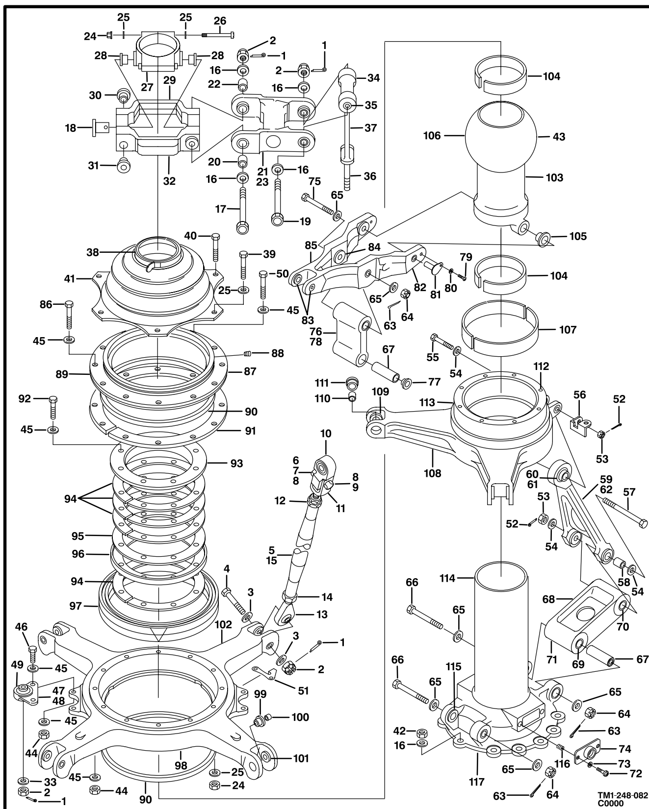
Figure 81. Controls Installation,Pylon Swashplate and Support
