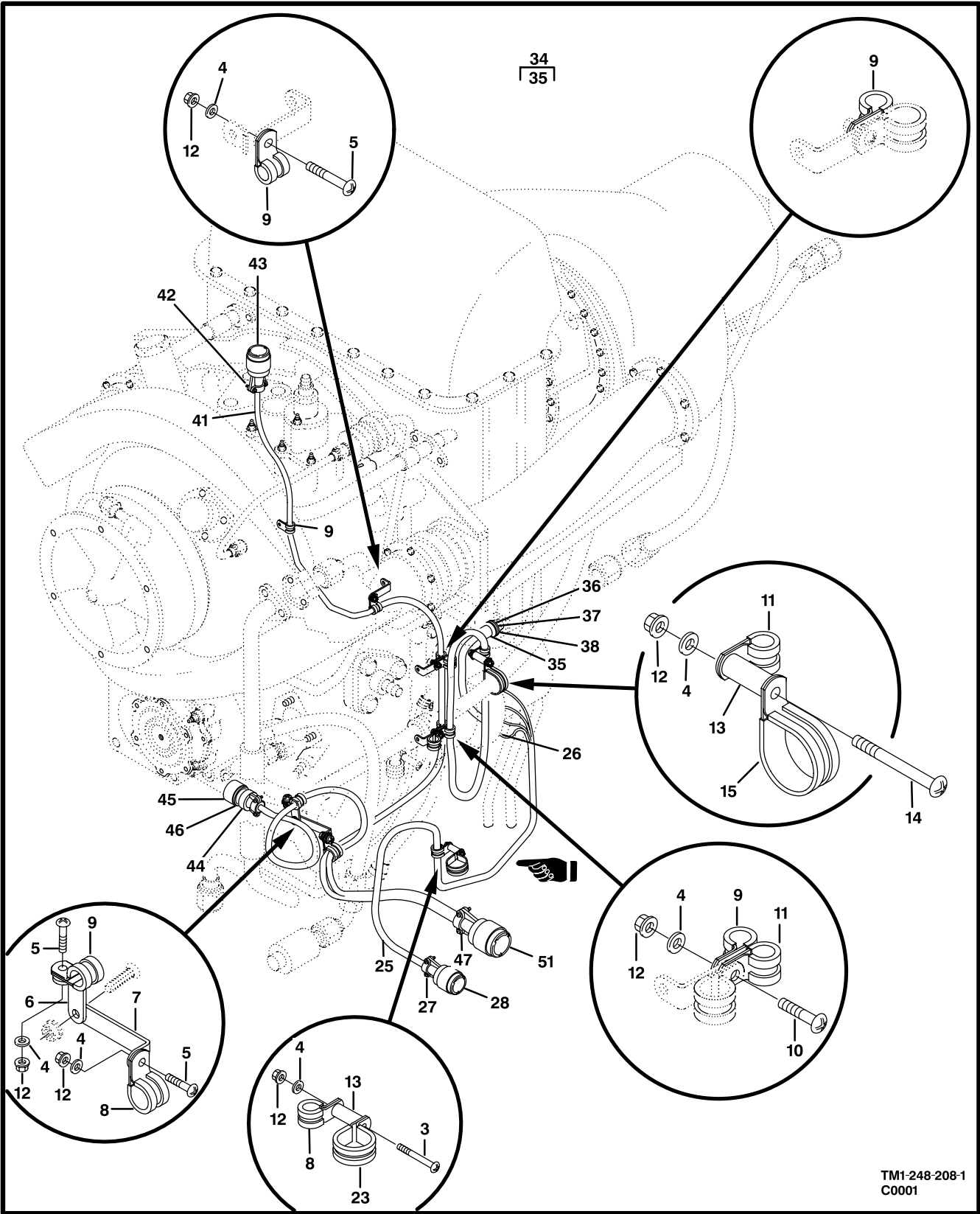
Figure 203. Electrical System,Power Plant (Sheet 1 of 2)
