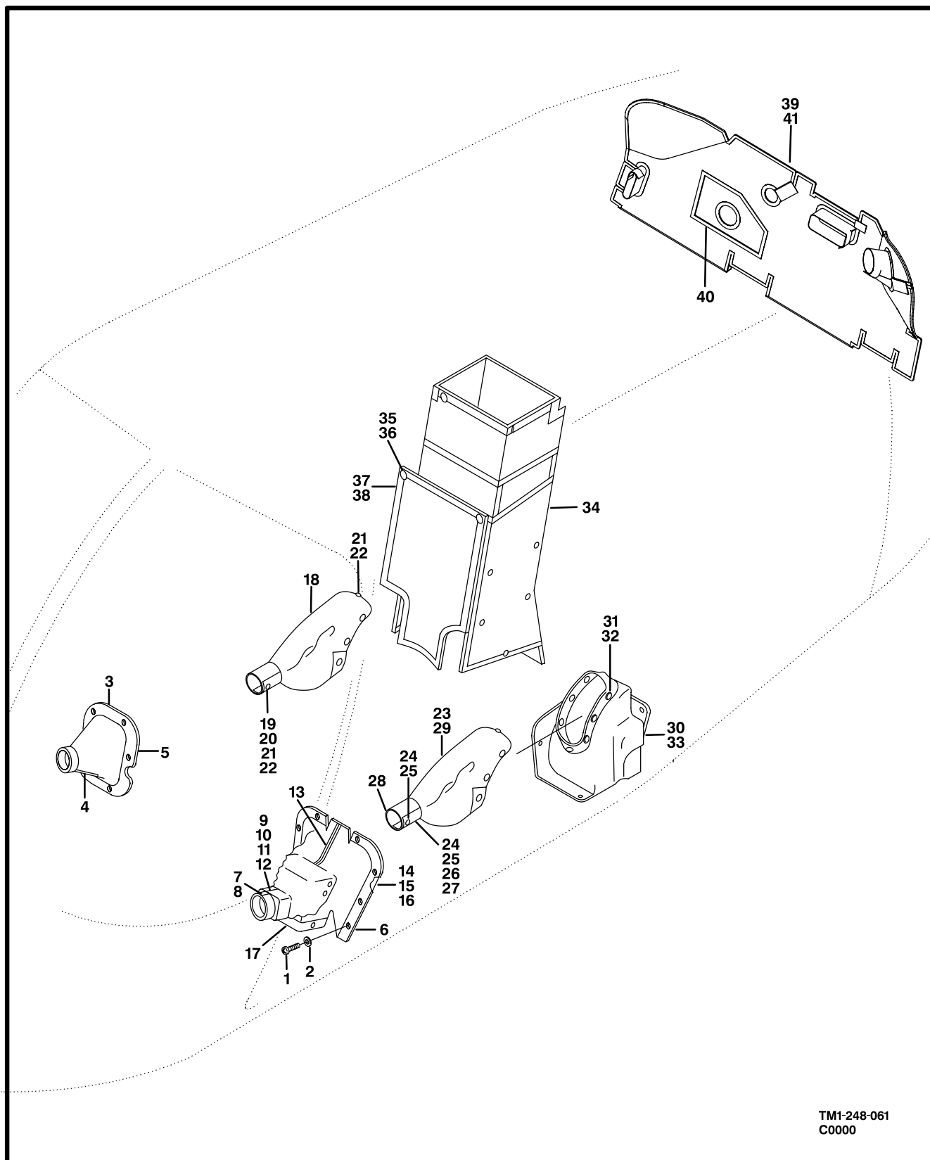
Figure 60. Soundproofing Installation
