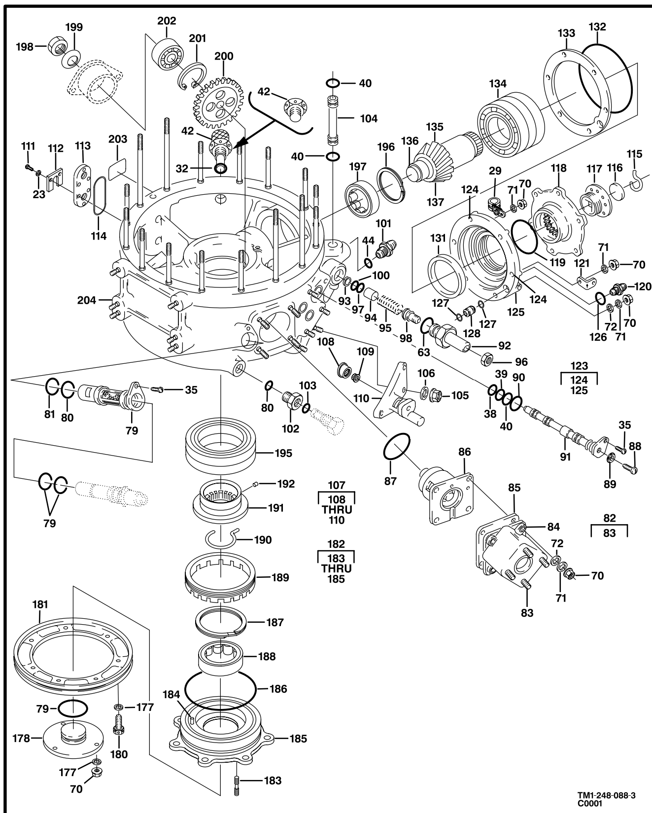
Figure 86. Transmission and Mast Assembly (Sheet 3 of 4)
