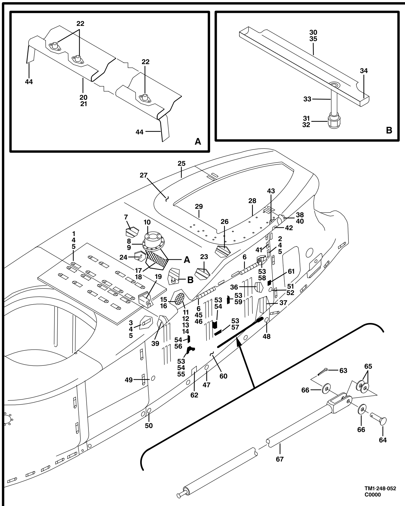
Figure 51. Cowl Assembly,Upper,Engine
