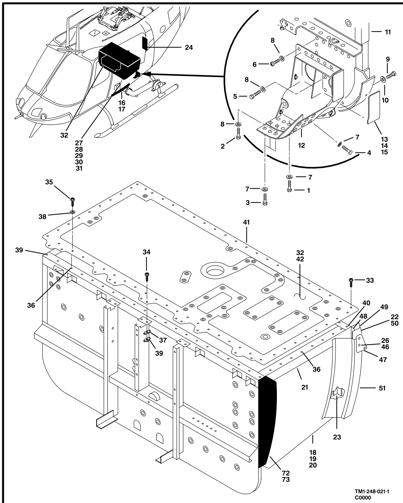
Figure 21. MOD-Fuel Cavity (Sheet 1 of 4)
