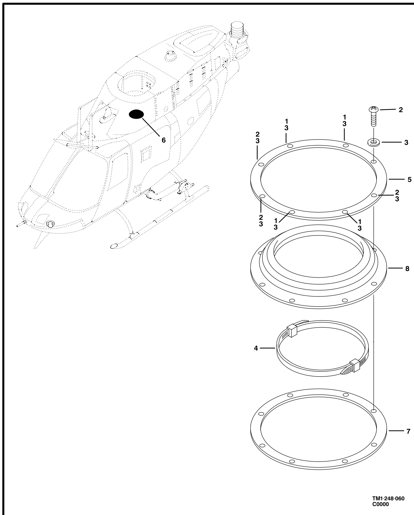
Figure 59. Seal Installation, Transmission to Roof
