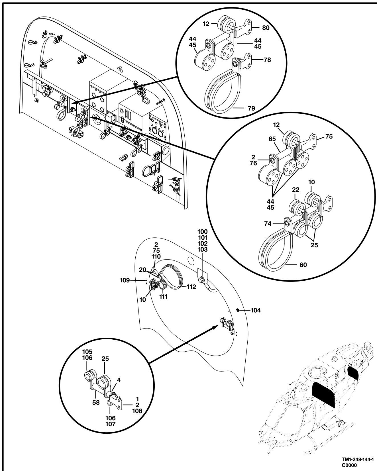
Figure 139. Electrical Installation,Bulkhead (Sheet 1 of 3)
