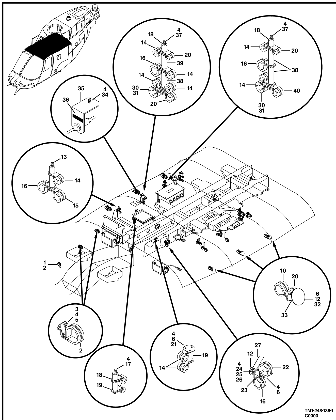
Figure 133. Electrical Installation,Bulkhead (Sheet 1 of 2)
