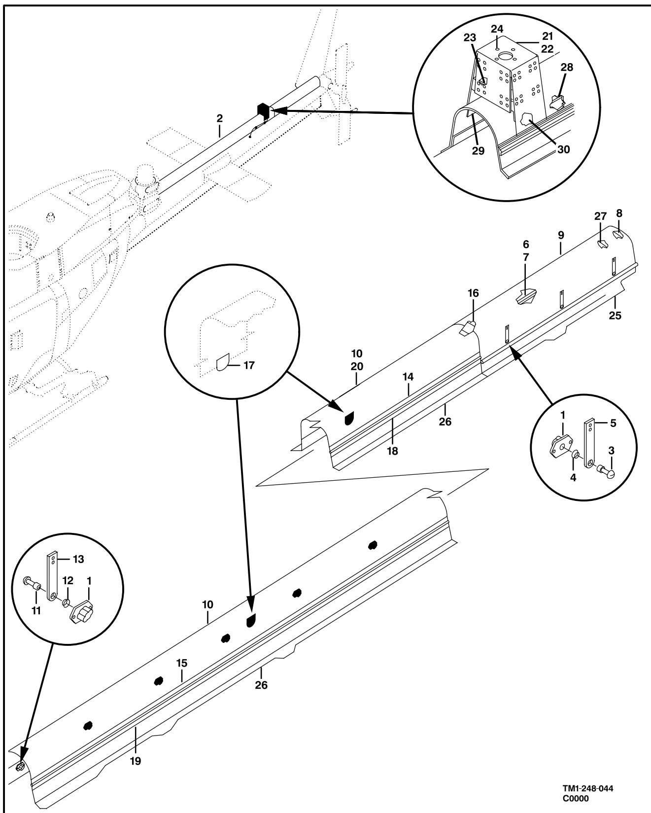
Figure 44. Cover Installation
