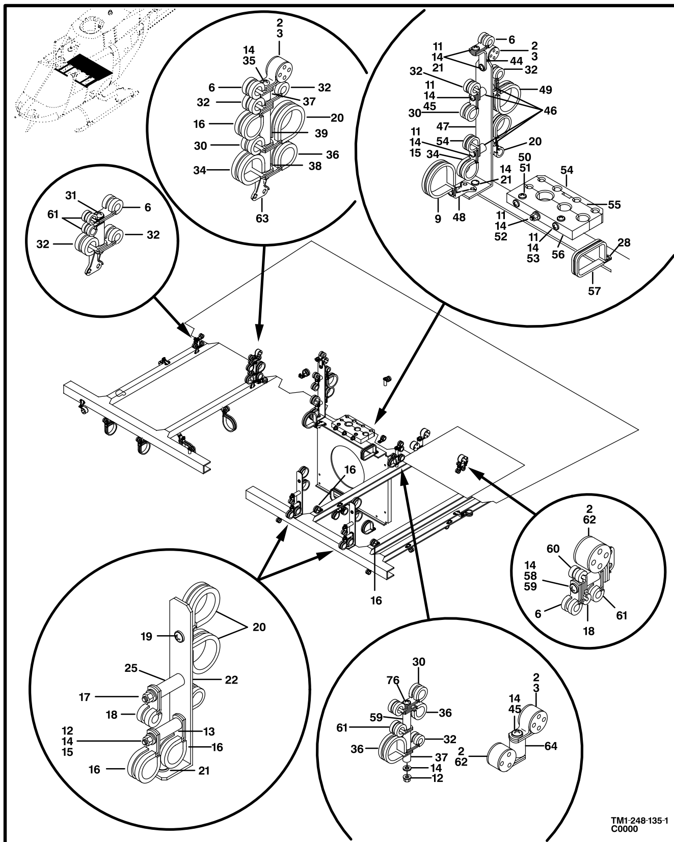
Figure 130. Electrical Installation, Shelf (Sheet 1 of 2)
