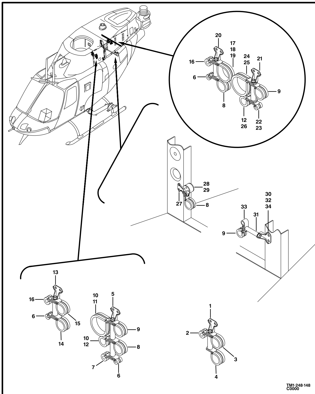
Figure 143. Electrical Installation
