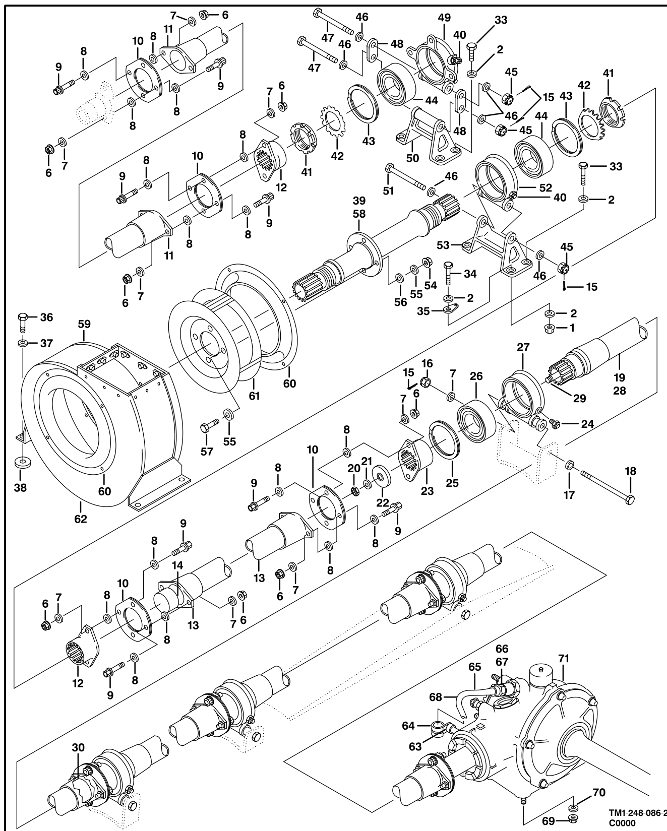
Figure 84. Drive System Installation (Sheet 2 of 2)
