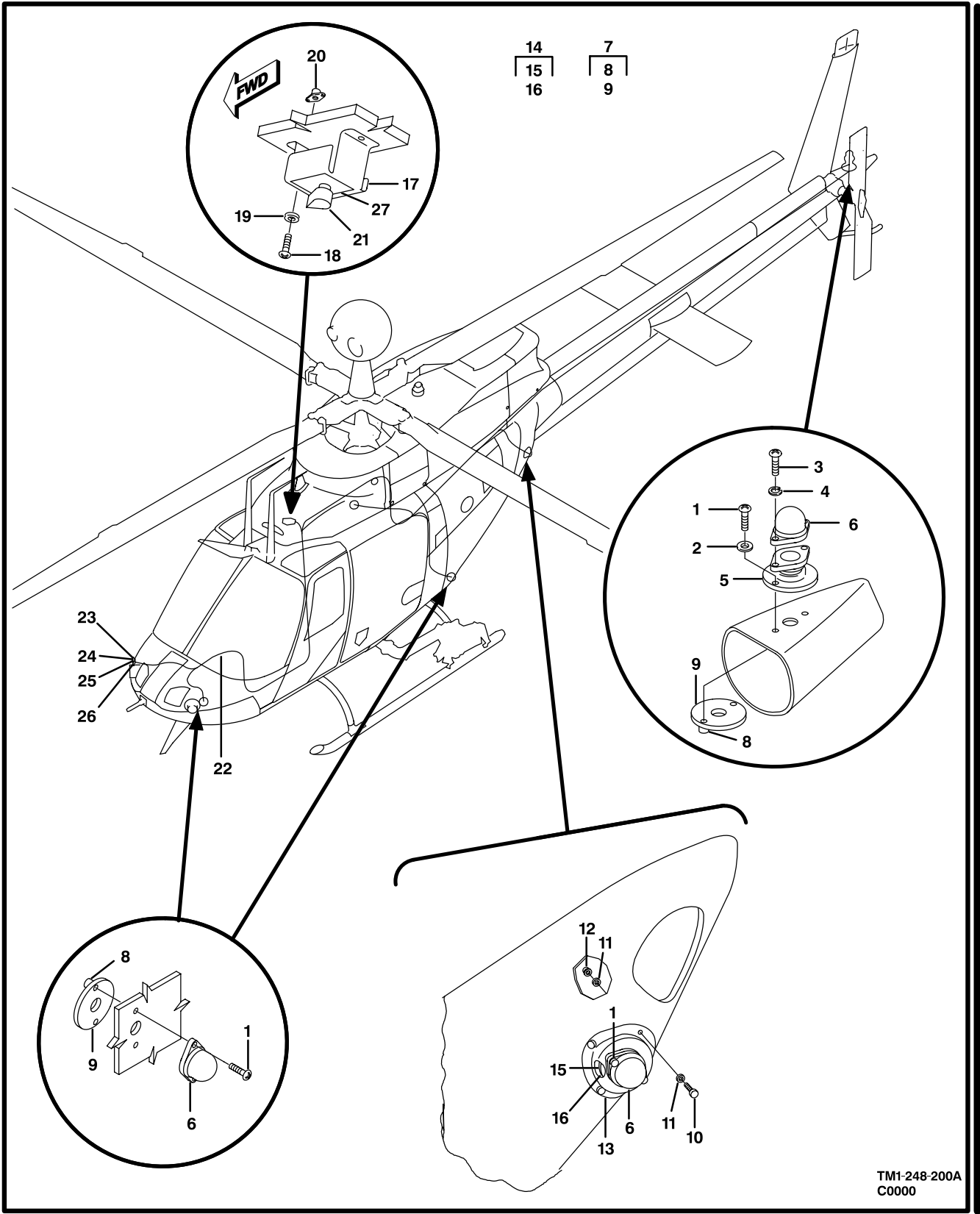
Figure 200A. NVG Formation Lights Installation
