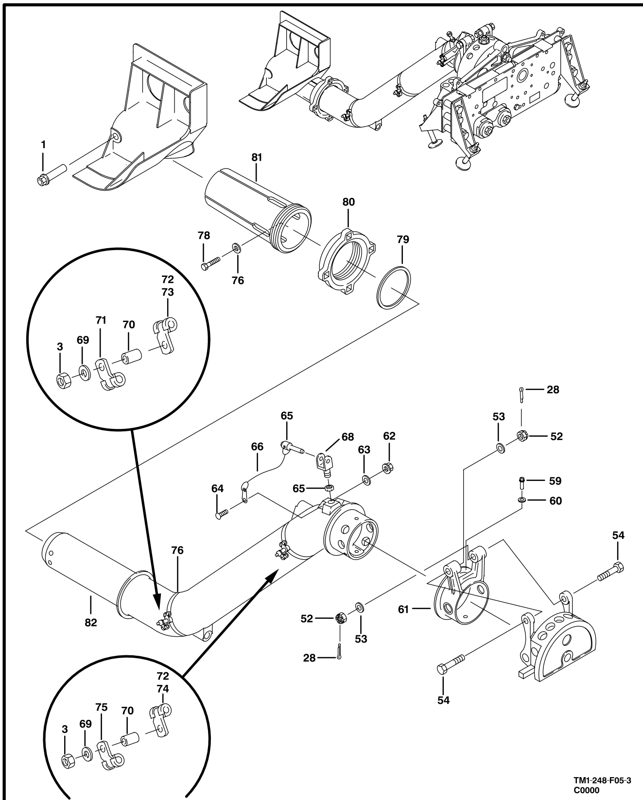
Figure F5. Universal Pylon Installation (Sheet 3 of 4)
