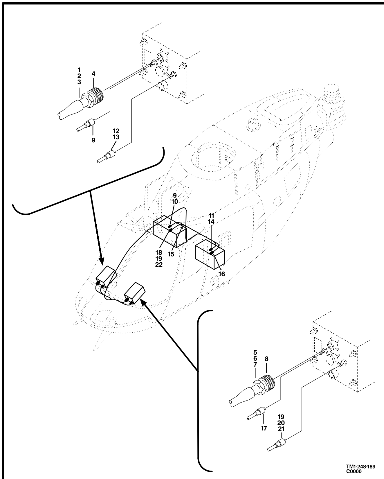
Figure 184. Cable Assembly,Control,Display System
