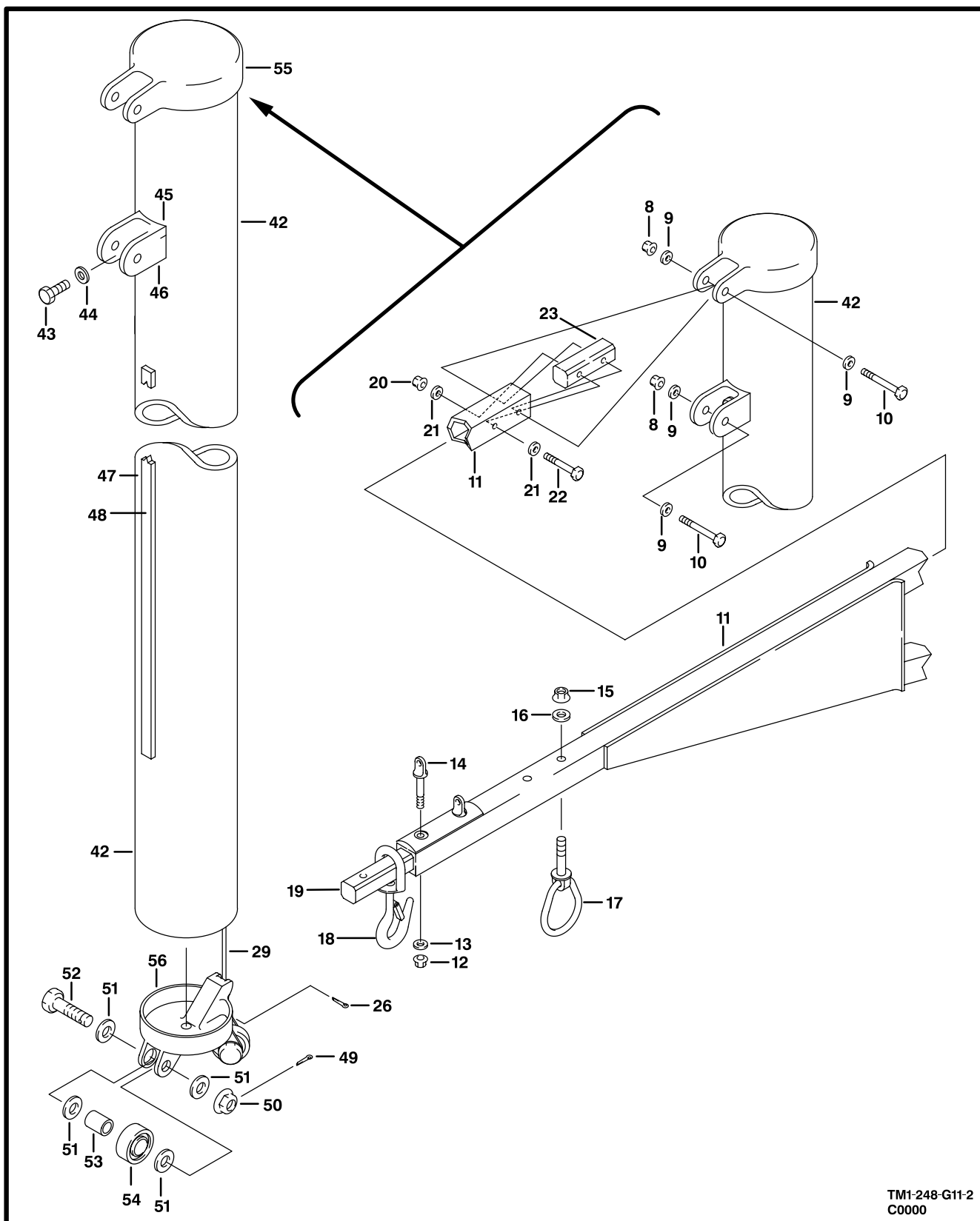
Figure G6. Hoist Installation, Mast Mounted Sight (Sheet 2 of 2)
