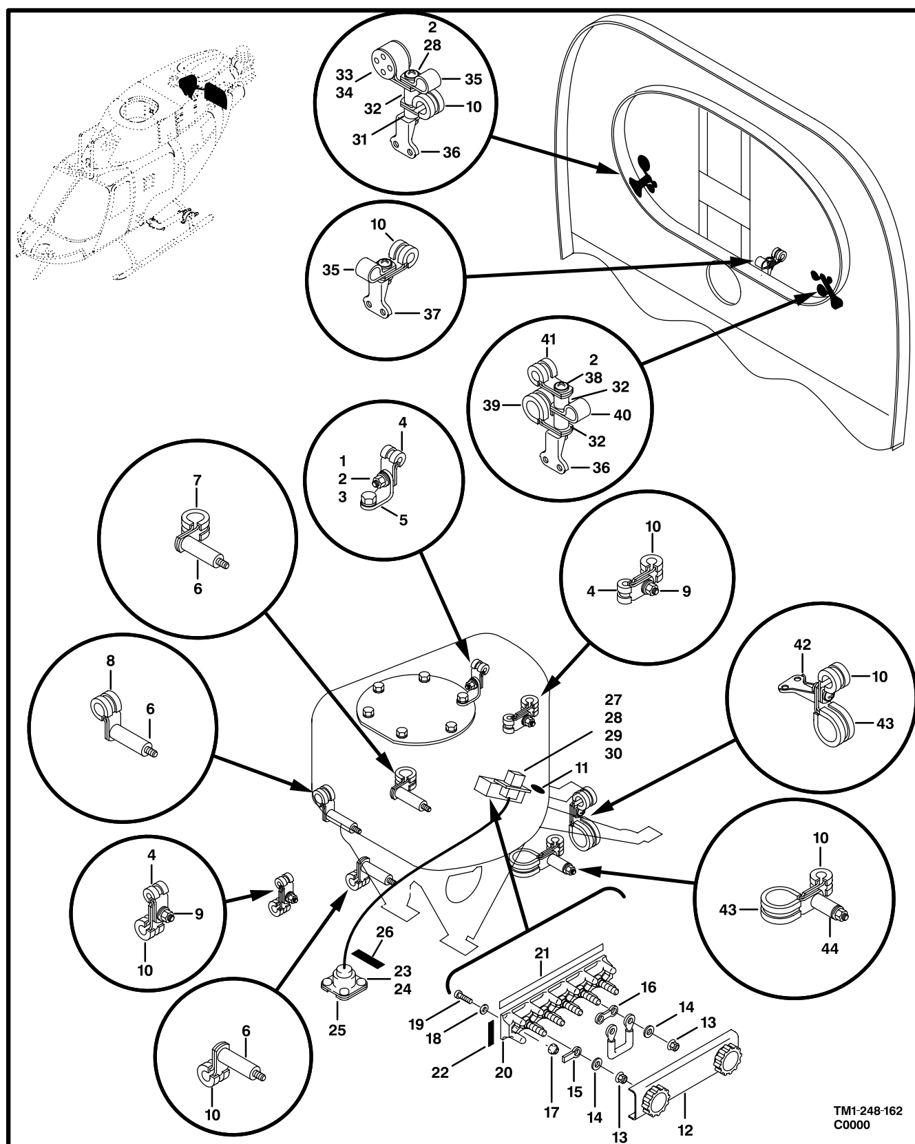
Figure 157. Electrical Installation
