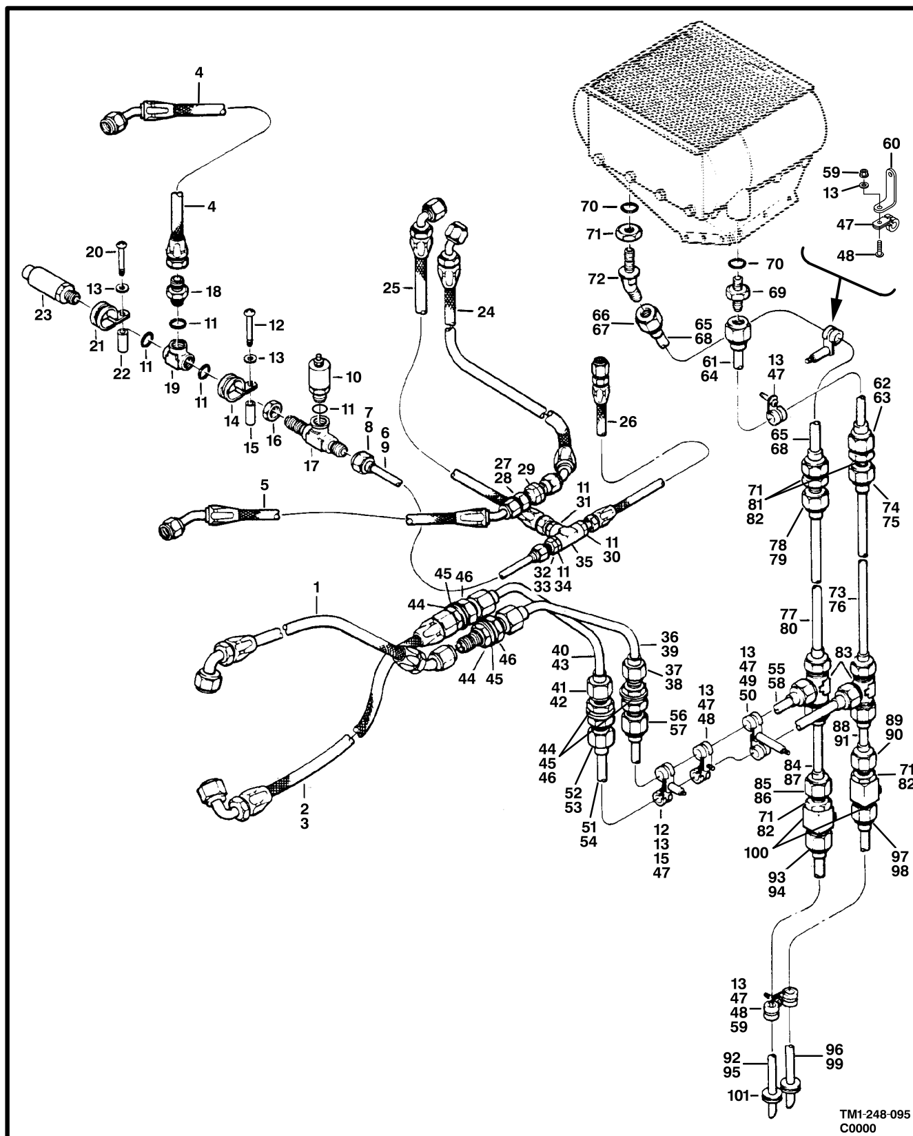
Figure 92. Oil System Installation
