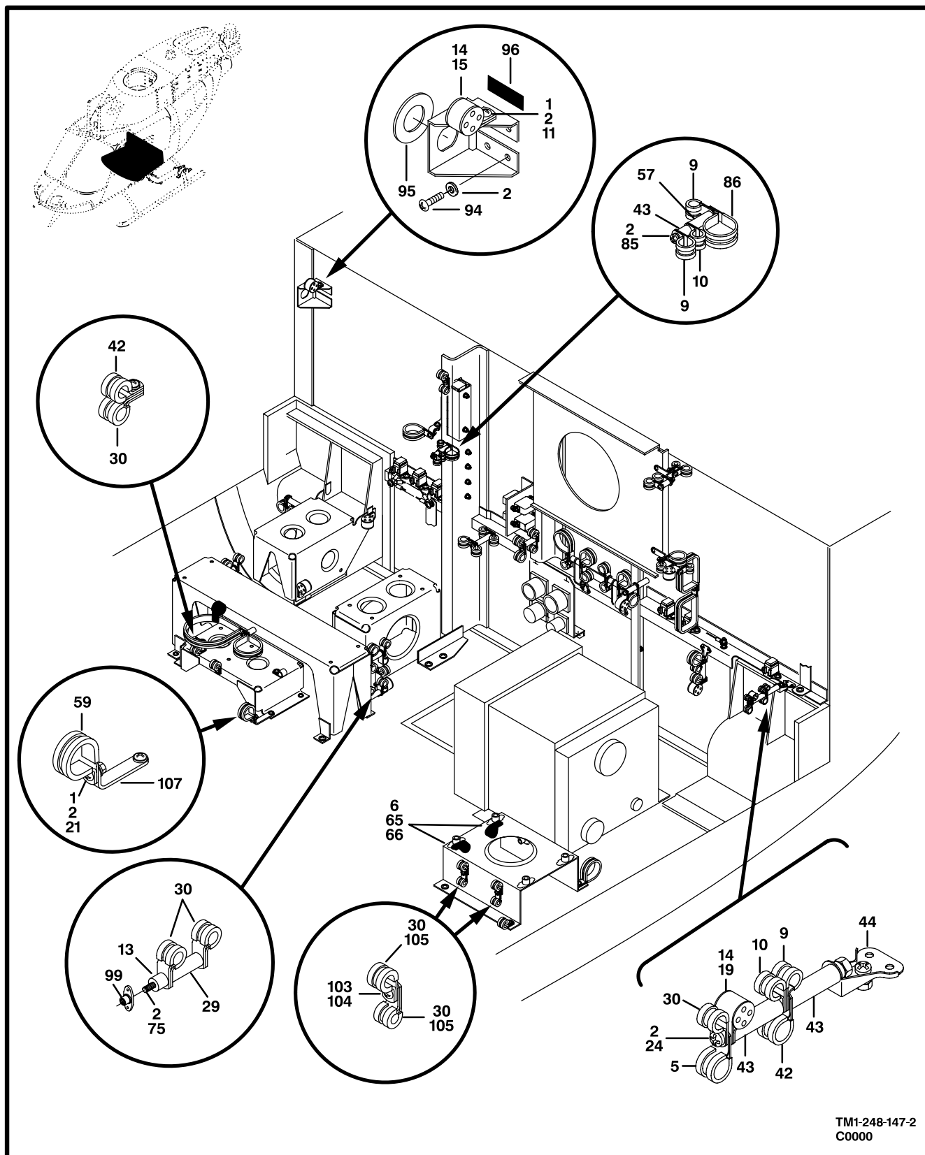
Figure 142. Electrical Installation, Bulkhead (Sheet 2 of 5)
