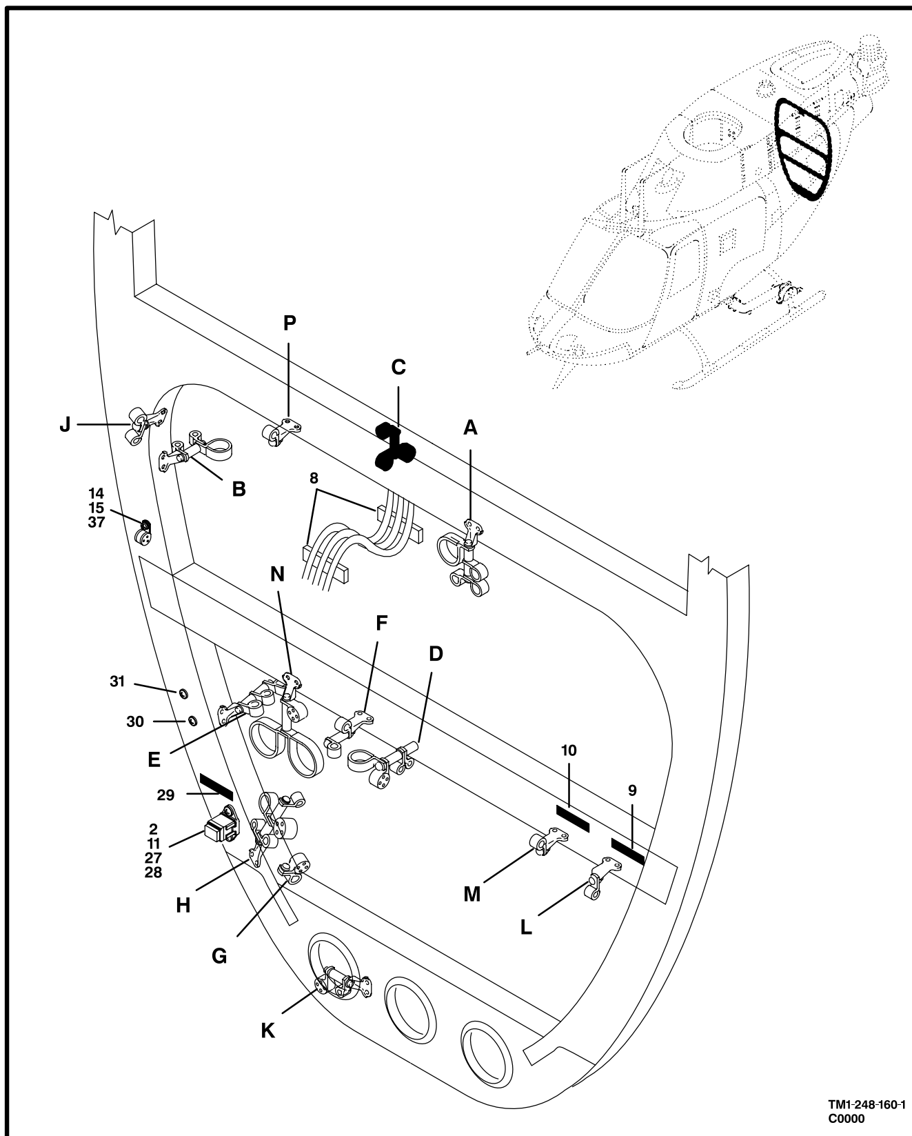
Figure 155. Electrical Installation (USBL EFF 89-0112 THRU 95-0079) (Sheet 1 of 2)
