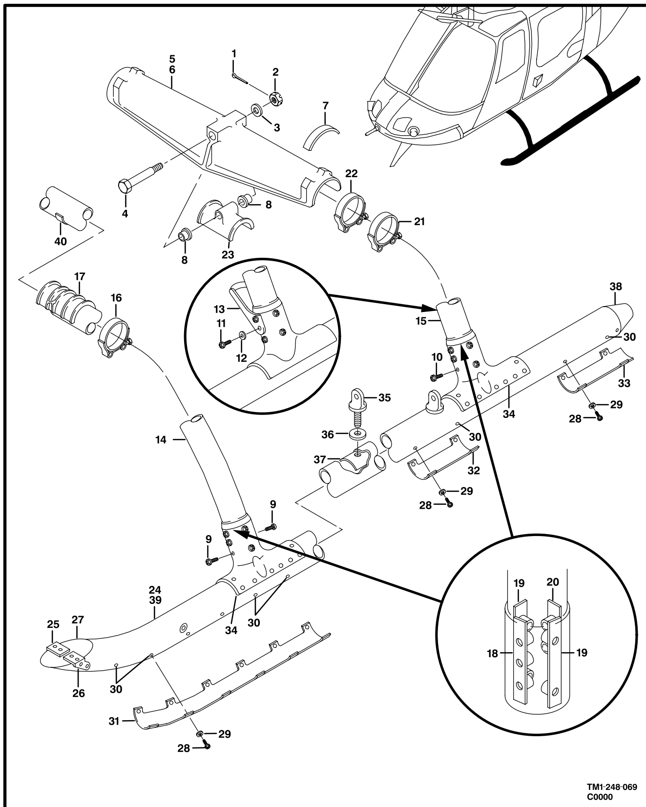
Figure 67. Landing Gear Assembly
