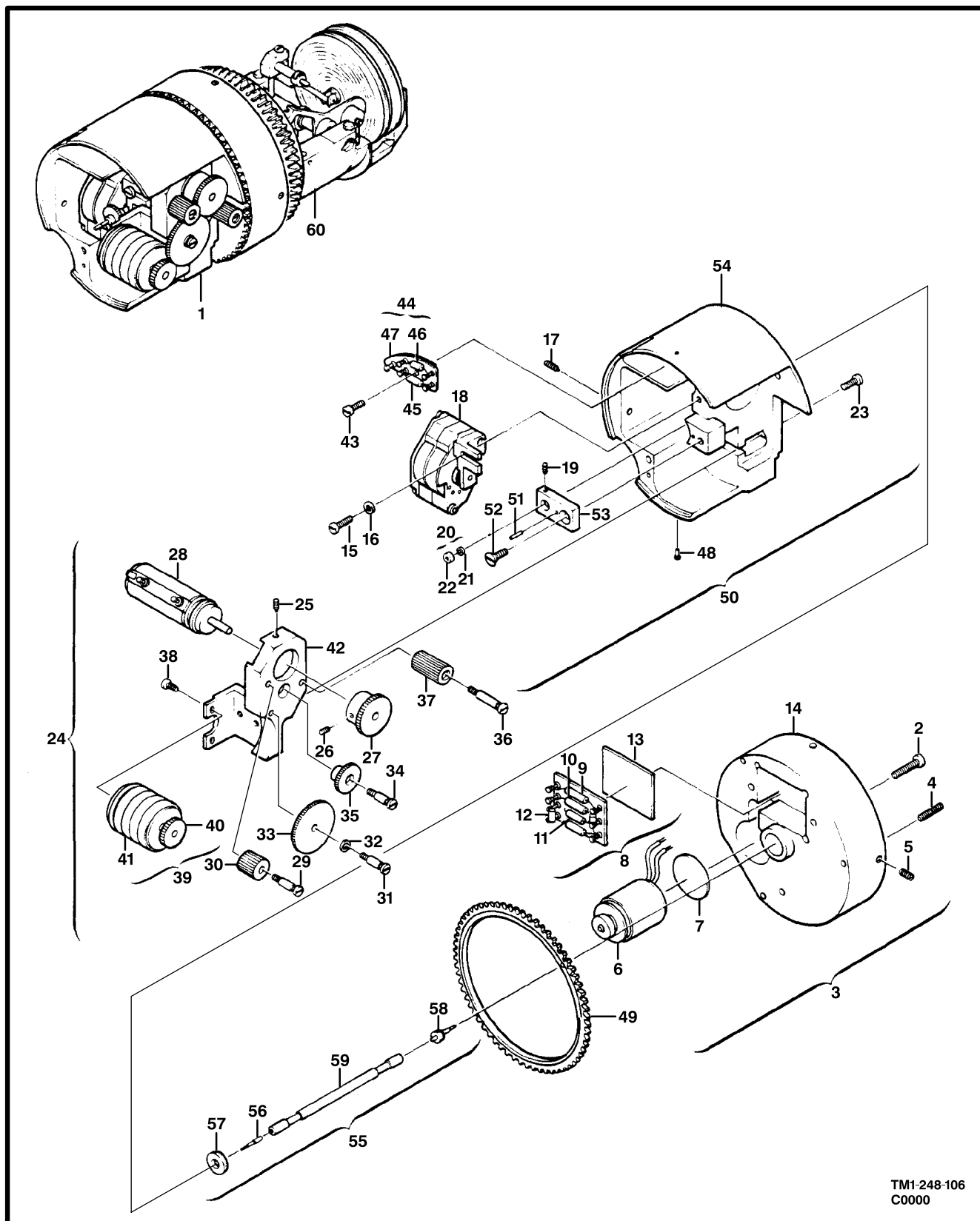
Figure 101. Barometric Counter Assembly
