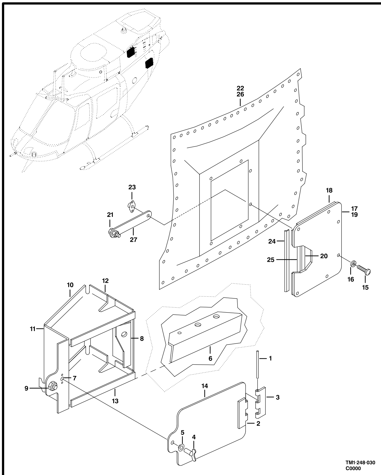
Figure 29. Support Installation
