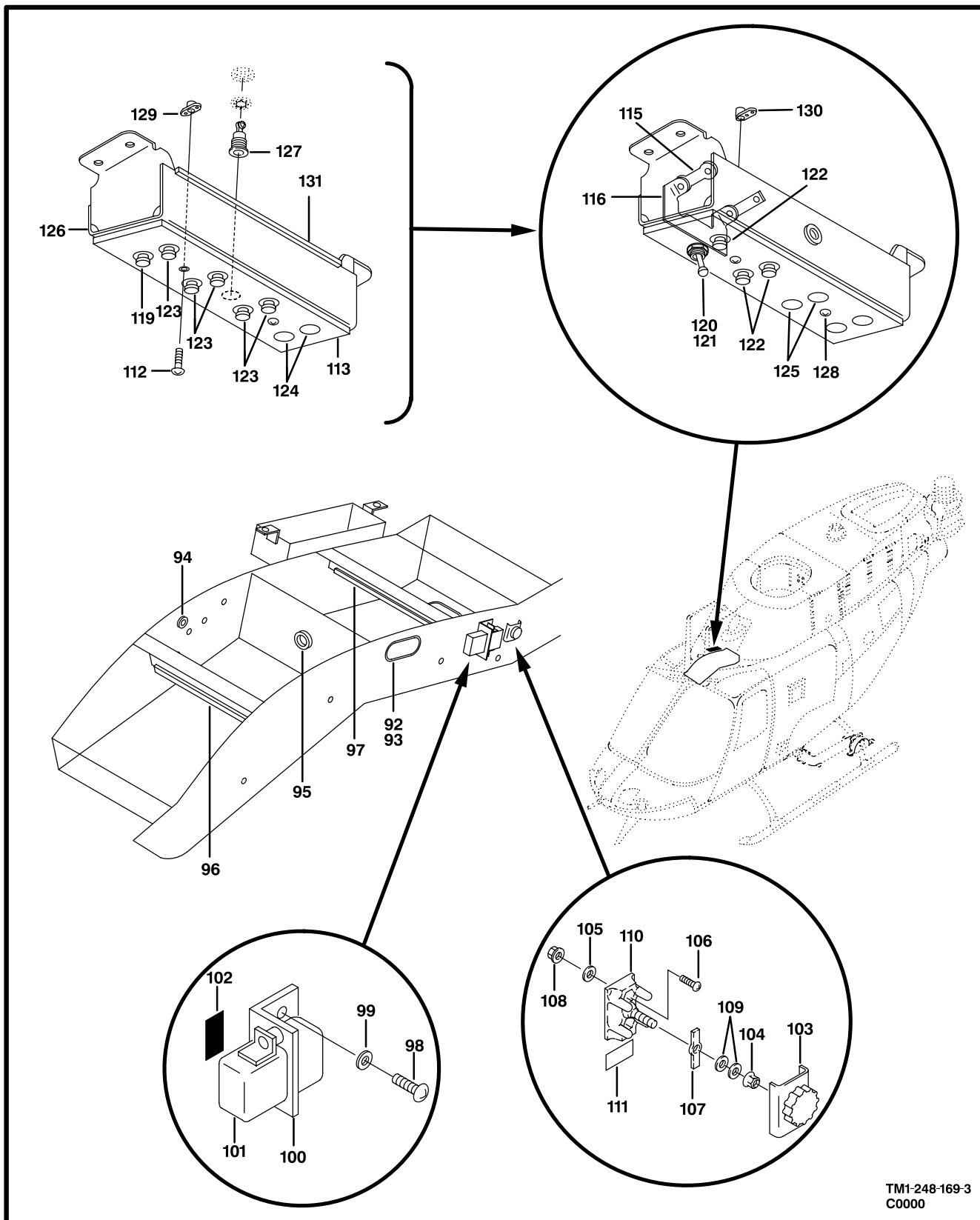
Figure 164. Console Installation, Overhead Electrical (Sheet 3 of 4)
