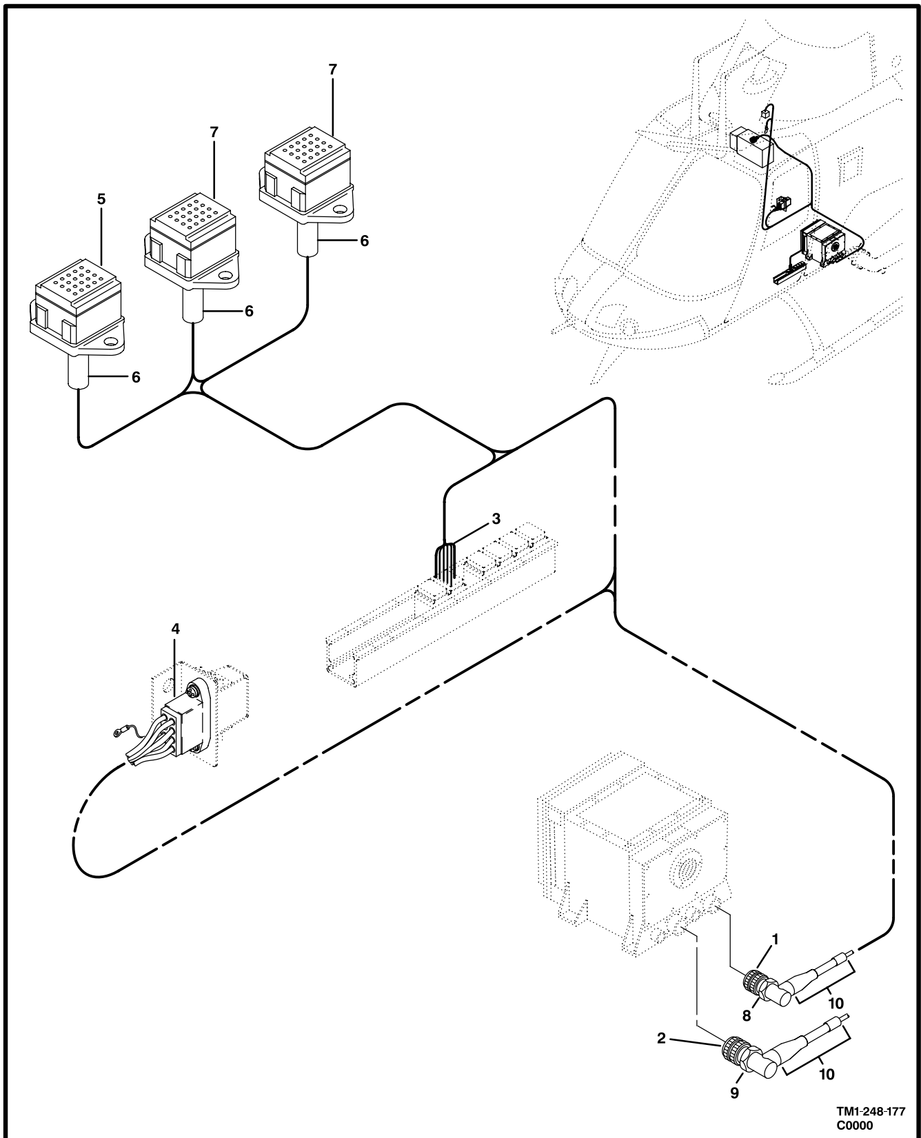
Figure 172. Cable Assembly,EGI
