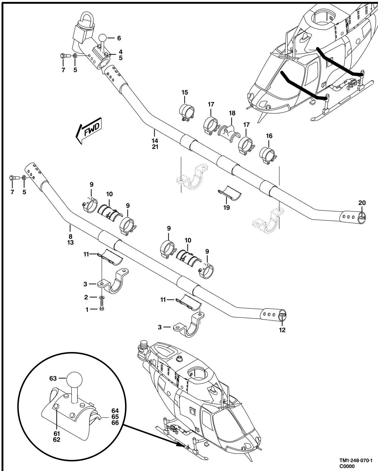
Figure 68. Landing Gear Installation (Sheet 1 of 2)
