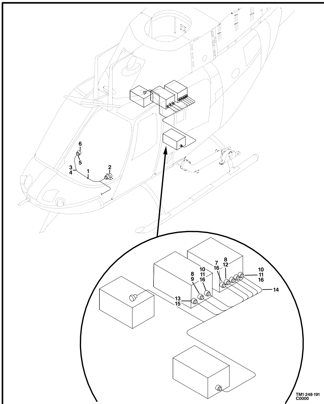
Figure 186. Cable Assembly, Mast Mounted Sight
