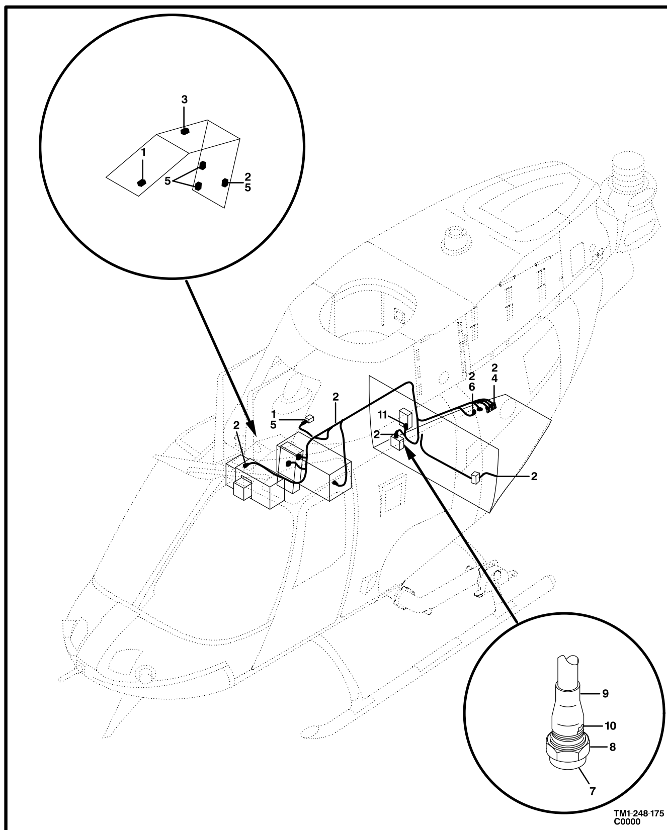
Figure 170. Cable Assembly, AC Power System
