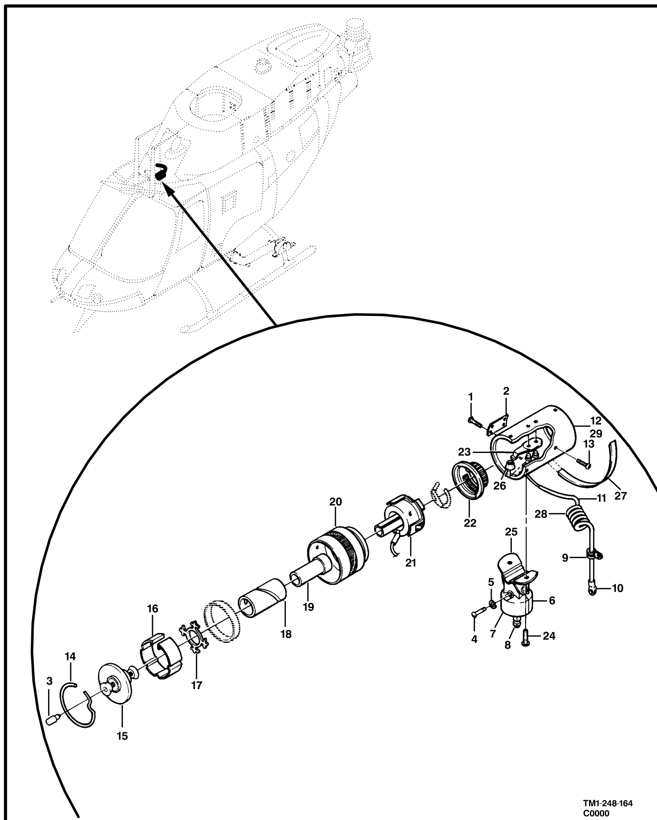
Figure 159. Light,Cockpit Utility
