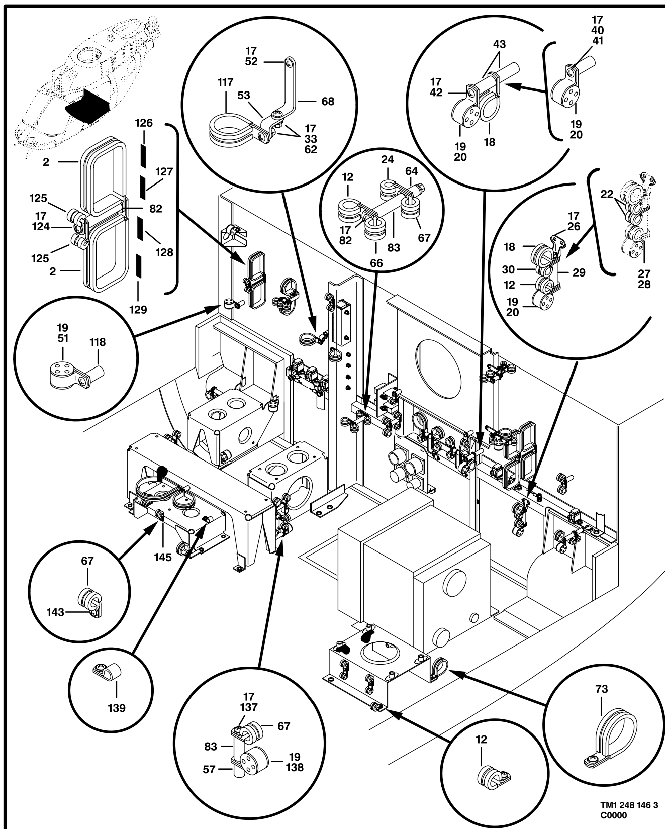
Figure 141. Electrical Installation,Bulkhead (Sheet 3 of 4)
