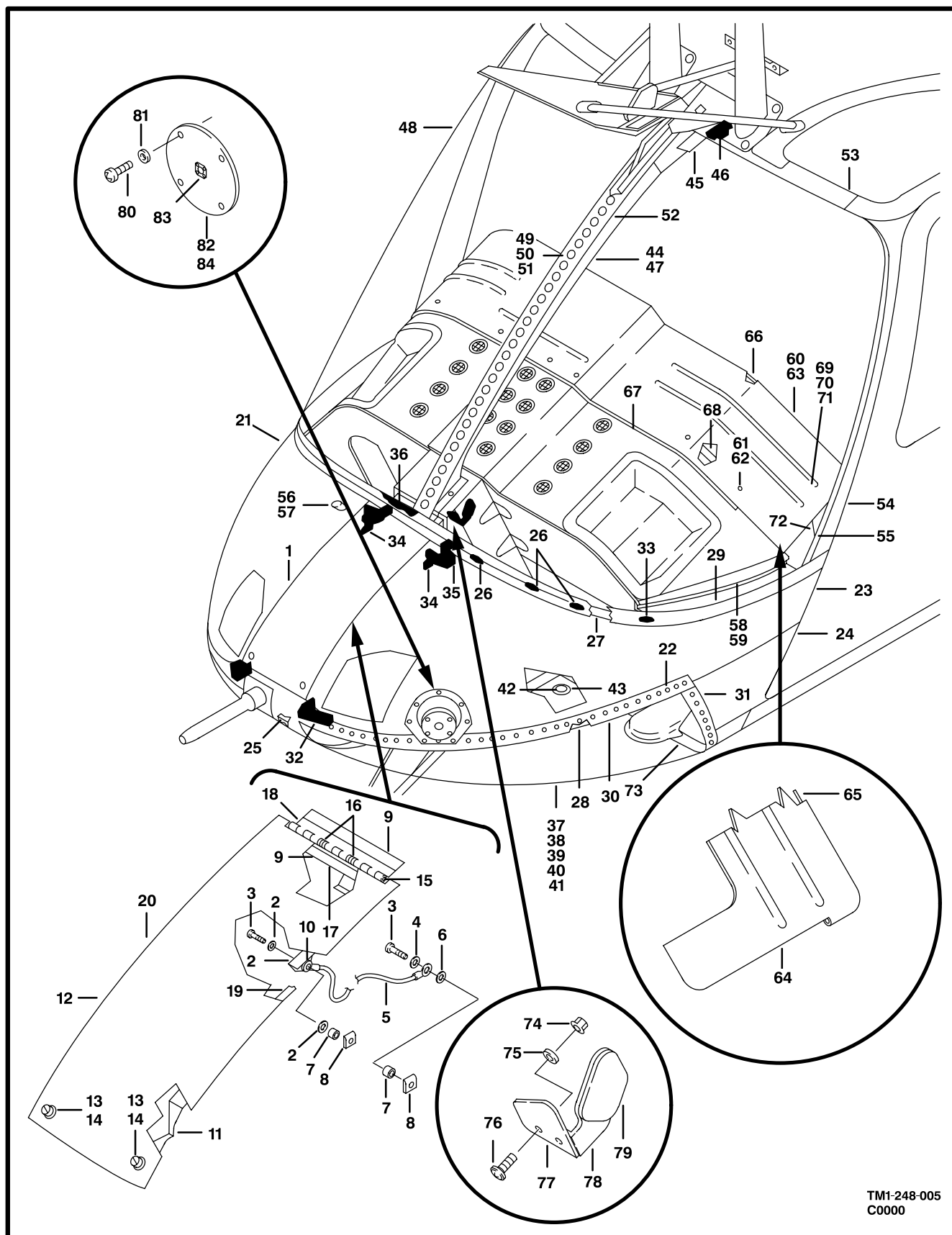
Figure 5. Nose Installation
