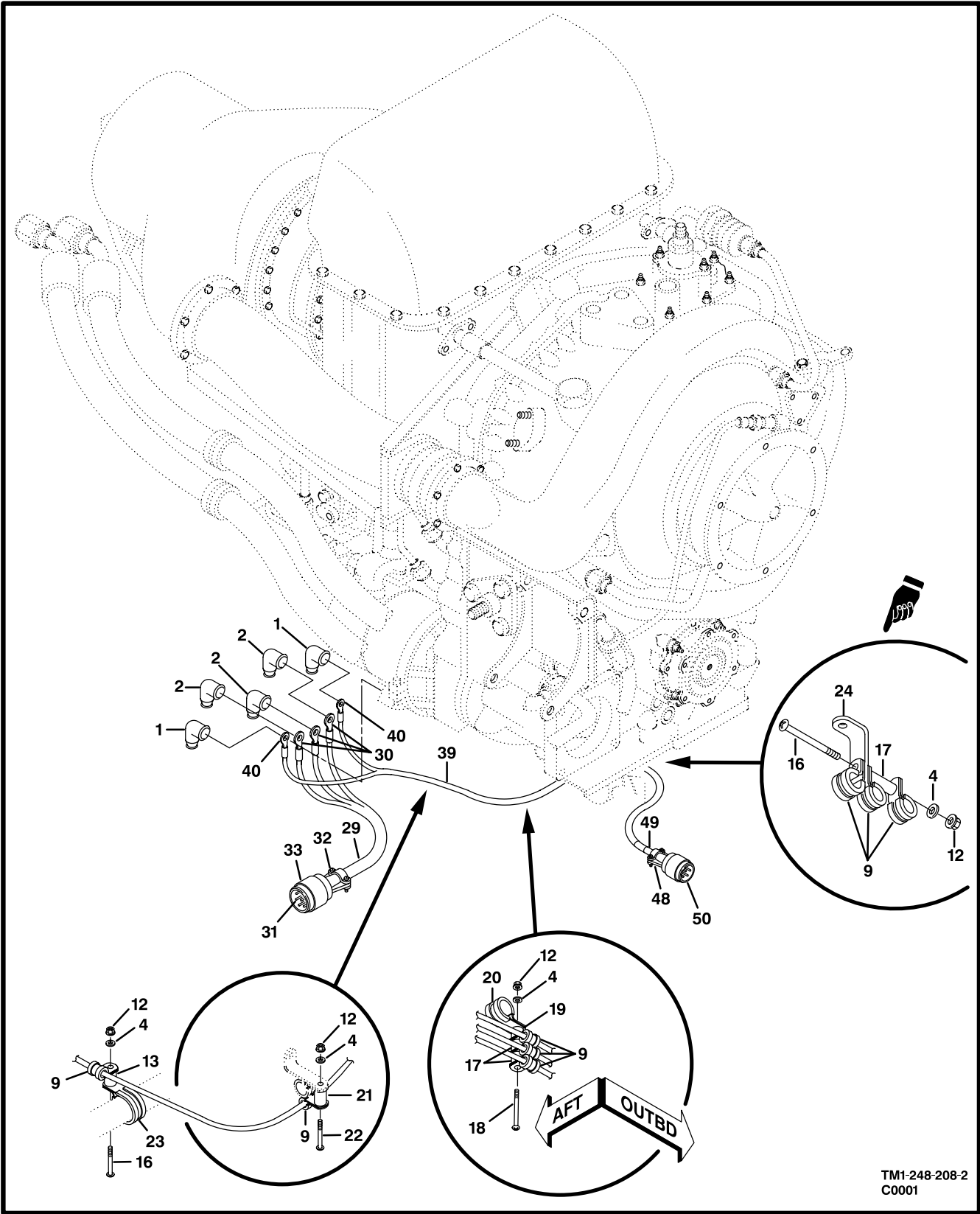
Figure 203. Electrical System,Power Plant (Sheet 2 of 2)
