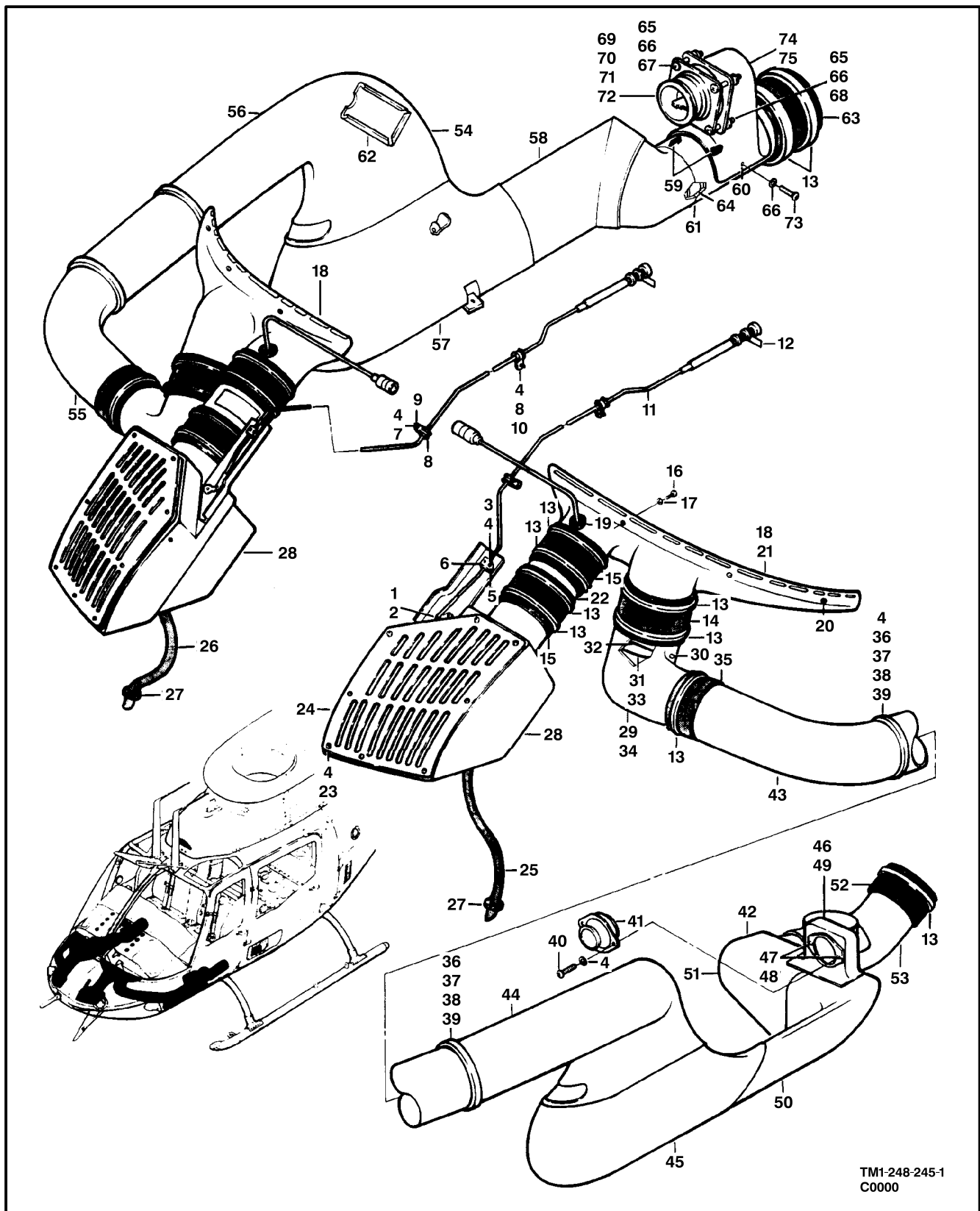
Figure 261. Environmental Control System (Sheet 1 of 3)
