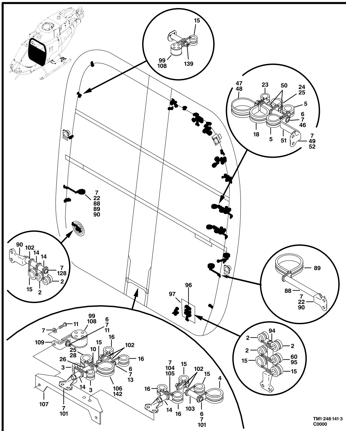
Figure 136. Electrical Installation,Bulkhead (Sheet 3 of 4)
