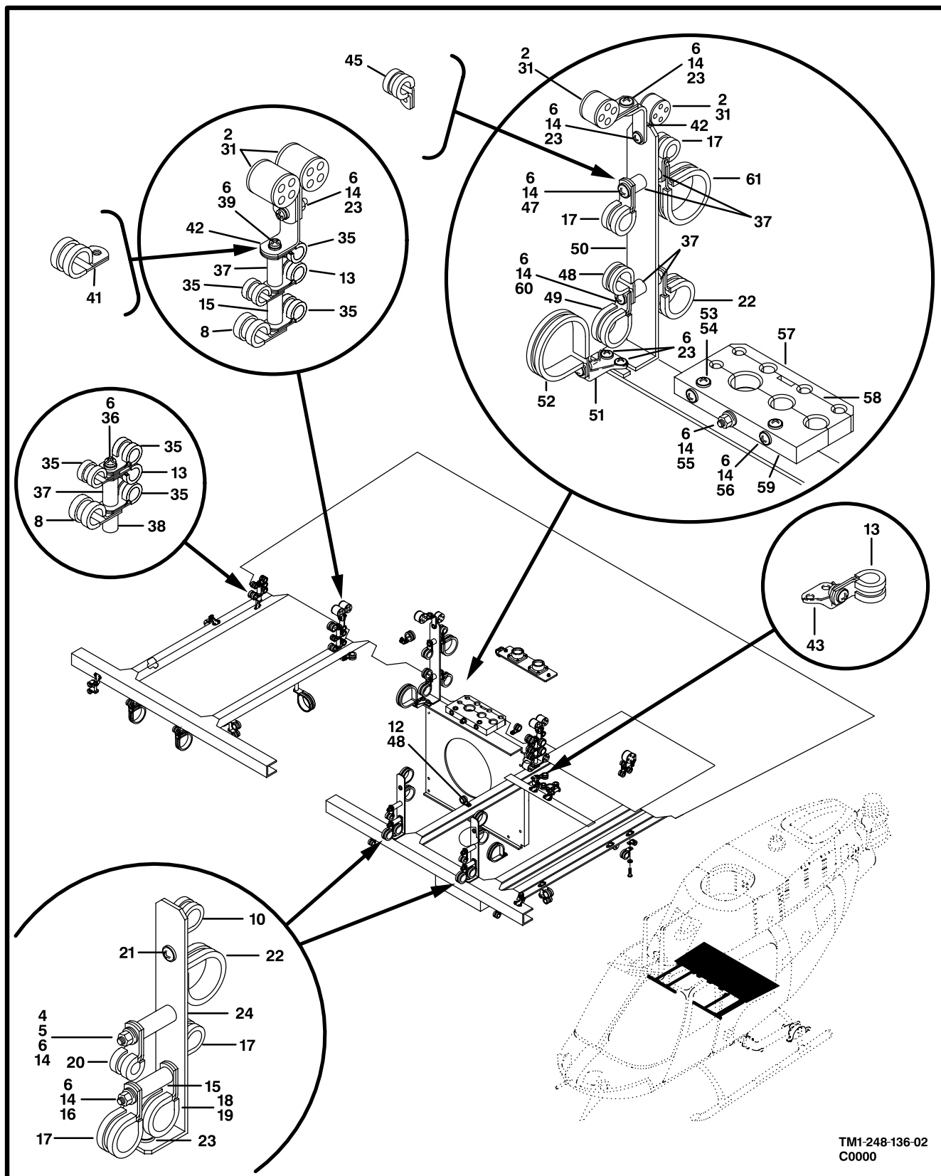
Figure 131. Electrical Installation, Shelf (Sheet 2 of 2)
