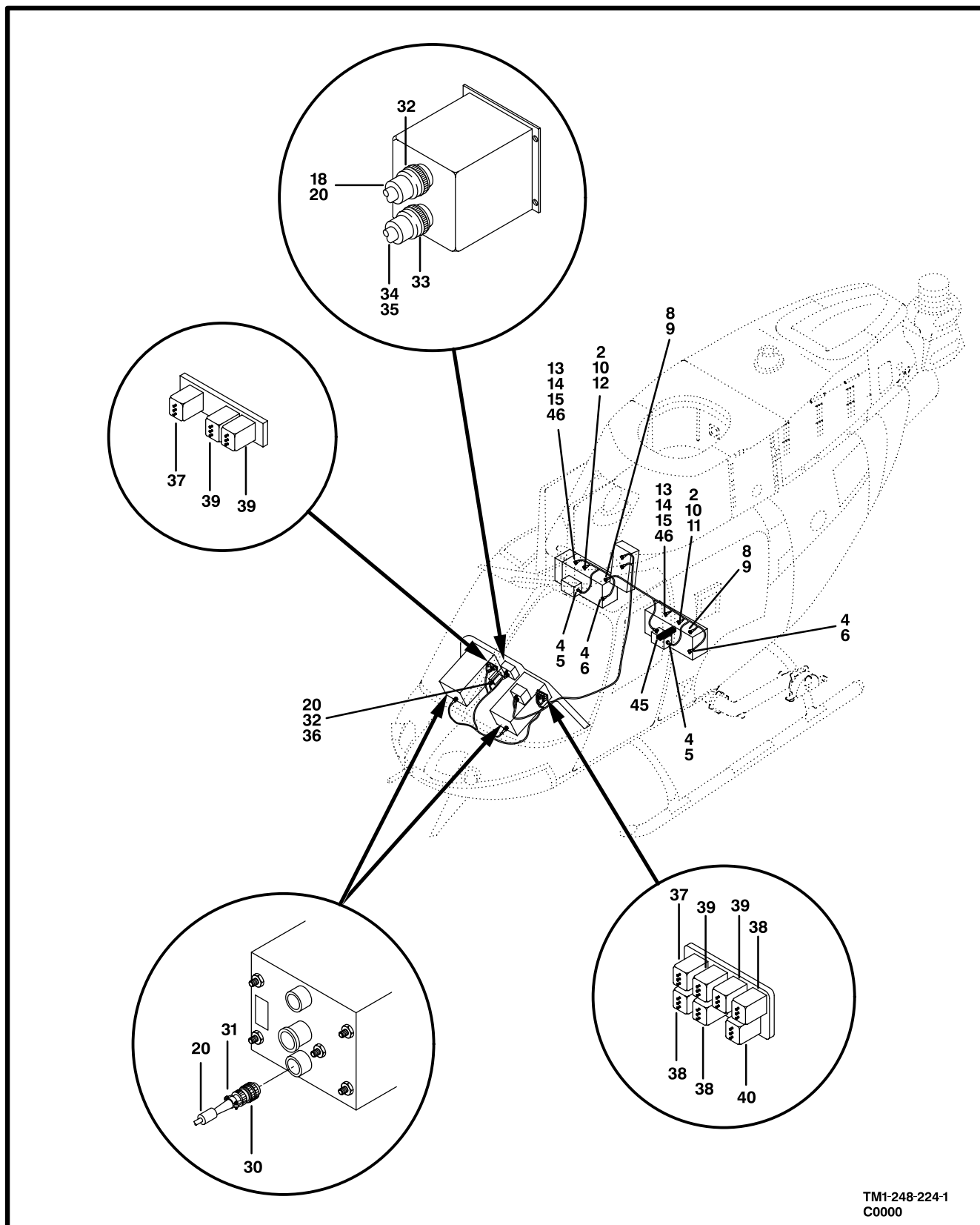
Figure 218. Cable Assembly,Control Display System (Sheet 1 of 2)
