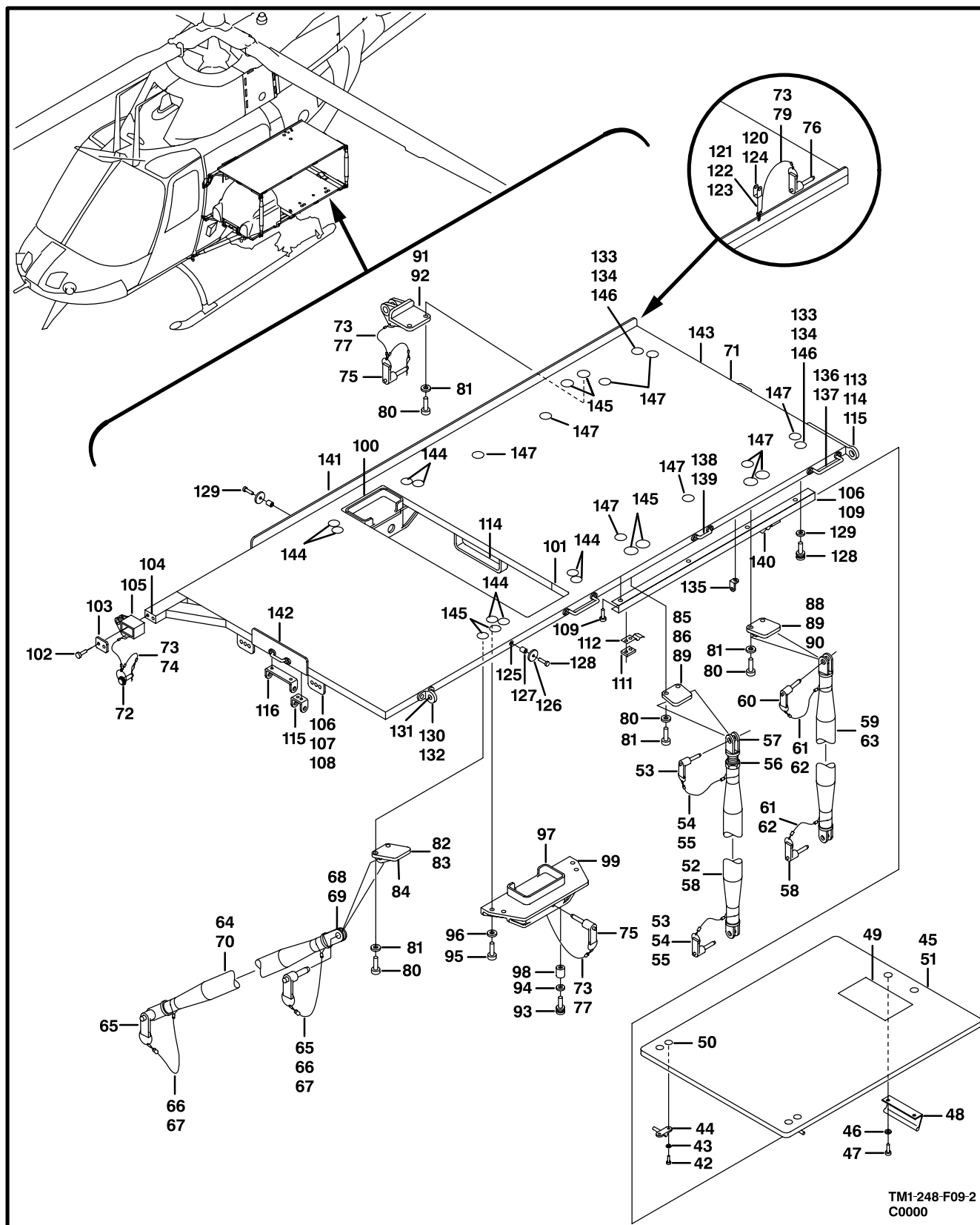
Figure F9. Aux Equipment Kit (Sheet 2 of 2)
