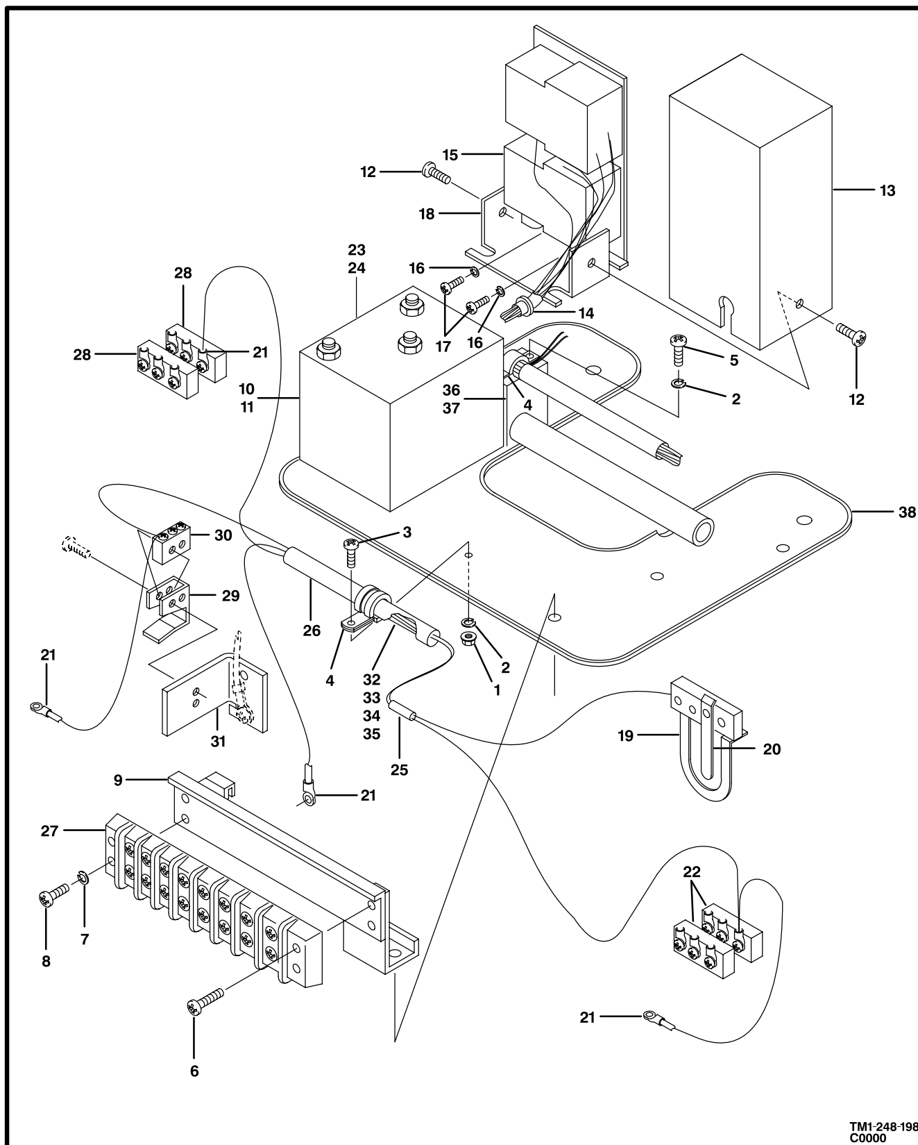
Figure 193. Base/Harness Assembly
