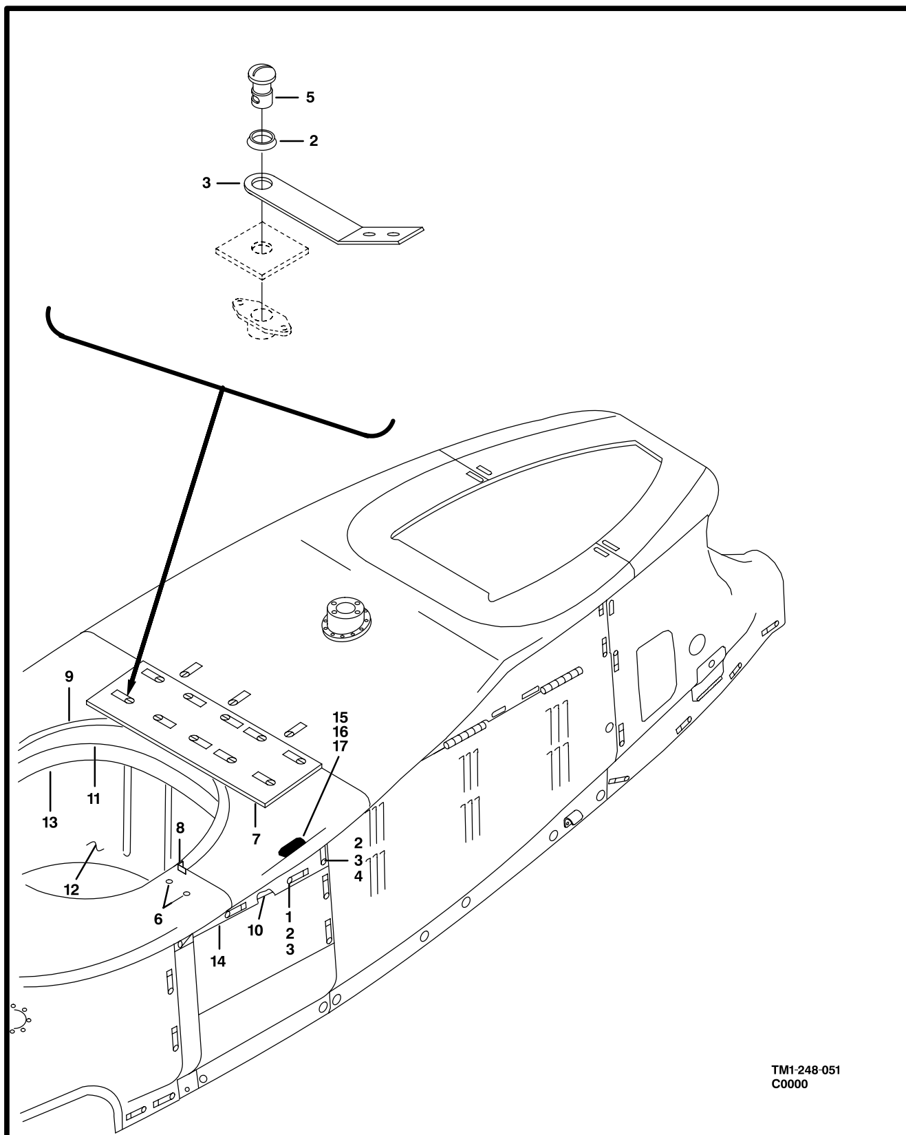
Figure 50. Shroud Assembly,Exhaust
